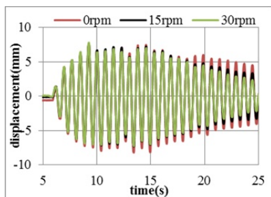
El-Centro wave PGA=0.1g
