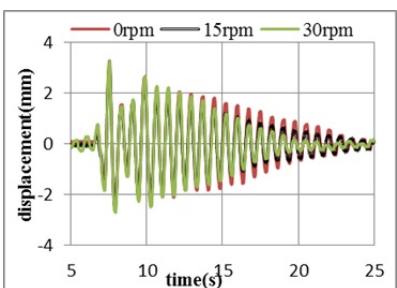
Kobe wave PGA=0.1g
