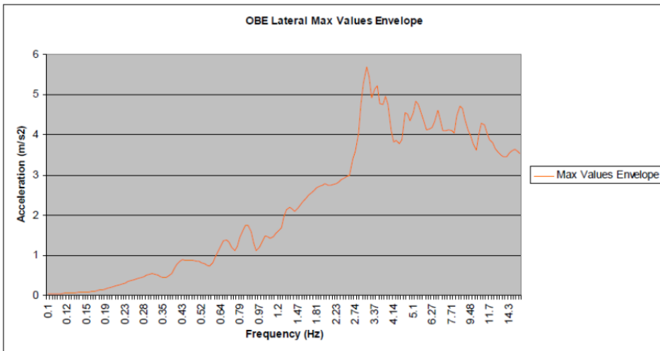
Figure 4: Horizontal response spectrum for OBE
