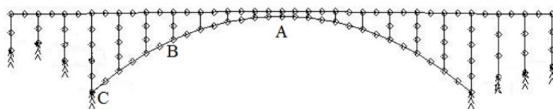
Figure 2: Finite element model
