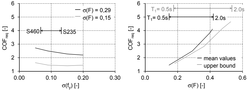
Figure 9: Required oversdesign factor COF for steel frames under seismic action: variation of yield strength (left) and of action (right)
