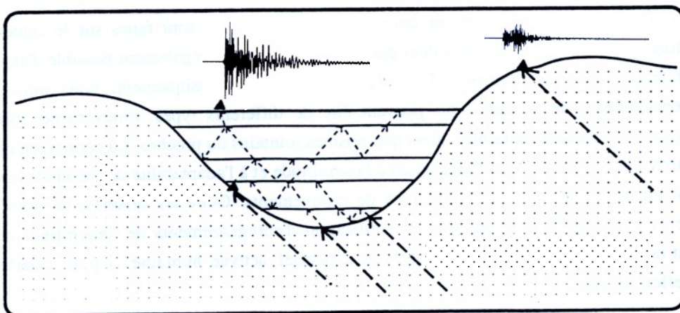
61 Figure 1: Illustration of site effects due to trapped waves in a sedimentary basin; ground 62 motion within the basin is significantly stronger than on an adjacent rock site
