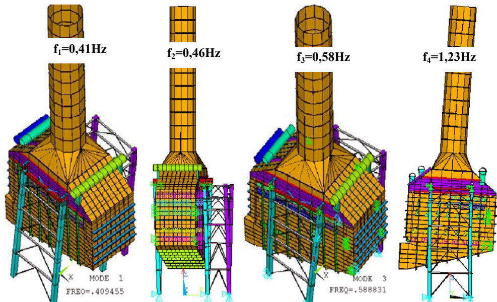
128 129 Figure 8: Eigenfrequencies and mode shapes of Model 4
