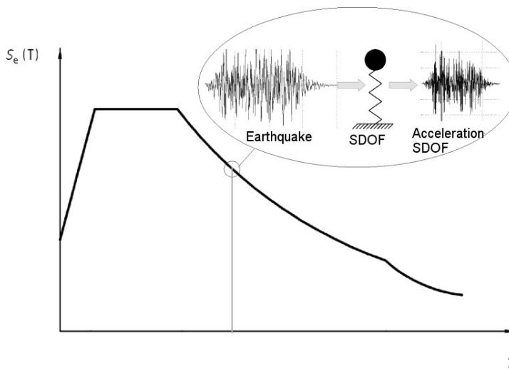
Figure 1: Generation of a response spectrum from an earthquake time record
