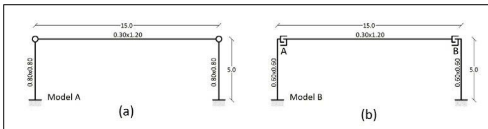
217 Figure 14: Geometric schemes; (a) beam with hinges; (b) system with devices
