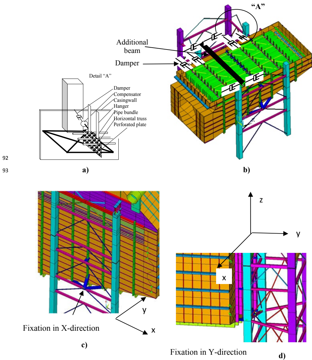
Figure 5: Discrete dampers on the pipe bundles (a) (b), casing fixed to the frame structure in the lower plane (c) (d)
