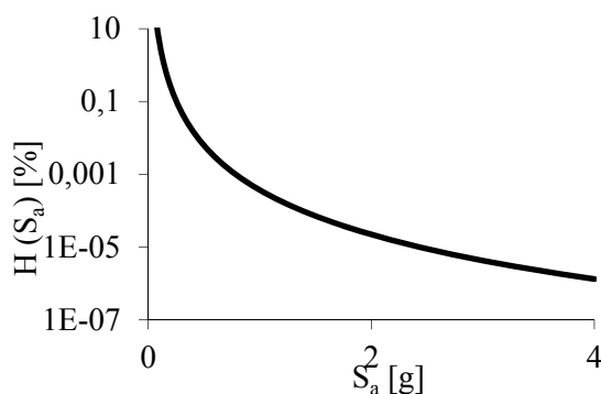
Figure 2: Site Specific Hazard Curve of Istanbul, Turkey ( T=2.2 s)
