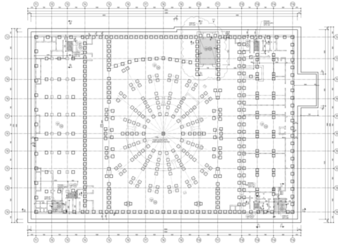
151 152 Figure 5: Tokamak Complex seismic isolation structure – Seismic isolation bearing 153 assembly arrangement
