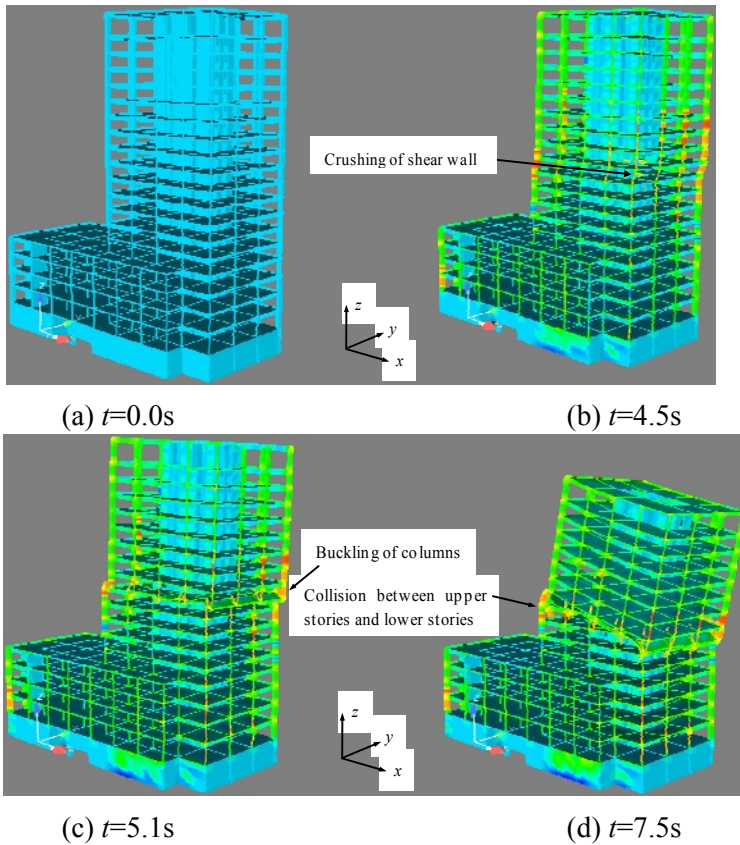
109 Figure 2: Collapse process of the 20-story frame-core tube building
