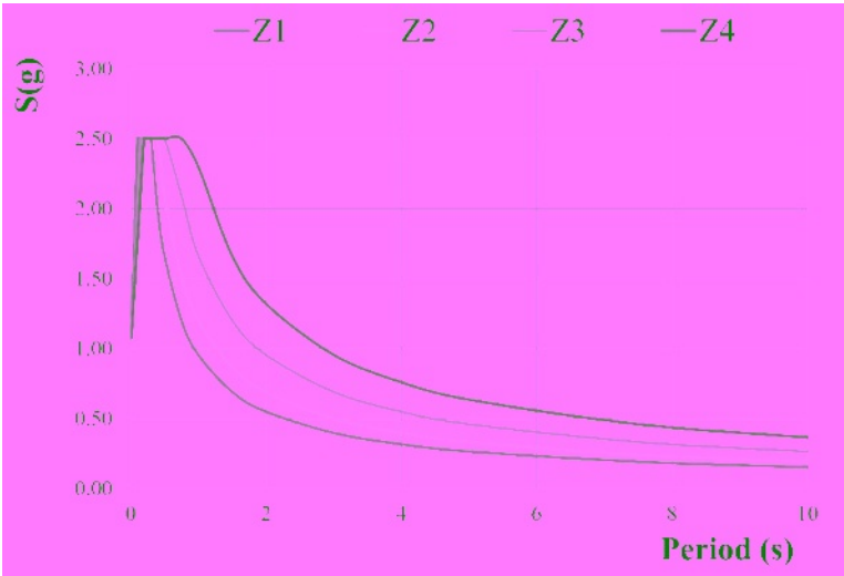
Figure 5: Elastic design acceleration spectra for different type of soil
