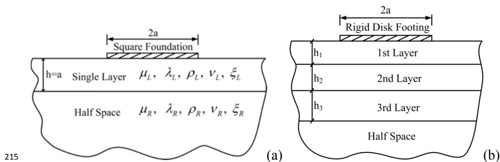
Fig. 4: Arbitrary-shaped foundation on multi-layered soil
