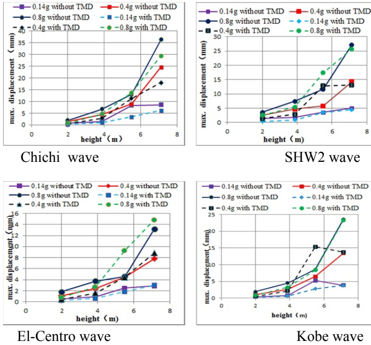
Figure 5: Comparison of max. displacement along the height of the model tower
