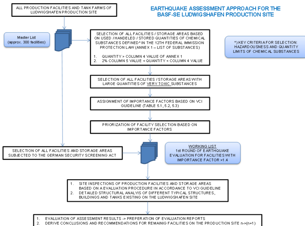
Figure 1: BASF earthquake assessment program
