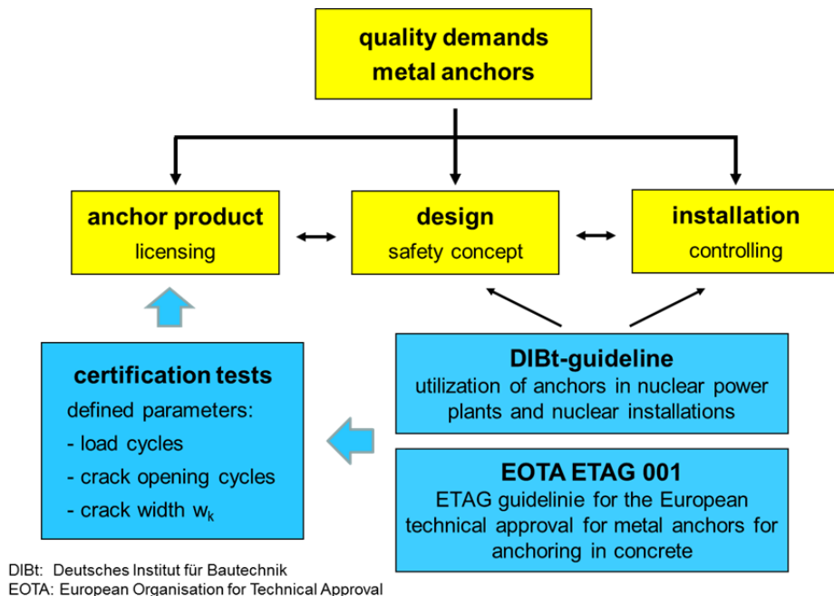
92 93 Figure 3: German licensing process for metal anchors
