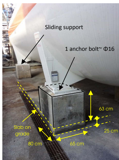
254 Figure 8: View and dimensions of column-shape leg-support of the reservoir
