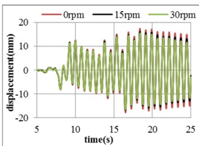
Wolong wave PGA=0.22g
