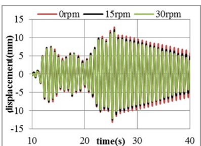
Chichi wave PGA=0.1g
