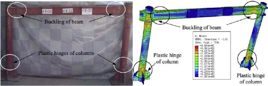
Figure 4: Failure modes of CFST frame (Adopted from Han et al. 2011[13])
