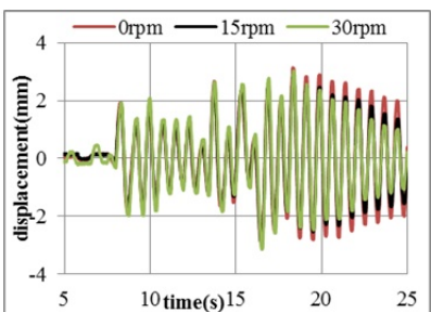
Wolong wave PGA=0.1g
