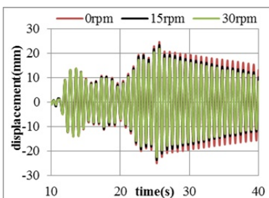
Chichi wave PGA=0.22g
