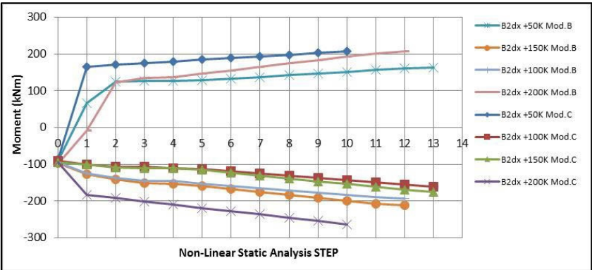
Figure 13: Moment-step diagram of the right end of beam n.2 for model B and C
