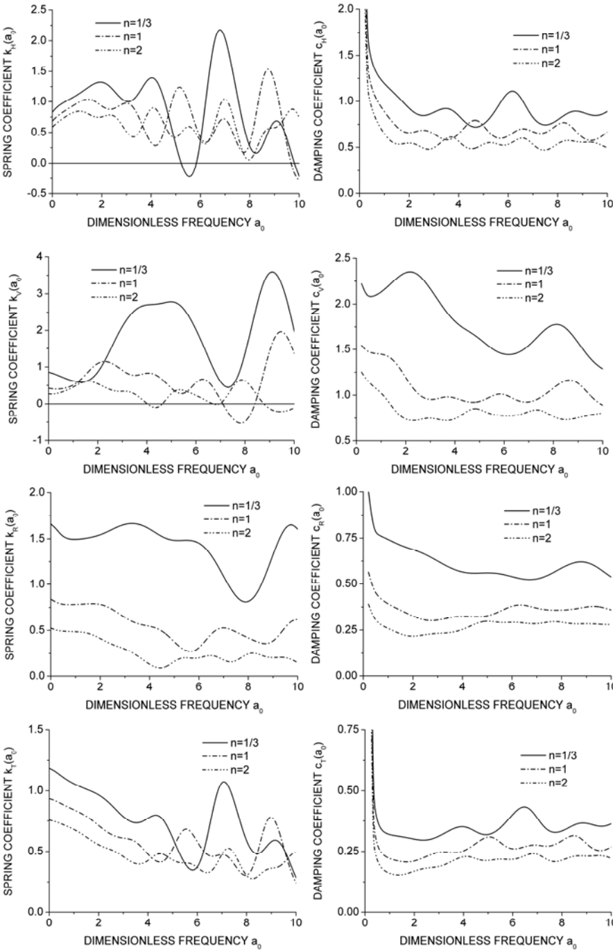
Figure 5: Dynamic impedance coefficients of circular foundation on layered half-space (anisotropic media)
