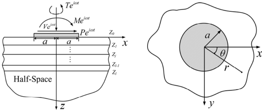
Figure 1: Description of the model
