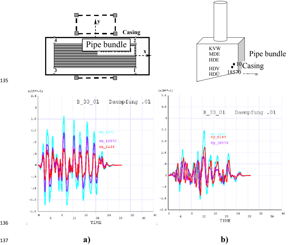
Figure 9: Seismic response of Model 3
