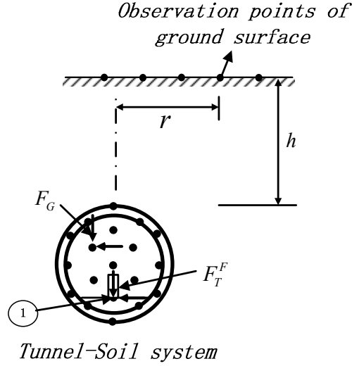
Figure 1: Analytical model
