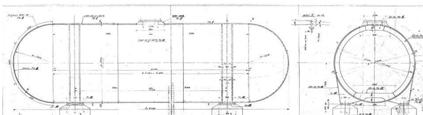
251 Figure 7: Construction drawing of a horizontal cylindrical reservoir including some 252 general dimensions
