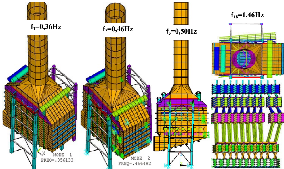
126 127 Figure 7: Eigenfrequencies and mode shapes of Model 3
