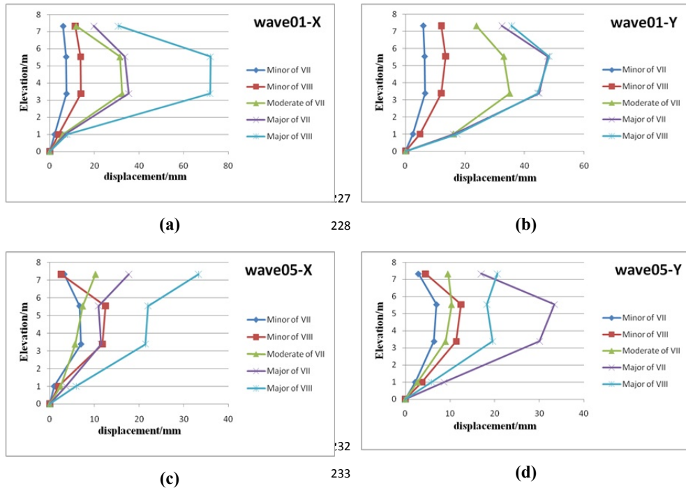
Fig. 7: Displacement
