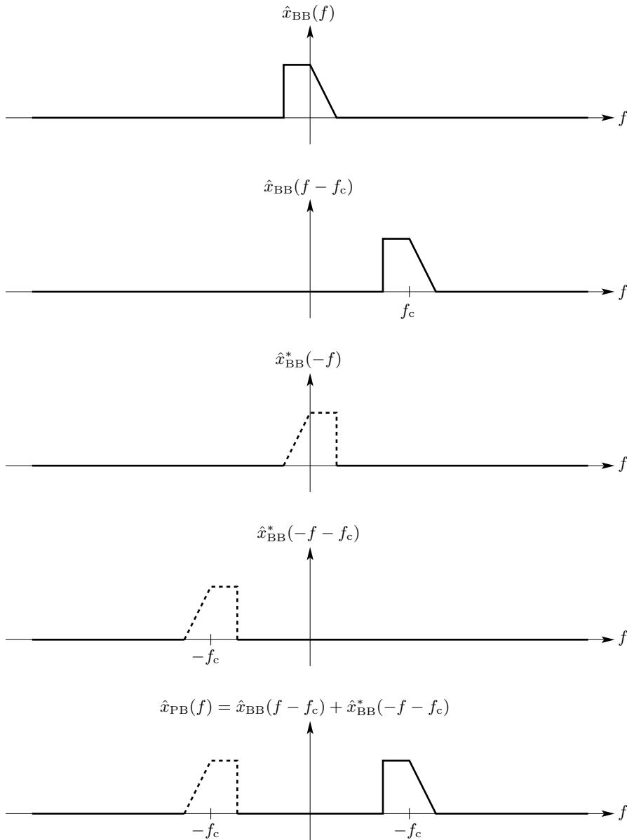
Figure 7.12: Recovering a passband signal from its baseband representation. Top plot of \hat{x}_{BB} is the transform of x_{BB} ; next is the transform of t \mapsto x_{BB}(t) e^{i2\pi f_c t} ; the transform of x_{BB}^*(t) ; the transform of t \mapsto x_{BB}^*(t) e^{-i2\pi f_c t} ; and finally the transform of t \mapsto x_{BB}(t) e^{i2\pi f_c t} + x_{BB}^*(t) e^{-i2\pi f_c t} = 2 \operatorname{Re}(x_{BB}(t) e^{i2\pi f_c t}) = x_{PB}(t) .
