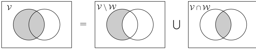
Figure 21.5: Diagram of two nondisjoint sets.
