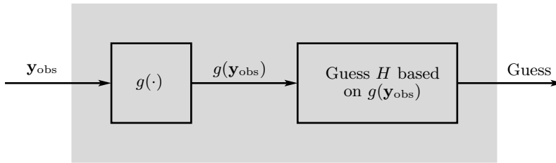
Figure 20.3: No decision rule based on g(\mathbf{y}_{\text{obs}}) can outperform an optimal decision rule based on \mathbf{y}_{\text{obs}} , because computing g(\mathbf{y}_{\text{obs}}) and then forming the decision based on the answer can be viewed as a special case of guessing based on \mathbf{y}_{\text{obs}} .
