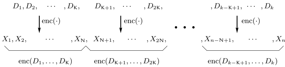
Figure 28.1: Block-mode encoding.
