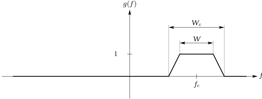
Figure 7.8: The function g of (7.16), which is used in the proof of Proposition 7.5.2.
