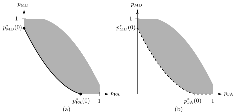
Figure 30.2: A generic achievable region. In (a) the solid line depicts the Pareto-optimal pairs. In (b) the dashed line is the graph of p_{\text{MD}}^*(\cdot) .
