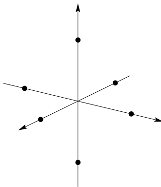
Figure 26.10: A bi-orthogonal constellation with six signals.
