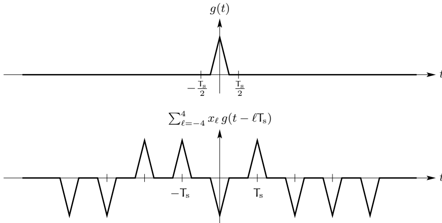
Figure 12.1: The pulse shape \mathbf{g}: t \mapsto (1 - 4|t|/T_s) \mathbf{I}\{|t| < T_s/4\} , and the sample function t \mapsto \sum_{\ell=-4}^4 x_\ell g(t - \ell T_s) when (x_{-4}, x_{-3}, x_{-2}, x_{-1}, x_0, x_1, x_2, x_3, x_4) = (-1, -1, +1, +1, -1, +1, -1, -1, -1) .
