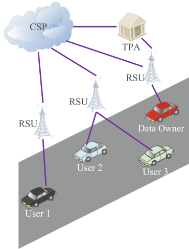
Fig. 2. The architecture of the proposed method for secure data sharing in VCC
