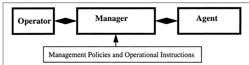
FIGURE 3.1.6 Real manager-agent model.
