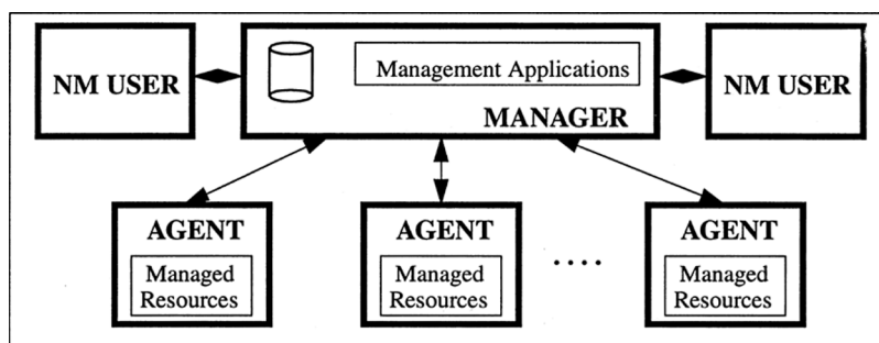
FIGURE 3.1.15 The “single manager” topological framework.
