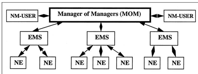
FIGURE 3.1.16 The “manager of managers” topological framework.
