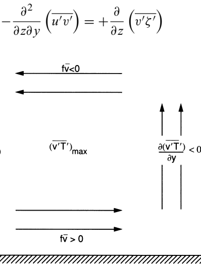
Fig. 10.4 Schematic Eulerian mean meridional circulation forced by poleward heat fluxes.
