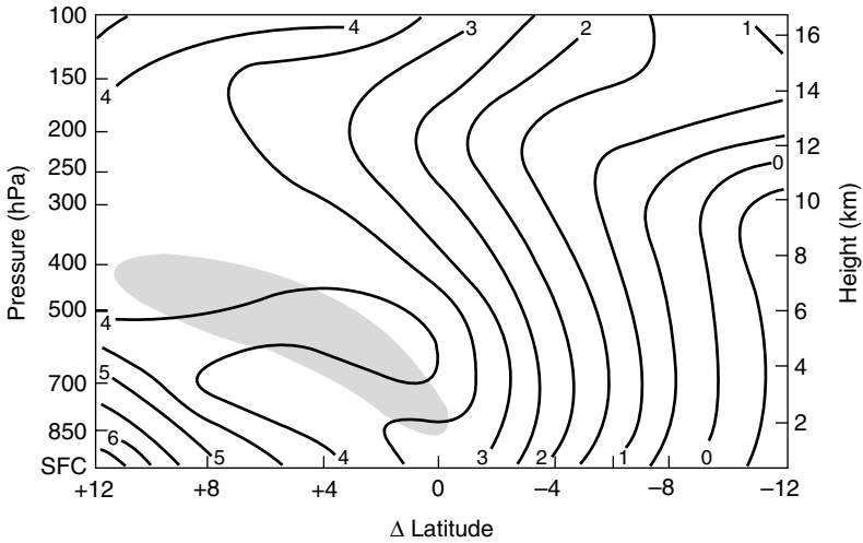
Fig. 11.8 Absolute vorticity (units 10^{-5}\text{s}^{-1} ) corresponding to the mean wind field of Fig. 11.6. Shading shows region where \beta - \partial^2 \bar{u} / \partial y^2 is negative. (After Reed et al., 1977. Reproduced with permission of the American Meteorological Society.)
