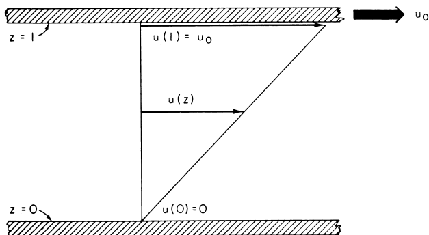
Fig. 1.3 One-dimensional steady-state viscous shear flow.
