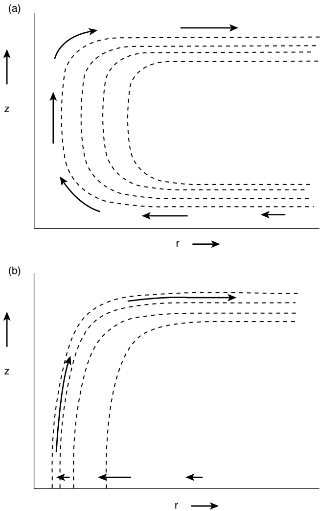
Fig. 9.15 Meridional cross sections showing the relationship between surfaces of constant saturation \theta_e (dashed contours; values decreasing as r increases) and meridional circulation (arrows) in CISK (a) and WISHE (b) theories for hurricane development. (a) Frictionally induced boundary layer convergence moistens the environment and destabilizes it through layer ascent. This enables small-scale plumes to reach their levels of free convection easily and to produce cumulonimbus clouds. Diabatic heating due to the resulting precipitation drives the large-scale circulation and thus maintains the large-scale convergence. (b) The saturation \theta_e is tied to the \theta_e of the boundary layer. The warm core occurs because enhanced surface fluxes of latent heat increase \theta_e there. (After Emanuel, 2000.)
