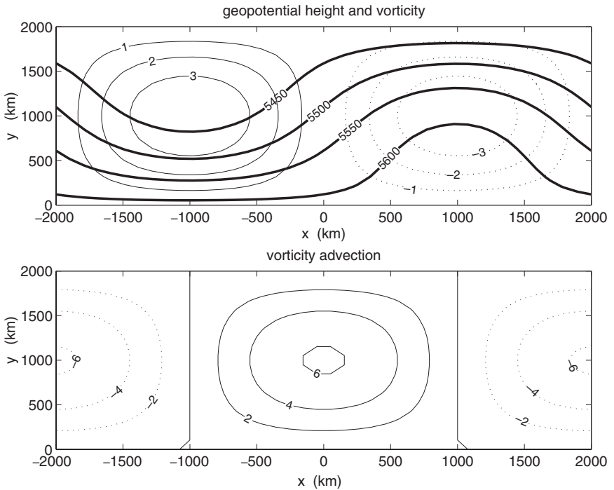
Fig. 6.8 (Top) Geopotential height in units of m, and relative vorticity in units of 10^{-5} \text{ s}^{-1} for the sinusoidal disturbance of equation (6.20). Here \Phi_0 = 5.5 \times 10^4 \text{ m}^2 \text{ s}^{-2} , f_0 = 10^{-4} \text{ s}^{-1} , f_0 A = 800 \text{ m}^2 \text{ s}^{-2} , U = 10 \text{ m s}^{-1} , and k = l = (\pi/2) \times 10^{-6} \text{ m}^{-1} . (Bottom) Advection of relative vorticity in units of 10^{-10} \text{ s}^{-2} for the disturbance shown above.
