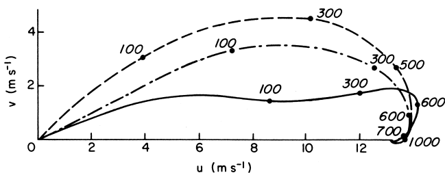
Fig. 5.5 Mean wind hodograph for Jacksonville, Florida ( \cong 30^\circ \text{ N} ), April 4, 1968 (solid line) compared with the Ekman spiral (dashed line) and the modified Ekman spiral (dash-dot line) computed with De \cong 1200 \text{ m} . Heights are shown in meters. (Adapted from Brown, 1970. Reproduced with permission of the American Meteorological Society.)
