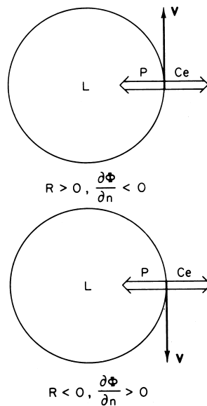
Fig. 3.4 Force balance in cyclostrophic flow: P designates the pressure gradient and Ce the centrifugal force.
