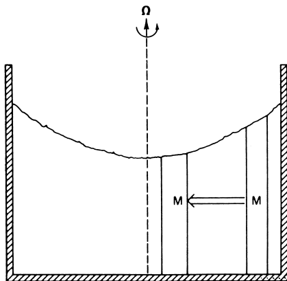
Fig. 4.11 Dependence of depth on radius in a rotating cylindrical vessel.
