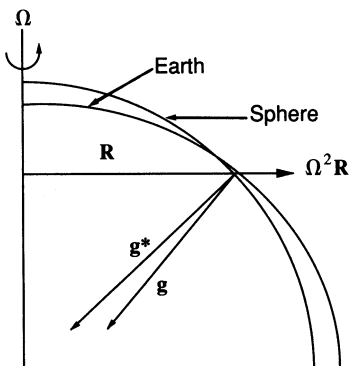
Fig. 1.6 Relationship between the true gravitation vector \mathbf{g}^* and gravity \mathbf{g} . For an idealized homogeneous spherical earth, \mathbf{g}^* would be directed toward the center of the earth. In reality, \mathbf{g}^* does not point exactly to the center except at the equator and the poles. Gravity, \mathbf{g} , is the vector sum of \mathbf{g}^* and the centrifugal force and is perpendicular to the level surface of the earth, which approximates an oblate spheroid.
