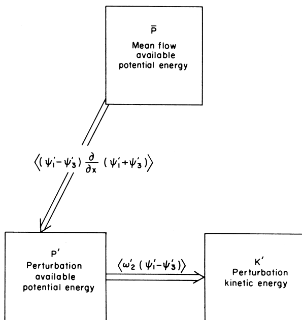
Fig. 8.9 Energy flow in an amplifying baroclinic wave.
