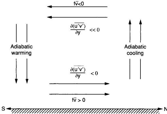
Fig. 10.5 Schematic Eulerian mean meridional circulation forced by a vertical gradient in eddy momentum flux convergence.
