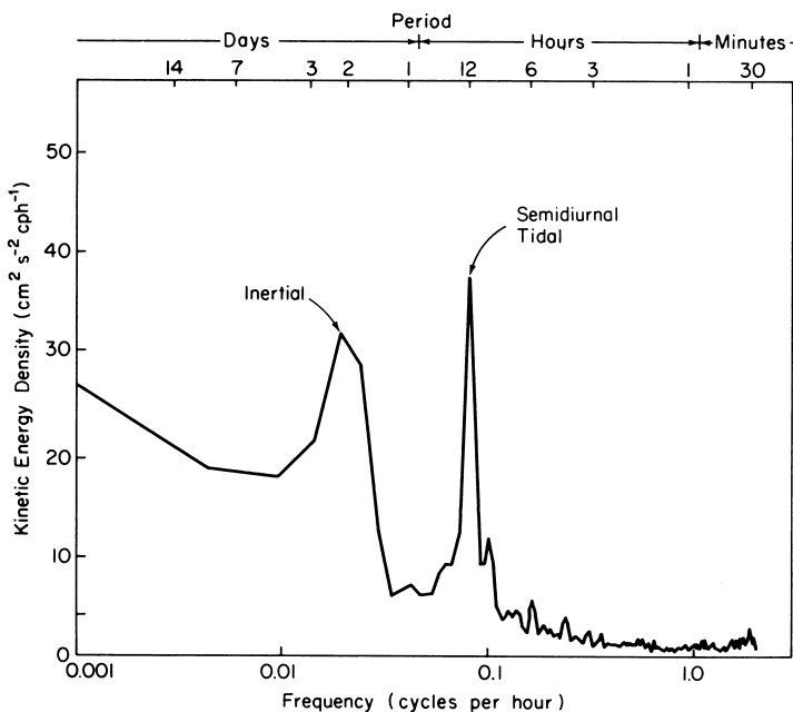
Fig. 3.3 Power spectrum of kinetic energy at 30-m depth in the ocean near Barbados ( 13^{\circ}\text{N} ). Ordinate shows kinetic energy density per unit frequency interval ( \text{cph}^{-1} designates cycles per hour). This type of plot indicates the manner in which the total kinetic energy is partitioned among oscillations of different periods. Note the strong peak at 53 h, which is the period of an inertial oscillation at 13^{\circ} latitude. [After Warsh et al., (1971.) Reproduced with permission of the American Meteorological Society.]
