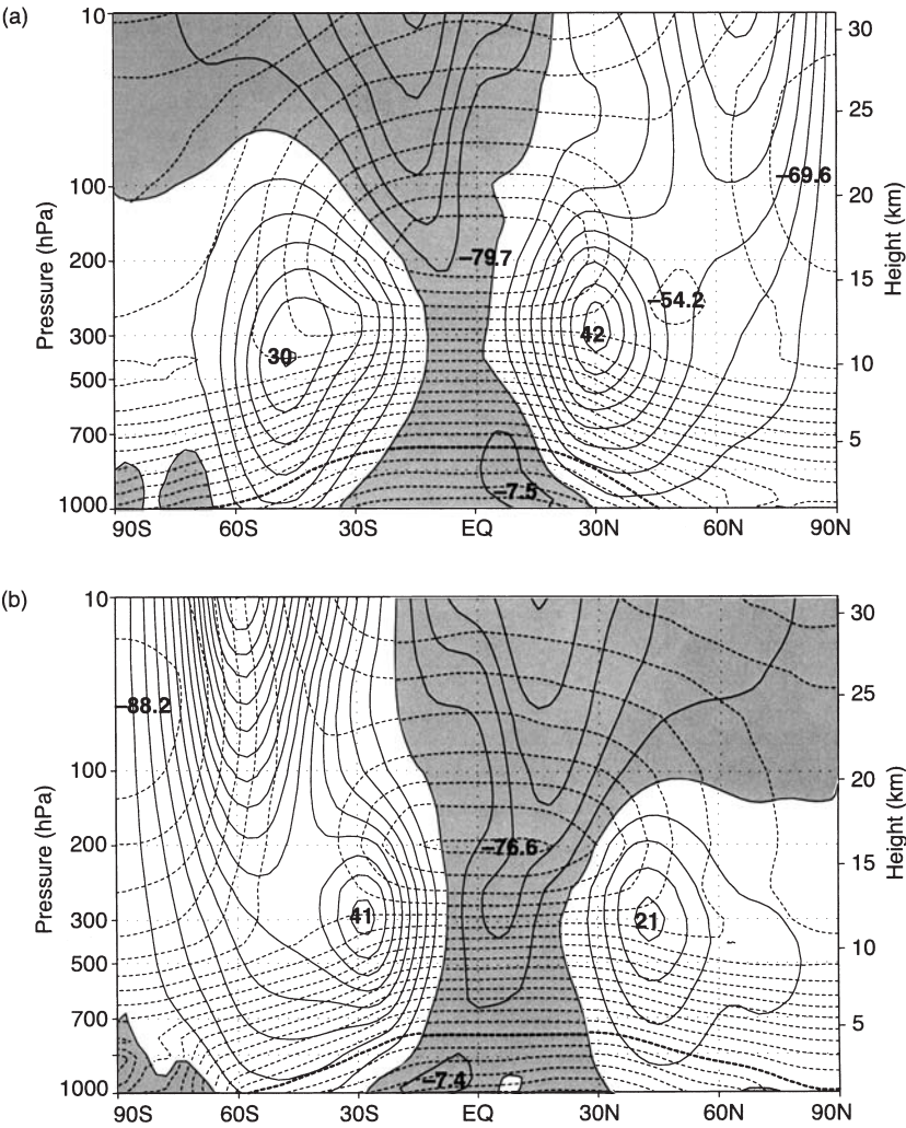
Fig. 6.1 Meridional cross sections of longitudinally and time-averaged zonal wind (solid contours, interval of \text{m s}^{-1} ) and temperature (dashed contours, interval of 5 \text{ K} ) for December–February (a) and June–August (b). Easterly winds are shaded and 0^{\circ}\text{C} isotherm is darkened. Wind maxima shown in \text{m s}^{-1} , temperature minima shown in ^{\circ}\text{C} . (Based on NCEP/NCAR reanalyses; after Wallace, 2003.)
