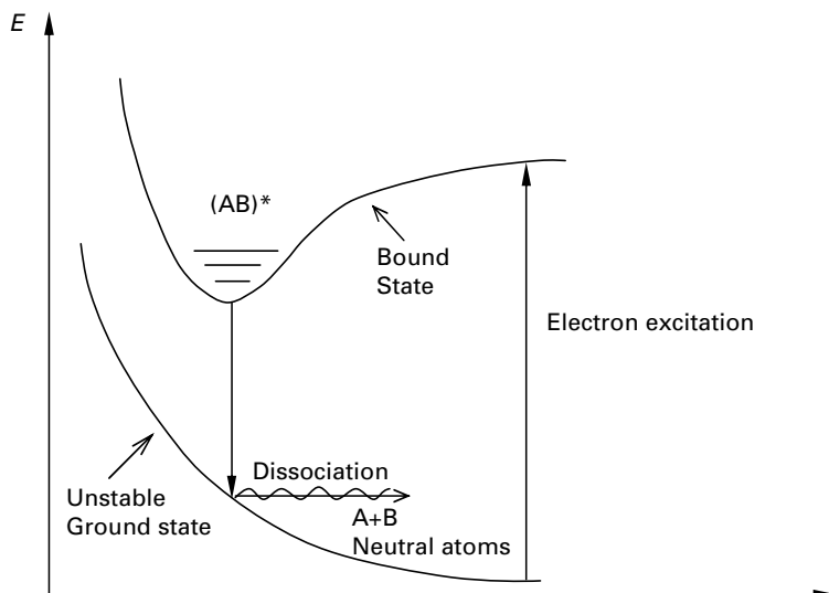
Figure 2.1. A schematic diagram of the transition process in an excimer laser.
