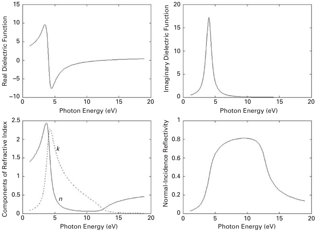
Figure 1.12. Lorentz-model predictions of the components of the complex dielectric function, the components of the complex refractive index, and the normal-incidence reflectance. A single resonance mode is assumed, with \hbar\omega_0 = 4 eV, \hbar\zeta = 1 eV, and oscillator number density N = 5 \times 10^{28} \text{ m}^{-3} .
