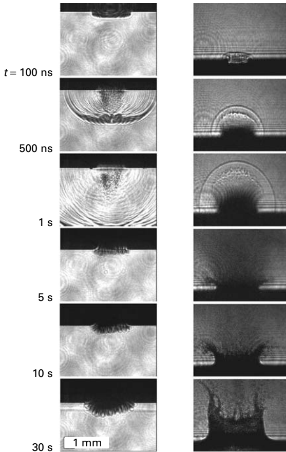
Figure 10.14. A sequence of images obtained by laser flash photography during ablation of K_2CO_4 solution by an excimer-laser pulse in the liquid (left column) and air (right column). The delay times t between the onset of laser irradiation and the image acquisition are marked in the figure. The excimer-laser fluence is F = 2.3 \text{ J/cm}^2 . From Kim et al. (1998), reproduced with permission from Springer-Verlag.
