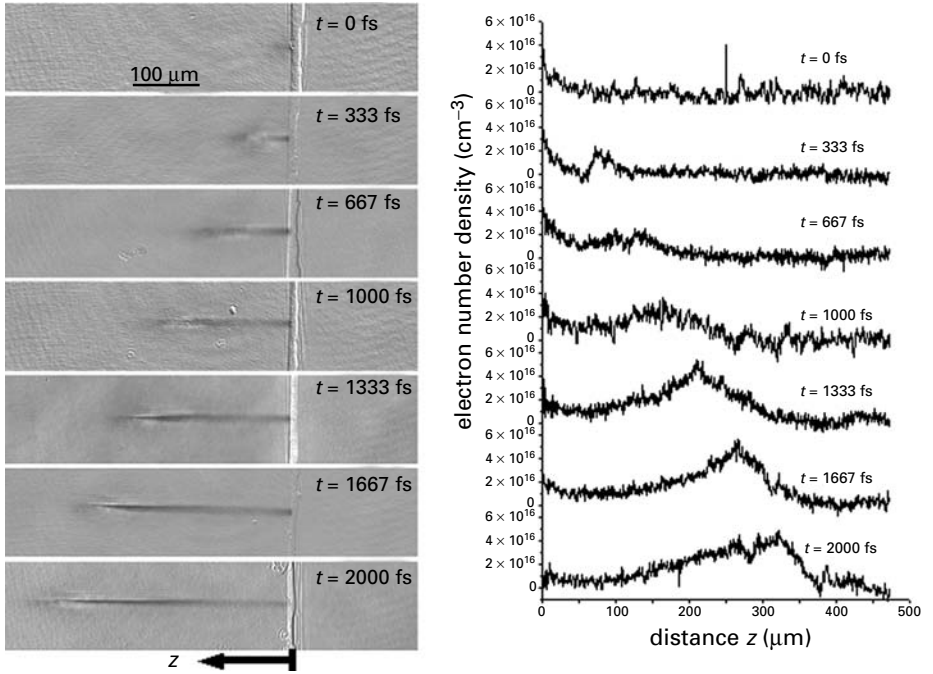
Figure 6.37. (a) Time-resolved images of femtosecond-laser-induced electronic excitation inside a silica glass; (b) evolution of the electron-number-density profile inside a femtosecond-laser-irradiated silica glass. From Mao et al. (2003), reproduced with permission by the American Institute of Physics.
