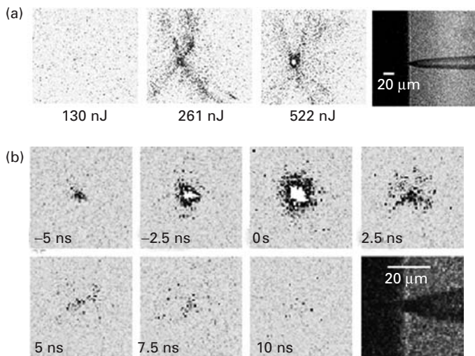
Figure 14.14. Side-view emission imaging of the optical-near-field-based ablation process.
