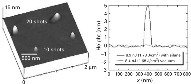
Figure 14.11. Nanodeposition of Si dots from silane using single nanosecond-laser shots at \lambda = 532 \text{ nm} through the apertured NSOM tip. The base diameter of the nanodeposit is \sim 100 \text{ nm} .
