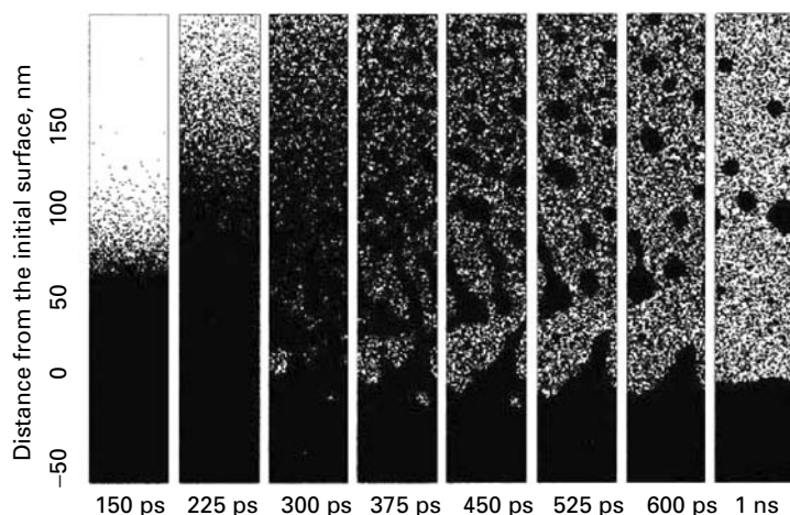
Figure 9.4. Snapshots from the molecular-dynamics simulation of laser irradiation of a molecular solid with pulse duration of 150 ps and fluence of 61 \text{ J/m}^2 , adapted from Zhigilei and Garrison (2000) with permission from the Institute of Applied Physics.
