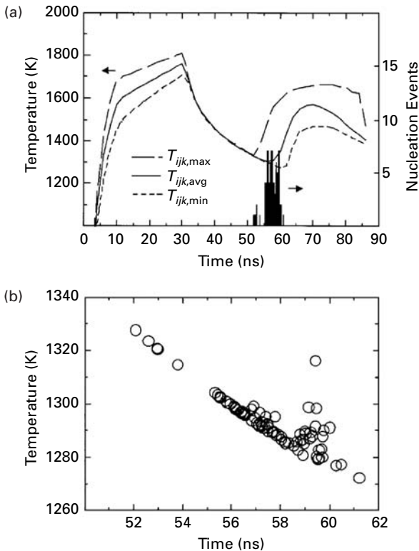
Figure 7.14. Node-temperature evolution in a single simulation showing maximum, minimum, and average temperatures in the film. The histogram corresponds to nucleation events that occurred during the transformation. (b) Some nucleation events, plotted as individual points at the time and temperature of occurrence. From Leonard and Im (2001), reproduced with permission from the American Institute of Physics.
