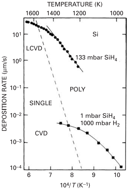
Figure 13.5. An Arrhenius plot for the growth of Si from \text{SiH}_4 by LCVD and standard CVD. Regions of single-crystalline and polycrystalline growth are shown (separated by a dashed line); the intersection points of the LCVD and CVD curves are at 1555 and 1262 K, respectively. From Bäuerle (2000), reproduced with permission from Springer-Verlag.
