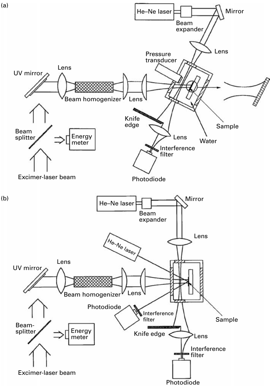
Figure 10.4. Schematic diagrams of the experimental setup with (a) the piezoelectric transducer and the photoacoustic-deflection probe, and (b) the optical-reflection probe and the photoacoustic-deflection probe. The diameter of the deflection probe beam is exaggerated. From Park et al. (1996c), reproduced with permission from the American Institute of Physics.
