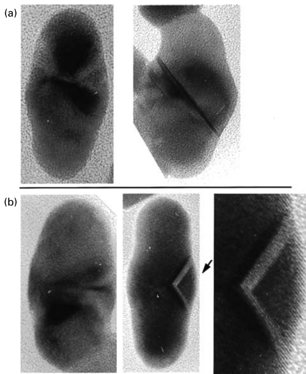
Figure 12.4. A high-resolution TEM image of gold nanorods after exposure to nanosecond-laser pulses with a fluence of 250 \text{ mJ/cm}^2 ( 20 \text{ } \mu\text{J} per pulse): (a) nanorods with stacking faults and (b) twinned particles. Similar defect structures are found in spherical gold nanoparticles after complete shape transformation from nanorods, whereas the as-prepared nanorods are found to be defect-free. From Link et al. (2000), reproduced with permission from the American Chemical Society.
