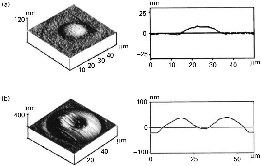
Figure 8.15. Atomic-force-microscopy images and cross sections for soda-lime glass:
