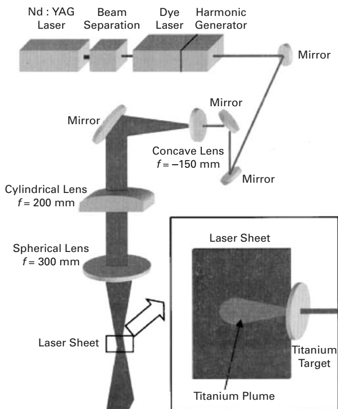
Figure 5.9. A schematic diagram of the excitation-laser setup. The output from the Nd : YAG laser contains both the fundamental (1064 nm) and the doubled harmonic (532 nm). The fundamental portion is disposed of in the beam-separation package, and the remainder, the second harmonic, is used to pump the dye laser. The vacuum chamber in which the titanium sample resides is omitted from this diagram.
