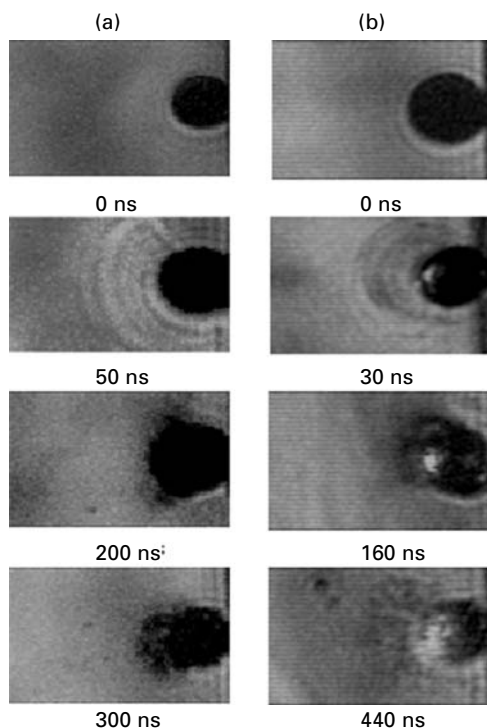
Figure 12.10. Time-resolved shadowgraph images displaying ablation of a Cu microparticle (diameter 48 \mu\text{m} ) during the synthesis of CuO nanoparticles; (a) wavelength 355 nm, fluence 1 \text{J}/\text{cm}^2 ; and (b) wavelength 532 nm, fluence 1.8 \text{J}/\text{cm}^2 . Courtesy of Dongsik Kim of POSTECH University, Korea.
