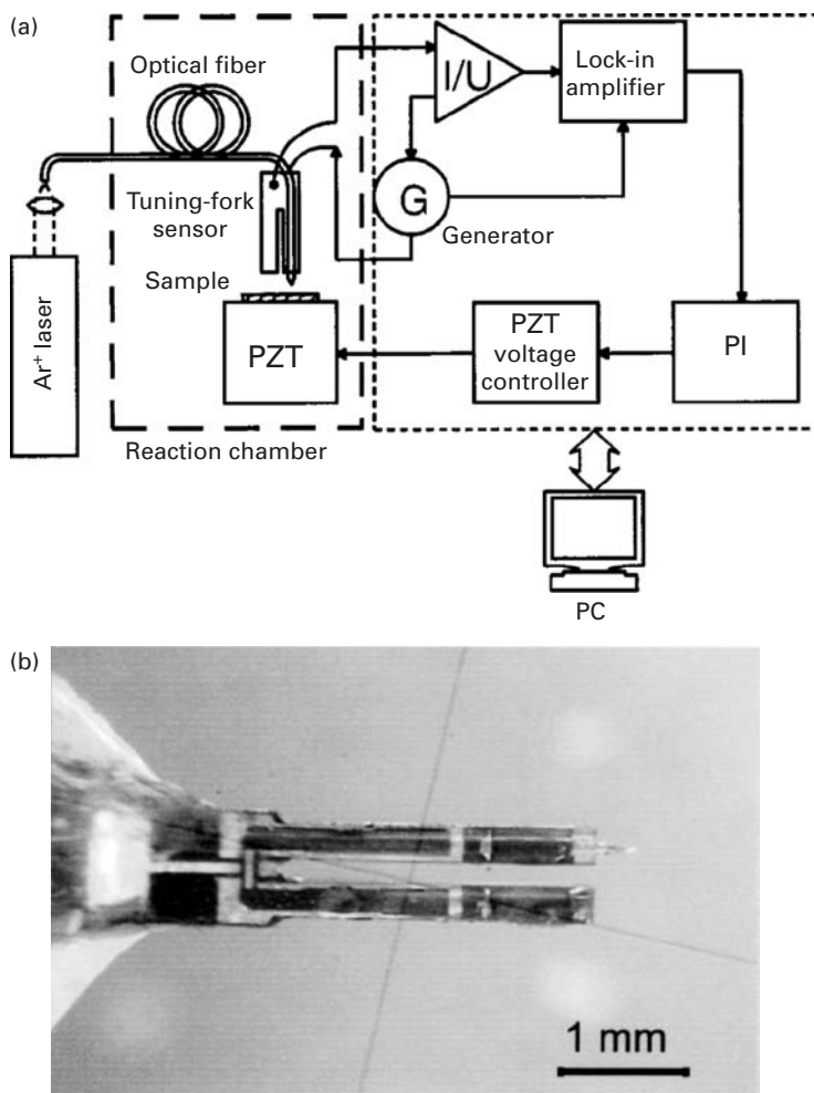
Figure 14.9. A schematic picture of the experimental setup used for laser-induced chemical etching of Si in Cl 2 atmosphere (Wysocki et al. , 2004). Courtesy of Professor Dieter Bäuerle. Reproduced with permission by the American Institute of Physics.
