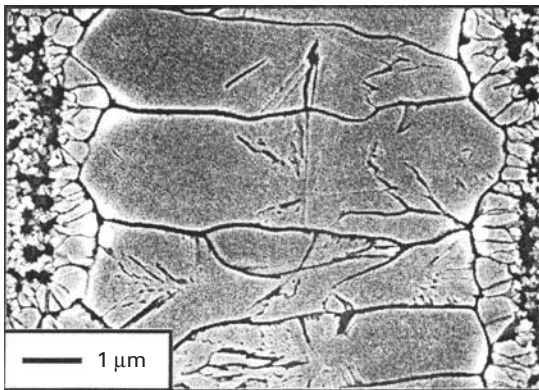
Figure 7.16. The top view of the crystallized Si film for the case of a mask-sample separation of 0.4 mm, \theta = 53^\circ , and I_{\text{pk}} = 900 \text{ mJ/cm}^2 . From Oh et al. (1998), reproduced with permission from the Institute of Pure and Applied Physics.
