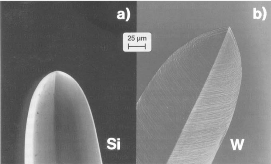
Figure 13.4. Scanning-electron-microscopy pictures of the tips of laser-grown single-crystalline fibers: (a) Si grown from \text{SiH}_4 and (b) W grown from \text{WF}_6 plus \text{H}_2 . From Bäuerle et al. (1983), reproduced with permission from Springer-Verlag.
