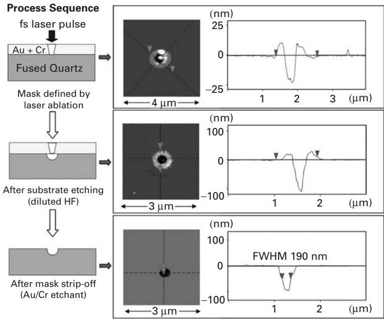
Figure 14.12. The process sequence for NSOM-based nanomachining of thin metal films and subsequent feature transfer onto a transparent quartz substrate. Also shown in the figure are the AFM scans corresponding to each of the steps in the process sequence, for a single case of an input laser fluence of 3.2 \text{ J/cm}^2 . From Chimmalgi et al. (2007), reproduced with permission by the Institute of Physics.
