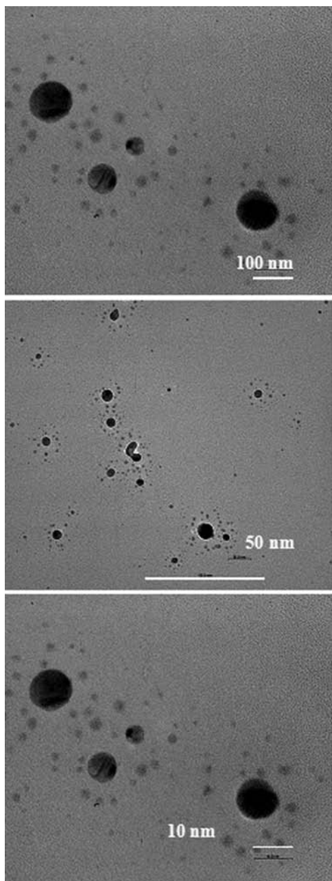
Figure 12.9. Transmission-electron-microscopy images of silver nanoparticles generated from 8- \mu\text{m} -sized microparticles (laser fluence 2 J/cm 2 , laser wavelength 355 nm, consolidation pressure 40 MPa; the ambient gas is air). Courtesy of Dongsik Kim of POSTECH University, Korea.
