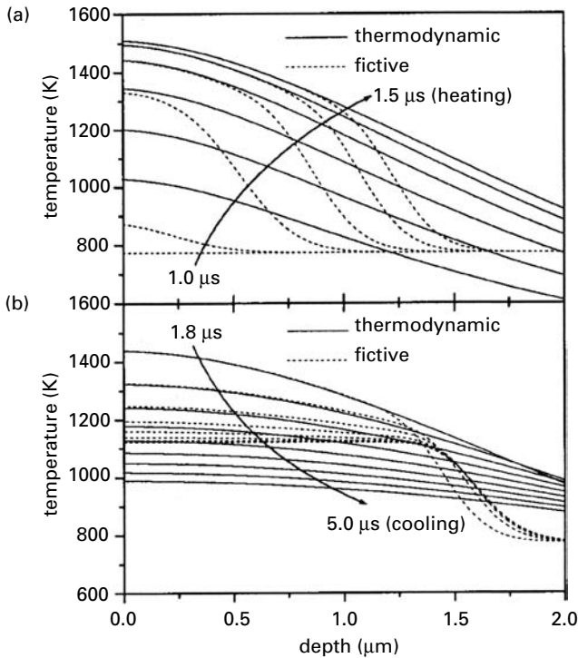
Figure 8.17. The relationship between thermodynamic temperature (solid lines) and fictive temperature (dashed lines) along the centerline of the laser-heated zone in an aluminosilicate glass. A CO 2 laser pulse of wavelength \lambda = 10.6 \mu\text{m} , 1/e^2 radius 13.5 \mu\text{m} , and pulse energy 3.0 \mu\text{J} , with a Gaussian temporal profile with FWHM pulse width t_{\text{pulse}} = 0.7 \mu\text{s} and peak intensity at t_{\text{max}} = 1 \mu\text{s} is utilized. (a) For heating, depth profiles are given at 100-ns intervals between 1.0 and 1.5 \mu\text{s} . (b) For cooling, depth profiles are given at 400-ns intervals between 1.8 and 5.0 \mu\text{s} . From Bennett and Li (2001), reproduced with permission from the American Institute of Physics.
