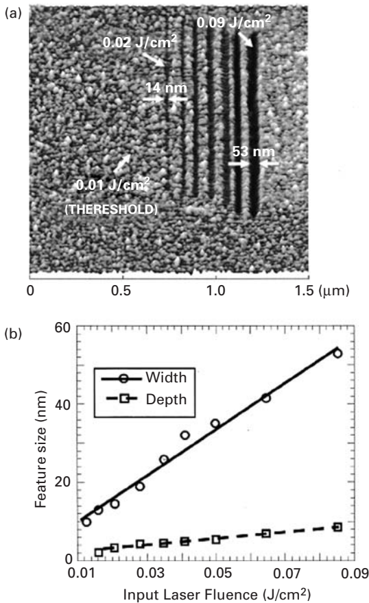
Figure 14.3. (a) Surface nanostructuring of 25-nm-thick Au film for laser fluence between 0.012 and 0.086 J/cm 2 . (b) The dependence of lateral feature size on laser fluence. From Chimmalgi et al. (2005a), reproduced with permission from the American Institute of Physics.
