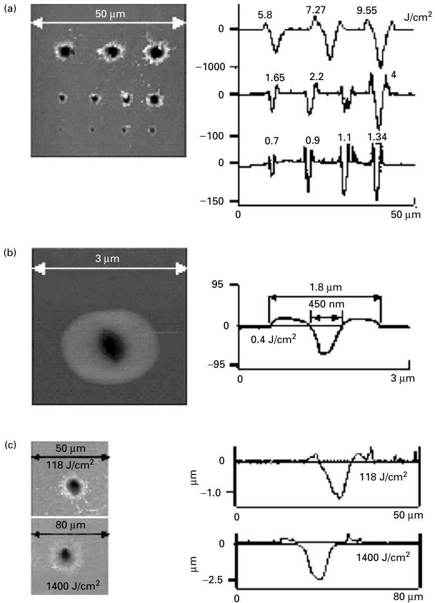
Figure 6.21. An AFM image and cross-sectional profile of a sub-micrometer hole being made to open in a c-Si wafer by single femtosecond laser pulses of \lambda = 800\ \text{nm} at medium energy densities (a), at near-threshold energy density (b), and at high energy densities (c); and the ablation efficiency as a function of the energy density (d). From Hwang et al. (2006), reproduced with permission by the American Institute of Physics.
