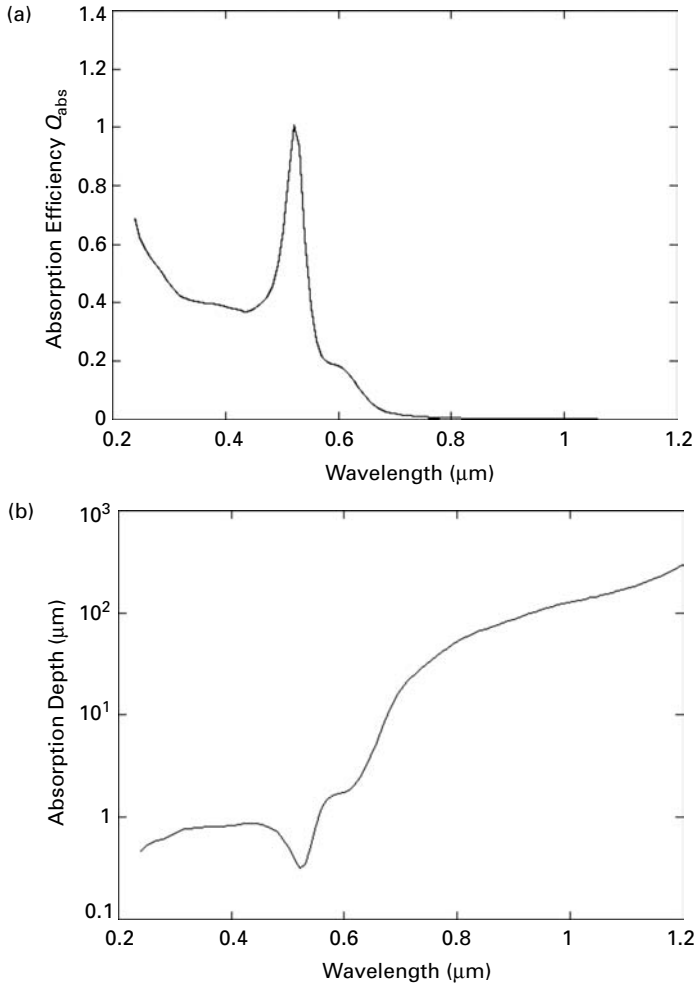
Figure 12.1. (a) The wavelength dependence of the absorption efficiency for a single gold particle of radius R_{\text{pa}} = 5 nm. (b) The dependence of the optical penetration depth in a toluene ( n = 1.5 ) suspension of 5-nm gold particles.
