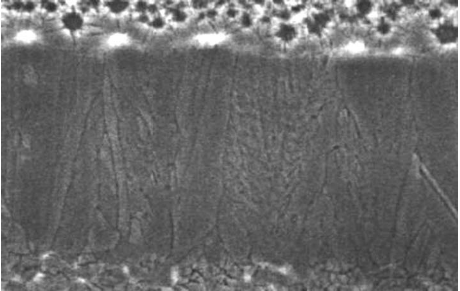
Figure 7.21. A lateral growth length of about 1.5 μm is obtained under a high fluence gradient. From Lee et al. (2000), reproduced with permission from the American Institute of Physics.
