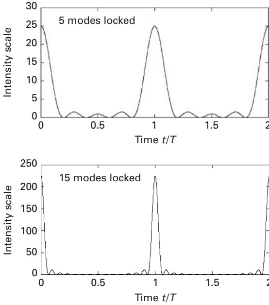
Figure 2.5. Plots of optical field amplitude resulting from phase locking of 5 and 15 laser modes.
