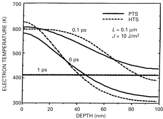
Figure 6.3. Predicted electron-temperature profiles from two-step models during a 100-fs laser pulse heating. The film thickness is 0.1 \mu\text{m} and the fluence is F = 10 \text{ J/m}^2 . From Qiu and Tien (1993), reproduced with permission by the American Society of Mechanical Engineers.
