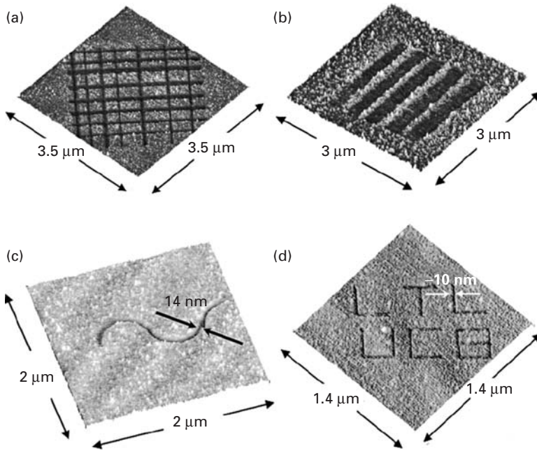
Figure 14.4. Surface nanostructuring of \sim 25 -nm-thick Au film, (a), (c), and (d), and 15-nm-thick Au film, (b), for laser fluence 0.069 \text{ J/cm}^2 . From Chimmalgi et al. (2005a), reproduced with permission from the American Institute of Physics.
