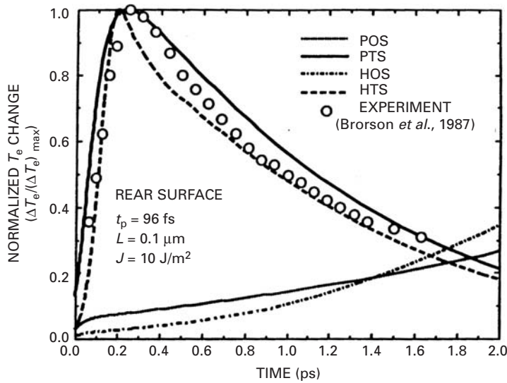
Figure 6.2. Comparison of predicted electron-temperature changes with experimental data at the rear surface. The pulse duration is 96 fs, the film thickness is 0.1 \mu\text{m} , and the fluence is F = 10 \text{ J/m}^2 . From Qiu and Tien (1993), reproduced with permission by the American Society of Mechanical Engineers.
