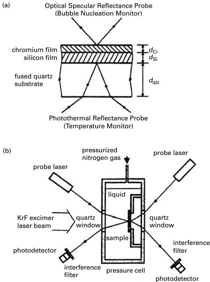
Figure 10.1. A schematic diagram of the experimental setup: (a) the optical detection scheme and (b) an overall view. The sample is composed of a 0.15- \mu\text{m} -thick Cr film and 0.35- \mu\text{m} -thick p-Si to maximize the optical response due to interference. From Park et al. (1996a), reproduced with permission from the American Institute of Physics.
