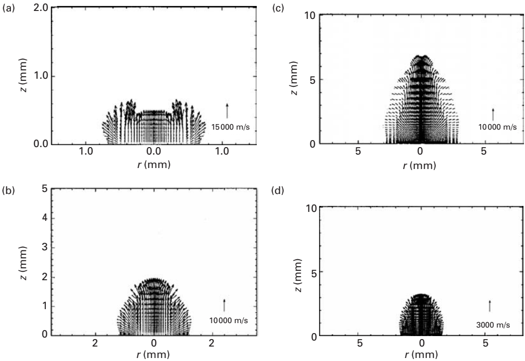
Figure 5.2. Velocity vectors for the conditions of Figure 5.1. From Ho et al. (1996), reproduced with permission by the American Institute of Physics.
