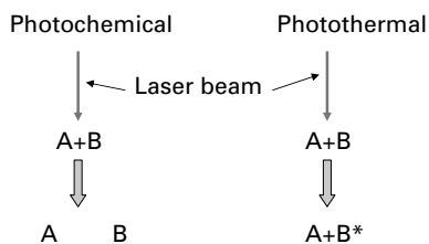
Figure 9.2. Main differences between photochemical and photothermal effects.
