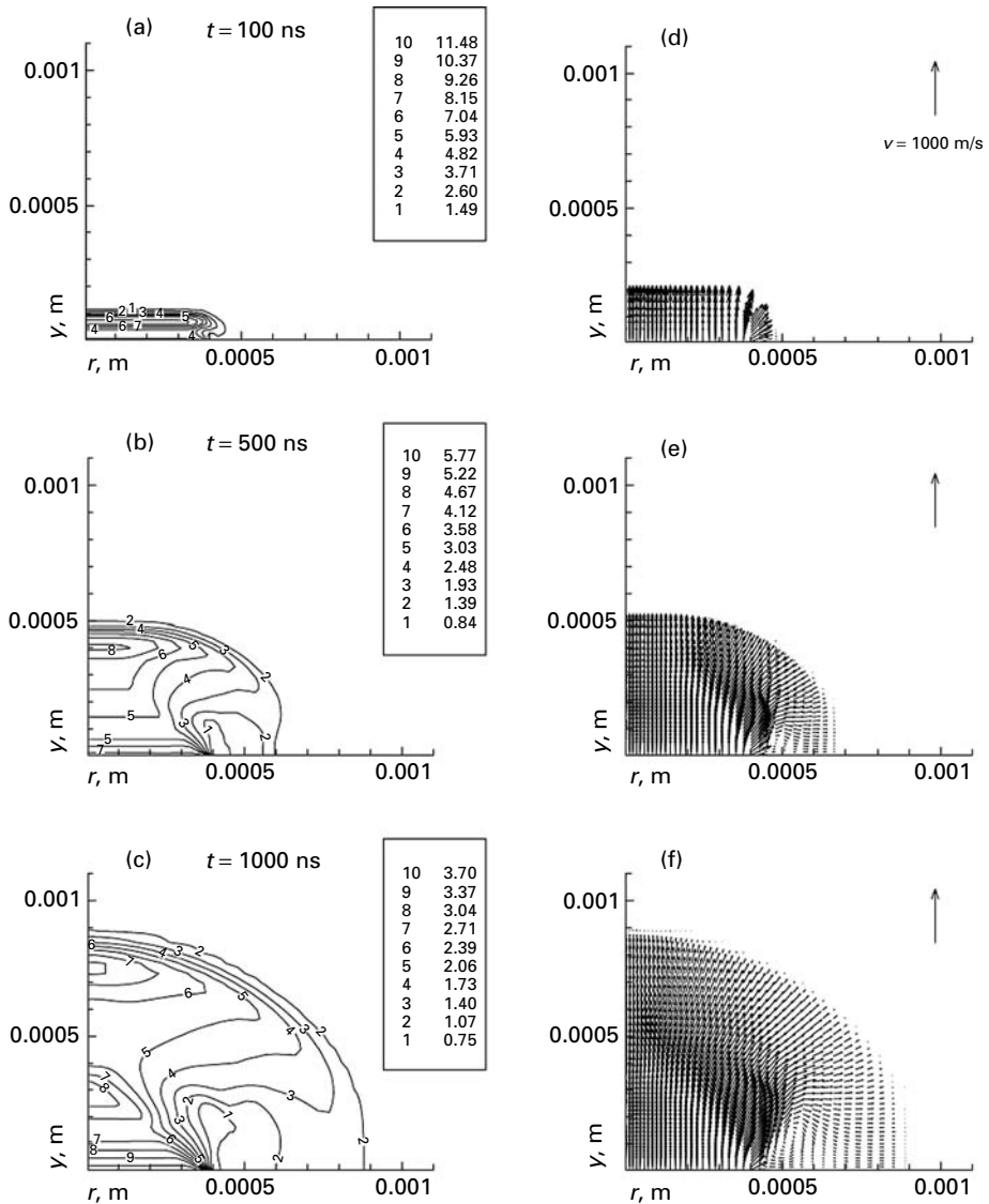
Figure 10.12. Normalized pressure contours (a)–(c) and velocity vectors (d)–(f) in the air for K_2CrO_4 concentration m = 0.03 and excimer-laser fluence F = 2.3 \text{ J/cm}^2 at t = 0.1 \mu\text{s} for (a) and (d); t = 0.5 \mu\text{s} for (b) and (e); and t = 1.0 \mu\text{s} for (c) and (f). The ambient pressure is 1 atm and the laser-spot diameter is 0.8 mm. From Kim et al. (1998), reproduced with permission from Springer-Verlag.
