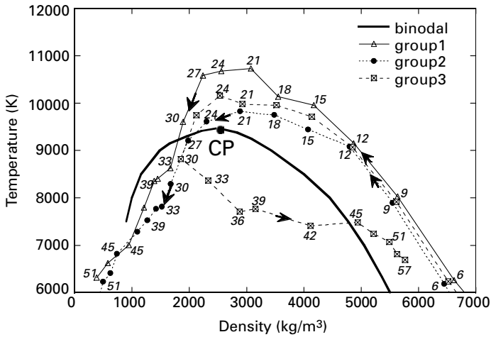
Figure 6.28. Thermodynamic trajectories of groups of atoms. The fluence is 0.65 \text{ J/cm}^2 . From Cheng and Xu (2005), reproduced with permission by the American Physical Society.
