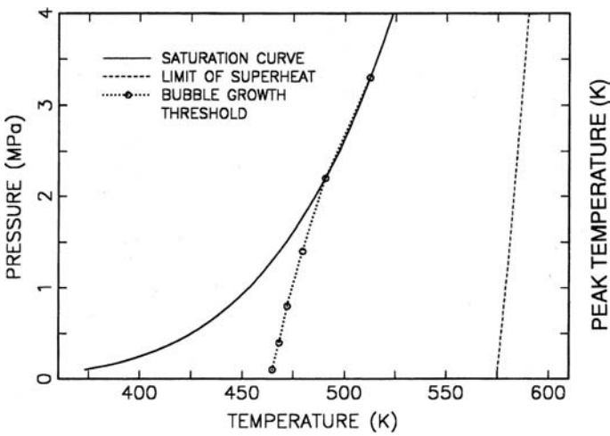
Figure 10.3. The bubble-growth-threshold temperatures and liquid pressures are identified as symbols o and connecting dotted lines in the P - T diagram. From Park et al. (1996b), reproduced with permission from the American Society of Mechanical Engineers.
