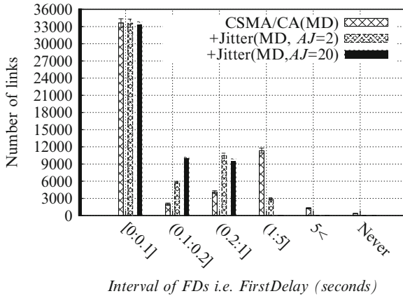
Fig. 16 The jitter scheme improves the FD significantly, when VD is approximately 50. In case of AJ = 2 , the number of cases for “5<” and “Never” are 31 \pm 6 and 29 \pm 9 , respectively. In case of AJ = 20 , the number of cases for “5<” and “Never” are both 0. It shows that the jitter scheme performs better than the elastic scheme. In case of AJ = 20 , the number of the links in an interval of (0.2:1] is much lower. The result shown is an average of ten simulations with a confidence interval of 99 %
