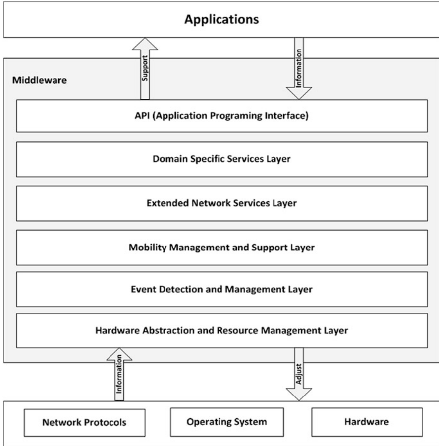
Fig. 1 General WSN middleware architecture
