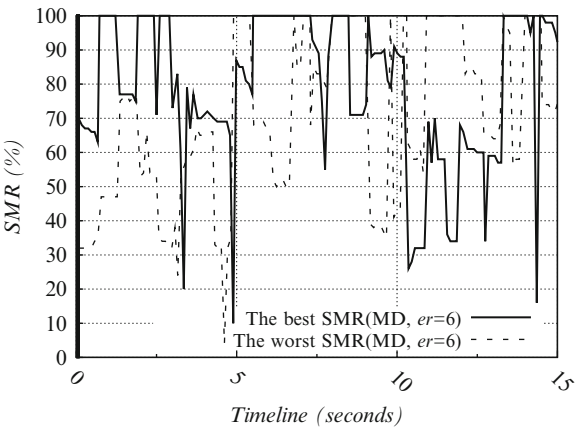
Fig. 10 SMR fluctuations over time of two individual vehicles that experience the best and the worst SMR , respectively, when VD is approximately 50. Compared to the pure CSMA/CA case, it is now hard to see any difference between the best and the worst cases. The graph shows the results of an arbitrary simulation
