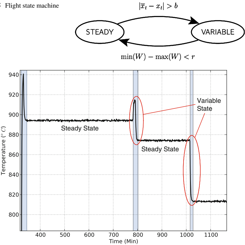
Fig. 6 System states within the flight profile
