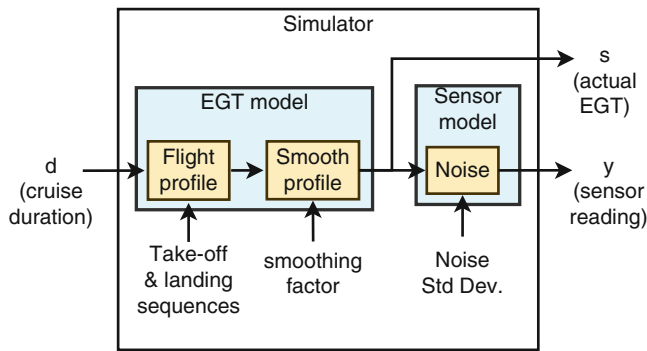
Fig. 3 Simulator architecture
