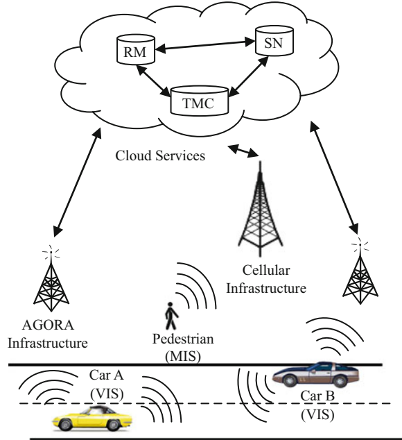
Fig. 1 AGORA framework for ITS with cloud services
