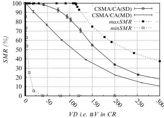
Fig. 3 Successful Message Ratio ( SMR ) of the entire network with respect to the vehicle density ( VD ) shows the communication reliability. maxSMR is the maximum possible SMR calculated analytically. minSMR is the minimum possible SMR obtained by means of simulations in which all vehicles have approximately the same phases for broadcasting. SD (Single Domain) case shows SMR degradation only due to the contention problem, where all the vehicles are deployed at fixed locations within a single CR, therefore, there are no HNs. MD (Multi-Domain) shows SMR degradation due to both the contention and HN problems, where all vehicles are deployed on a 3 km long highway with three lanes per direction. Both cases show average values of ten simulations with a 99 % confidence interval
