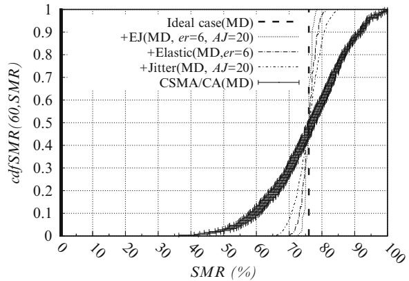
Fig. 17 The EJ scheme outperforms the jitter scheme and it is slightly better than the elastic scheme for improving the fairness. The result shown is an average of ten simulations with a confidence interval of 99 %. For the elastic scheme, the confidence interval is \pm 0.3
