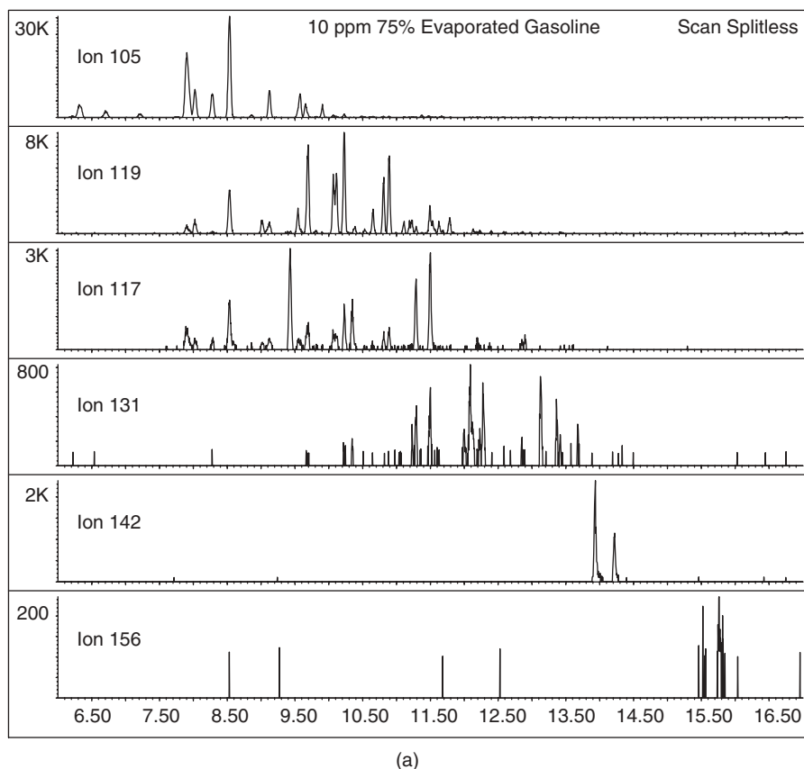
Figure 3.34 Six ion chromatograms produced by a 10-ppm solution of 75% evaporated gasoline run in the full-scan mode, with splitless injection; (b) run in the SIM mode, with a 20:1 split ratio..
