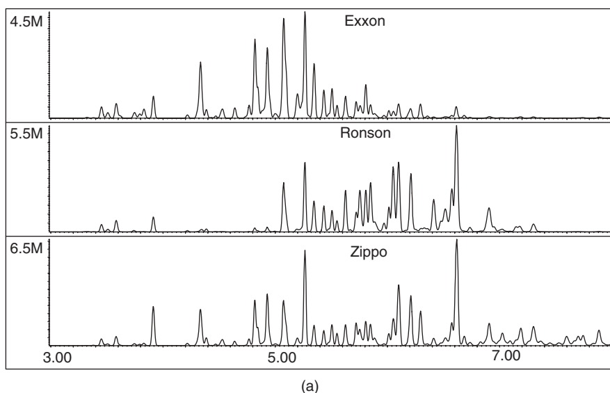
Figure 3.17 (a) Total ion chromatograms of three different brands of cigarette lighter fluid. (b) Ion chromatograms of ions 57, 55, 83, and 91 from a standard of Ronson lighter fluid.
