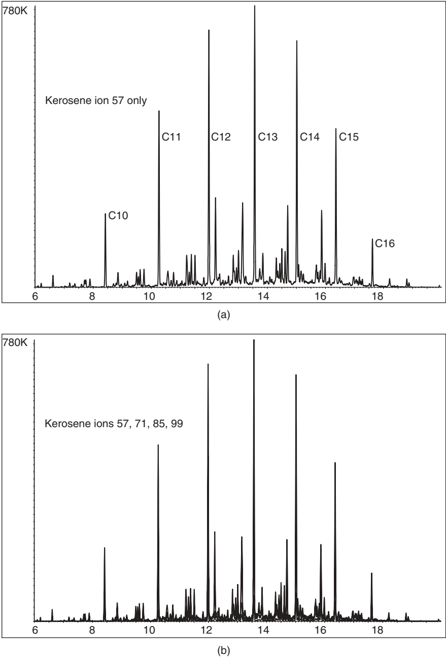
Figure 3.7 Ion profiling versus ion chromatography. Comparison of (a) the ion 57 chromatogram with (b) the ion profile combining ions 57, 71, 85, and 99 from a kerosene standard. The four ions in the profile are plotted in the merged format. Plotted individually, they are all very similar, with ion 57 presenting the tallest peaks.
