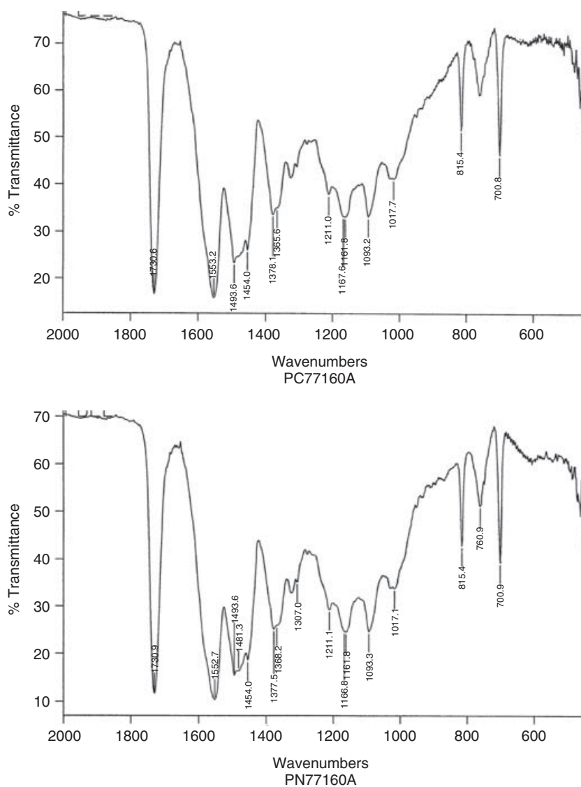
Figure 5.25 Transmission infrared spectra of two different acrylic-melamine enamel automotive finishes having the same color. Both were manufactured by PPG for use on the same year vehicle line; however, one is a low-solvent-emission formulation while the other is not.
