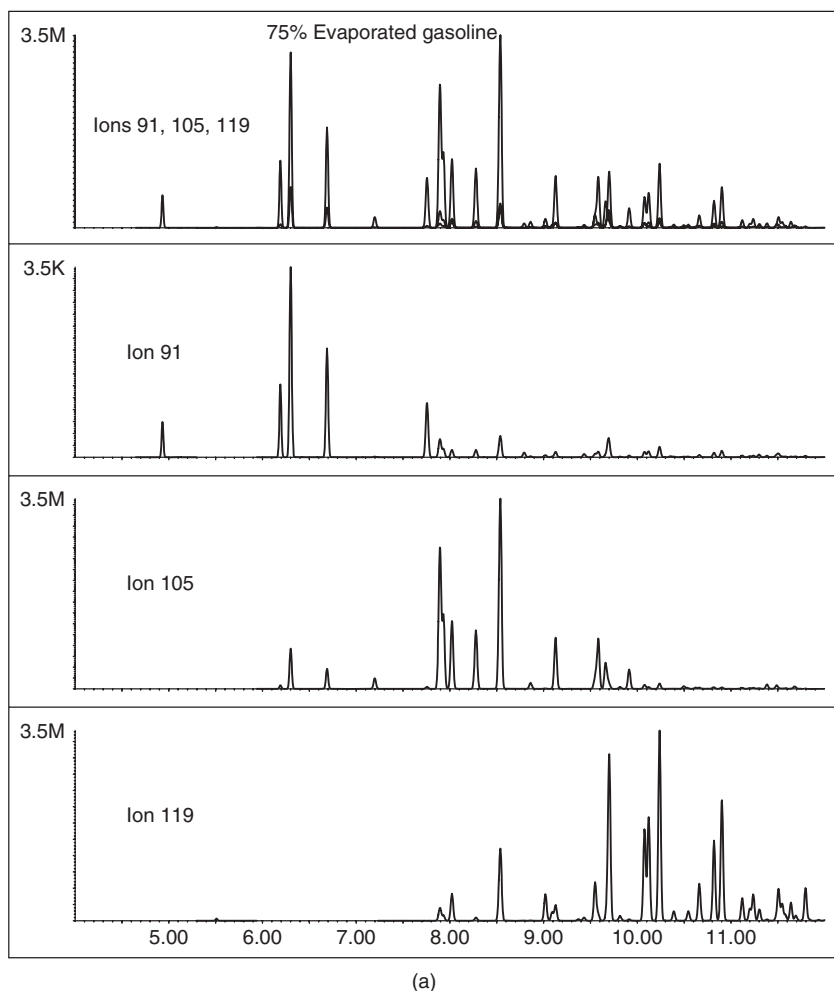
Figure 3.9 Ion profiling versus ion chromatography. (a) Comparison of ion profiles from 75%-evaporated gasoline. The top chart shows a combination of ions 91, 105, and 119. The next three charts show those ion chromatograms plotted independently. (b) Comparison of ion profiles from 90%-evaporated gasoline. The top chart shows a combination of ions 91, 105, and 119. The next three charts show those ion chromatograms plotted independently. Note the improvement in the level of detail presented for the xylenes.
