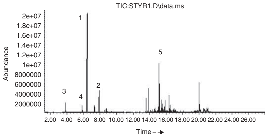
Figure 5.28 Pyrogram of pure polystyrene pyrolyzed at 750°C in an inductively heated pyrolysis probe and chromatographed on a PyGC–MS system using a 30-m narrow-bore 5% phenyl methyl siloxane fused-silica capillary column. The pyrogram consists of many other pyrolyzates in addition to the styrene peak (1), including methyl styrene (2), toluene (3) and ethyl benzene (4). Some of the longer retention time pyrolyzates are dimmers and trimers of these pyrolyzates (5).
