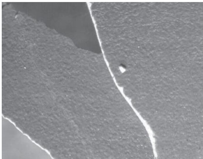
Figure 5.4 Stereomicroscopic view of the underside of the original base primer from an automotive application revealing the characteristic “orange peel” appearance. Magnification of 20 \times . ( See insert for color representation. )
