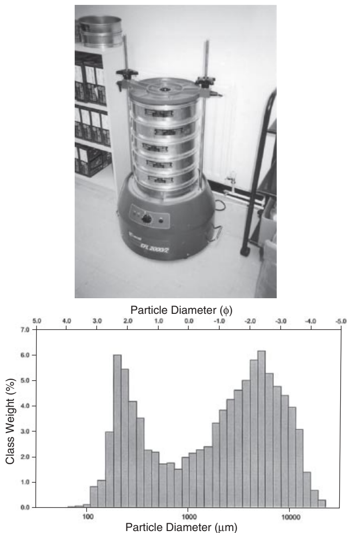
Figure 4.3 Nest of sieves used to separate particles into different size grades and a diagram showing the size distribution of particles. (See insert for color representation.)
