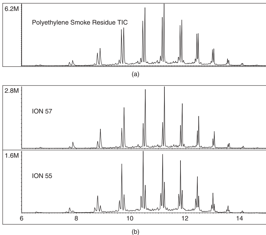
Figure 3.23 Total ion chromatogram of (a) polyethylene smoke condensate. The first peak in each doublet is the alkene; the second is the alkane. Pristane, phytane cycloalkanes, and aromatics are all absent. (b) Ion 57 EIC, and (c) ion 55 EIC. In the ion 55 chromatogram, a third peak, representing the n , (n - 1) -diene, appears.
