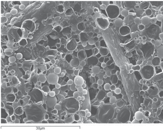
Figure 3.25 Scanning electron micrograph of the underside of a carbonless form. The microspheres range in size from 2 to 20 \mu\text{m} and are filled with normal alkanes.
