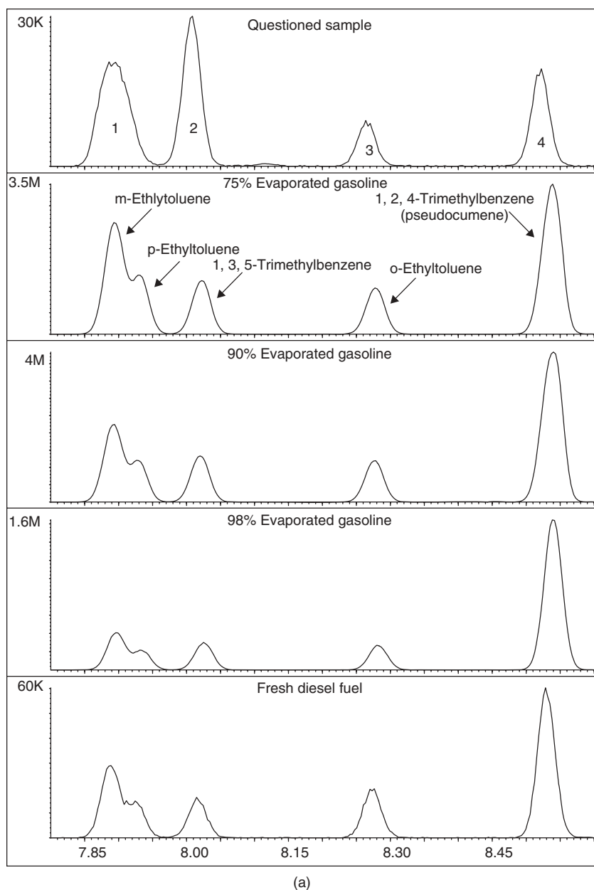
Figure 3.14 Study of the C_3 alkylbenzene group. (a) The top chromatogram shows an unknown sample. This is followed by gasoline in three stages of evaporation, and fresh diesel fuel. The TIC of the unknown did not look like gasoline, but based on this EIP and a few other ion chromatography comparisons, an analyst called the sample positive for gasoline.
