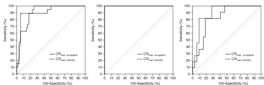
Figure 2. Receiving operator characteristic (ROC) curves used to compare predictive accuracy between CR_{\max} occupation and CR_{\max} intensity for the development of MES during exposure of the carotid arteries ( left , for all patients; middle , for patients with identification of the image with the POR_{\max} occupation and that with the maximum plaque intensity; right , for patients without this identification). In the middle panel, each area under the ROC curve for CR_{\max} occupation or CR_{\max} intensity (each CR_{\max} occupation is identical to CR_{\max} intensity, respectively) is 1.000.
