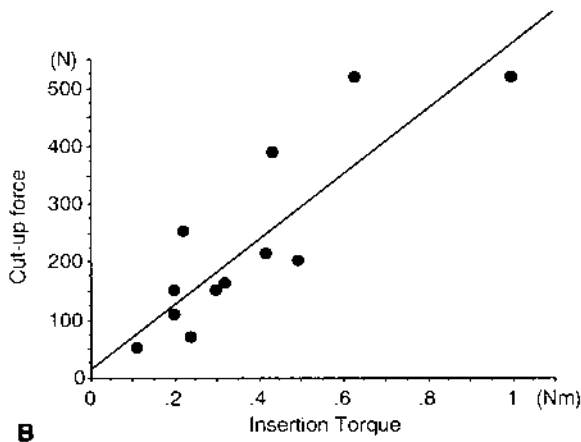
Figure 7 (a) The correlation between the cut-up force and BMD ( y = 2.44x - 97.61 ; r = 0.76 ; n = 12 , p < 0.01 ). (b) The correlation between cut-up force and insertion torque ( y = 558.80x + 24.08 ; r = 0.857 ; n = 12 ; p < 0.01 ). Mean \pm SD. (From Ref. 48. Published, with permission, from Okuyama K, et al. Stability of transpedicle screwing for the osteoporotic spine. An in vitro study of the mechanical stability. Spine 1993; 18: 2240–2245.)
