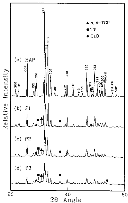
Figure 2 x-ray diffraction pattern (Cu K \alpha ) for (a) HAP, (b) P1-HAC, (c) P2-HAC, and (d) P3-HAC. It was revealed that the HAP has a well-crystallized single phase of \text{Ca}_{10}(\text{PO}_4)_6(\text{OH})_2 . P3-HAC contained the highest amount of CaO phase and the lowest crystallinity. (From Ref. 24.)
