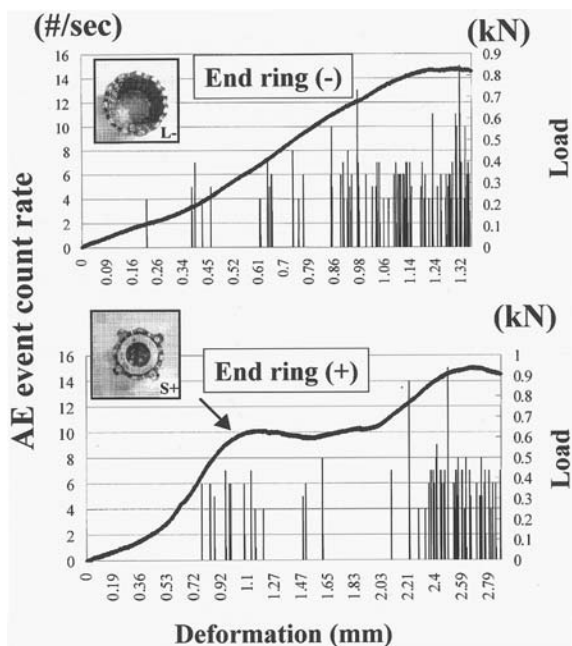
Figure 9 Load-deformation curve with an AE event count rate.
