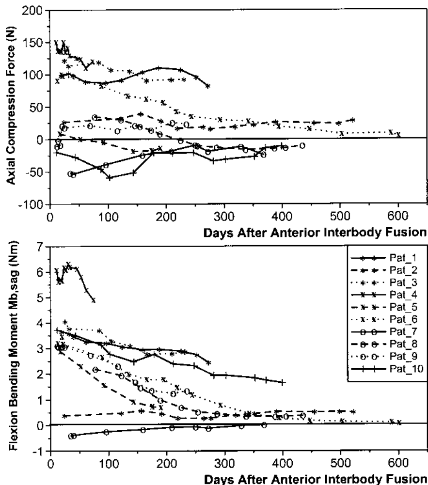
Figure 4 Load differences between a standing and lying position as a function of time after the anterior procedure. The figure shows average differences in load on the left and right fixators measured in the implants of the 10 patients. The curves were slightly smoothed. (From Ref. 13.)
