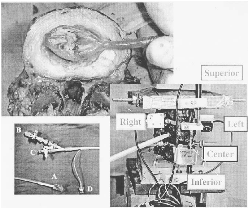
Figure 2 In situ curable prosthetic intervertebral nucleus (PIN) being developed by Disc Dynamics, Inc., Minnetonka, MN. (From Ref. 13.)
