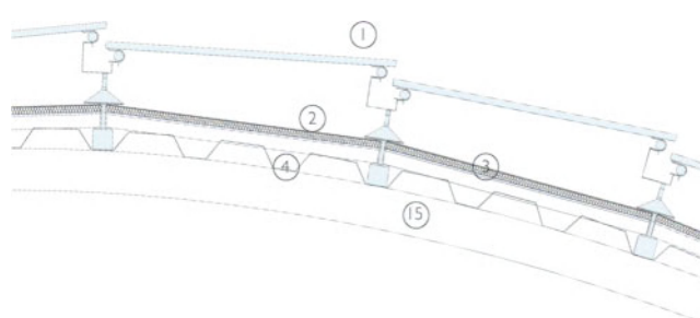
Section 1:25 typical section with rainscreen panels draining from panel to panel
