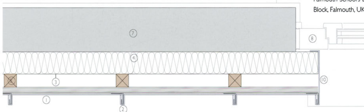
Plan 1:10. Profiled metal sheet fixed to concrete backing wall
