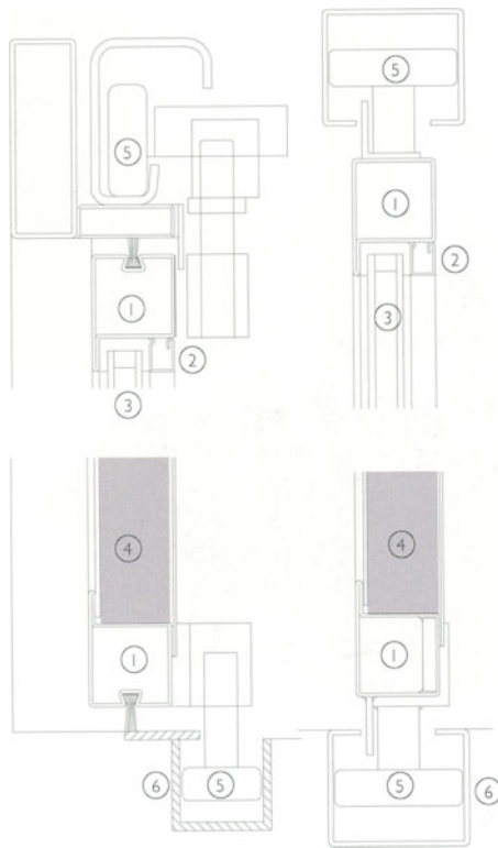
Vertical sections 1:5. Sliding/folding door with rubber seals
