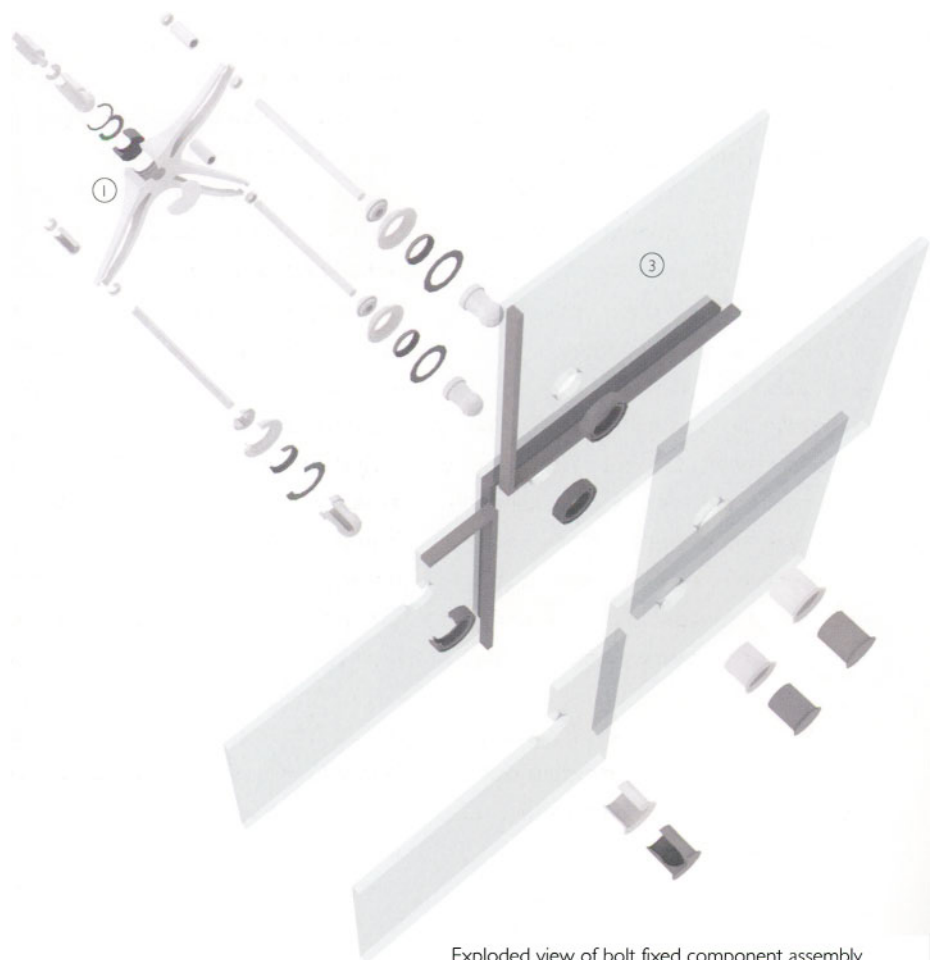
Exploded view of bolt fixed component assembly
