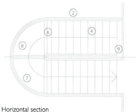
Horizontal section
