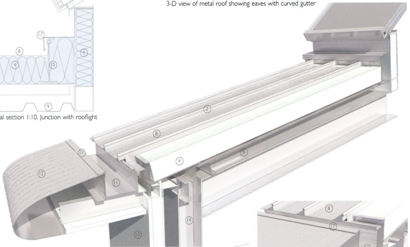
3-D view of metal roof showing eaves with curved gutter
