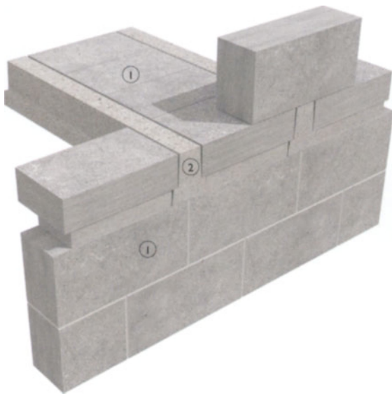
3-D detail of traditional beam and block floor system
