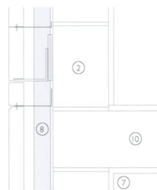
Section 1:10. Stone supported on individual fixings
