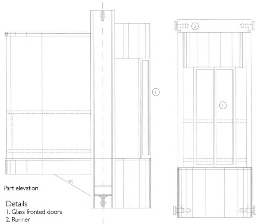
Part elevation
