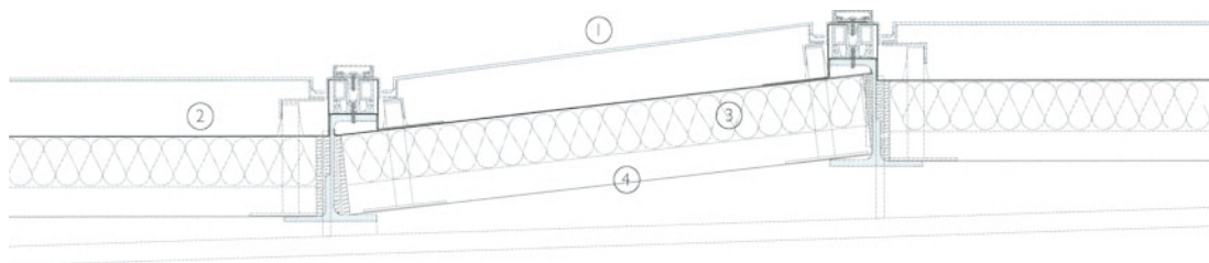
Vertical section 1:25. Typical long section through metal rainscreen roof
