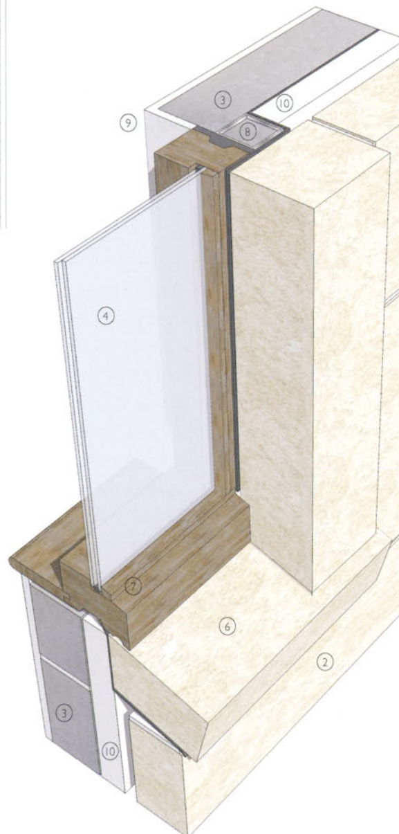
3-D view of timber window frame in stone cavity wall
