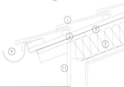
Section I:20. Eaves detail for profiled tile
