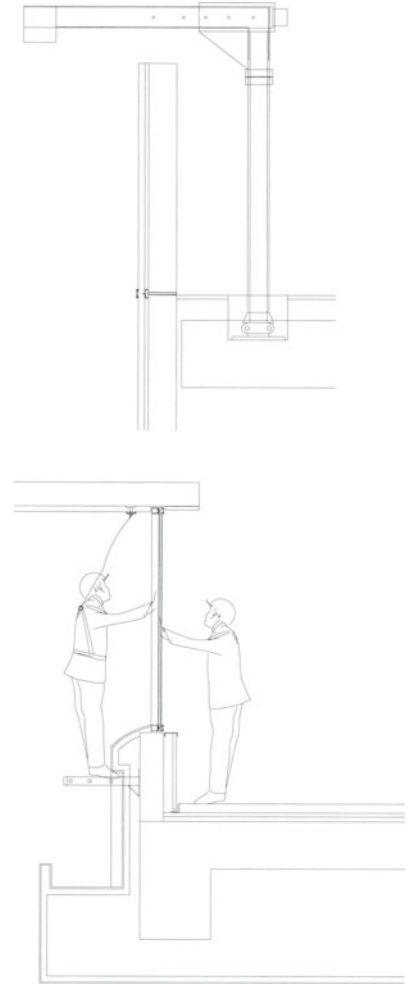
Section NTS cleaning with harness on a platform
