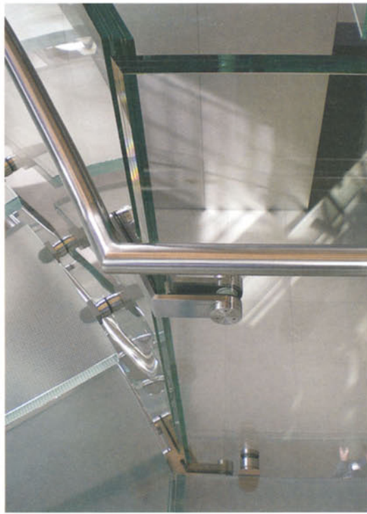
Glass stair in Apple store , Regents Street, London, UK. Architect: Bohlin Cywinski Jackson
