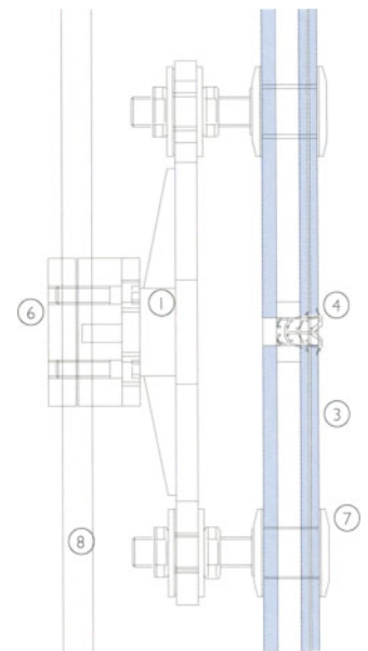
Vertical section 1:10, bolt fixed glazing detail
