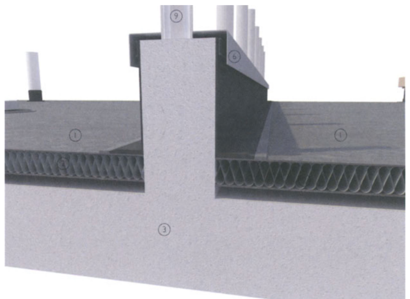
3-D detail of upstand
