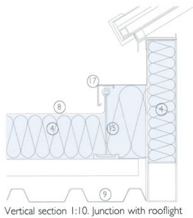
Vertical section 1:10. Junction with rooflight
