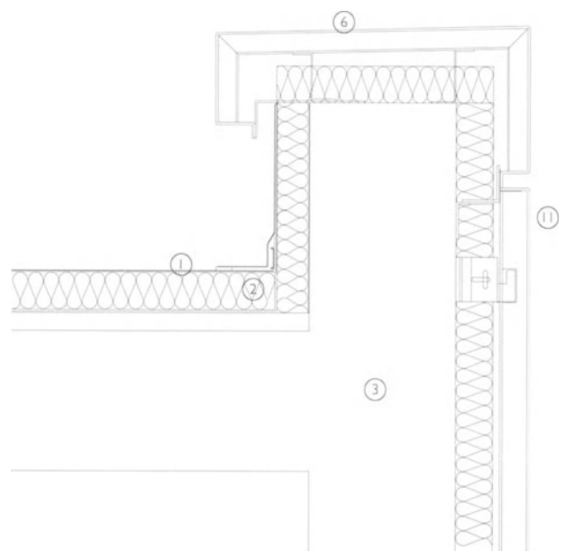
Vertical section 1:10. Low parapet
