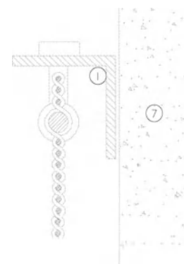
1:2 Section through woven mesh fixed to wall
