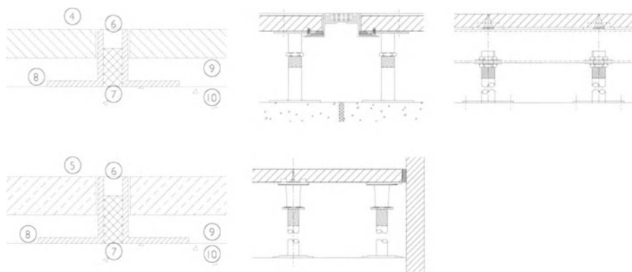
Vertical section
