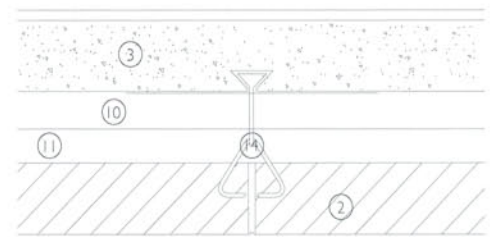
Plan 1:10. Typical wall system showing wall tie
