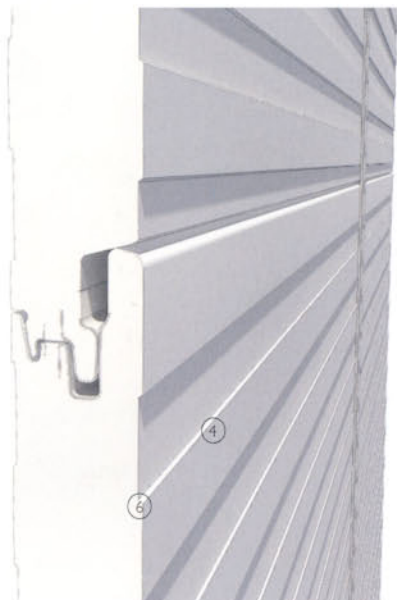
Connection profile for vertical two-way interlocking profiled panels
