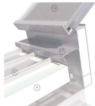
3-D view of metal roof at abutment
