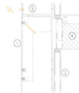
Plan view of twin wall with openable screen
