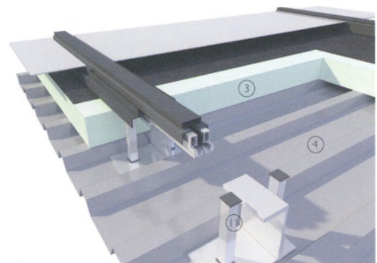
3-D view of metal rainscreen roof assembly with optional capping to seam
