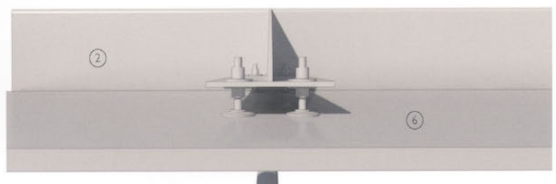
3-D detail of louvre support
