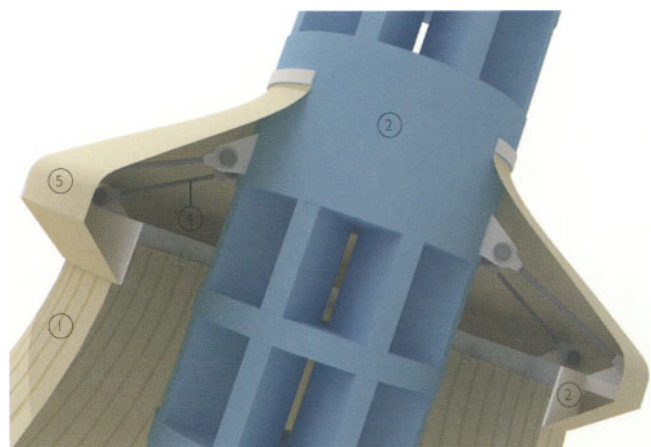
3-D detail of alternative pinnacle condition with membrane hood
