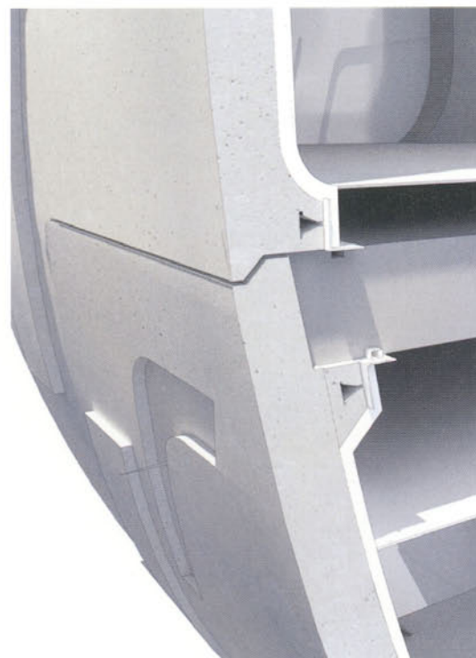
Structural in-situ reinforced concrete backing wall with precast concrete cladding
