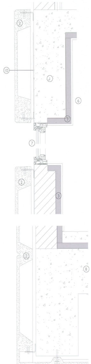
Section 1:10. Panel soffit and window junctions of GRC panels with open joints
