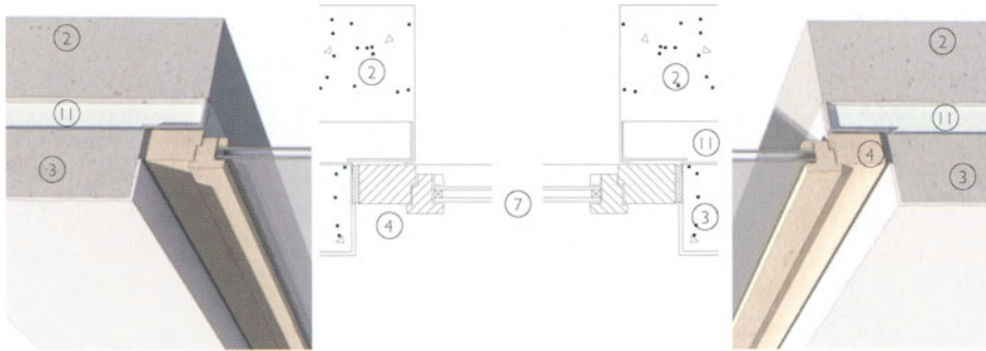
3-D view & horizontal section 1:10. Concrete wall: Insulation set within wall
