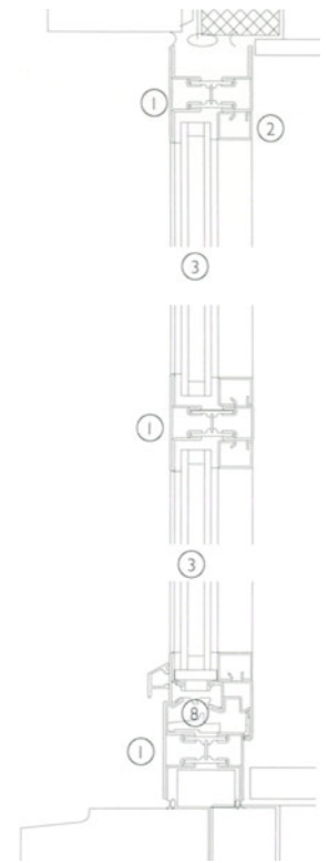
Section 1:5 Pressed Steel window, thermally broken
