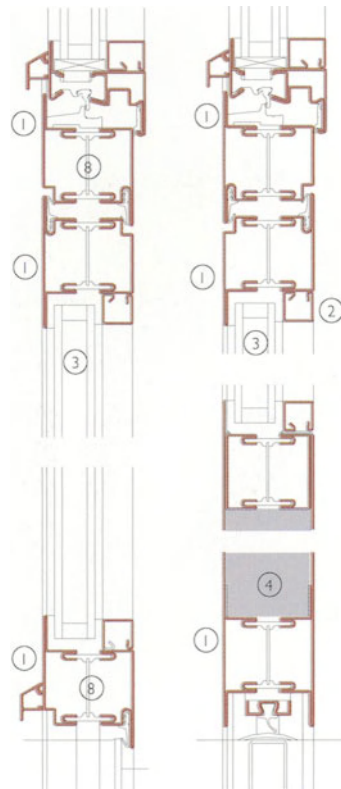
Sections 1:5 of pressed steel doors with thermal breaks. Left: Outward opening. Right: Inward opening
