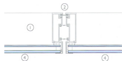
Horizontal section 1:5 through unitised mullion
