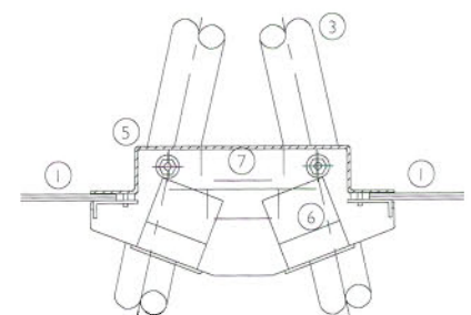
Vertical section
