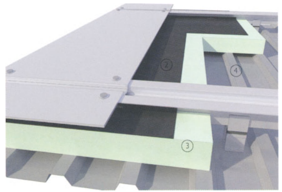
3-D view of metal rainscreen roof assembly
