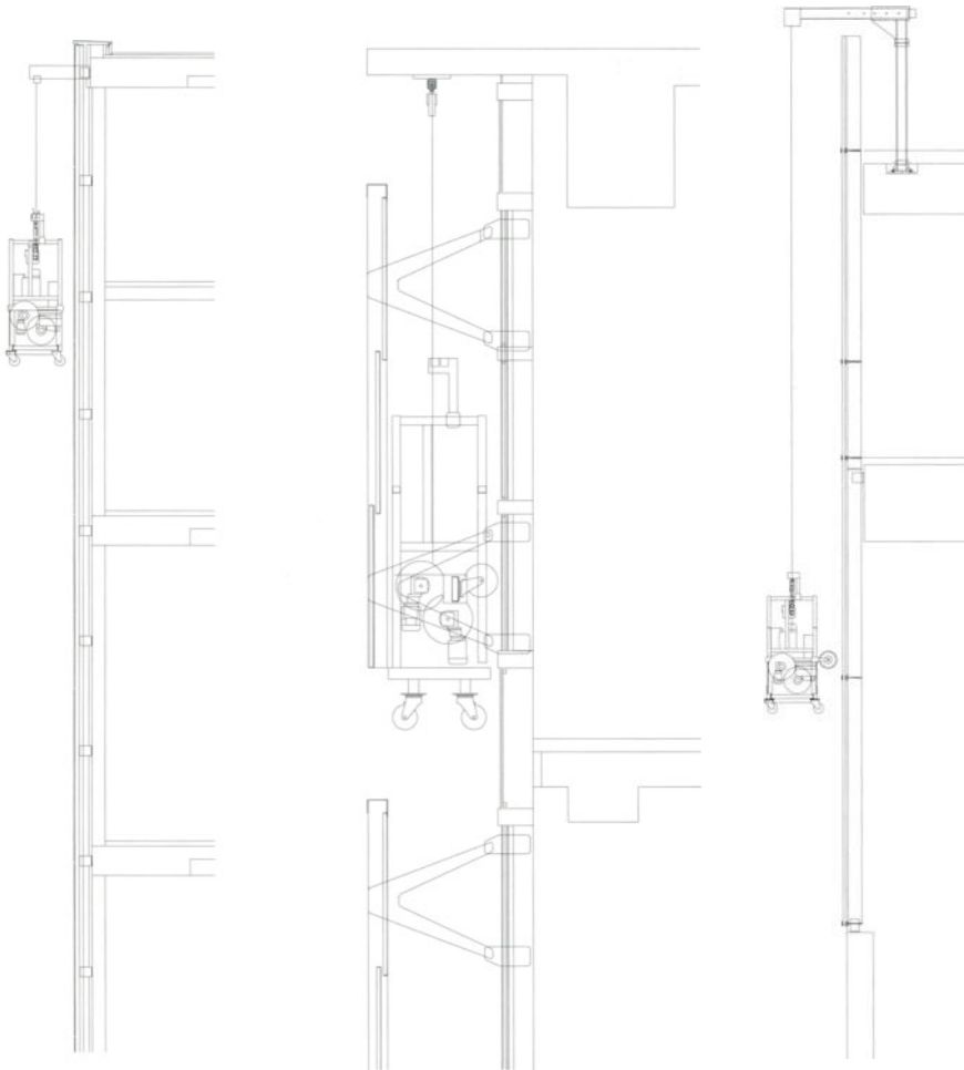
Section 1:100 and 1:50 Monorail supporting cradle from cantilevered brackets/ beam
