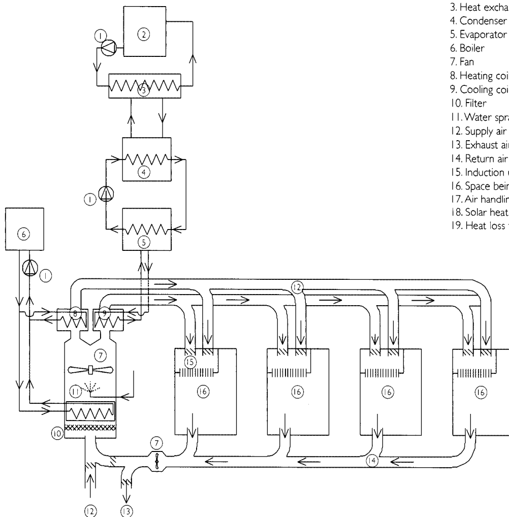
Dual duct CAV system
