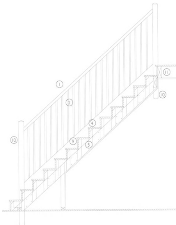
Vertical section
