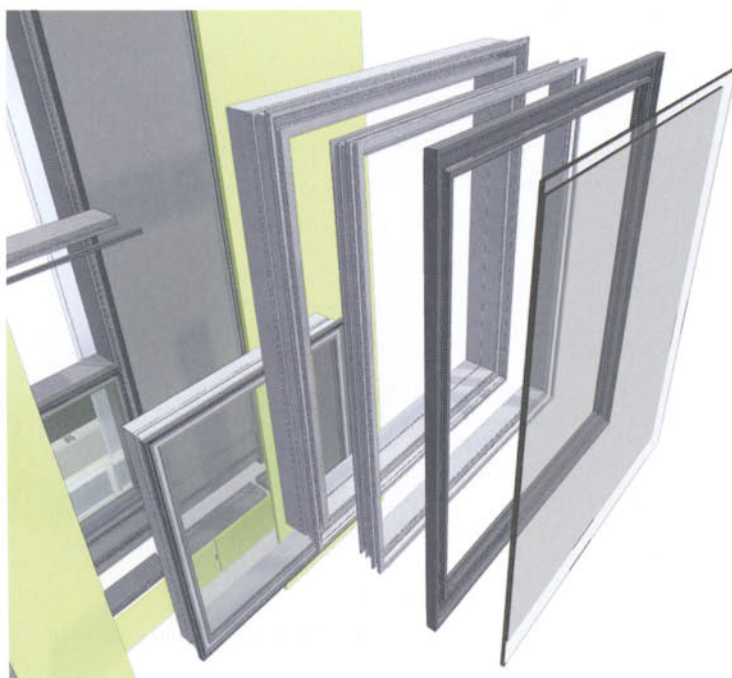
Exploded view showing window assembly within stick based curtain wall
