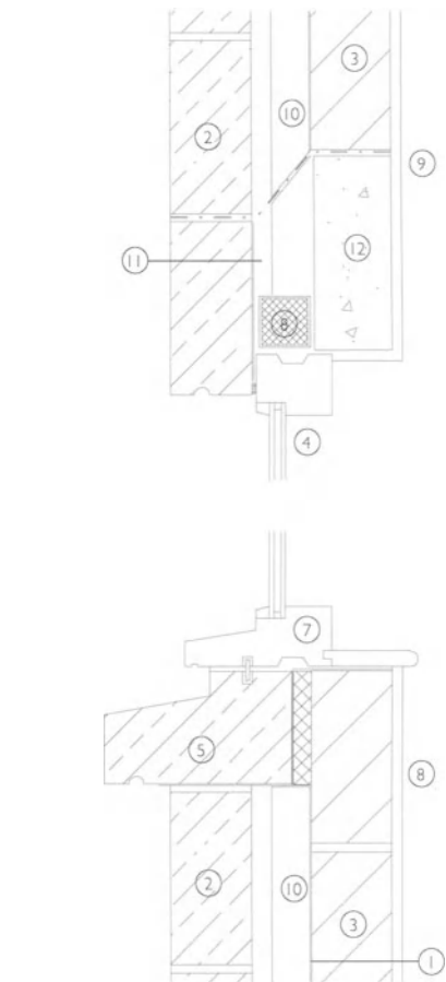
Vertical section 1:10. Typical window at cill and head in block cavity wall system
