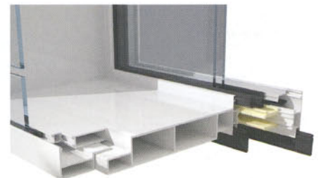
Detail of unitised connection for double skin mullion
