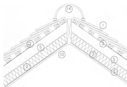
Section I:20. Ventilated roof
