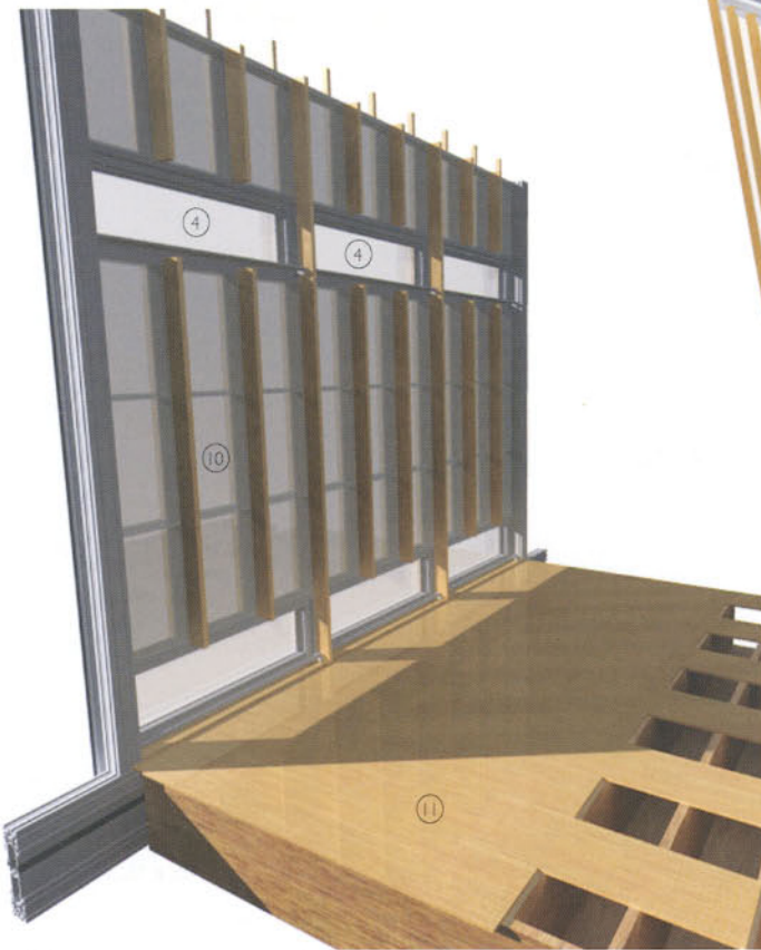
3-D detail of window wall connection to floor system
