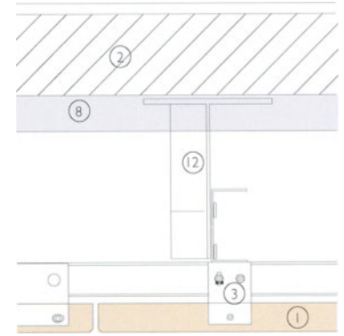
Plan 1:10. Typical stone carrier system made from extruded aluminium section
