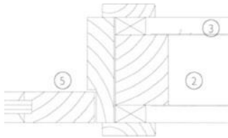
Horizontal elevation
