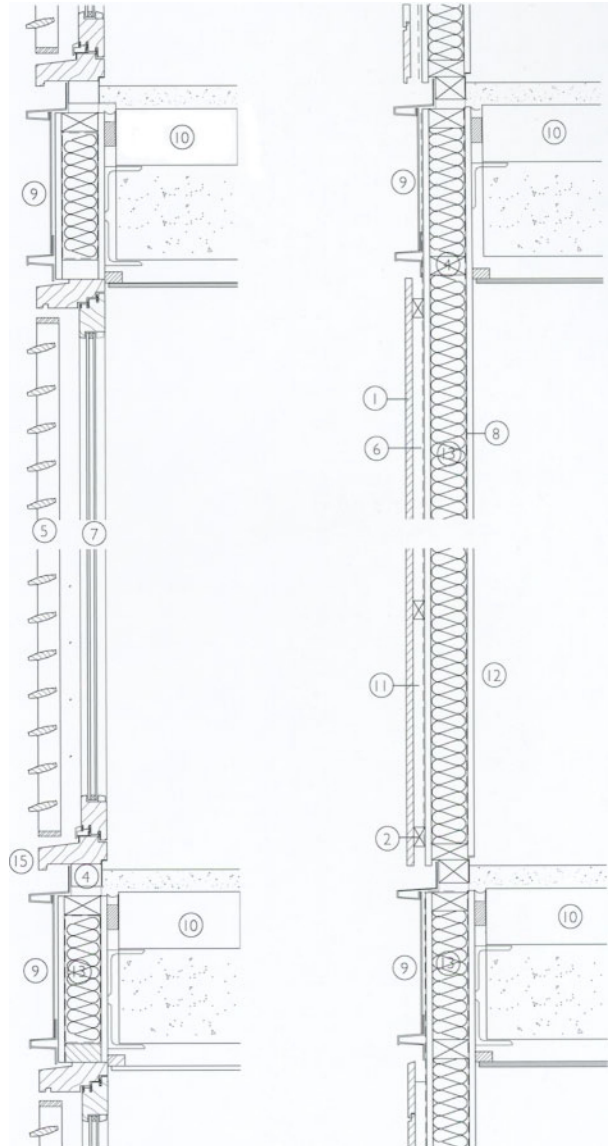
Vertical section 1:10 through timber cladding panels showing typical details
