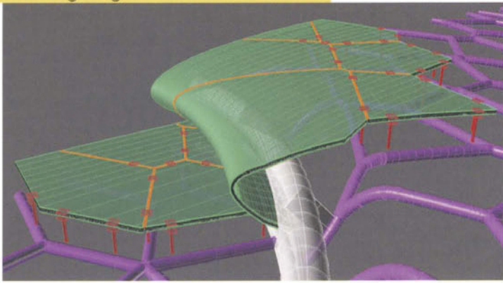
Images of a system which uses a facade structure based on a voronoi pattern to support irregular shaped glazed panels
