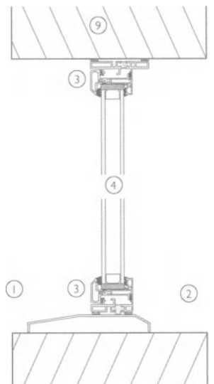
Vertical section 1:10. Outward opening aluminium window set within typical wall construction
