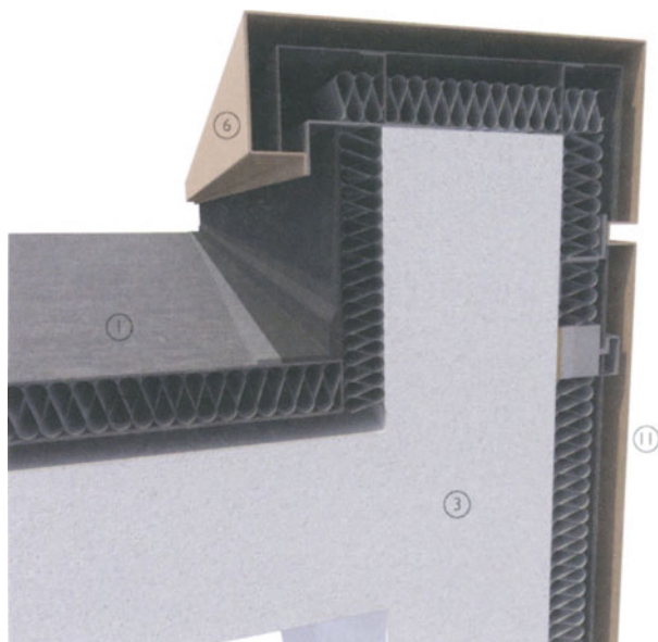
3-D detail of low parapet
