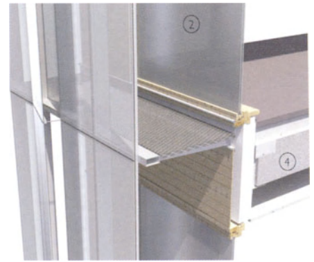
3-D section cut through double skin system with openable screen
