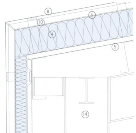
Vertical section 1:10. Folded Eaves
