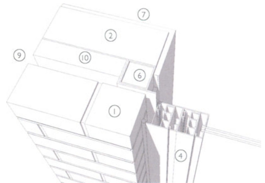
Isometric detail through window connection
