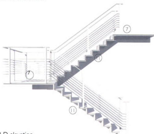
3-D elevation
