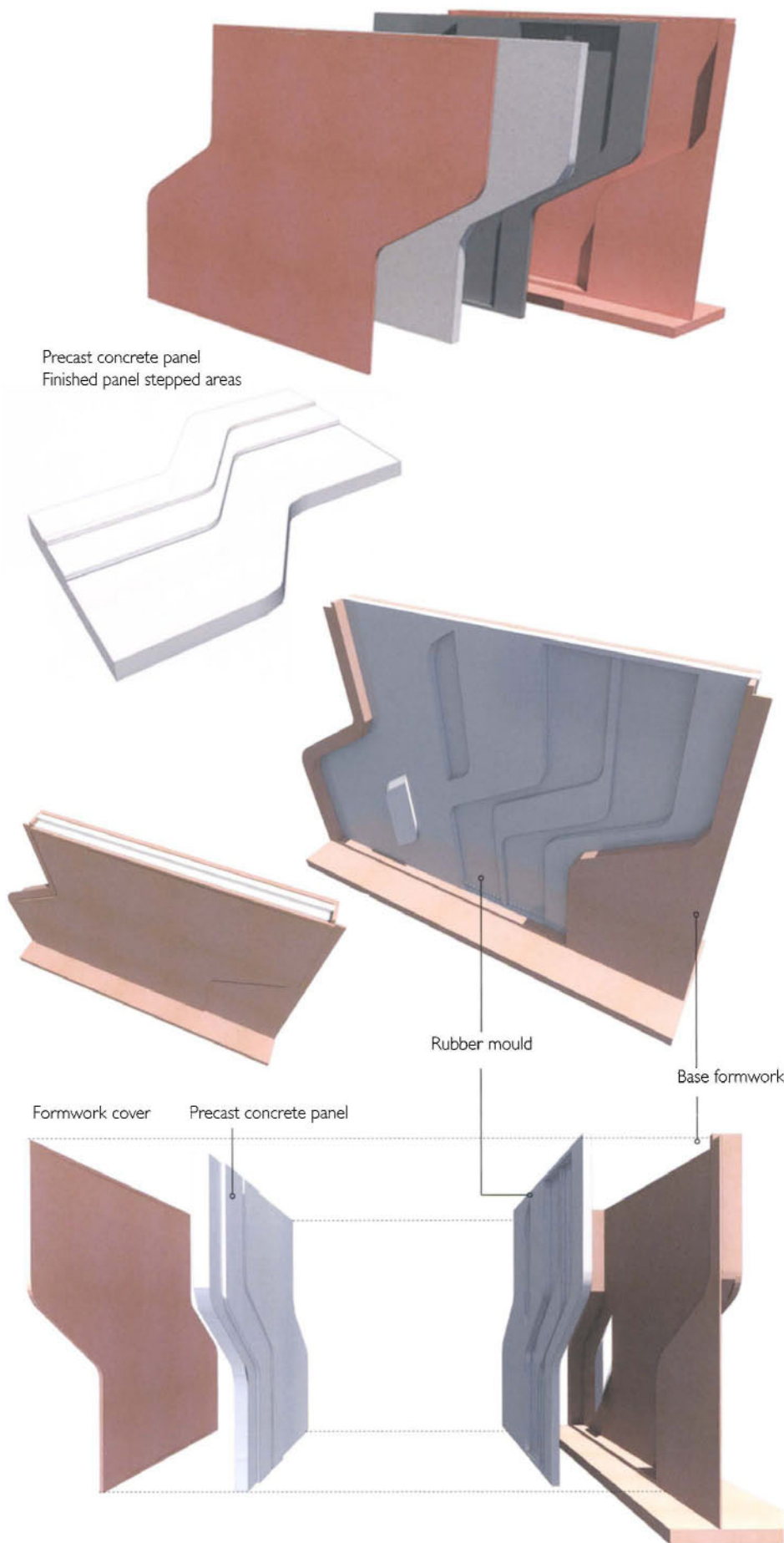
Rendered views showing process of precast concrete panel
