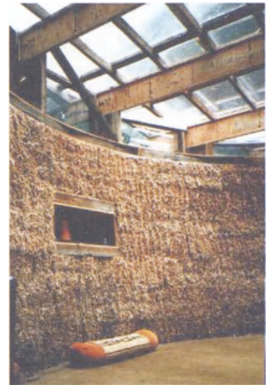
Strawbale dance studio, London.
