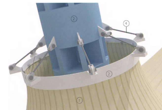
3-D detail of cone top with protruding structural support
