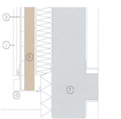
Vertical section 1:10 through typical wall system
