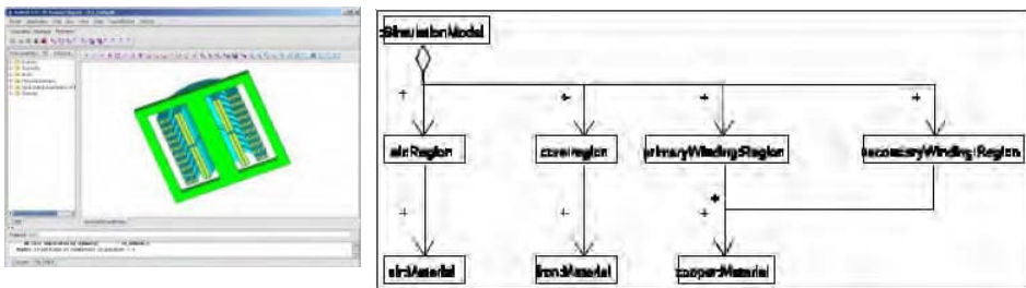
Fig. 2: Geometric model of a transformer and its object diagram
