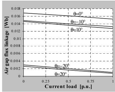
Fig. 7. Air gap flux linkage for different current loads at various rotor displacements
