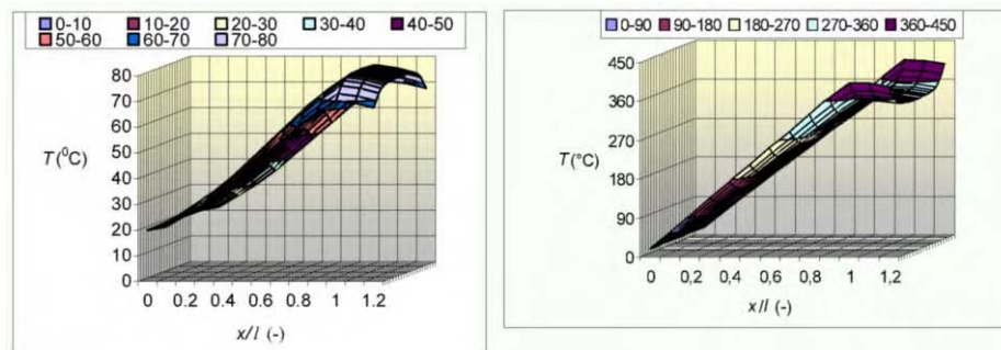
Fig. 4. Temperature distribution on the upper plane of the moving brass strip ( v = 0.02 m/s) heated inductively in TFIHS supplied by the field current of frequency a) f = 50 Hz, b) f = 2000 Hz
