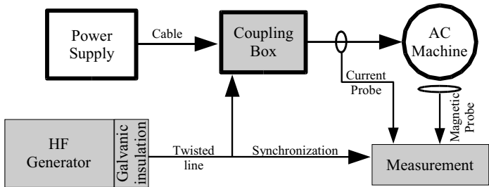
Fig. 4. Synopsis of monitoring system.
