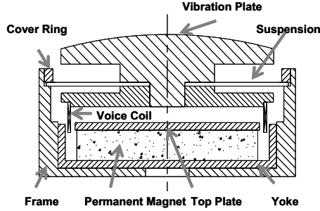
Fig.1 Schematic of BCV
