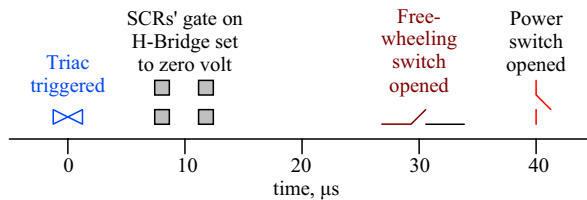
Figure 4 b): De-energising procedure. (The triac trigger pulse lasts for about 160 \mu s to ensure that its current is properly established before its gate voltage is removed.)
