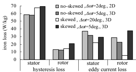
Fig.5. Comparison of iron loss.
