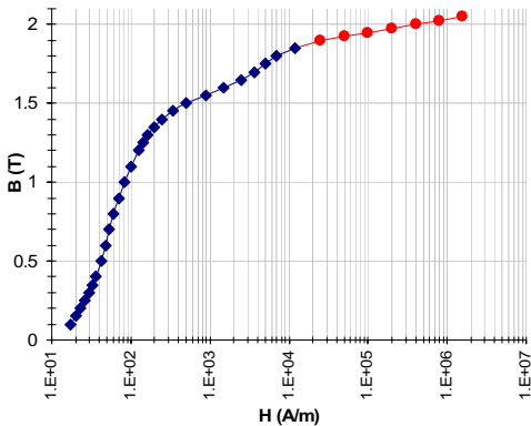
Fig.2 Magnetization curve of the magnetic steel used in the electromagnet.
