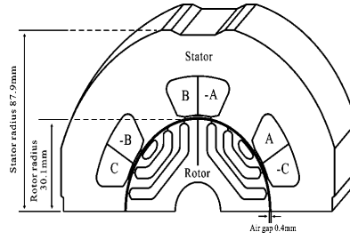
Fig. 1 The initial design model of the SynRM
