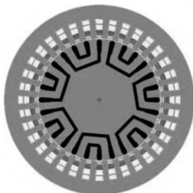
Fig. 1. B.D.F.I.M. diagram
