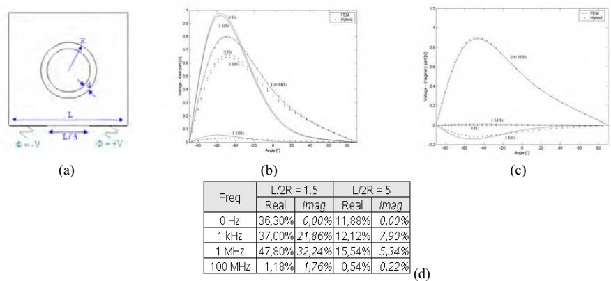
Fig. 6. Coplanar electrodes : general view (a); comparison of FEM and hybrid results for \Phi(R) , L/2R = 1.5 : real (b) and imaginary (c) parts ; FSR error on amplitude (d)
