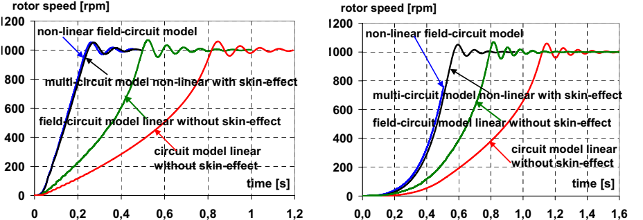
Fig. 3. Speed versus time during soft starting for different circuit and field-circuit models of the induction motor Sf 400Y6
