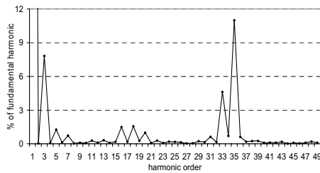
Fig. 8 Harmonic spectrum of induced voltage in measuring coil D, where the fundamental harmonic equaled 1,24 V
