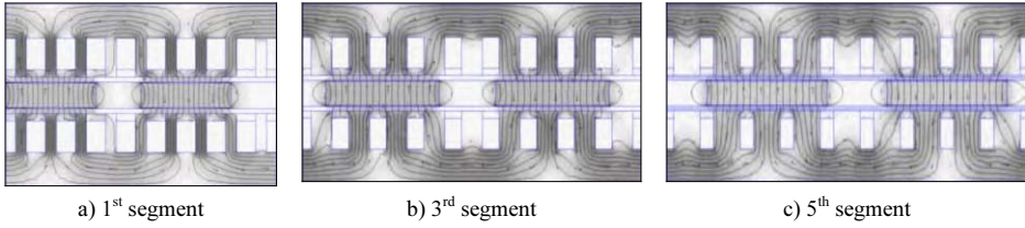
Fig. 3. Magnetic field distribution at no load
