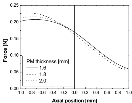
Fig.4 Magnetic force
