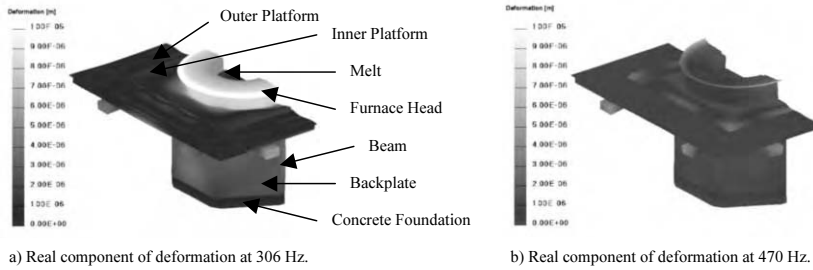
Fig. 2: Results of the structure-dynamic simulation.
