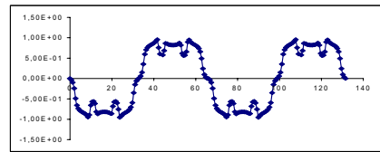
Fig. 7. Radial magnetic field – FE model
