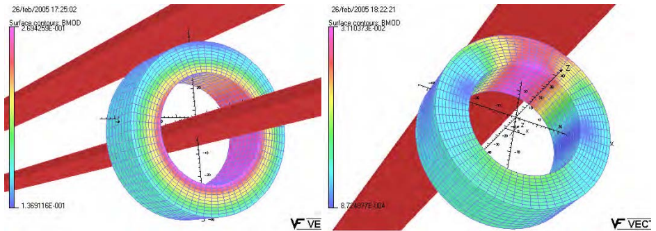
Fig 3. Simulation of the single circuit model with two conductor, I_{CIN} = 150A ; I_{CEX} = 300A . Fig 4. Influence of current near to conductor, I_{CIN} = 0A ; I_{CEX} = 300A .
