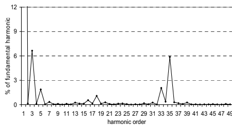
Fig. 6 Harmonic spectrum of induced voltage in measuring coil B, where the fundamental harmonic equaled 2,54 V
