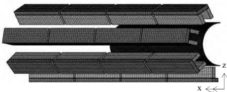
Fig. 4. 3-D finite element mesh (except the air).
