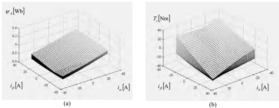
Fig. 4. The families of surfaces resulting from FEM. (a) phase A flux. \Psi_A = \Psi_A(i_\alpha, i_\beta) | \theta \in [0 \div 30] . (b) electromagnetic torque T_e = T_e(i_\alpha, i_\beta) | \theta \in [0 \div 30] .
