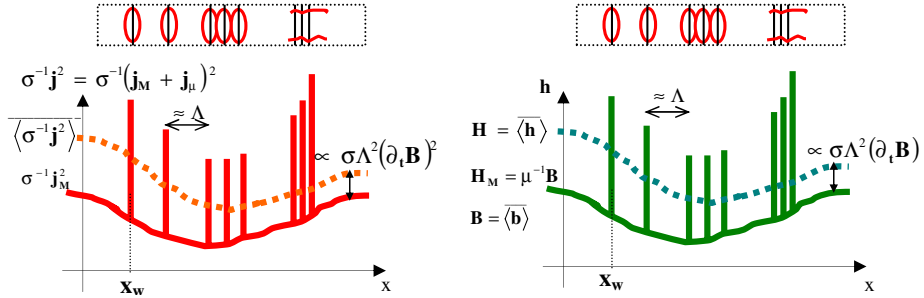
Figure 1: Actual (plain lines) and smoothed (dashed lines) squared eddy currents (on the left) and magnetic field (on the right) distributions. \mu is the static permeability. \langle \cdot \rangle means to smooth and upper score to take the space average of the distribution as it will be developed in the following.
