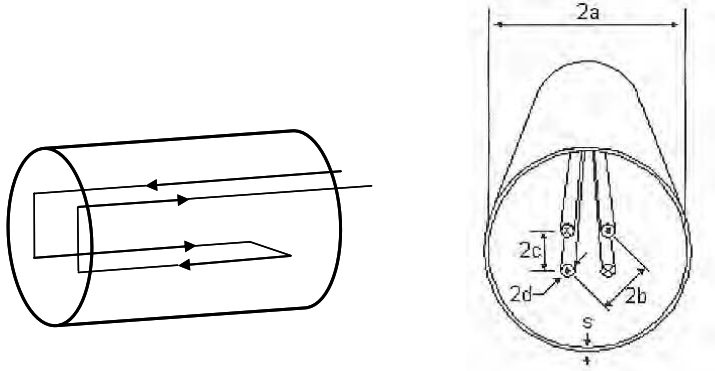
Fig. 1 Geometrical and electrical parameters of the studied resistor: a = 47.5 mm; b = 7.07 mm; c = 5 mm; d = 16 \mu\text{m} ; s = 3 mm; length of wires h = 51 cm; length of shield h_s = 55 cm. Wire dc resistance R_{dc} = 12906.403555 \Omega , aluminium resistivity \rho_a = 2.655 \times 10^{-8} \Omega\text{m} ; Evanhom and aluminium magnetic susceptibility \mu = \mu_0 = 4\pi \times 10^{-7} \text{ H/m} ; terminal capacitance C_t = 4.07 \times 10^{-14} \text{ F} .
