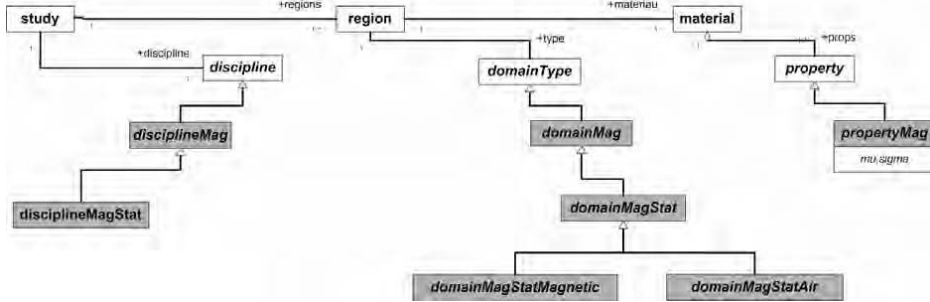
Figure 2 – Data model with added classes in magneto static case
