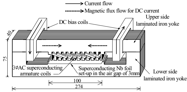
Fig. 2 Structure of fabricated linear-type magnetic flux pump [5,6].
