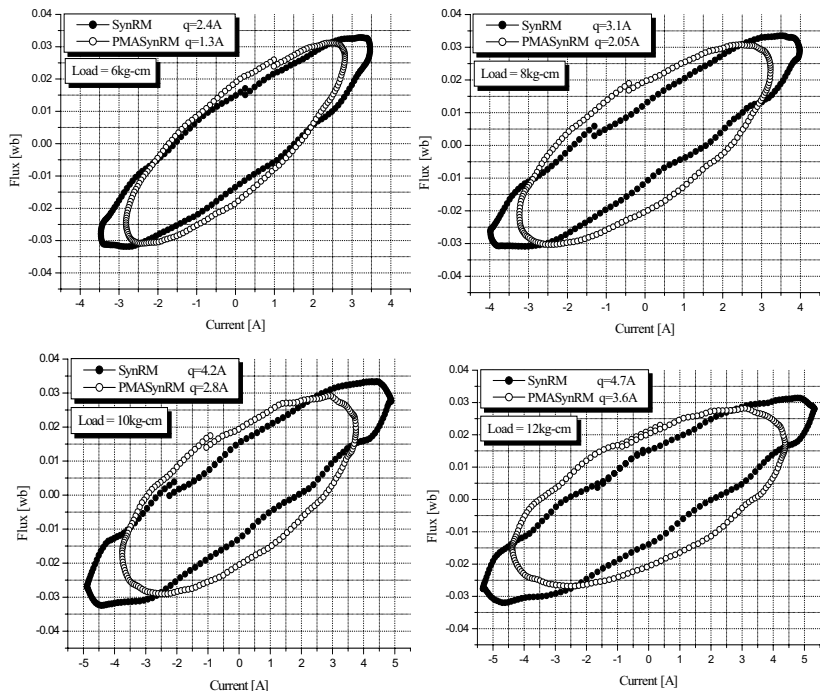
Fig.4 i-λ loci in each load condition
