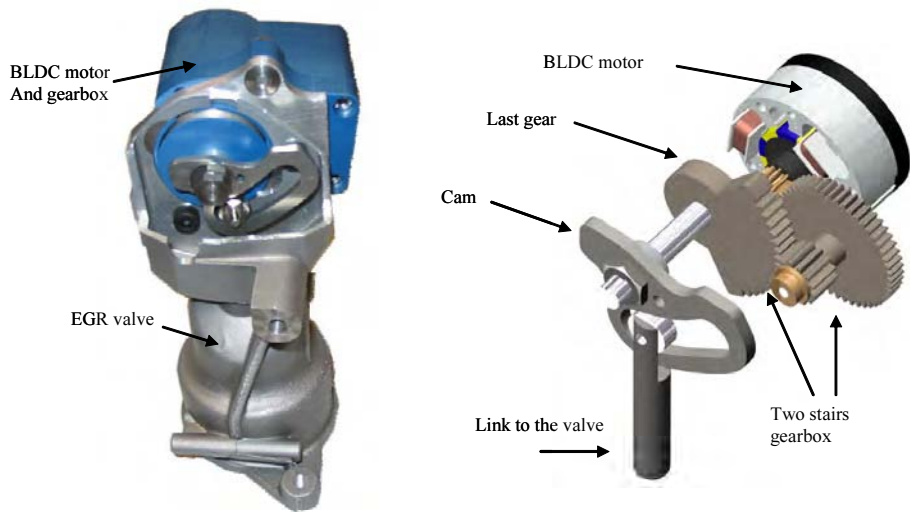
Fig 1 : EGR system and MM41 view
