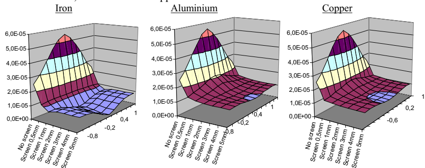
Figure 6 - Lateral screening with iron, aluminium and copper.
