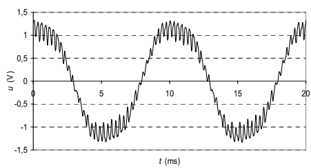
Fig. 4 Induced voltage in measuring coil D (pasted on stator teeth, l = l_{Fe}/16 )
