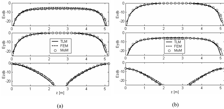
Fig. 3 – Electric field components along the z -axis, f = 2.0\text{ MHz} , \Phi = 0^\circ (a) and 180^\circ (b).
