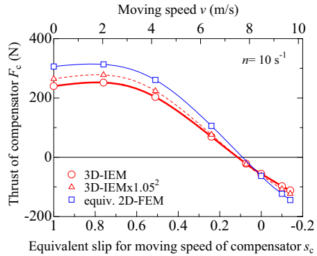
Fig. 10. Thrust of compensator.
