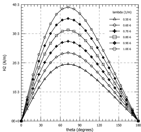
Fig.3 Distribution of the circuital component of magnetic field intensity on the cylinder surface, for z = 0 , and different parameters \lambda (see eq. (1)).
