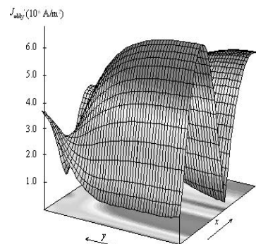
Fig. 3. Distribution of the module of eddy currents at mains frequency f = 50 Hz in the internal plane of flat brass strip for strip width b = 0.25 m
