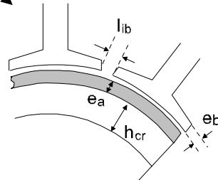
fig.4: definition of studied parameters
