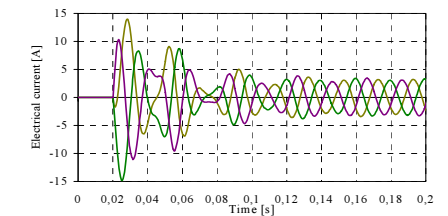
Figure 5: Numerical calculated electrical phase currents for the machine with semi-closed stator slots.
