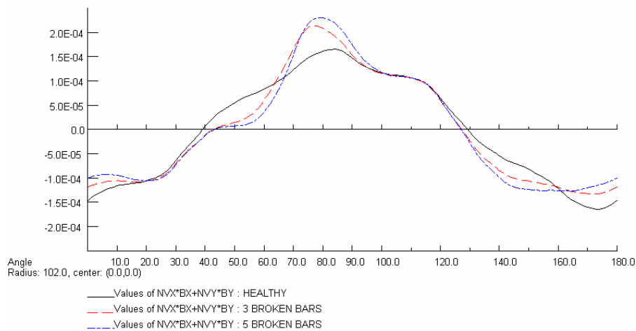
Fig. 6. Distribution of the radial component of the induction field, outside the stator for: the healthy case and for the cases of 3 and 5 broken bars.
