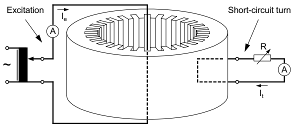
Fig. 3. Electrical scheme of the laboratory model.
