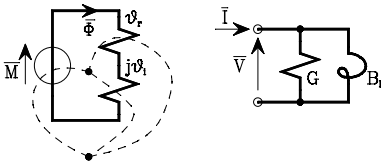
Fig.2. The rule of Colin Cherry in the case of complex characteristic relation B = \mu \cdot H .
