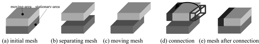
Fig. 1. Mesh modification method.
