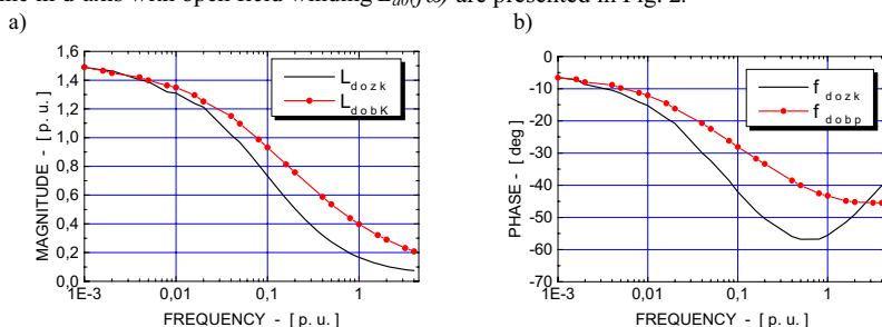
Fig. 2. Frequency characteristics of spectral impedance in d-axis for two constructional rotor structure with opened field winding L_{d0zk} – with damping cage, L_{dobk} – without damping cage a) magnitude, b) phase
