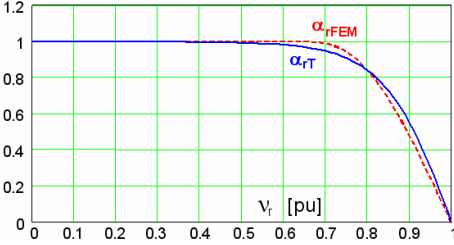
Fig.1 Selected MS-FEM analysis for the determination of the rotor field functions:
