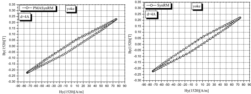
Fig. 7 B-H Curve in a yoke of PMASynRM and SynRM
