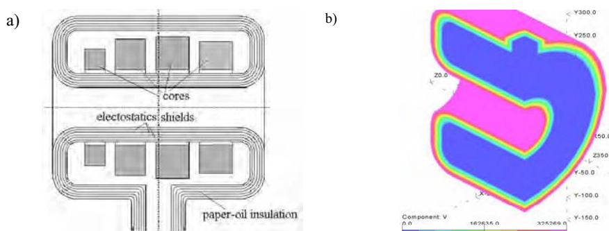
Fig.2 The casing with cores and paper-oil insulation with electrostatic shields and distribution of electric potential inside paper-oil insulation of the casing
