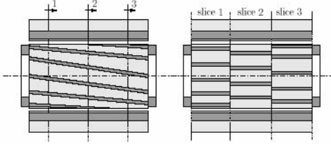
Fig. 1. Multi-slice model: approximation of skew by means of three slices of equal length
