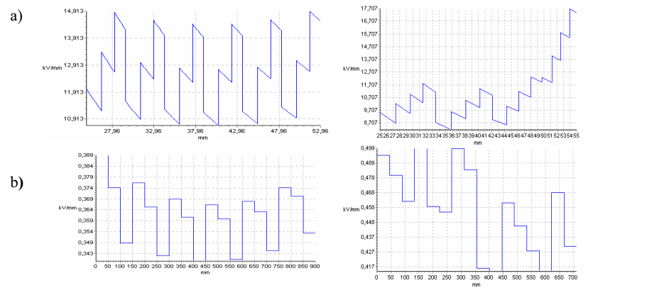
Fig.4 Distribution of the electric field strength in the insulation system with capacitance control for an old (left hand column) and new (right hand column) method of placing electrostatic shields a) in the axis direction and b) in the radius direction
