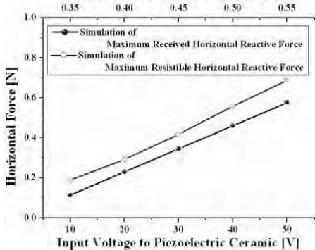
Fig.10 Analysis result of the maximum received and resistible horizontal reactive forces at the electromagnet by using FEM.
