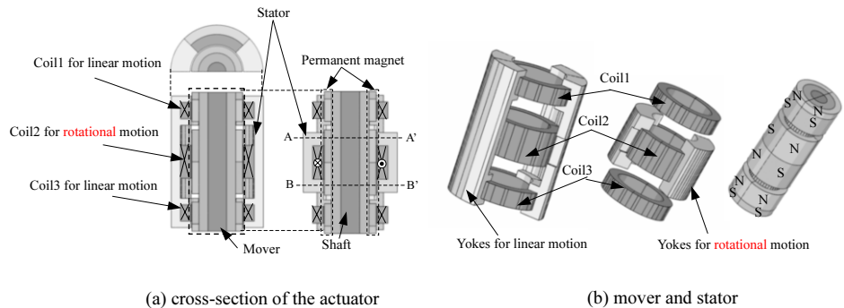
Fig.1 Basic structure.
