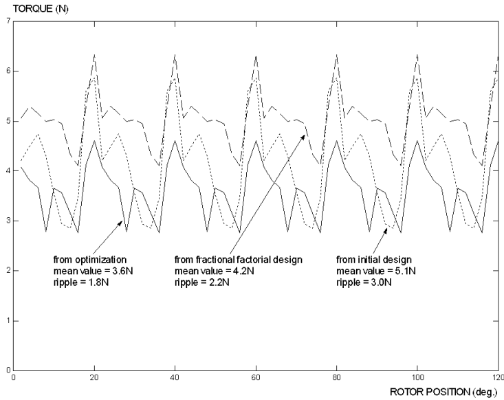
fig.7 : Torque obtained for analytical study, fractional factorial design (experiment n°5) and optimization.
