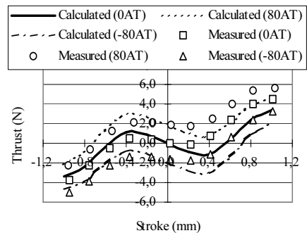
Fig.4 Comparison between measured and calculated thrust characteristics.
