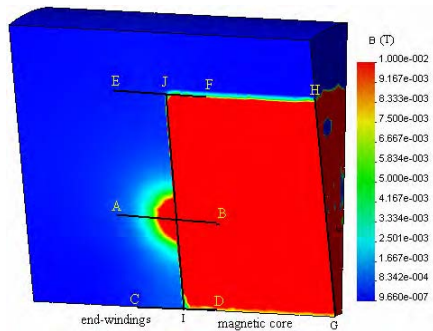
Fig.5 Magnetic flux density ( 0 < B < 0.01 T)
