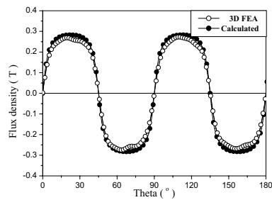
Fig. 6. Flux density of axial component.
