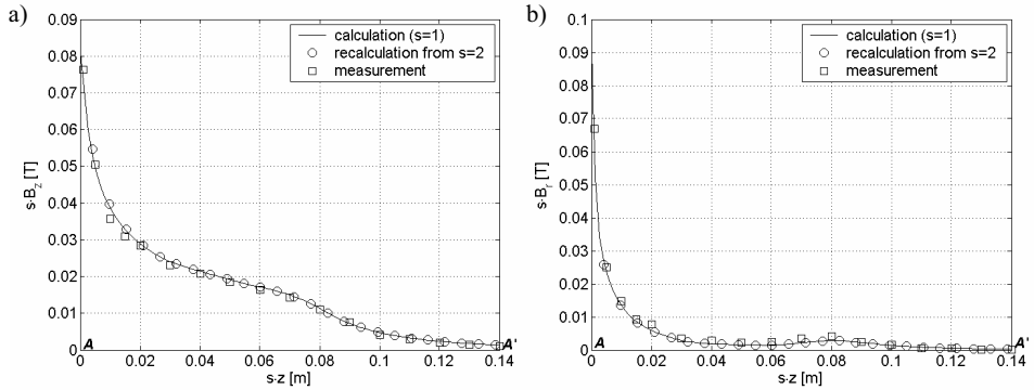
Fig. 4. The recalculated B_z and B_r components along the line A-A' (current value I=1A )
