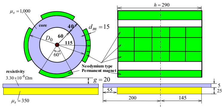
Fig. 3 Test machine of magnet rotator type of compensator.
