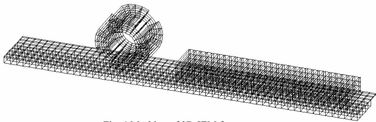
Fig. 4 Meshing of 3D-IEM for compensator.
