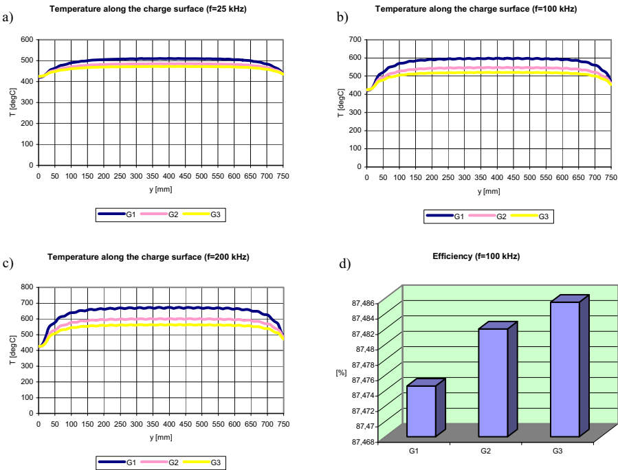
Fig. 3. Charge surface temperature (a, b, c) and electrical efficiency of system (d)
