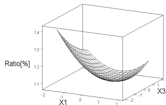
Fig. 4 Response Surface for the Ratio of 6slot
