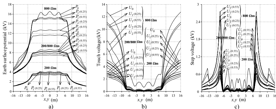
Fig. 4. Distribution of: a) earth surface potentials; b) touch voltages; c) step voltages along a diagonal of the grid for different volumes of soil layers impregnated with an additional substance in all three soil structure models.
