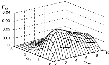
Fig.6 Dependencies F_{rz} = f(\omega_{rm}, \alpha_r) a - a_r = 0.3, b_r =
