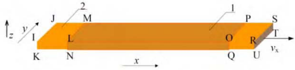
Fig.1 Calculation model of coupled electromagnetic (Fig.1a) and temperature fields (Fig.1b) \Omega_1 – strip, \Omega_2 – winding, \Omega_3 – magnetic core, \Omega_4 – air-gap and surroundings. 1- part of the strip located in the air-gap, 2 – remaining part of the strip being outside the inductor
