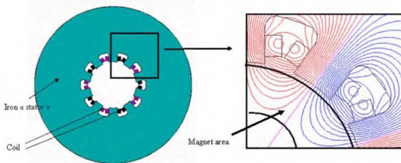
Fig 1 : Magnetizer device and polar magnetization.
