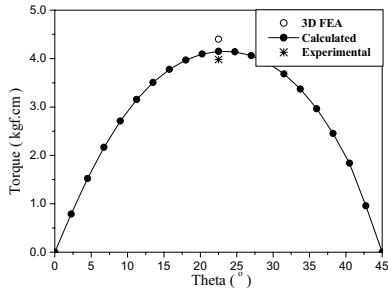
Fig. 8. Comparison of magnetic torque.
