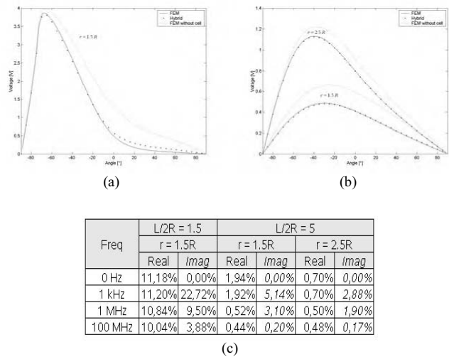
Fig. 7. Coplanar electrodes : comparison of FEM and hybrid results, f = 0\text{Hz} : L/2R = 1.5 , r = 1.5R (a) and L/2R = 5 , r = 1.5R and r = 2.5R (b); FSR error on amplitude (c)
