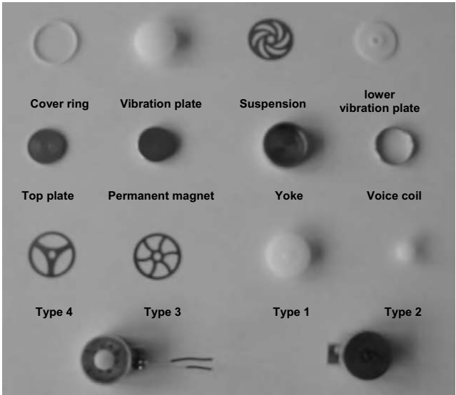
Fig.9 Photograph of the BCV
