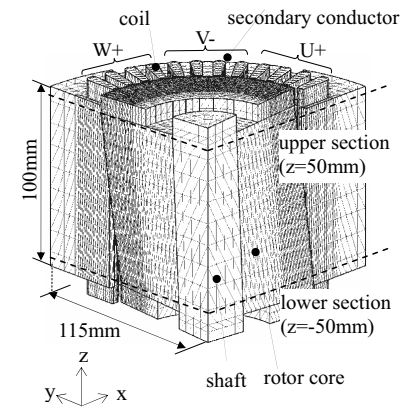
Fig.2. Analyzed model (skewed model).
