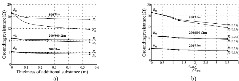
Fig. 3. The influence of: a) additional substance thickness; and b) surface ratio on grounding resistance.
