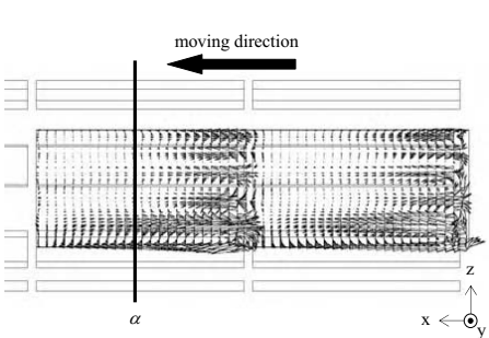
Fig. 5. Distributions of eddy current density vectors ( v = v_0 (m/s)).
