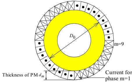
Fig. 7. Equivalent model of magnet rotator for 2-D FEM.
