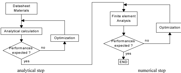
Fig. 1: Synoptic of the complete design process
