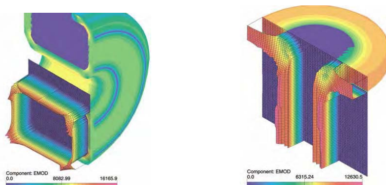
Fig.5 Distribution of electric field strength [V/mm] inside paper-oil insulation
