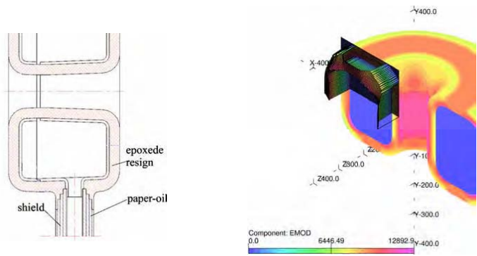
Fig.7 Diagram of joining paper-oil and epoxide resin insulation and distribution of electric field strength [V/mm] inside epoxide resin insulation for versions with casing corners 40mm joining paper-oil and epoxide resin insulation
