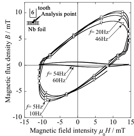
Fig.6 Frequency dependence of hysteresis loops for a travelling magnetic field in the superconducting Nb foil. Analysis point is illustrated in the inset (see Fig. 4 for the tooth number 6).
