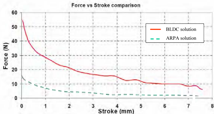
Fig 6: Force versus stroke.
