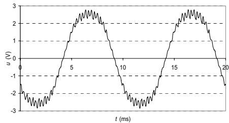
Fig. 3 Induced voltage in measuring coil C (pasted on stator teeth, skewed, l = l_{Fe}/2 )
