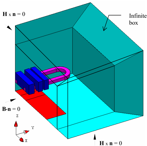
Fig. 2. Computation domain and boundary conditions
