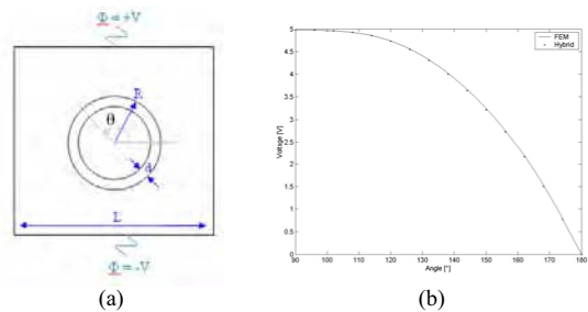
Fig. 3. 3D case : general view (a); comparison of FEM and hybrid results for \Phi(R) , null frequency (b)
