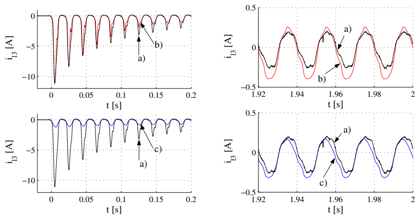
Fig. 6: Line current i_{l3} during switch-on and in steady state: a) measured; b) calculated - \psi(i) characteristic determined by alternative method; c) calculated - \psi(i) characteristic determined by standard method.
