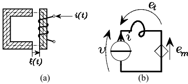
Fig.4. Time-varying magneto-electric system with one mesh and corresponding electric network.
