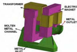
Fig.1 Physical construction of the electromagnetic pump with all ceramic shapes deleted.
