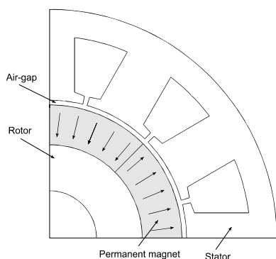
Fig. 1. Structure of the traction motor
