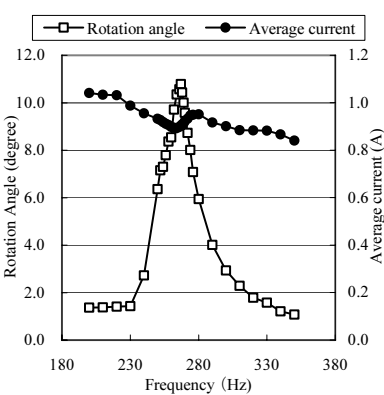
Fig.9 Measured frequency characteristics (rotation).
