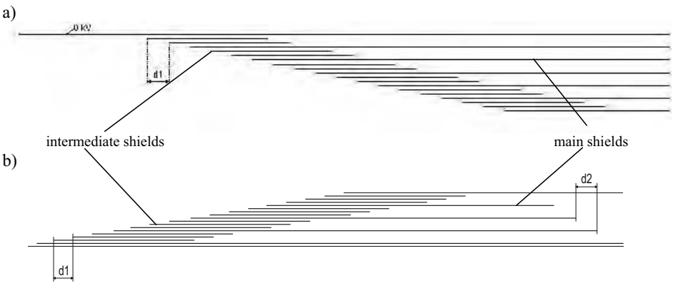
Fig.3 The difference between an old (a) and new (b) method of placing electrostatic shields
