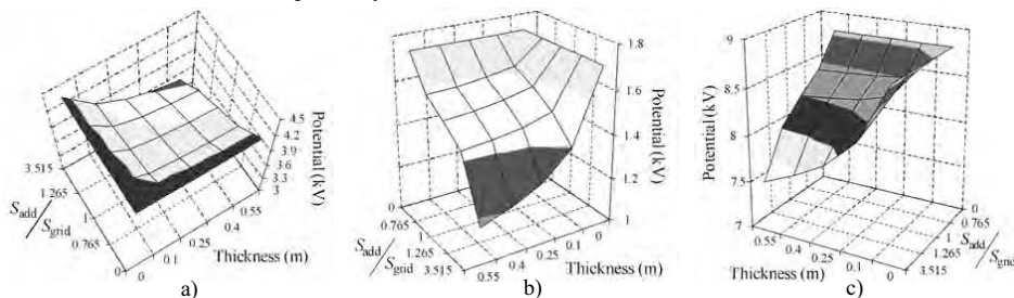
Fig. 2. 3D plot of the additional substance thickness and surface ratio influence on the ground potential rise in case of: a) uniform soil model 200 \Omega m; b) uniform soil model 800 \Omega m; and c) two-layer soil model 200/800 \Omega m
