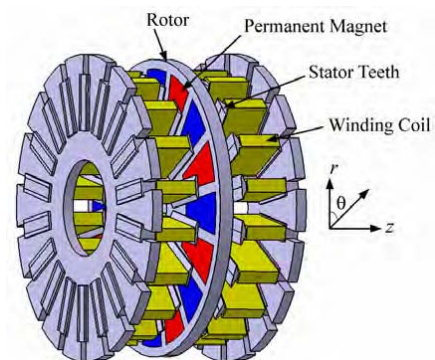
Fig. 1. The structure of AFPM motor with the innovated slot.
