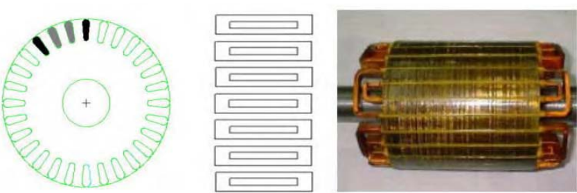
a) Nest distribution b) Rotor loops scheme c) Prototype
