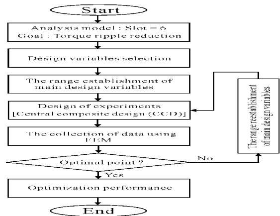
Fig. 5 The flow chart of design procedure
