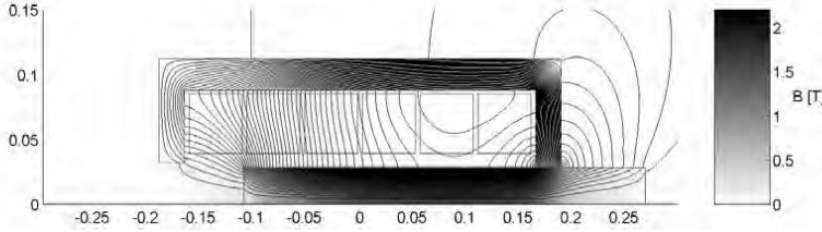
Fig. 1. Flux density map and field lines for the scaled (enlargement s=2 ) actuator ( I=1\text{A} )
