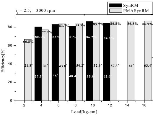
Fig. 5 Efficiency, current angle and runaway point of PMASynRM and SynRM according to load in experimental test
