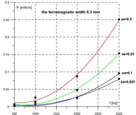
Fig. 2 The specific power losses vs. frequency. aa – the half of the domain width
