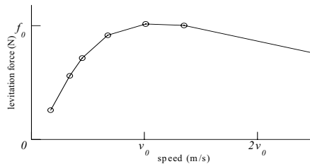
Fig. 11. Average value of levitation force characteristics.
