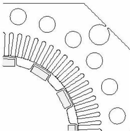
Fig.1 One-quarter of motor geometry
