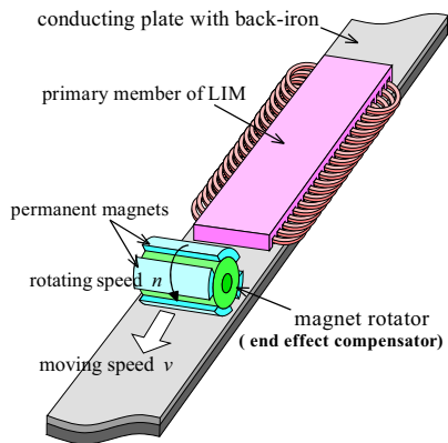
Fig. 1. Model of magnet rotator and LIM.
