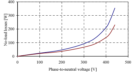
Figure 10: No-load losses for both machines in dependency on the applied voltage.
