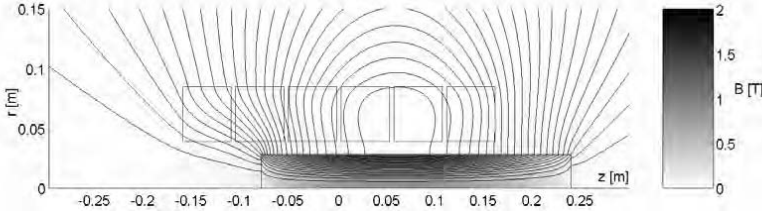
Fig. 2. Actuator with open magnetic circuit ( s=2 , I=1\text{A} )
