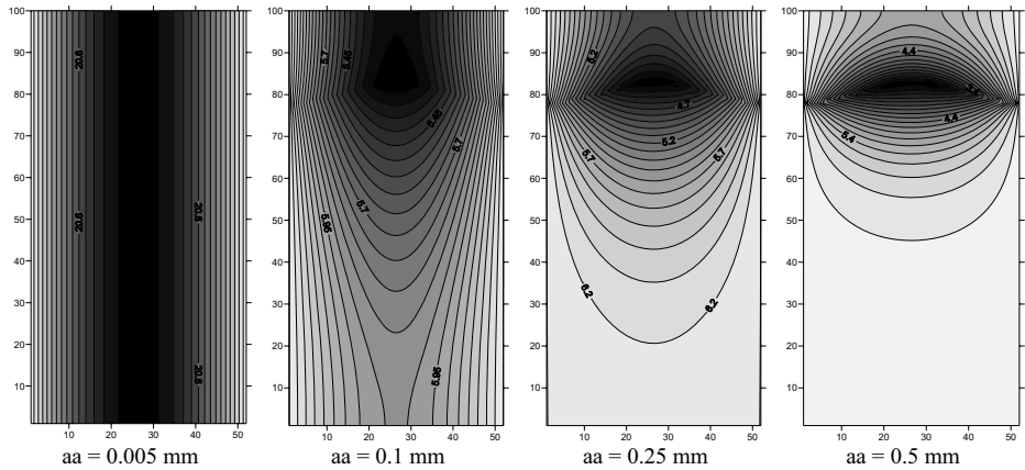
Fig.5 The temporary fields strength distribution. The field frequency – 500 Hz, the ferromagnetic width – 0.5 mm. Model bra-ket 6/100.
