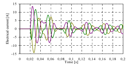
Figure 6: Numerical calculated electrical phase currents for the machine without any stator slots.
