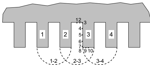
Fig. 8. Positions of the faults and defined lines between teeth.
