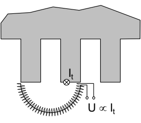
Fig. 4. Position of pick-up coil on stator teeth
