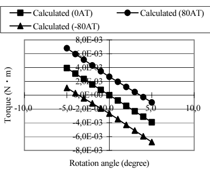
Fig.5 Torque characteristics.
