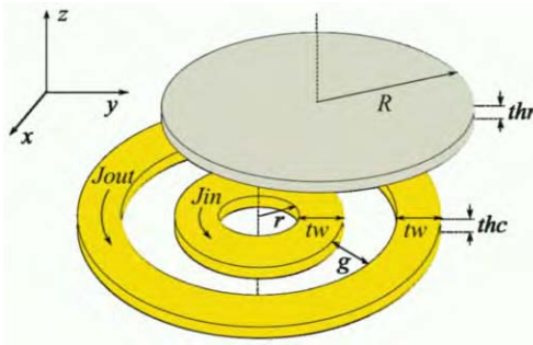
Fig. 1 Micro-motor geometry
