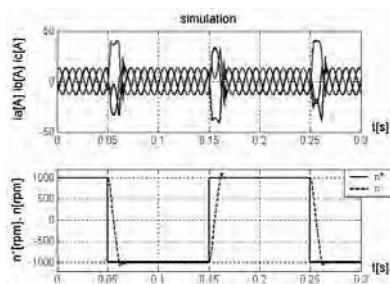
Fig. 10. Simulation results of motor reversing
