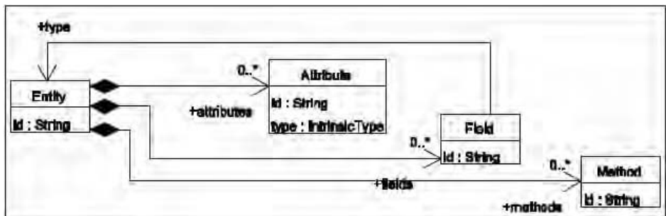
Fig. 3: A basic metamodel
