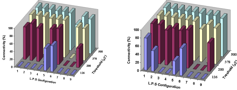
Fig 2 – Connectivity index (%) as a function L.P.S and threshold levels ( \mu T ), for the earth resistances R=5\Omega (Left) and R=80\Omega (Right), Plane \alpha ( y = -5,0m ), and Asymmetric Scenario.
