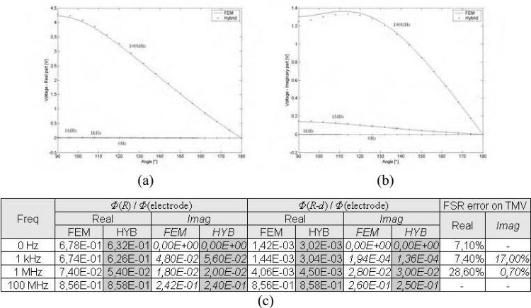
Fig. 8. Face-to-face electrodes, L/2R = 1.1 : comparison of FEM and hybrid results for \Phi(R-d) : real (a) and imaginary (b) parts ; results for TMV = \Phi(R) - \Phi(R-d) (c)
