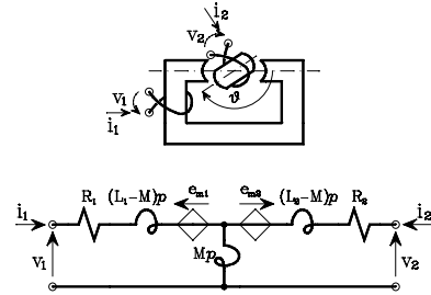
Fig.5. The time varying case for n=2
