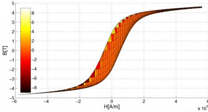
Fig. 5: Boundary conditions of \Psi^+(H^+, B^+)[2] vector field
