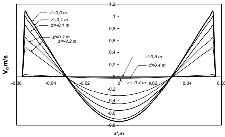
Fig.8 Velocity distribution of liquid metal at the same direction of travelling fields (Fig.2a)
