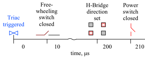
Figure 4 a): Energising procedure (Although not illustrated, the triac triggering pulse lasts for about 120 \mu s to ensure that its conducting current is established above the holding level.)
