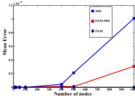
Fig. 7: Plot of the mean error, for FEM only solutions (♦), MM only solutions (■), and FEM-MM solutions (●).
