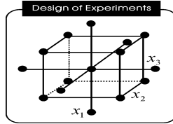
Fig. 3 Central Composite Design for the number of three design variables
