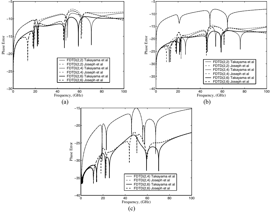
Fig.2 The phase error as a function of frequency for the Lorentz medium with parameters of Fig. 1(b) and \Delta x = 37.5\mu\text{m} and Courant number (a) Q = 0.4 and (b) Q = 0.01 and (c) comparison of the HO schemes for very small time step ( Q = 10^{-4} )
