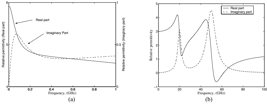
Fig.1 Complex relative permittivity of (a) a Debye medium ( \varepsilon_\infty = 4.048\varepsilon_0 , \varepsilon_{s1} = 5.248\varepsilon_0 , \varepsilon_{s2} = 4.715\varepsilon_0 , \tau_1 = 2.386 nsec, \tau_2 = 0.09 nsec) and (b) a Lorentz medium ( \varepsilon_s = 3\varepsilon_0 , \varepsilon_\infty = 1.5\varepsilon_0 , \omega_1 = 40\pi \times 10^9 rad/sec, \delta_1 = 0.1\omega_1 , G_1 = 0.4 , \omega_2 = 100\pi \times 10^9 rad/sec, \delta_2 = 0.1\omega_2 , G_2 = 0.6 )
