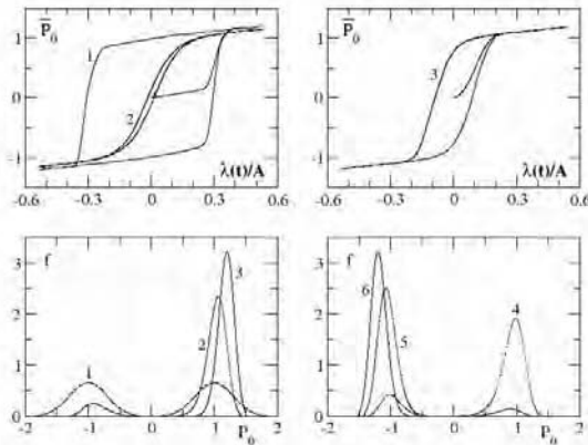
Fig.1 Hysteresis of the mean polarization depending to the external field (top) and the probability distribution over the polarization values at different time moments (bottom). The hysteresis loops 1, 2 (left), and 3 (right) correspond to the noise intensities \theta = 0.01 , \theta = 0.1 , and \theta = 0.05 , respectively. The curves 1 to 6 in the lower pictures show the probability distribution for \theta = 0.05 at the time moments t = 0.0002, 266.68, 1600.4, 3200, 3466.7 , and 4667 . The corresponding values of the external field are 6.18 \cdot 10^{-8}, 0.08143, 0.30886, -0.01804, -0.0987 , and -0.30868 .
