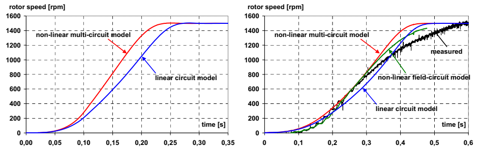
Fig. 4. The curves of the rotational speed vs. time for linear increasing of the voltage during of the time 0,1 s and for polynomial approximation of the rms. value of phase voltage vs. time.
