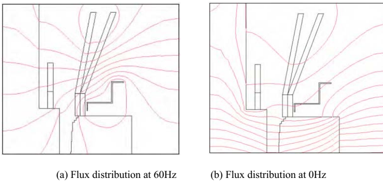
Fig. 7 Flux distribution for frequencies
