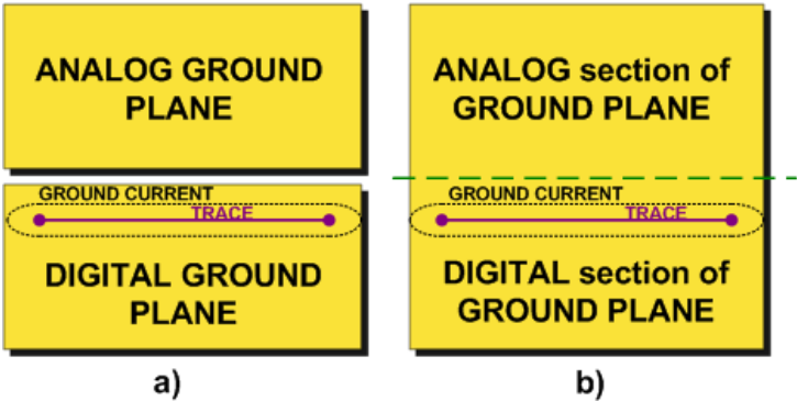
Fig.3 Different grounding strategies: a) Physical isolation (split plane); b) Partitioning
