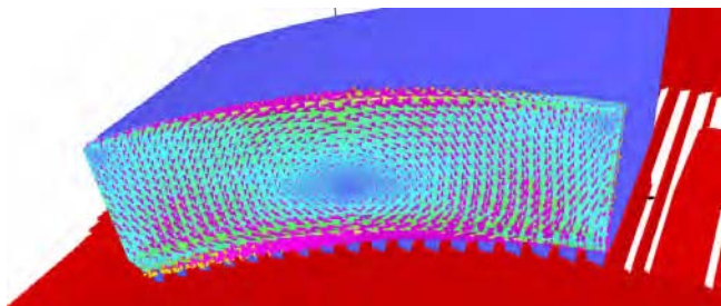
Fig. 1. Eddy current distribution on a clamping plate
