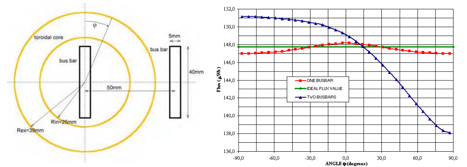
Fig 1. Illustration of the experimental model. Fig 2. Magnetic flux measured with one and two bus bars, versus the angle \varphi of the sensor I_{CIN} = I_{CEX} = 300A .
