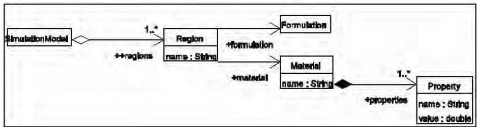
Fig. 1: Partial simplified class diagram of the data model of some simulation software
