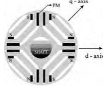
Fig.1 Rotor cross-section of PMA SynRM
