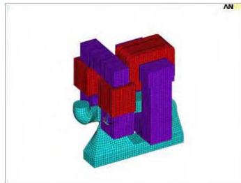
Fig.3 Mesh of the pump. Air elements are not shown.
