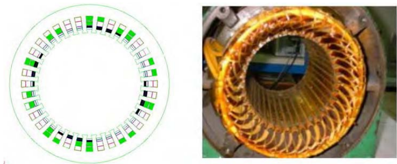
a) Power and control winding distribution. Phase U b) Prototype
