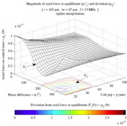
Fig. 5 Verification of axial optimum
