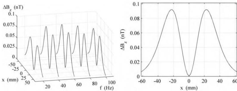
Fig. 8 Calculated changes in magnetic flux density for f = 20 - 100 Hz and for f_{\text{opt}} = 55 Hz
