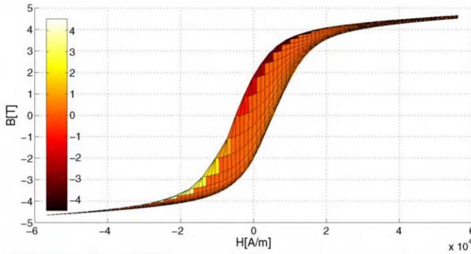
Fig. 4: \psi^*(\mathbf{H}^+, \mathbf{B}^+)[2] vector field without boundary conditions
