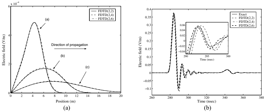
Fig.4 (a) Time history of the electric field through a three-pole Debye medium at several time steps: (i) 0.834\mu\text{sec} (ii) 1.668\mu\text{sec} (iii) 3.336\mu\text{sec} (b) The transmitted, exact and the computed, time-domain solutions at distance 4m away from a two-pole Lorentz slab.
