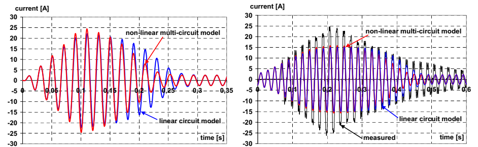
Fig. 5. The curves of the current vs. time for linear increasing of the voltage during of the time 0,1 s and for polynomial approximation of the rms. value of phase voltage vs. time.
