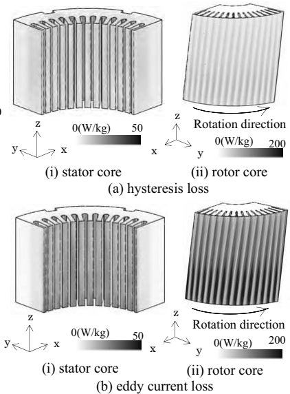
Fig.4. Contours of iron loss ( \Delta\omega = 5 deg.).
