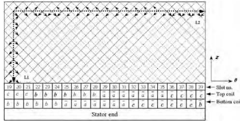
Fig. 4 Current distribution on the stator end winding
