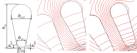
Fig. 3. Comparison of two similar slots, with data obtained from finite element simulations.
