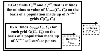
Fig.2 Graphical representation of the NEA
