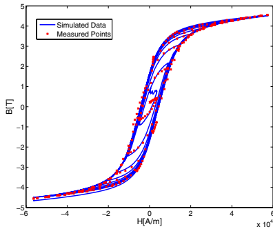
Fig. 6: Simulation result and measurement data of concentric loops
