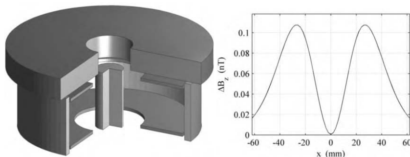
Fig. 9 Optimized eddy current transducer and calculated changes in magnetic flux density for f_{\text{opt}} = 45 Hz
