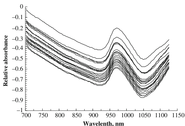
Fig. 6.28 Original spectra of tomato juice
