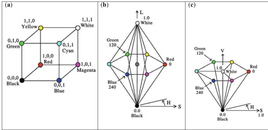
Fig. 3.12 Different color spaces used in representing color images. (a) RGB, red-green-blue; (b) HLS, hue-lightness-saturation; and (c) HSV, hue-saturation-value
