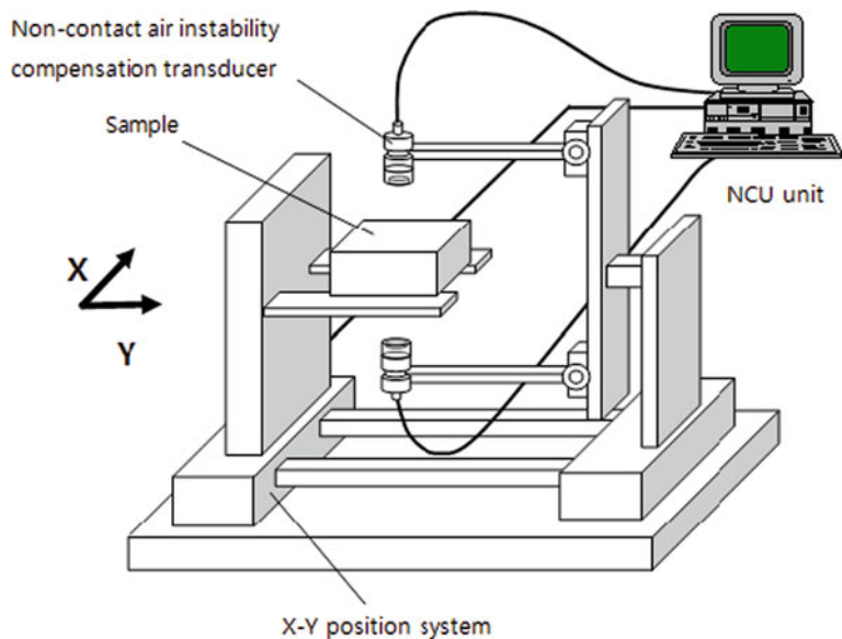
Fig. 7.7 Schematic of the non-contact ultrasonic imaging system (Cho and Irudayaraj 2003b)
