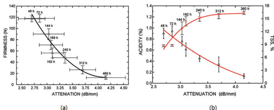
Fig. 7.18 Relationship between ultrasonic attenuation coefficient and (a) firmness, (b) sugar contents (○) and acidity (Δ) of mango fruits (Mizrach et al. 1997)
