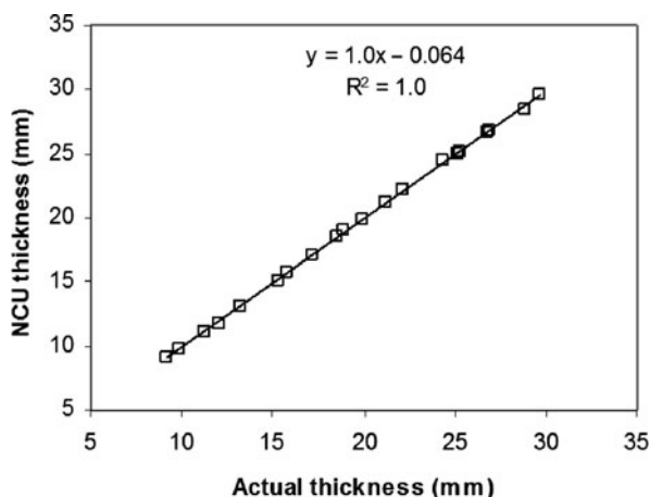
Fig. 7.14 NCU thickness measurement for cheese blocks (Cho and Irudayaraj 2003a)
