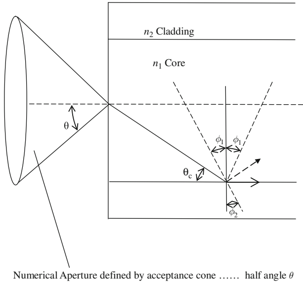
Fig. 6.19 Schematic structure of fibre showing light rays
