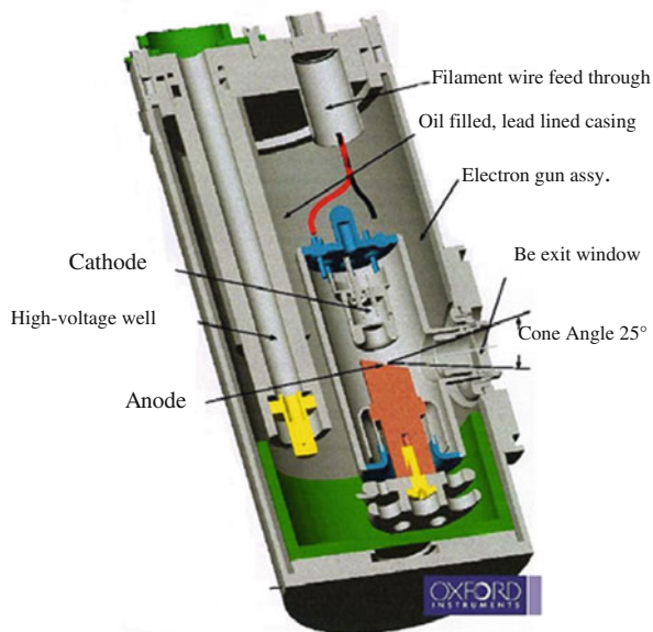
Fig. 5.4 Cut-away view of the X-ray tube (Courtesy: Oxford Instruments, USA)
