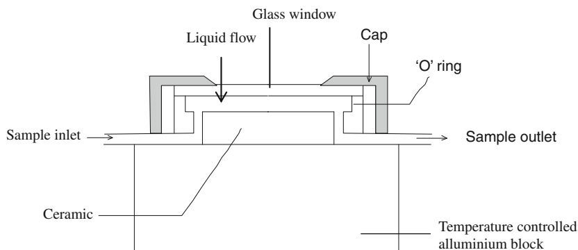
Fig. 6.21 Flowing liquid samples for acquiring transmittance data
