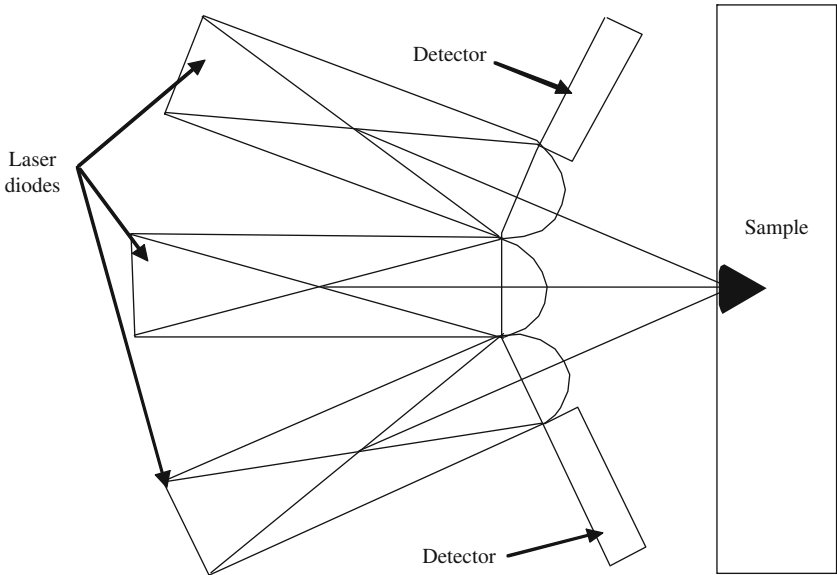
Fig. 6.9 Schematic diagram of a laser-diode arrays spectrometer for making reflection measurements
