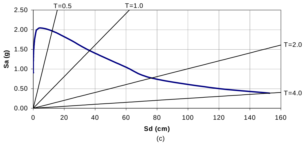
Fig. 4-1: Site-specific design response spectrum for a building near San Francisco, California, 975 year return period, 5% damping. (a) Acceleration versus period, (b) displacement versus period, (c) acceleration versus displacement
