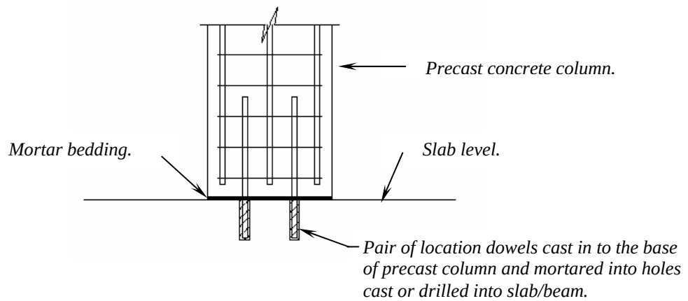
Fig. 7-3: Typical dowel located precast concrete column base detail
