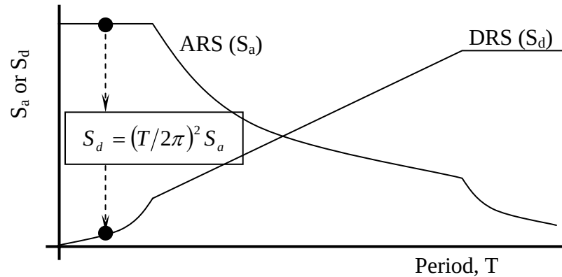
Fig. A-3: Conversion from ARS to DRS
