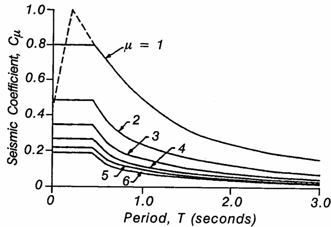
Fig. 4-16: Basic seismic hazard coefficient, for intermediate soil sites, for different displacement ductility capacities, \mu , used in New Zealand [Standards New Zealand 1992]
