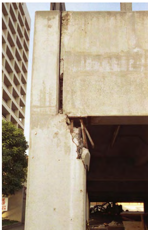
Fig. 2-17: Brittle failure of beam-column pin connection at top of corner column (1994 Northridge earthquake)
