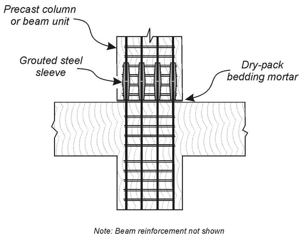
Fig. 5-33: General details of column-to-column connection through grouted steel sleeves
