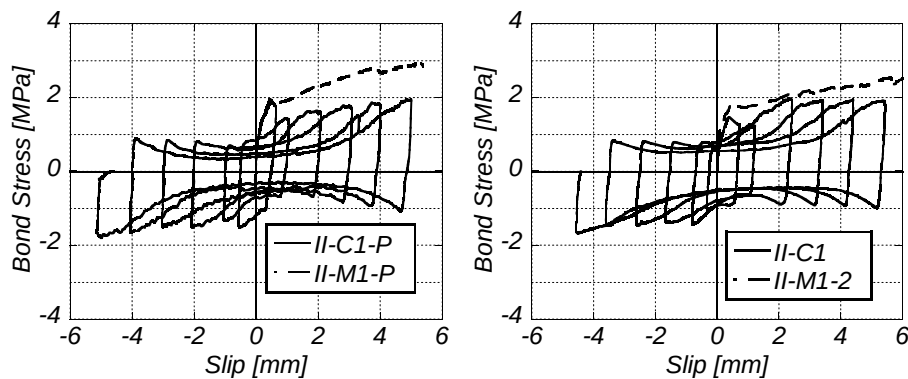
Fig. A-8: Bond behaviour of prestressing strand under cyclic loading
