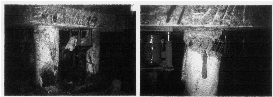
Fig. 8-5: Damage of pretensioned spun concrete piles in 1995 Kobe earthquake
