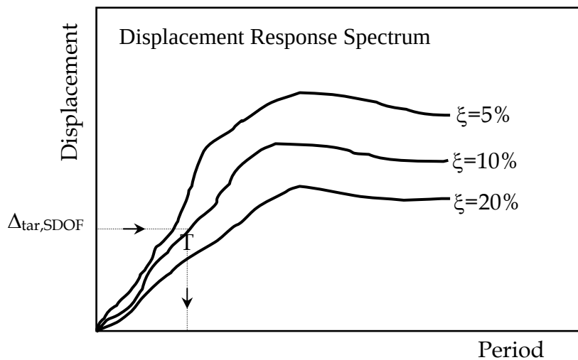
Fig. A-1: Use of DRS to find period corresponding to a target displacement
