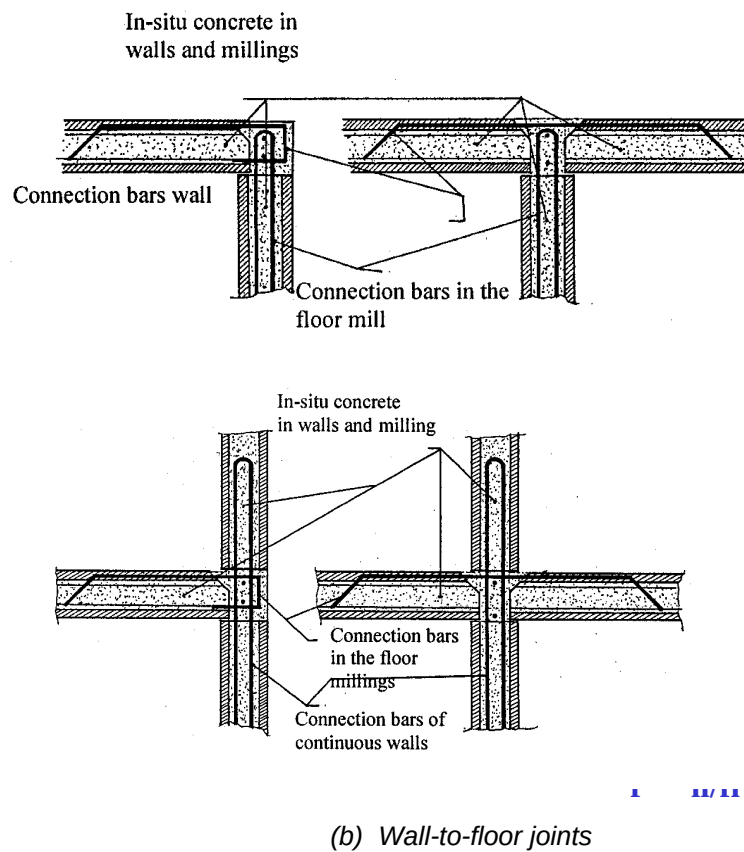
Fig. 5-46: Typical connection details in large panel construction (Courtesy of M. Menegotto)
