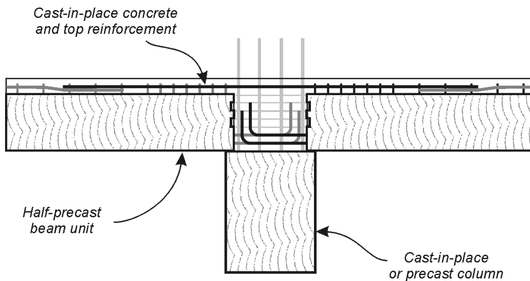
(a) Approach using hooked bar anchorages
