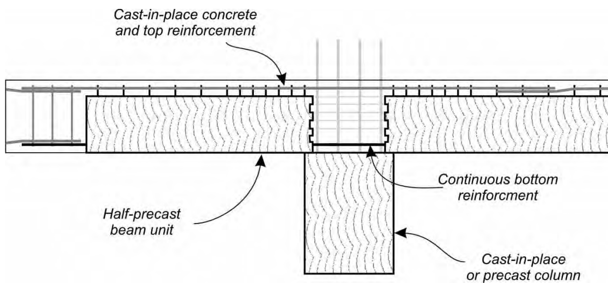
(b) Approach using straight bottom beam bars
