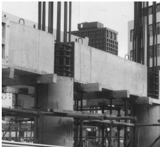
(c) Example from New Zealand (Courtesy of R. Park)
