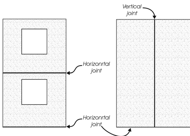
Fig. 5-38: Examples of wall partitioning
