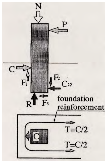
Fig. 8-2: Actions in the socket [Osana et al. 1996]
