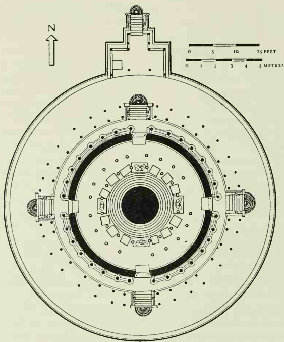
Figure 36. Wata-da-ge, Poḷonnāruwa: Ground plan
