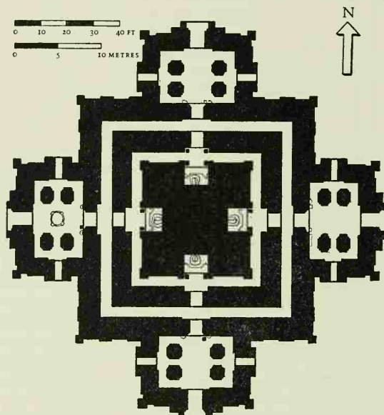
Figure 46. Ānanda Temple, Pagān: Ground plan
