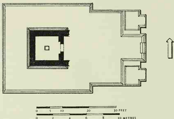
Figure 21. Temple at Bhumara: Ground plan
