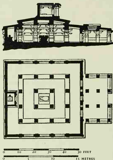
Figure 18. Lādh Khān Temple, Aihole: Plan and Section
