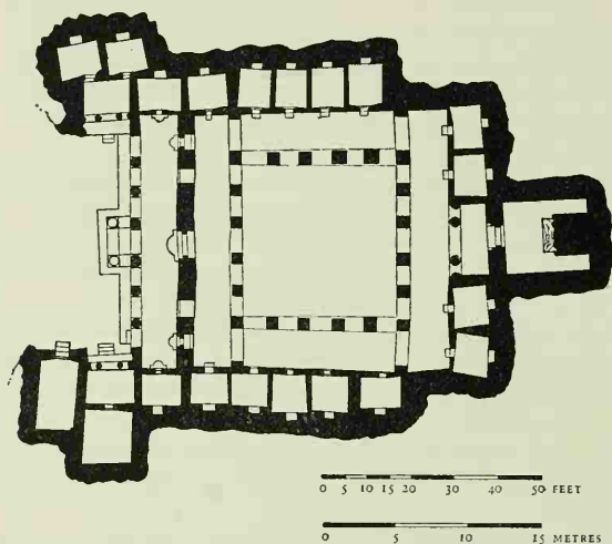
Figure 22. Cave I, Ajaṇṭā: Ground plan
