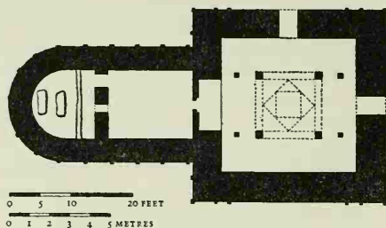
Figure 16. Trivikrama Temple at Ter: Ground plan
