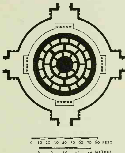
Figure 15. Stupa at Nāgārjunakoṇḍa: Ground plan
