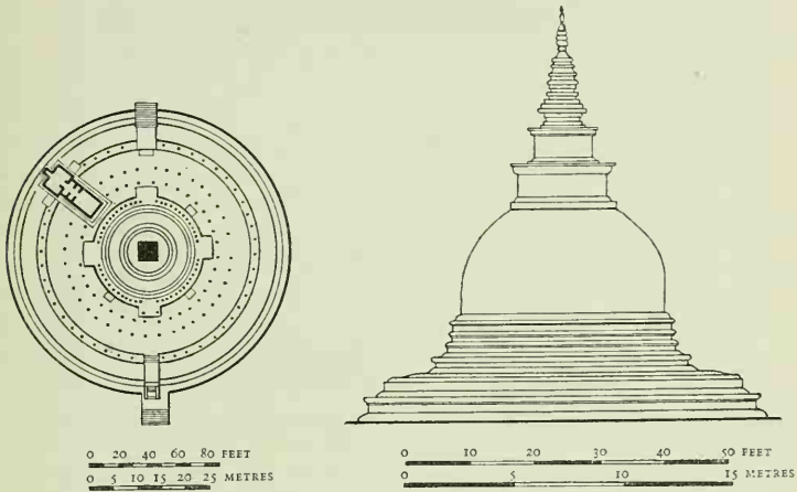
Figure 32. Thūpārāma, Anurādhapura: Ground plan and Elevation
