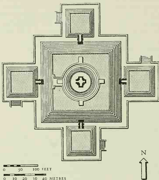
Figure 45. Néak Péan, Angkor Thom: Plan
