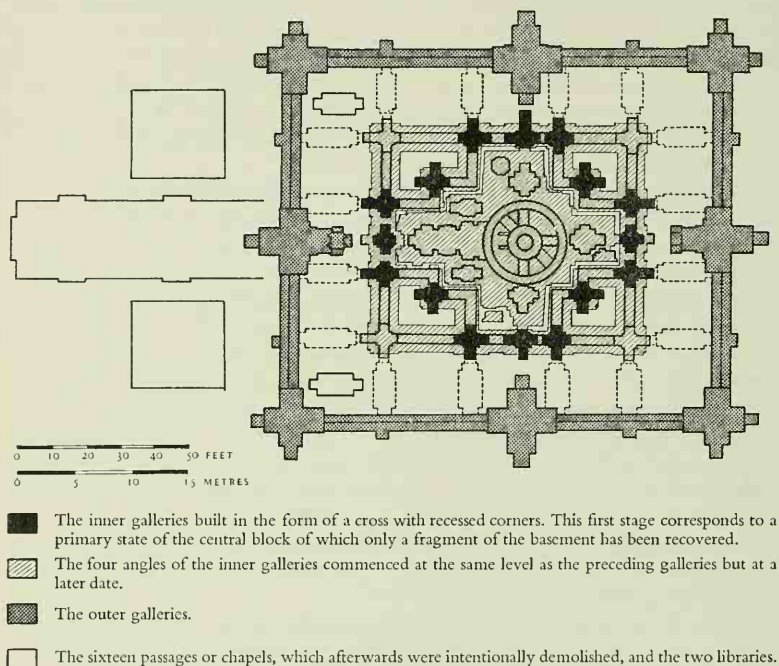
Figure 43. The Bayon, Angkor Thom: Plan
