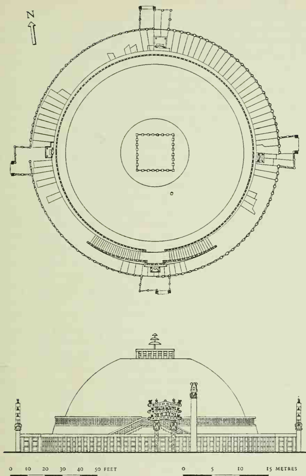
Figure 4. Great Stupa, Sāñchī: Plan and Elevation
