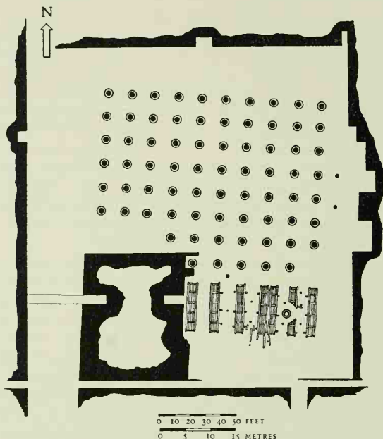
Figure 2. Maurya Palace, Pāṭaliputra: Plan
