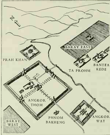
Figure 44. Angkor Thom: Plan
