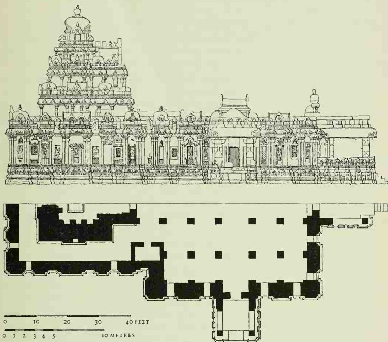
Figure 25. Virūpāksha Temple, Paṭṭadakal: Half-plan and Section
