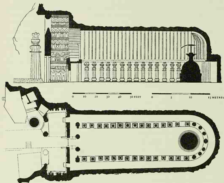
Figure 7. Chaitya-hall at Kārli: Plan and Elevation
