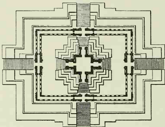
Figure 40. Phiméanakas, Angkor Thom: Plan
