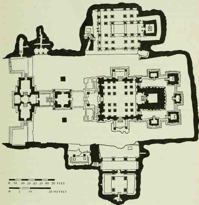
Figure 28. Kailāsanāth Temple, Ellūrā: Plan of Upper Storey
