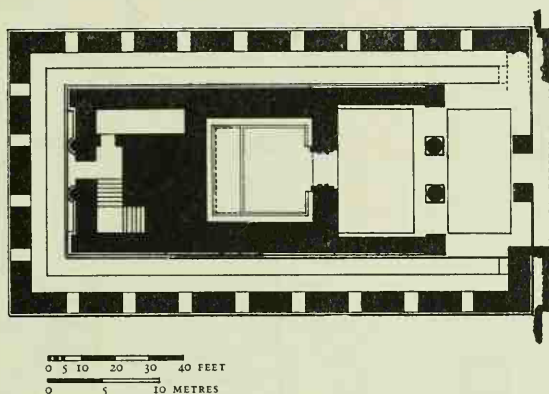
Figure 9. Temple at Jandial, Taxila: Plan
