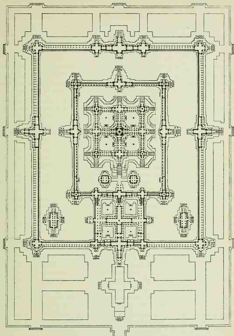
Figure 42. Angkor Wāt: Plan
