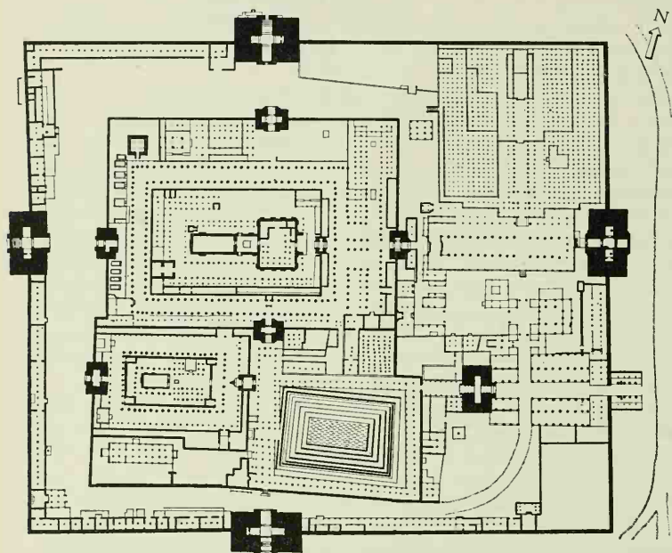
Figure 30. Great Temple, Madurai: Ground plan
