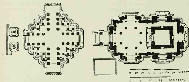
Figure 27. Temple at Modhera: Ground plan
