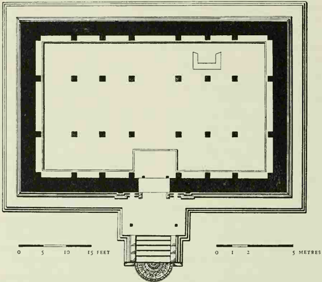
Figure 33. Vihāra near Thūpārāma, Anurādhapura: Ground plan
