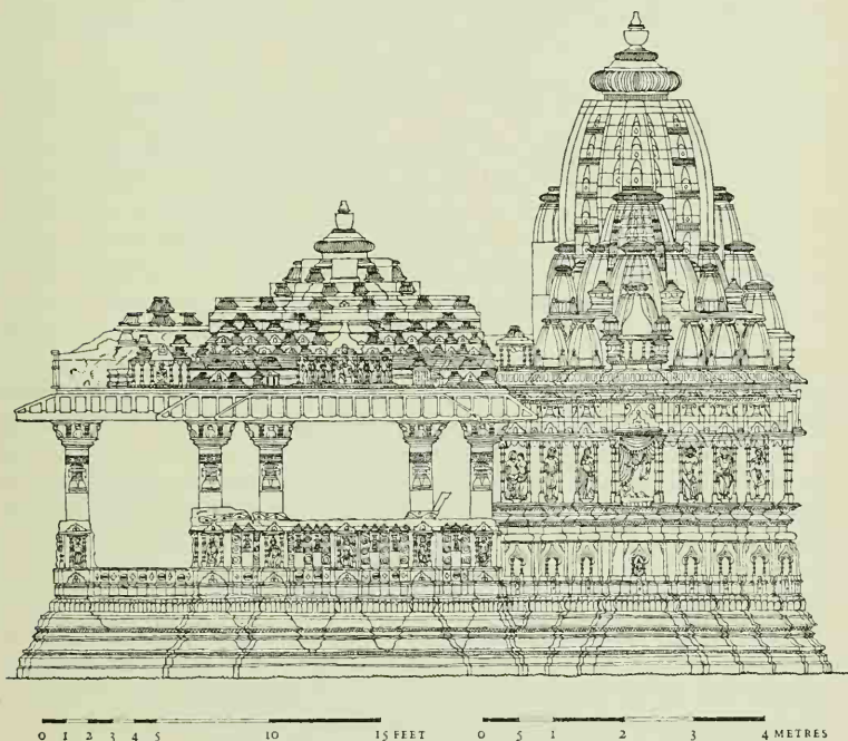
Figure 26. Nilakantha Temple, Sunak: Elevation
