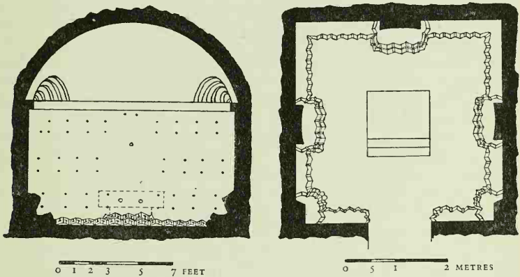
Figure 11. Cave G, Bāmiyān: Plan and Section
