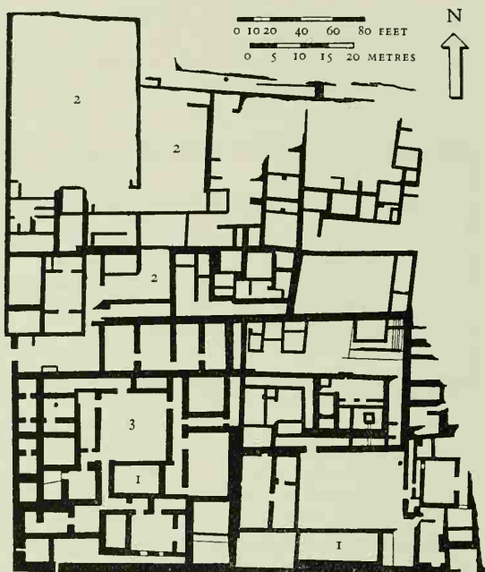
Figure 8. Palace at Sirkap, Taxila: Plan
