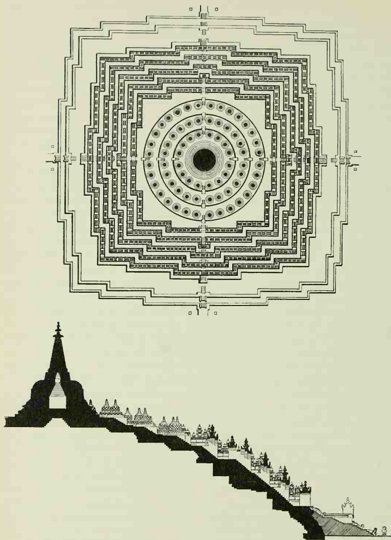
Figure 48. Barabudur: (A) Ground plan and (B) vertical section
