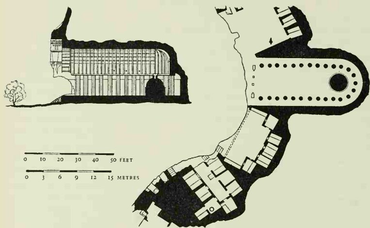
Figure 6. Chaitya-hall and Vihāra at Bhājā: Plan
