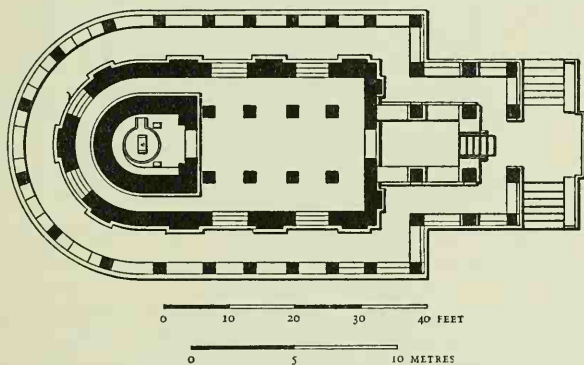
Figure 17. Durgā Temple, Aihole: Ground plan
