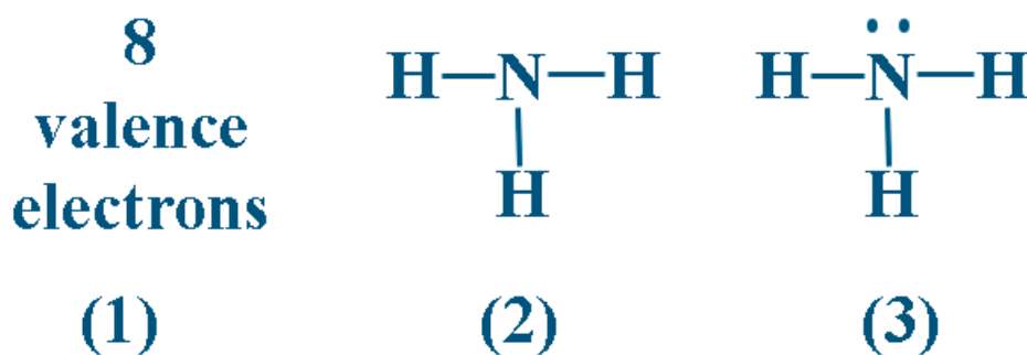
Figure 2- 9: Lewis structure for the ammonia molecule
