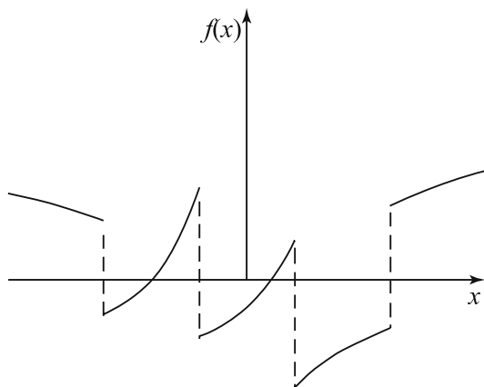
Figure 6.2.1 Graph of a Piecewise Continuous Function.
