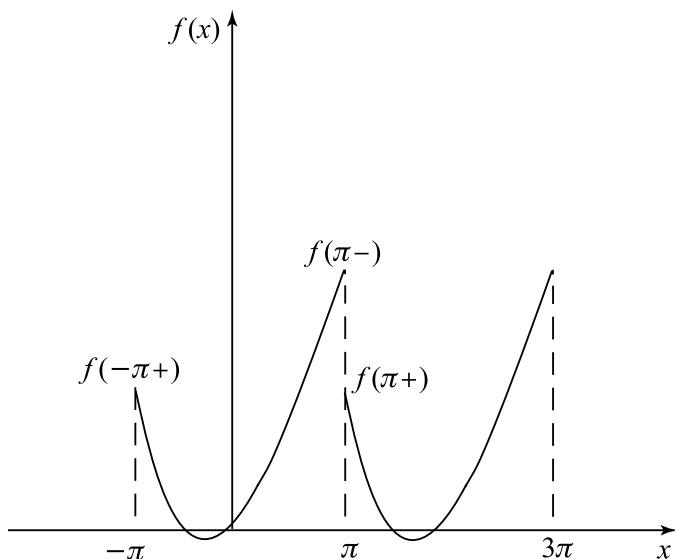
Figure 6.10.2 Graph of f(x) .
