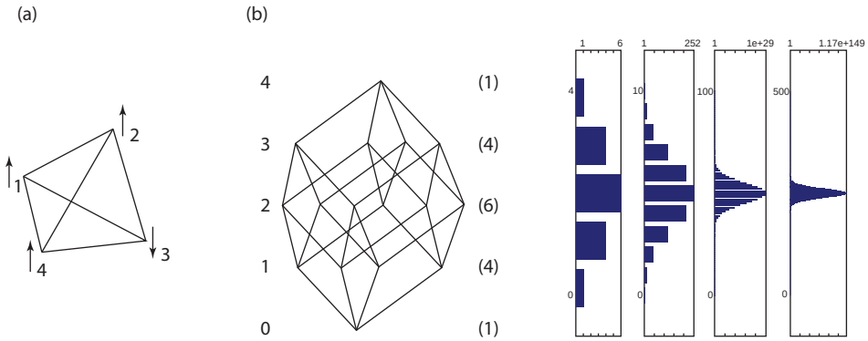
Figure 7.1 (a) The all-to-all coupling of ( N = 4 ) spins that can take values s_i \in \{-1, 1\} , indicated by up or down arrows. Each link between a pair of spins \langle i, j \rangle represents a contribution to the energy of -\epsilon s_i s_j / N . (b) The possible spin configurations for N = 4 make a four-dimensional hypercube. Vertices in the same row have the same number n = |\{i \mid s_i = 1\}| . n is shown on the left beside each row, and the number of vertices at that n , given by the binomial coefficient (7.29), is shown on the right in parentheses. Binomial coefficients rapidly become concentrated near the “equator” of the hypercube as N grows large. The third panel shows bar graphs counting the number of vertices at each level n for N \in \{4, 10, 100, 500\} .
