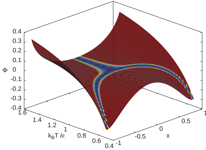
Figure 7.2 The effective potential \Phi of Eq. (7.33). Potential surface shows the change of curvature from attractive toward x = 0 to repulsive as k_B T / \epsilon passes below 1, and the emergence of new minimum values \Phi < 0 , where the cooperative effect in the energy dominates the combinatorial effect in the entropy. Colormap shows the set of x values at each T for which \Phi is within 1/N of its minimum value at that T , as the non-red colors. Only these x make a significant contribution to the partition function (7.32).
