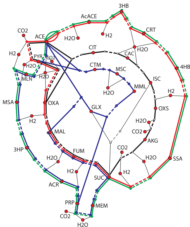
Figure 4.6 Four autocatalytic-loop carbon fixation pathways are contained in the covering graph of Figure 4.5, and pass through some or all of the precursors of anabolism. Color scheme is: rTCA cycle (black); dicarboxylate/4-hydroxybutyrate cycle (red); 3-hydroxypropionate bicycle (blue); 3-hydroxypropionate/4-hydroxybutyrate cycle (green). Acetate (ACE) and succinate (SUC) (both as coenzyme-A thioesters) are intermediates in all four pathways, and define the boundaries on which distinct pathway segments are combined to form different loops. Radially aligned reactions are homologous in local-group chemistry; deviations from strict homology in different pathways appear as excursions from concentric circles. (After [91], Creative Commons [153].)
