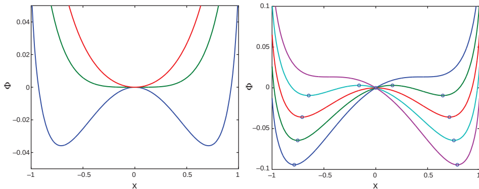
Figure 7.4 The effective potential \Phi(x) interpreted as a large-deviations rate function or joint system/bath entropy as in Eq. (7.41). Left-hand panel: h = 0 and T = \{0.8, 1.0, 1.2\} , showing the transition through the critical point and symmetry breaking. Right-hand panel: T = 0.8 and h = \{-1, -0.5, 0, 0.5, 1\} \times h_c , where h_c \approx 0.06225 is the critical field strength above which \Phi has a single minimum. Positions d\Phi/dx = 0 are marked with circles.
