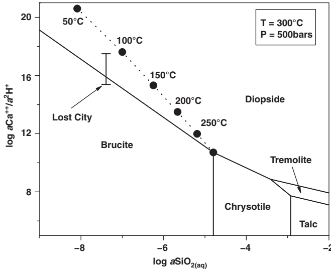
Figure 3.7 A mineral phase coexistence diagram for the \text{MgO-CaO-SiO}_2\text{-HCl-H}_2\text{O} system at 300^\circ\text{C} and 500 bars, after Foustoukos et al. [268]. Upper phases diopside and tremolite are calcic silicates, while lower phases brucite, chrysotile, and talc are non-calcic. Parallel sets of coexistence curves, displaced from the ones drawn, run through the dots at a series of temperatures between 50^\circ\text{C} and 300^\circ\text{C} (labeled). The dashed line affords an idea of the way a\text{Ca}^{2+}/a^2\text{H}^+ would depend on a\text{SiO}_{2(\text{aq})} in a hydrothermal system where temperature also varied with depth due to conductive cooling.
