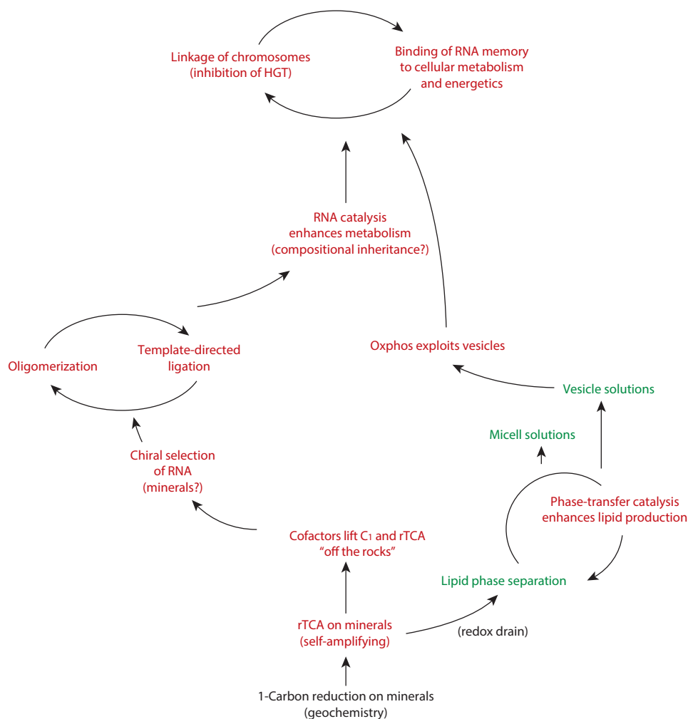
Figure 8.1 The major (phase) transitions in (prebiotic) evolution. Black indicates geochemical processes that are not distinctively biotic, though they may later be displaced by more efficient biotic counterparts. Green indicates formation of equilibrium ordered phases, understood with classical thermodynamics. Red entries are those that inherently incorporate dynamics, and in which the order is principally an order of processes.
