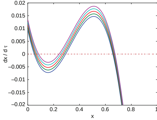
Figure 7.12 The rate equation (7.76) for the (A, X, \emptyset) system with reactions (7.64) with constitutive parameters x_1 = 0.4 , x_2 = 0.6 . Five values of \epsilon \in \epsilon_{\text{crit}} + [-0.002, 0.002] , where \epsilon_{\text{crit}} \approx 0.01166 is the critical value for detailed balance, are shown. Zero-crossings of the rate dx/d\tau are fixed points. Crossings with negative slope are stable, those with positive slope are unstable.
