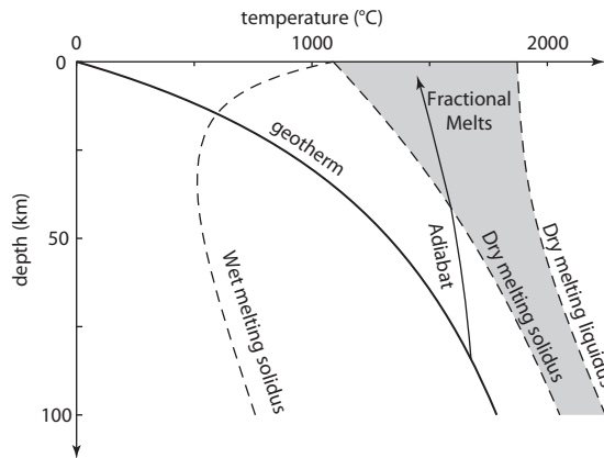
Figure 3.5 Decompression melting along the trajectory of upwelling mantle. The geotherm is the temperature profile of stationary mantle. The dry melting solidus is the curve of first melt separation for pristine mantle peridotites, and the dry melting liquidus is the curve of complete melting. The interval between the two is the freezing range , where a slurry of coexisting liquid and crystalline phases forms, with the liquid fraction increasing to the right. Perfect adiabatic upwelling from a point on the geotherm (thus, not taking into account heat dissipation to the surroundings) would transport mantle material on the adiabatic cooling curve. Where this curve crosses the solidus, decompression melting begins. In an alternative to decompression melting, introduction of hydrated minerals into the assemblage, which occurs in subduction zones, can produce a wet melting solidus with temperatures well below those of the geotherm, leading to forms of melt separation below island arcs and continental margins. (Material adapted from [555] and [669].)
