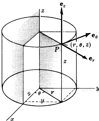
Fig. 22-12. Cylindrical coordinates.
