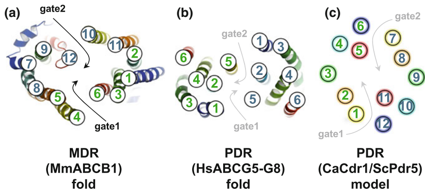
Fig. 18.5 Fungal PDR transporters are predicted to fold like HsABCG5-G8. The TMD folds for MmABC1 (a) and HsABCG5-G8 (b) are the same as shown in Fig. 18.2b, c. This figure shows how MDR transporters (a) have TMS4, -5, -6 and TMS10, -11, -12 lining the substrate-binding pocket, whereas the PDR transporter homolog HsABCG5-G8 (b) has TMS1, -2, and -5 of ABCG5 (left half) and ABCG8 (right half) lining the substrate-binding pocket. Annotations are the same as in Fig. 18.2c. The predicted TMS topology for Cdr1 and Pdr5 (Lamping et al. 2014) (c). This topology model was created by careful consideration of all published and unpublished data relating to the structure and function of Cdr1 and Pdr5. The colours of TMSs: red, orange, yellow, green, turquoise and blue indicate homologous N- (lighter colours) and C-terminal (darker colours) TMS pairs from the most to the least ‘important’ (i.e. the most important TMSs had the most number of residues affecting Cdr1/Pdr5 ATPase activity and/or drug efflux; also see Fig. 18.4a). Proposed (a) and possible gates (b; c) where pump substrates may enter the transporter from the inner leaflet of the lipid bilayer are indicated with black (a) and grey (b; c) arrows. Note how the predicted PDR TMS topology closely resembles that of ABCG5-G8 (b) but has little semblance to type I exporters (a)
