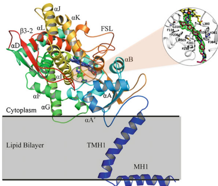
Fig. 22.3 The structure of Erg11p showing bound triazole drugs. The full structure of Erg11p from Saccharomyces cerevisiae is shown with bound substrate in active site with its heme moiety and enlargement of the same region ( inset ) with bound itraconazole per Sagatova et al. (2015)
