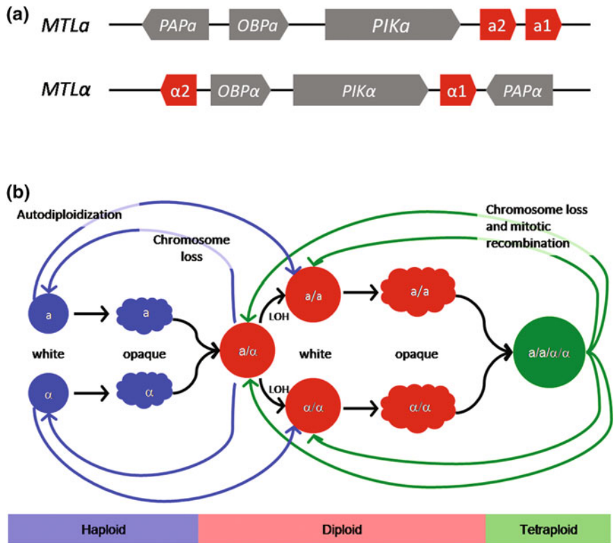
Fig. 11.1 Parisexuality and the haploid, diploid and tetraploid states of Candida albicans . a Schematic representation of the MTLα and MTLα idiotypes. The genes encoding transcription factors responsible for cellular identity are shown in red while the OBP , PAP and PIK genes that are not involved in cellular identity but differ between the two idiotypes are shown in grey. b Schematic representation of the haploid-diploid-tetraploid life cycle of C. albicans . C. albicans is predominantly existing in the diploid state with heterozygosity at the MTL locus. Homozygosity at the MTL locus allows white-opaque phenotypic switching and mating. Transition from tetraploidy to diploidy or diploidy to haploidy is independent of meiosis and involves random concerted chromosome loss with the intermediate production of aneuploids. Haploids are shown in blue, diploids in red and tetraploids in green
