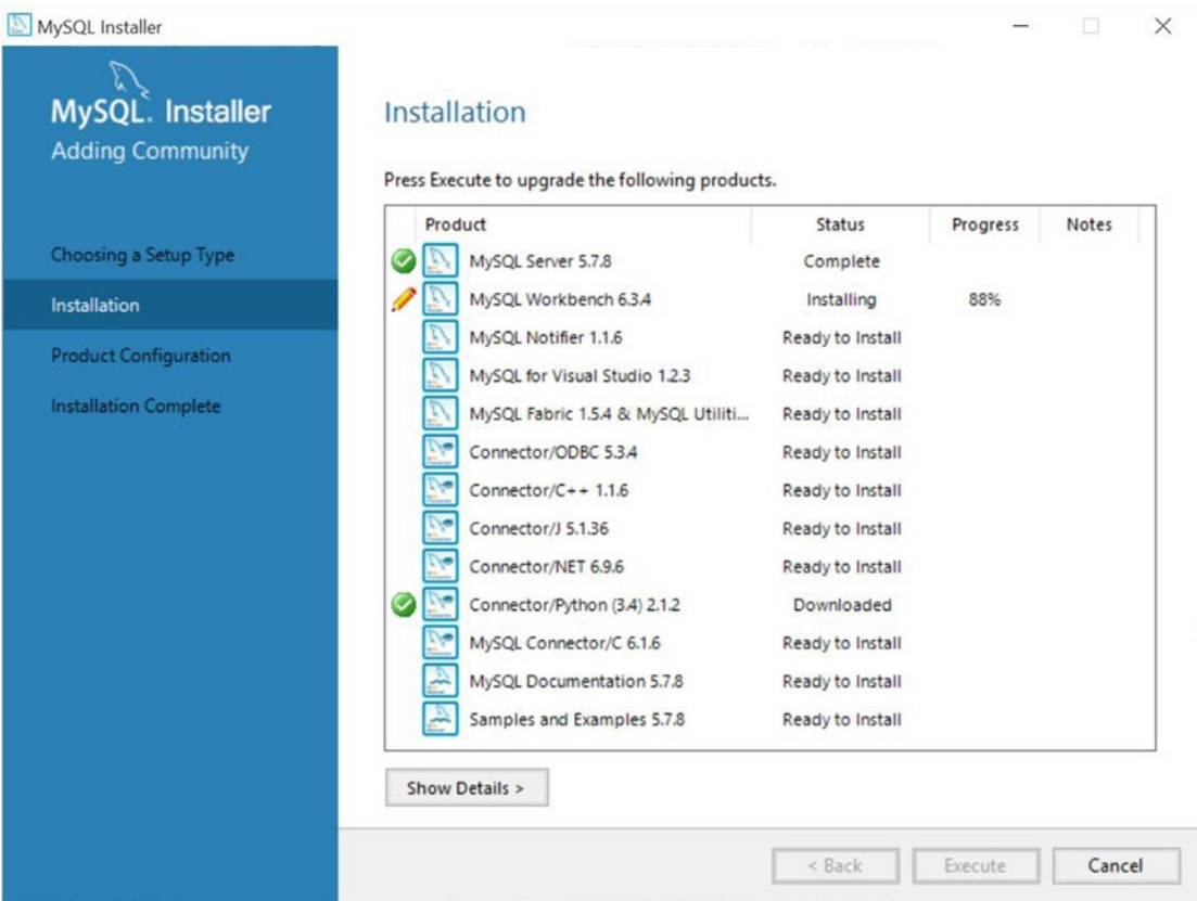
Figure 5-7. Installing packages
