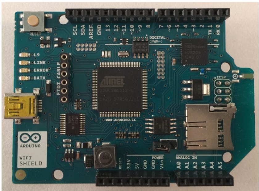
Figure 2-19. Arduino
