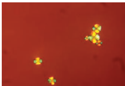
Figure 9.10 Maltese cross-like lipid liquid crystals seen with compensated polarized light. (See page 165.)
