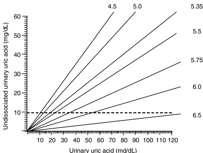
Figure 1 Nomogram used to estimate the concentration of undissociated uric acid ( y axis ) depending on (total) urinary uric acid concentration ( x axis ) and urinary pH. The physicochemical—not necessarily clinical—limit for saturation of uric acid is shown with dotted line.
