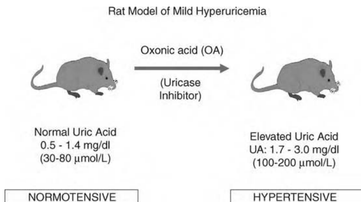
Figure 3 Rat model of mild hyperuricemia associated with hypertension. Sprague-Dawley rats that are fed oxonic acid (a uricase inhibitor) develop mild hyperuricemia and hypertension (57). A characteristic intrarenal vascular lesion develops (afferent arteriolopathy), which is associated with salt sensitive hypertension (5).
