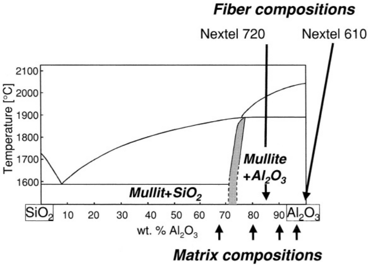
FIGURE 2. The system SiO 2 -Al 2 O 3 (after Klug et al. [12]). Fiber and matrix compositions used for WHIPOX CMCs are indicated by arrows.
