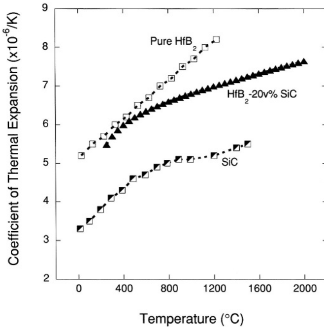
FIGURE 7. Plots of CTE vs. temperature for \text{HfB}_2 , SiC, and \text{HfB}_2 -20v% SiC. 31-32
