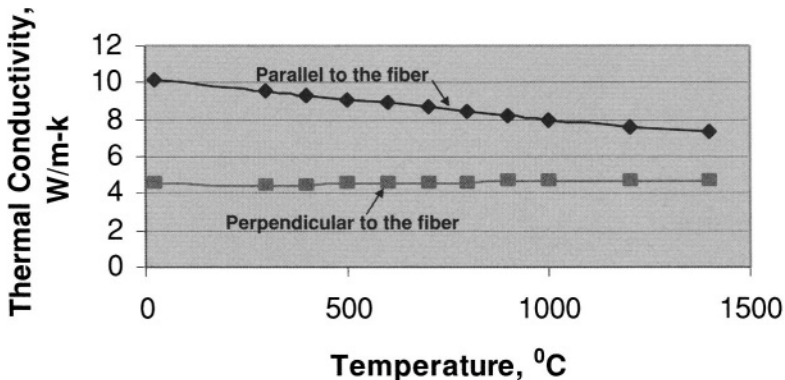
FIGURE 7. Variation of thermal conductivity with temperature for 1-D SiC/RBSN composites containing \sim 24 vol% fibers measured in nitrogen [18, 19].
