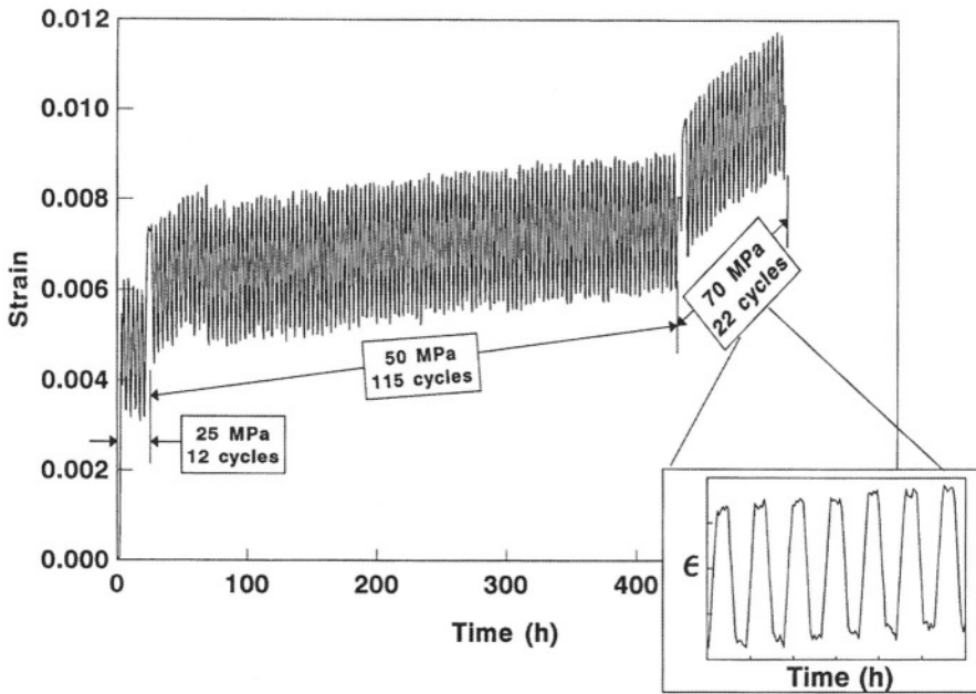
FIGURE 11. Strain versus time plotted for a 2-D Nicalon TM /Al 2 O 3 composite during thermal cycling between 1100 and 600°C in air with a simultaneously applied tensile stress.
