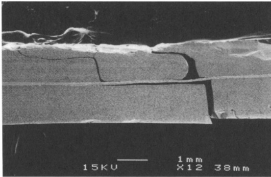
FIGURE 7. SEM micrograph of a bioactive laminate composite fractured in flexure. The tensile side was located at the bottom of the micrograph. The outer layers (tape-cast sintered Bioglass ® ) are bioactive, whereas the middle metallic layer provides ductility [53, 54]. (Micrograph courtesy of Prof. J. J. Mecholsky Jr, University of Florida, USA).
