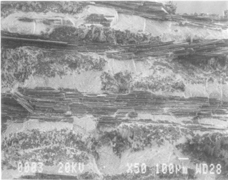
FIGURE 10. Fracture surface of a 2-D Nicalon TM /Al 2 O 3 composite following stress rupture testing at 1100°C in air.
