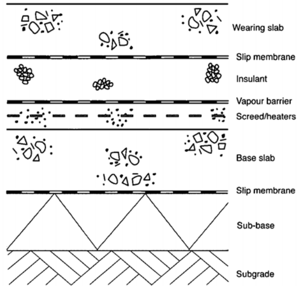
Figure 2.4: Typical construction layers in cold stores.
