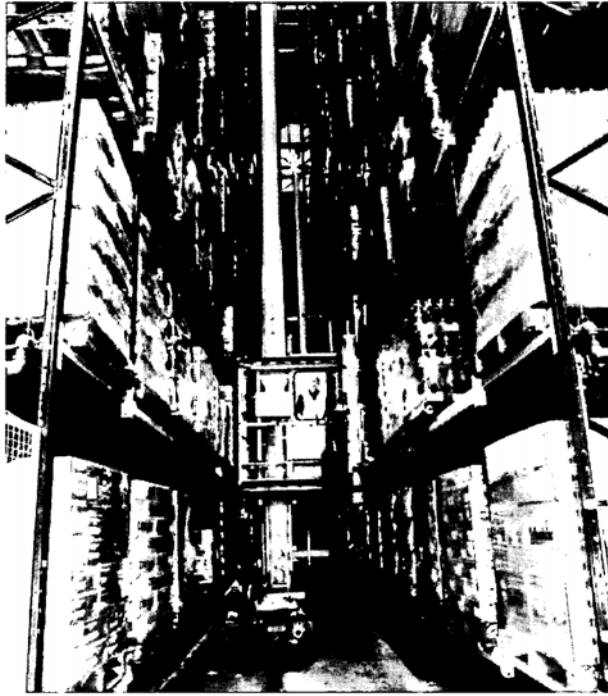
Figure 3.16: Stacker crane, running on a floor-mounted rail.
