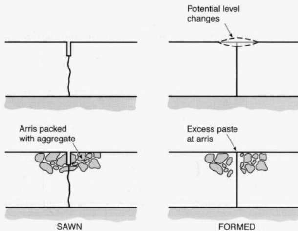
Figure 8.10: Concrete integrity and levels at sawn and formed joints.
