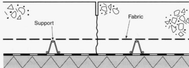
Figure 8.3: Sawn restrained-movement joint (shown with fabric).
