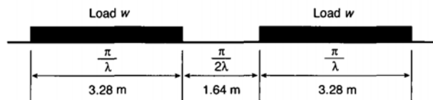
Figure B3: Arrangement of loads for maximum hogging moment.
