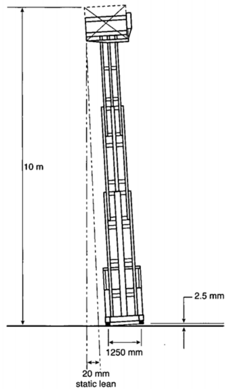
Figure 4.6: Static lean.
