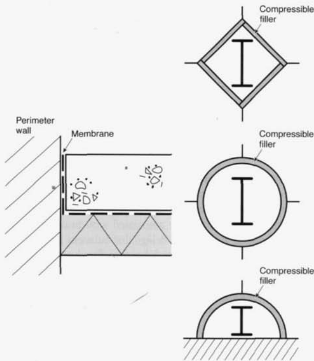
Figure 8.7: Slab isolation details at slab perimeter and columns.
