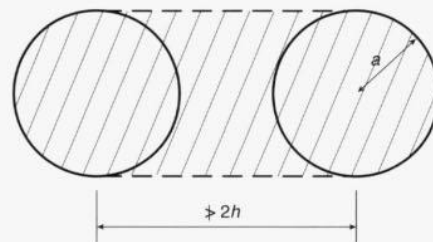
Figure 9.4: Calculation of equivalent contact area for two adjacent point loads.
