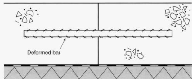
Figure 8.5: Tied joint.
