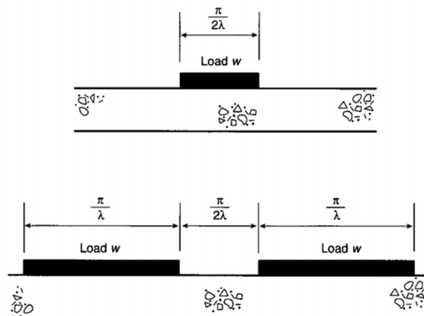
Figure 9.8: Loading patterns for uniformly distributed load, w , causing maximum positive bending moment (upper drawing) and maximum negative bending moment (lower drawing).
