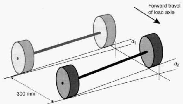
Figure C3: Property B ( = d_2 - d_1 )
