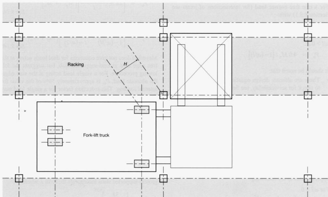
Figure 9.5: Adjacent point loads in very narrow aisles.
