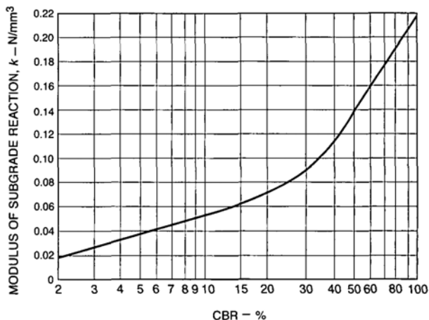
Figure 6.2: Relationship between modulus of subgrade reaction and in situ CBR.
