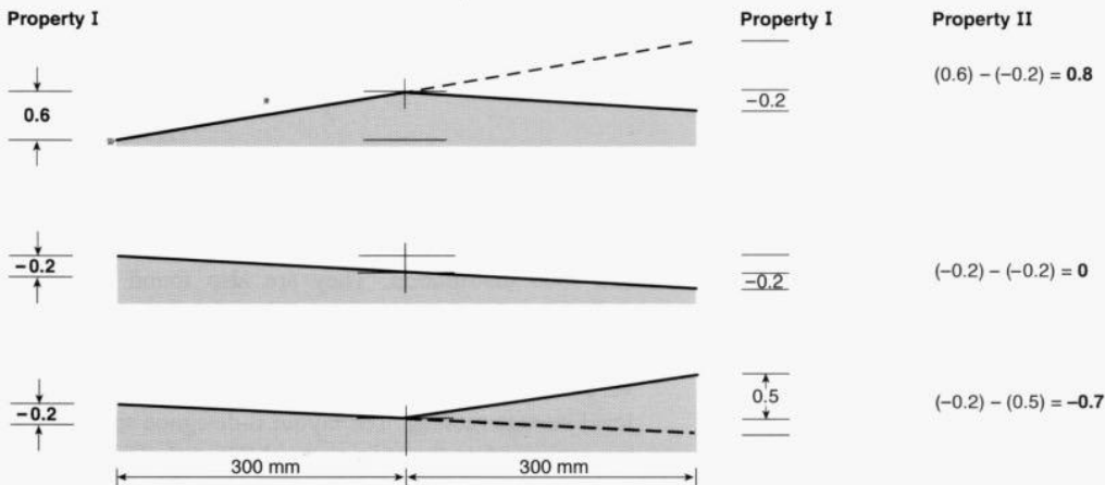
Figure 4.3: Examples of measurements of Property I over 300 mm and the resultant determination of change in elevational difference over a distance of 300 mm (Property II). All dimensions in mm.
