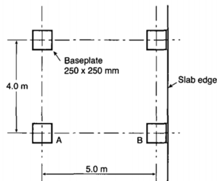
Figure B4: Arrangement of mezzanine baseplate grid.
