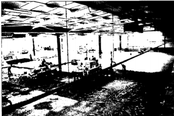
Figure 12.1: A well-laid sub-base is providing a sound platform for construction operations. Fabric is placed just ahead of the laser screed machine so it is not displaced by this mobile plant. The building is almost completely enclosed.
