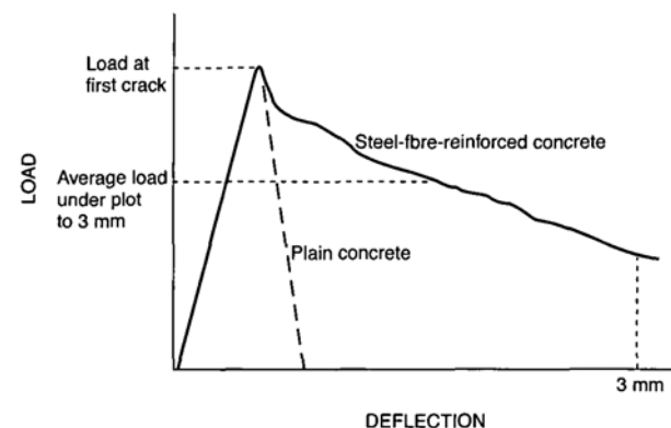
Figure 7.2: Typical load-deflection graph for steel-fibre-reinforced concrete beams.
