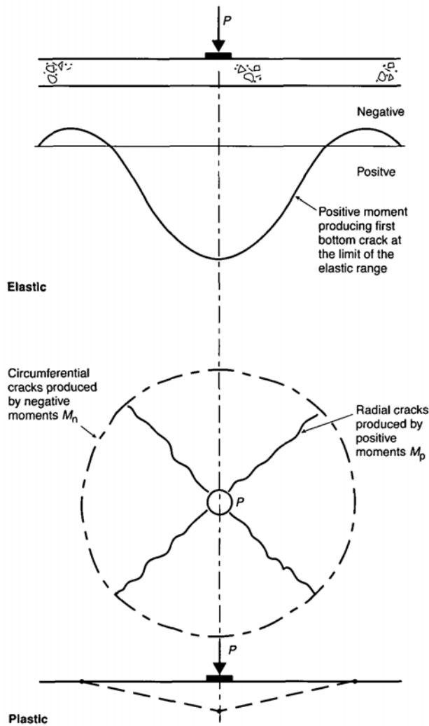
Figure 9.2: Development of radial and circumferential cracks in a concrete ground-supported slab.
