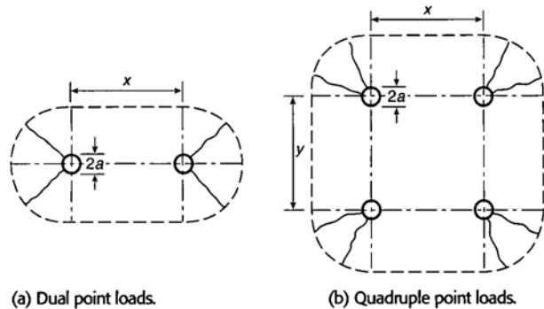
Figure 9.6: Yield line patterns for multiple point loads.
