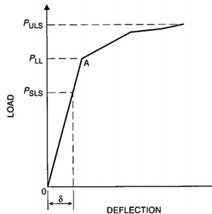
Figure 9.12: Typical load–deflection relationship for steel-fibre-reinforced ground-supported slab.
