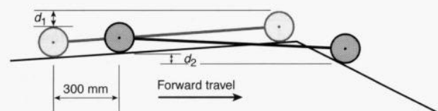
Figure C4: Property D ( = d_2 - d_1 )
