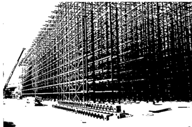
Figure 3.12: Clad rack system.
