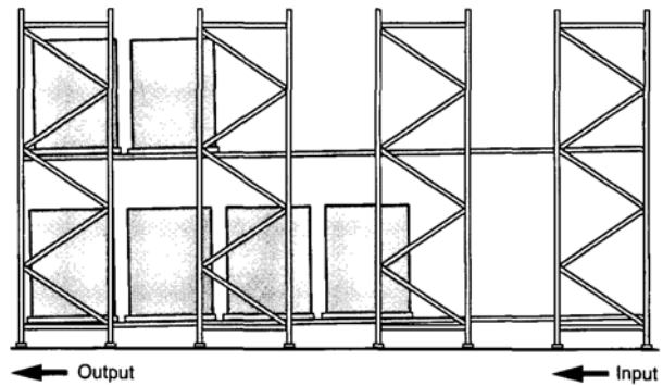
Figure 3.6: Live storage systems.
