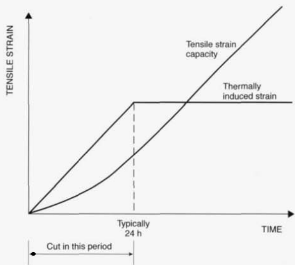
Figure 8.9: Suggested mechanism of crack inducement.
