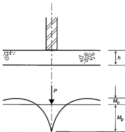
Figure 9.7: Use of Hetenyi's equations for a line load P .
