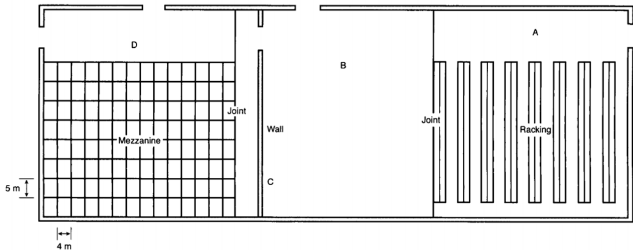
Figure B1: Plan of warehouse (not to scale).
