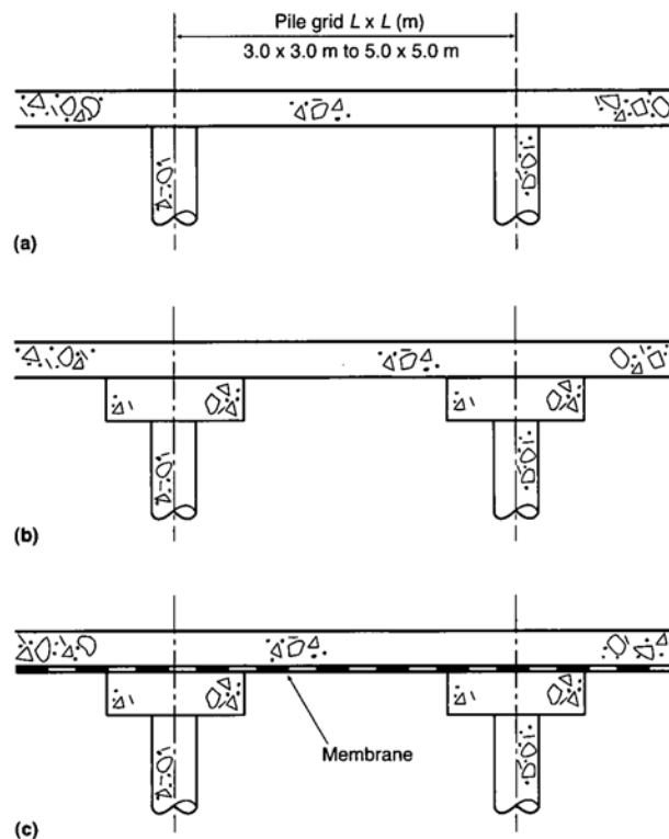
Figure D1: Cross-sections of typical piled slabs (not to scale).
