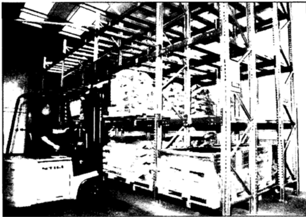
Figure 3.8: Push-back racking.
