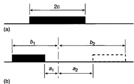
Figure 9.9: Defined areas of uniformly distributed load.
