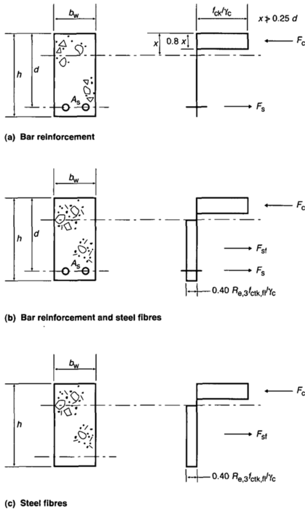
Figure D2: Stress blocks for concrete with steel fibres and/or reinforcement in flexure at the ultimate limit state.
