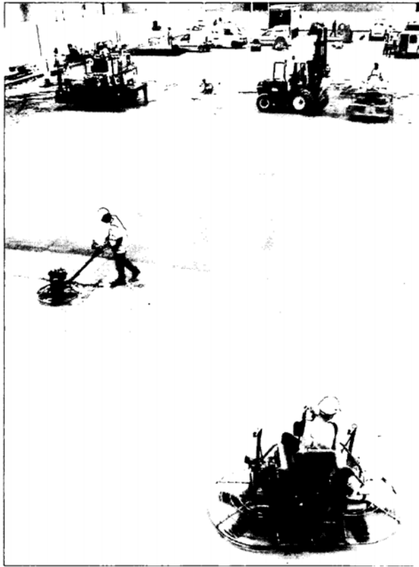
Figure 2.2: Large area construction. In the background (left) a laser screed machine is spreading and levelling the concrete. To the right a dry shake finish is being spread mechanically. In the foreground, the concrete placed several hours earlier is being finished by a power float and a ride-on power trowel.
