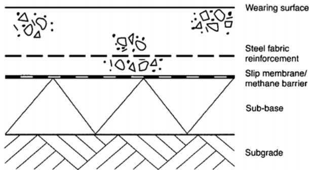
Figure 2.1: Typical slab construction.
