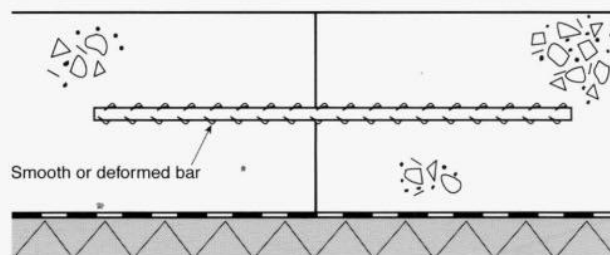
Figure 8.4: Formed restrained-movement joint.
