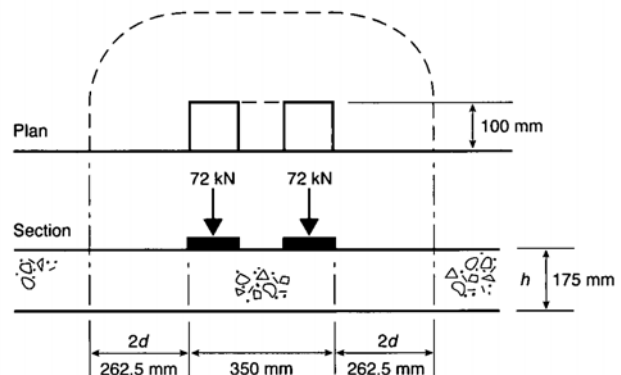
Figure B2: Punching shear perimeter at edge.
