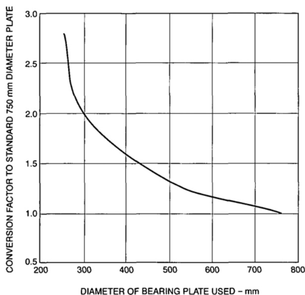
Figure 6.1: Conversion factors for different loading plate sizes.
