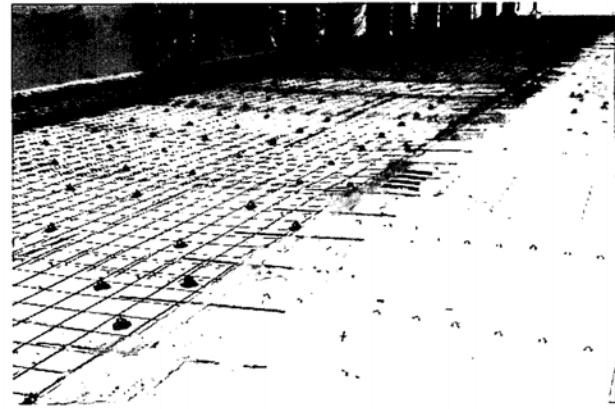
Figure 8.11: Permanent formwork, with dowel bars in place, for a formed restrained-movement joint in a long strip construction. The walls and columns are protected with polythene.
