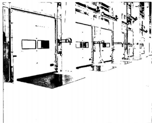
Figure 7.1: Dock levellers. Additional reinforcement may be needed in the areas around each entrance.
