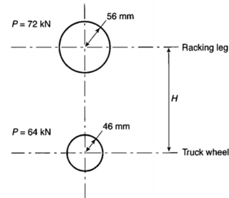
Figure B5: Equivalent loaded areas for racking legs and fork-lift truck wheels.
