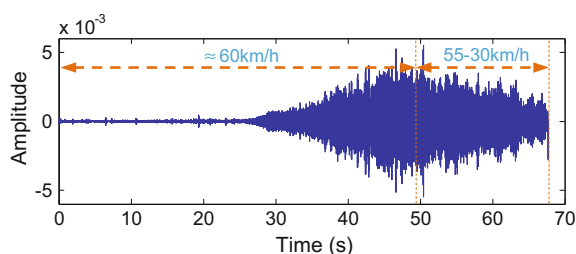
Fig. 3 Narrowband acoustic signal recorded before a metro vehicle passing by the microphone at the 67th second (measured in Shanghai Metro Line 2)
