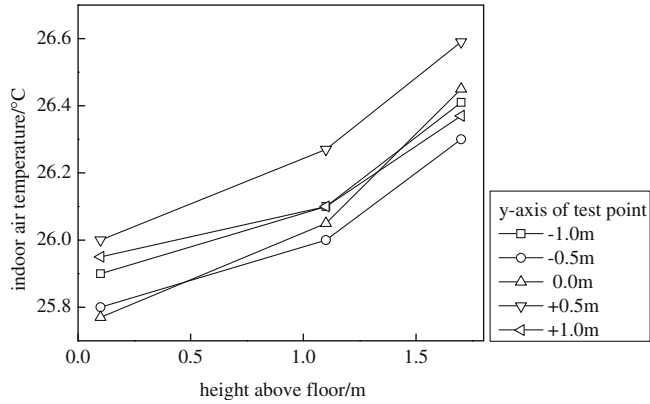
Fig. 6 Indoor air temperature distribution in vertical direction
