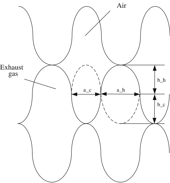
Fig. 2 Diagram of elliptical cross section for PSR
