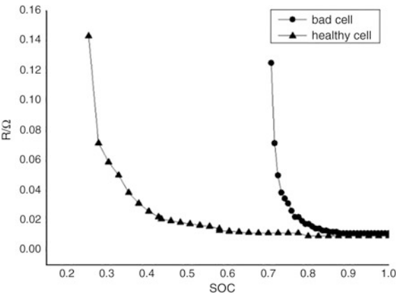
Fig. 5 The internal resistance under different conditions
