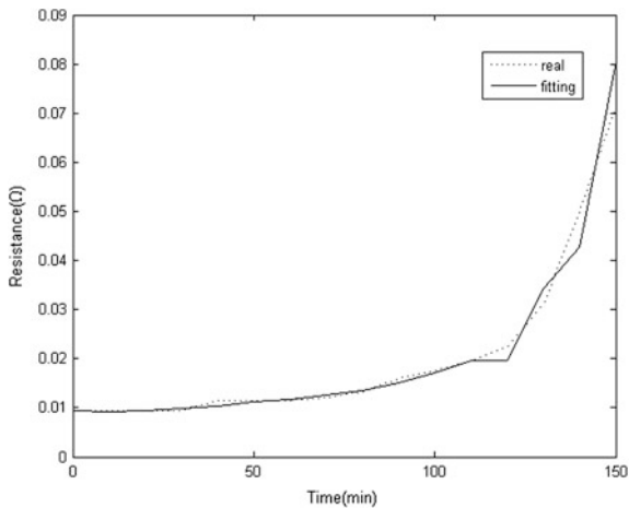
Fig. 9 Identification result of internal resistance
