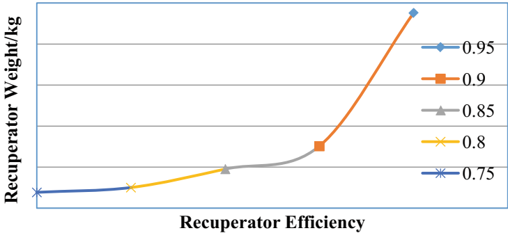
Fig. 3 Weight of the recuperator changes with the efficiency
