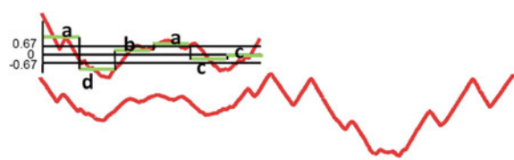
Fig. 2 The SAX word adbacc created from a subsequence of Object1's time series using the sliding window technique
