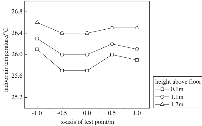
Fig. 5 Indoor air temperature distribution in horizontal direction
