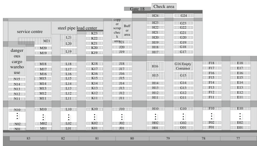
Fig. 2 Qingdao Qianwan container terminal layout
