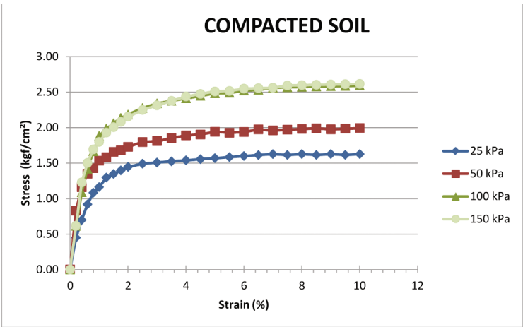
Fig. 12. Stress-strain behavior of compacted soil
