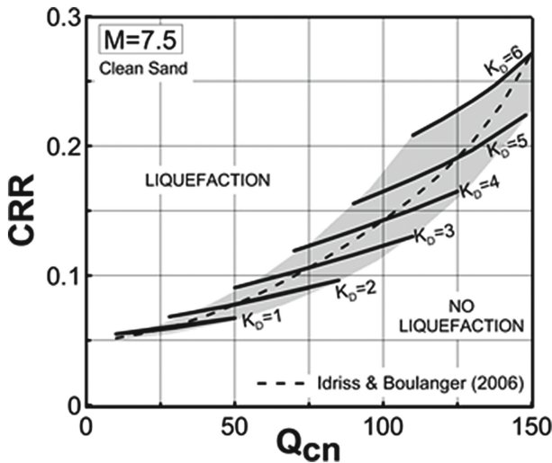
Fig. 11. Chart for estimating CRR in clean sand based on Q_{cn} & K_D (Marchetti 2016)
