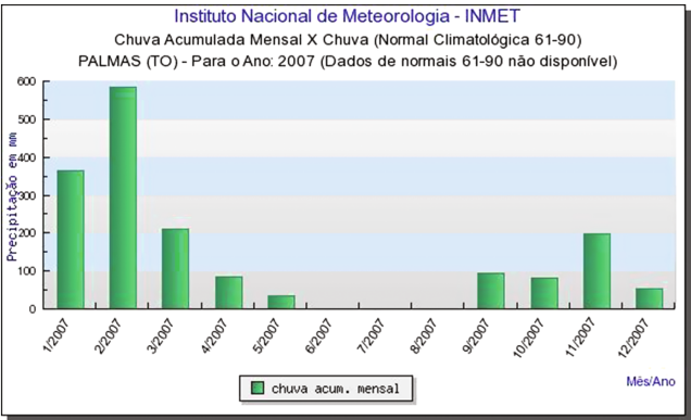
Fig. 24. Accumulated rainfall of 2007.
