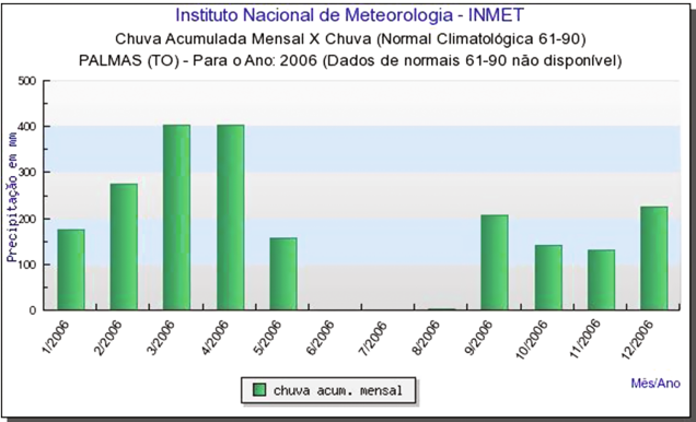
Fig. 23. Accumulated rainfall of 2006.
