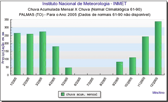
Fig. 22. Accumulated rainfall of 2005.
