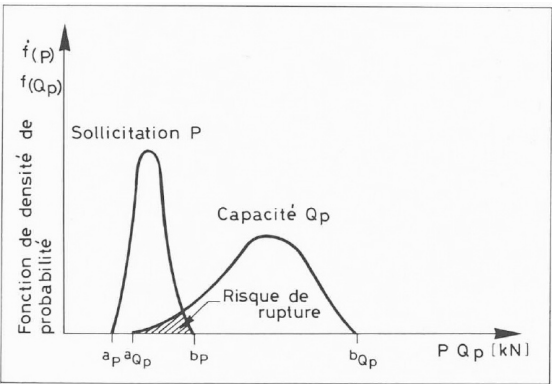
Fig. 10. Capacity-Solicitation model
