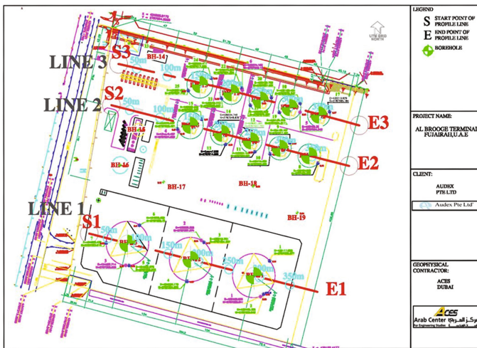
Fig. 23. Layout of 3 MASW lines covering all tanks locations
