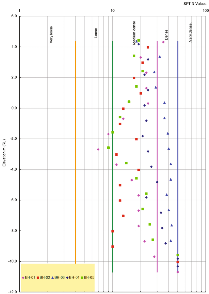
Fig. 7. SPT vs. Elevation – Duqm site
