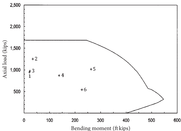
FIGURE 8.8 Design strength interaction diagram about the minor axis of the column given in Example 8.4.
