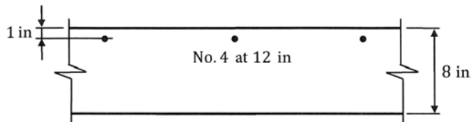
FIGURE 5.12 The one-way slab of Example 5.2.
