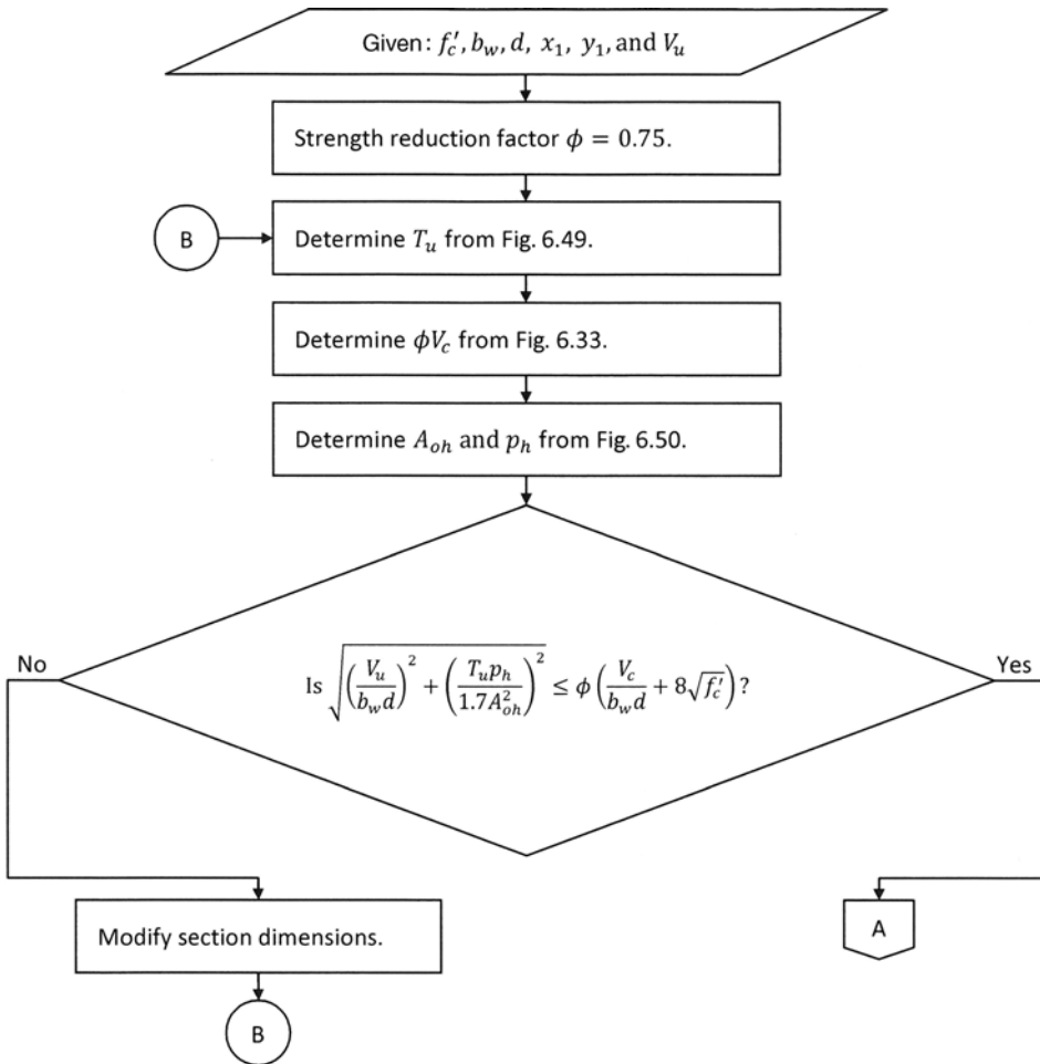
FIGURE 6.51 Transverse and longitudinal reinforcements for torsion. (continued)
