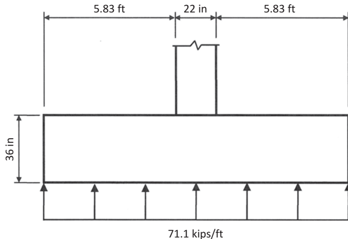
FIGURE 10.31 Bending moment in the transverse direction at the interior column of Example 10.9.
