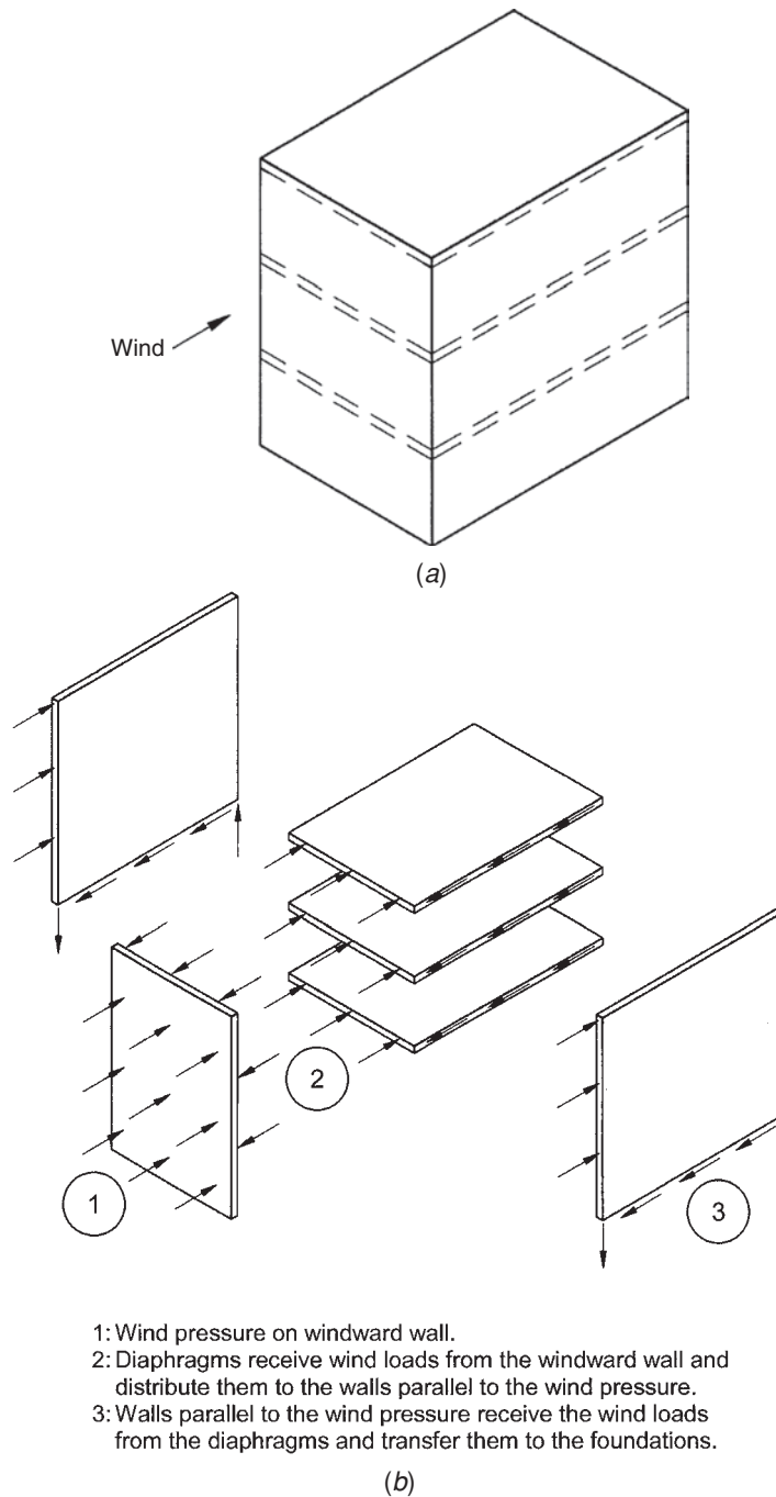
FIGURE 3.10 The propagation of wind forces in a concrete building: (a) wind load on overall building and (b) distribution of wind load to elements of the MWFRS.
