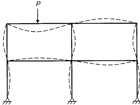
FIGURE 3.12 Vertical load propagation in a reinforced concrete frame.
