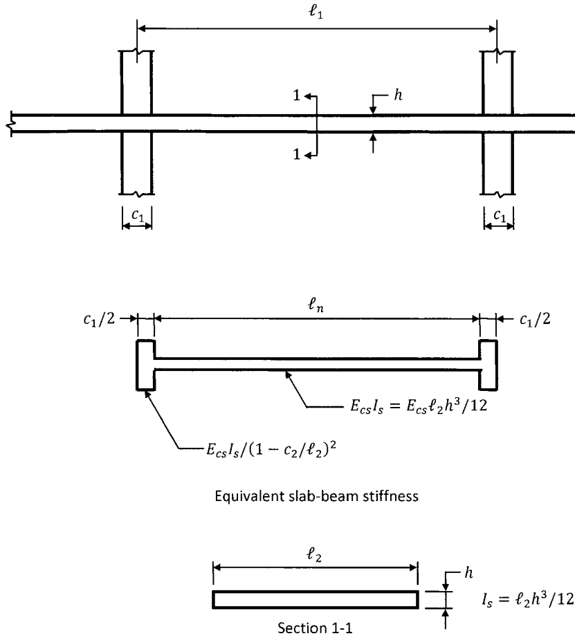
FIGURE 7.26 Slab-beam stiffness in a flat plate.
