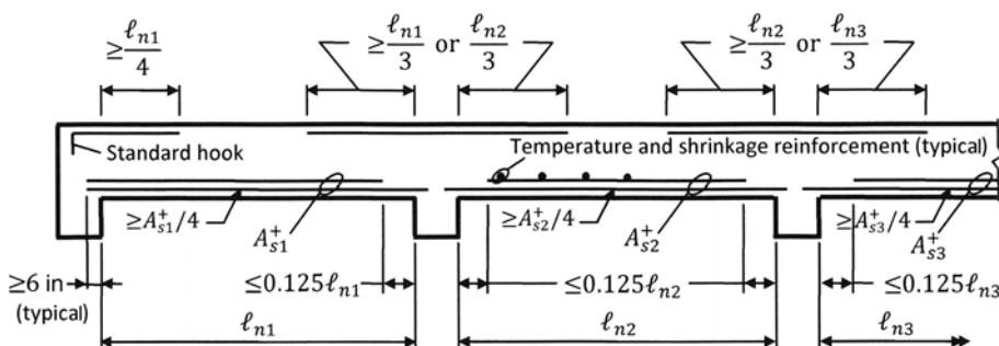
FIGURE 6.26 Recommended flexural reinforcement details for one-way slabs.
