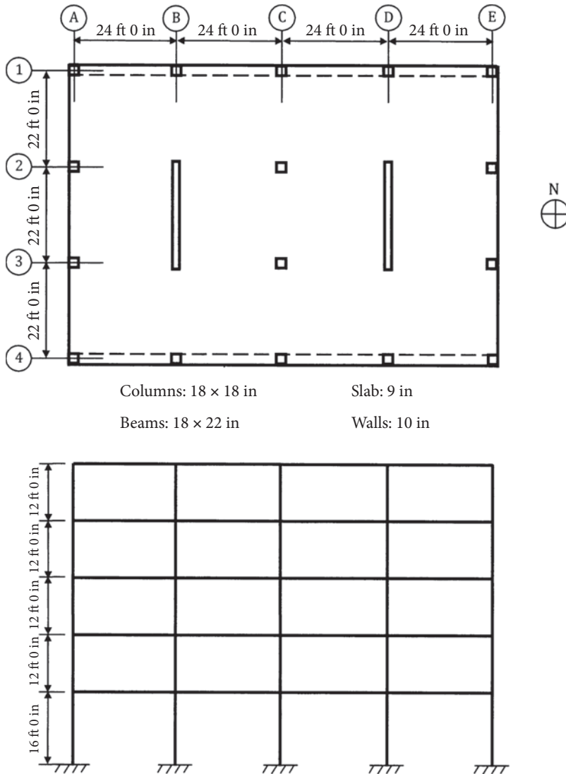
FIGURE 8.18 The typical floor plan of building given in Example 8.7.
