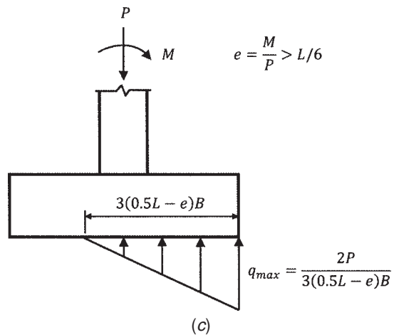
FIGURE 10.12 Soil pressure distribution for footing subjected to axial load and bending moment: (a) e < L/6 , (b) e = L/6 , and (c) e > L/6 .
