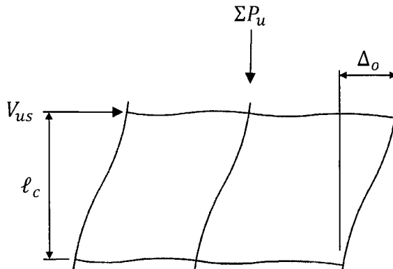
FIGURE 8.13 Definition of stability index Q .
