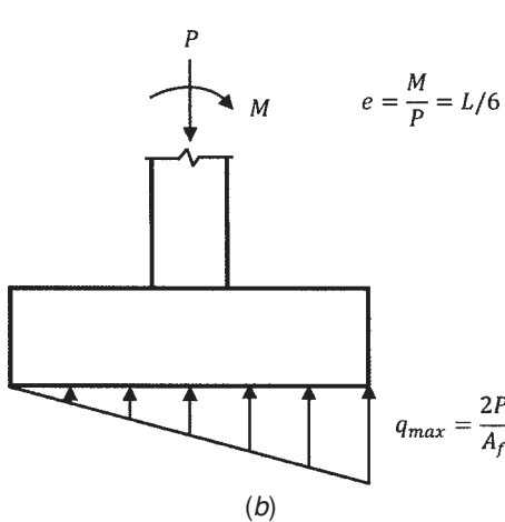
FIGURE 10.12 Soil pressure distribution for footing subjected to axial load and bending moment: (a) e < L/6 , (b) e = L/6 , and (c) e > L/6 .
