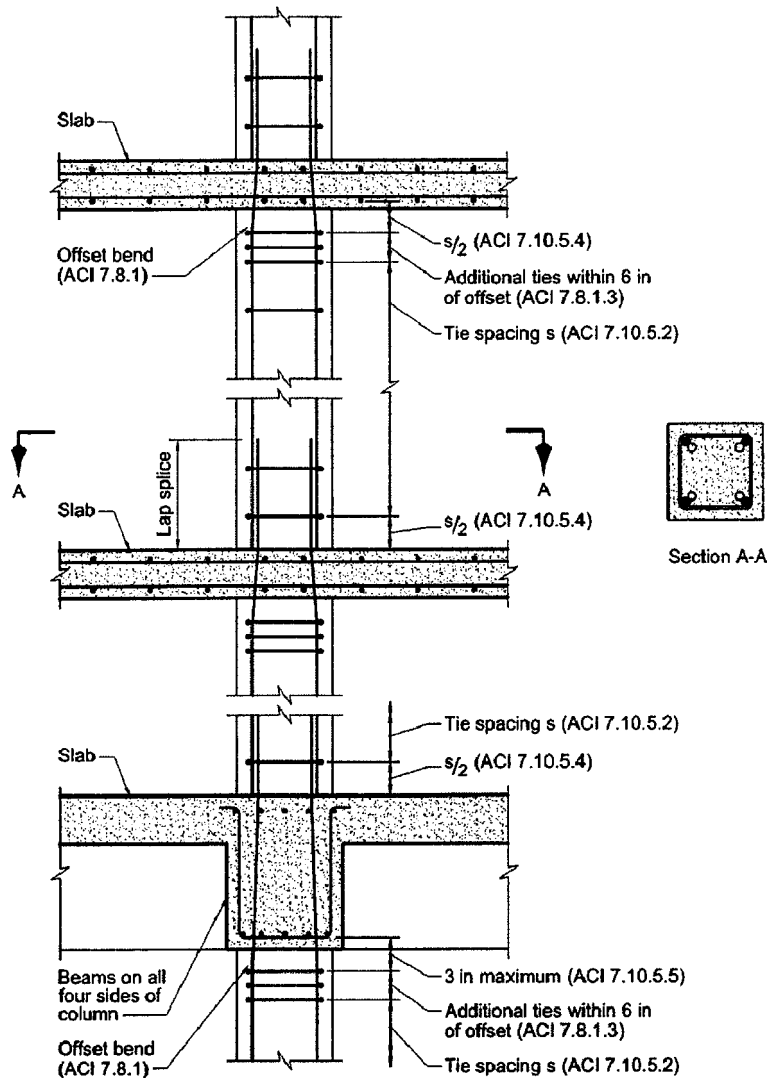
FIGURE 8.29 Tie and splice details.
