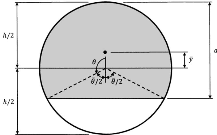
FIGURE 8.10 Circular column where the depth of the compression zone a is greater than h/2 .
