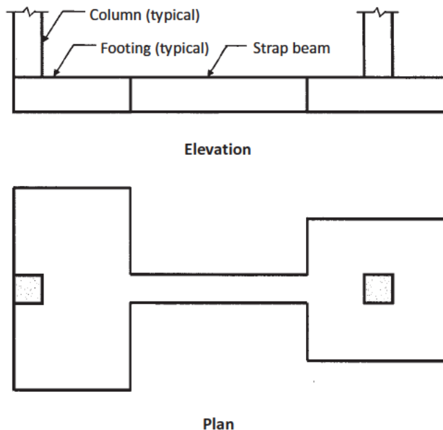
FIGURE 10.3 Strap footings.
