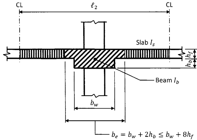
Interior beam
