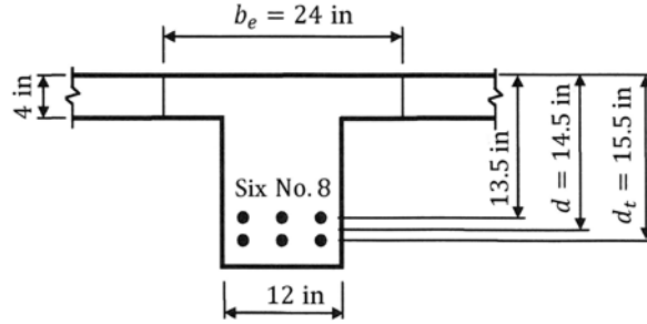
FIGURE 5.33 The T-beam of Example 5.8.
