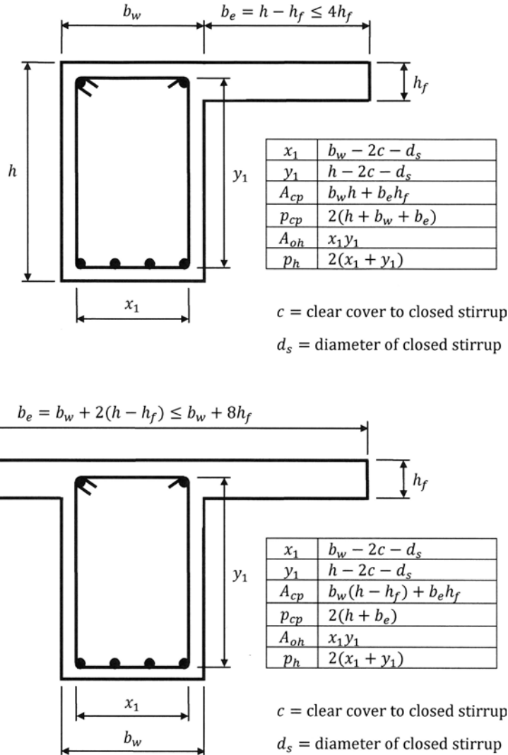
FIGURE 6.50 Torsional section properties.
