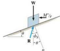
Downward screw motion ( \theta < \phi_s )
