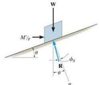
Downward screw motion ( \theta > \phi_s )
