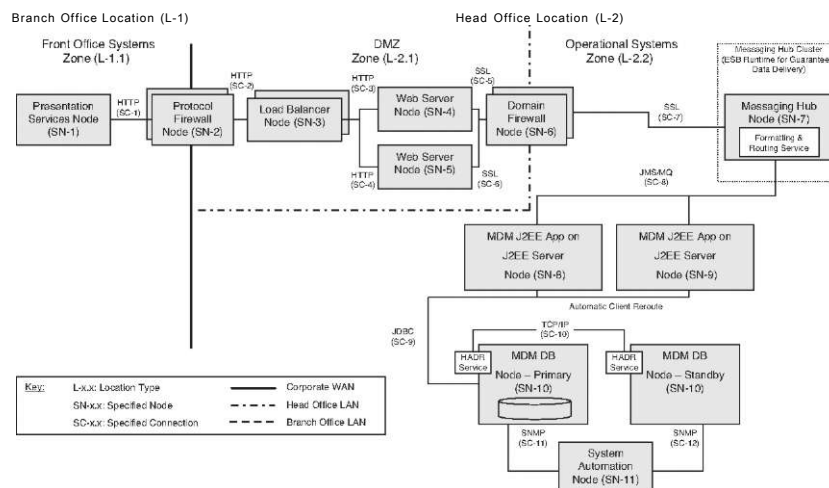
Figure 11.4 Multi-tier high availability for Critical Data Pattern for Transactional Hub deployment
