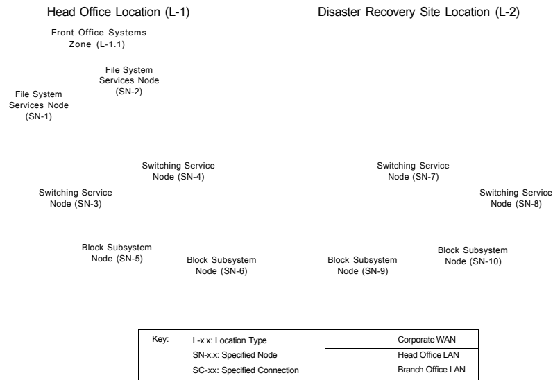
Figure 6.12 Continuous Availability and Resiliency operational pattern
