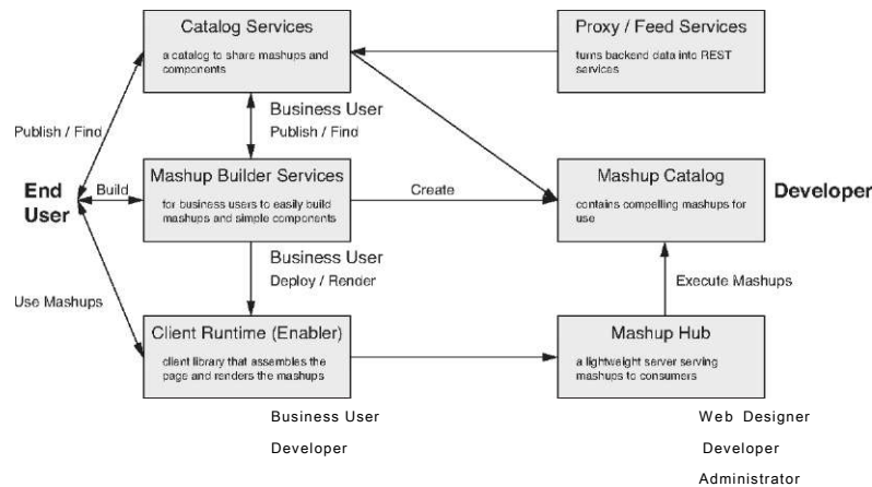
Figure 12.5 Component Interaction Diagram
