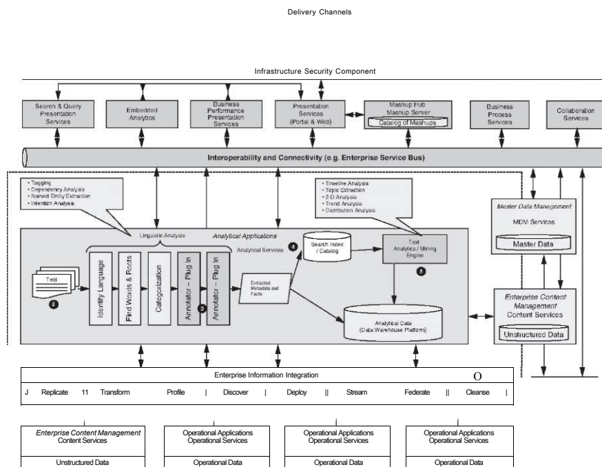
Figure 13.3 Extend the DW platform with text analytics
