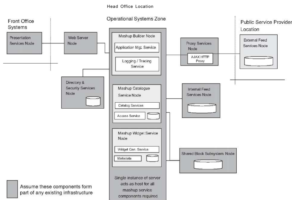
Figure 12.8 Simple Deployment Model
