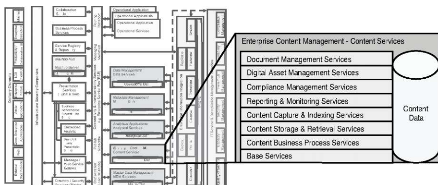
Figure 5.7 The Enterprise Content Management Component
