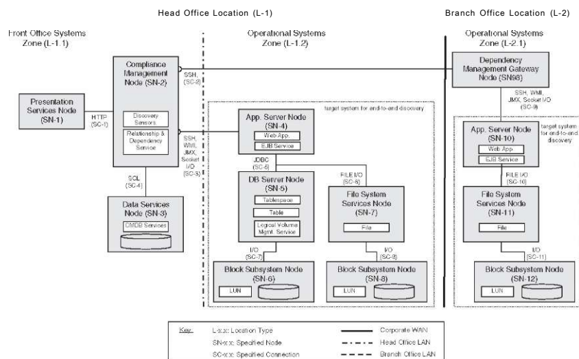
Figure 6.17 Compliance and Dependency Management for Operational Risk pattern
