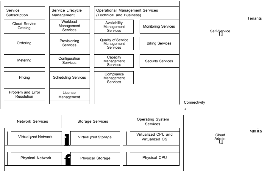
Figure 7.7 High-level Cloud Computing architecture from an Operational Model perspective
