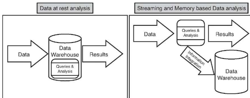
Figure 8.10 Traditional query management versus streaming data
