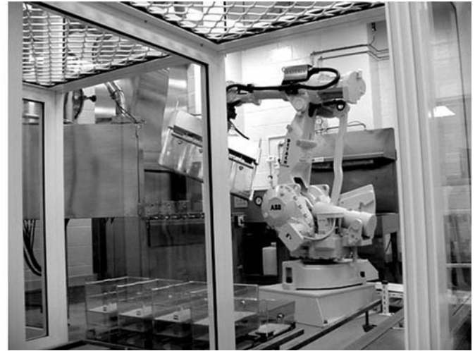
Fig. 12-8 Robotic cage-washing system showing both the soiled-side robot (left) and clean-side counterpart (right). The soiled side also shows the dirty bedding dumping station (D), in conveyor track (I) and first tunnel washer section (T). On the clean side are bedding cages on the out conveyor (O), automated bedding dispenser (B) and egress section of the tunnel washer (T).
