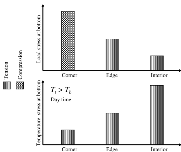
Figure 7.2: A schematic diagram indicating the possible relative magnitudes (not to scale) and nature (tension/compression) of load and thermal bending stresses in concrete pavement at the corner, edge, and interior.
