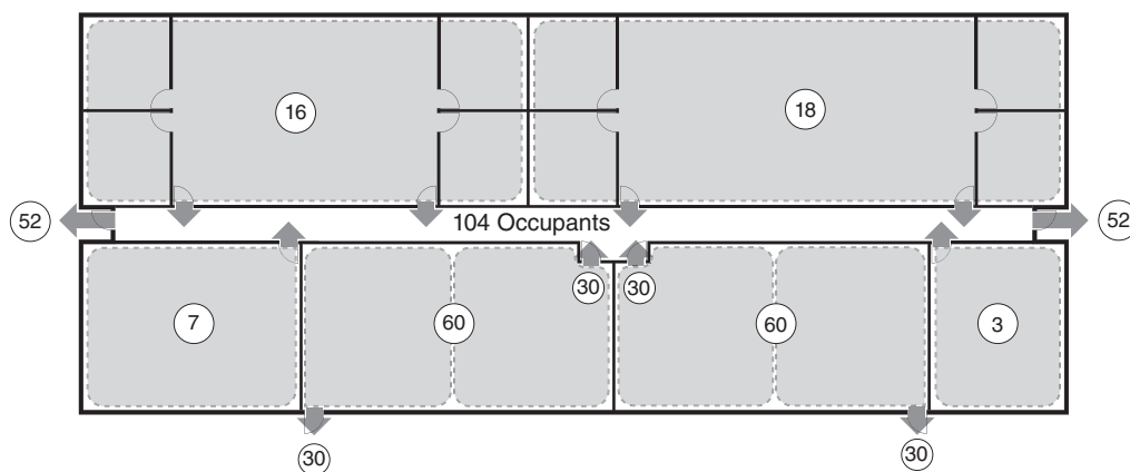
FIGURE 19.1.2-1. This floor plan has a couple of spaces that have exits directly to the exterior, which are sized for those occupant loads . The occupant load of the remaining building spaces will be used to size the means of egress serving those spaces.
