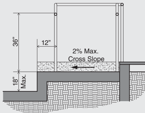
(B) SECTION
