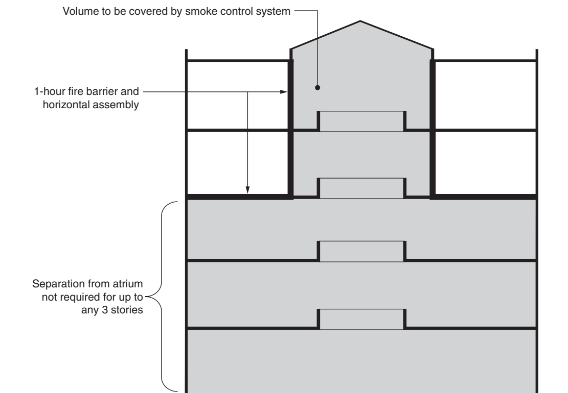
FIGURE 6.3-1. Atriums.
