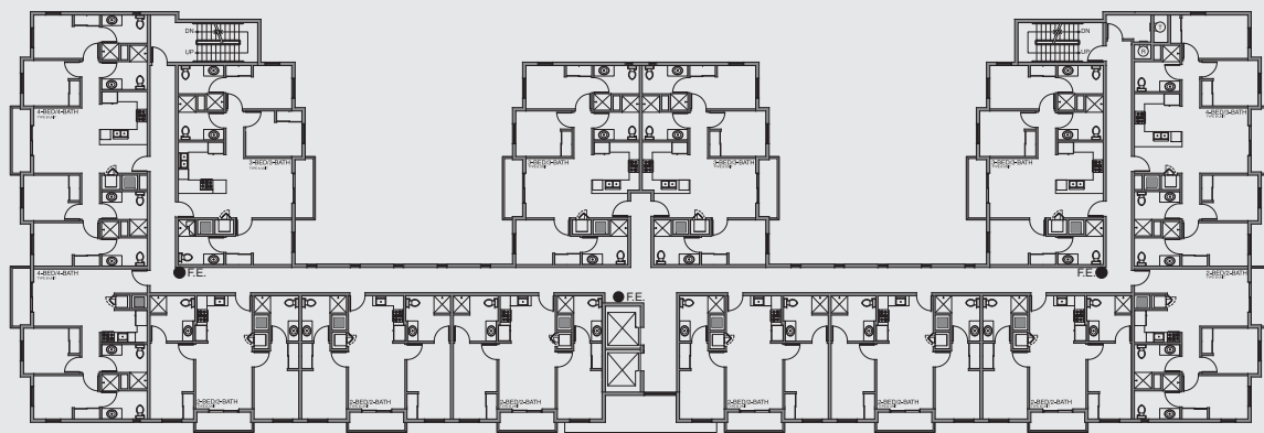
EXAMPLE PROJECT FIGURE 26-3. Location of fire extinguishers within the residential stories.
