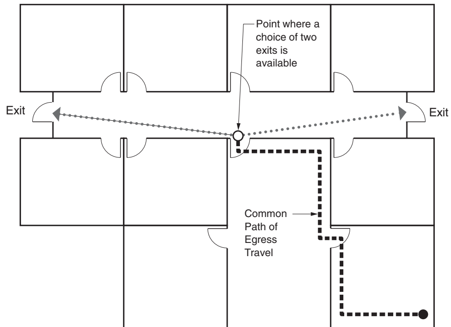
FIGURE 10.2.2-1. Determination of common path of egress travel .
