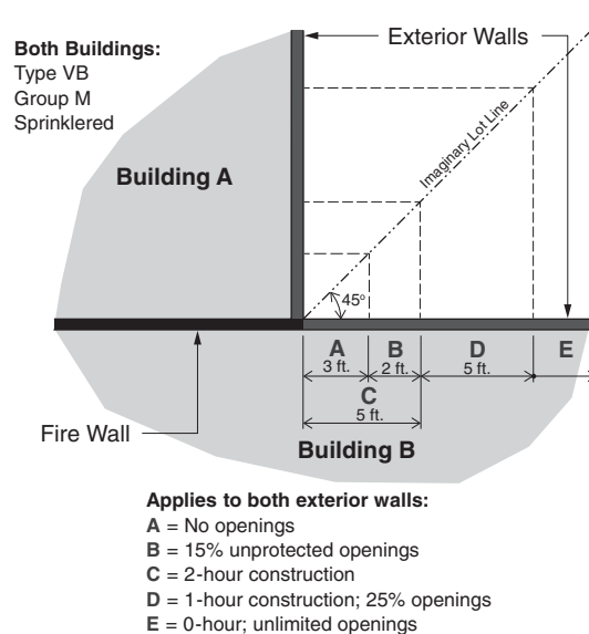
FIGURE 15.1.1.1-2. Example of terminating a fire wall at exterior walls less than 180 degrees apart using Option 2 fire separation distance method.
