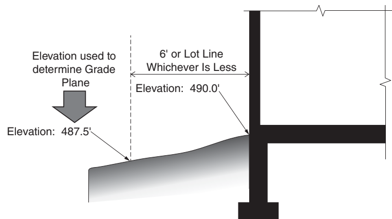
FIGURE 2.2.1-1. Establishing points to determine grade plane .
