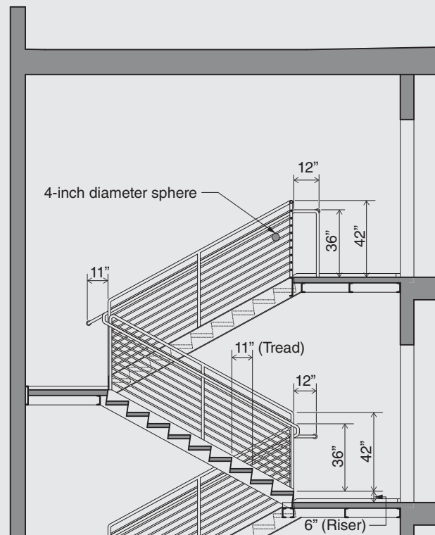
(B) SECTION
