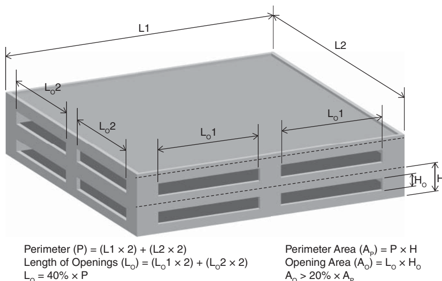
FIGURE 6.5.2.1-1. Open parking garage opening requirements.
