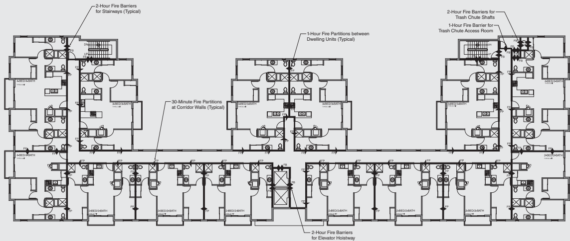
EXAMPLE PROJECT FIGURE 15-3. The residential stories with fire-resistance-rated assemblies identified.
