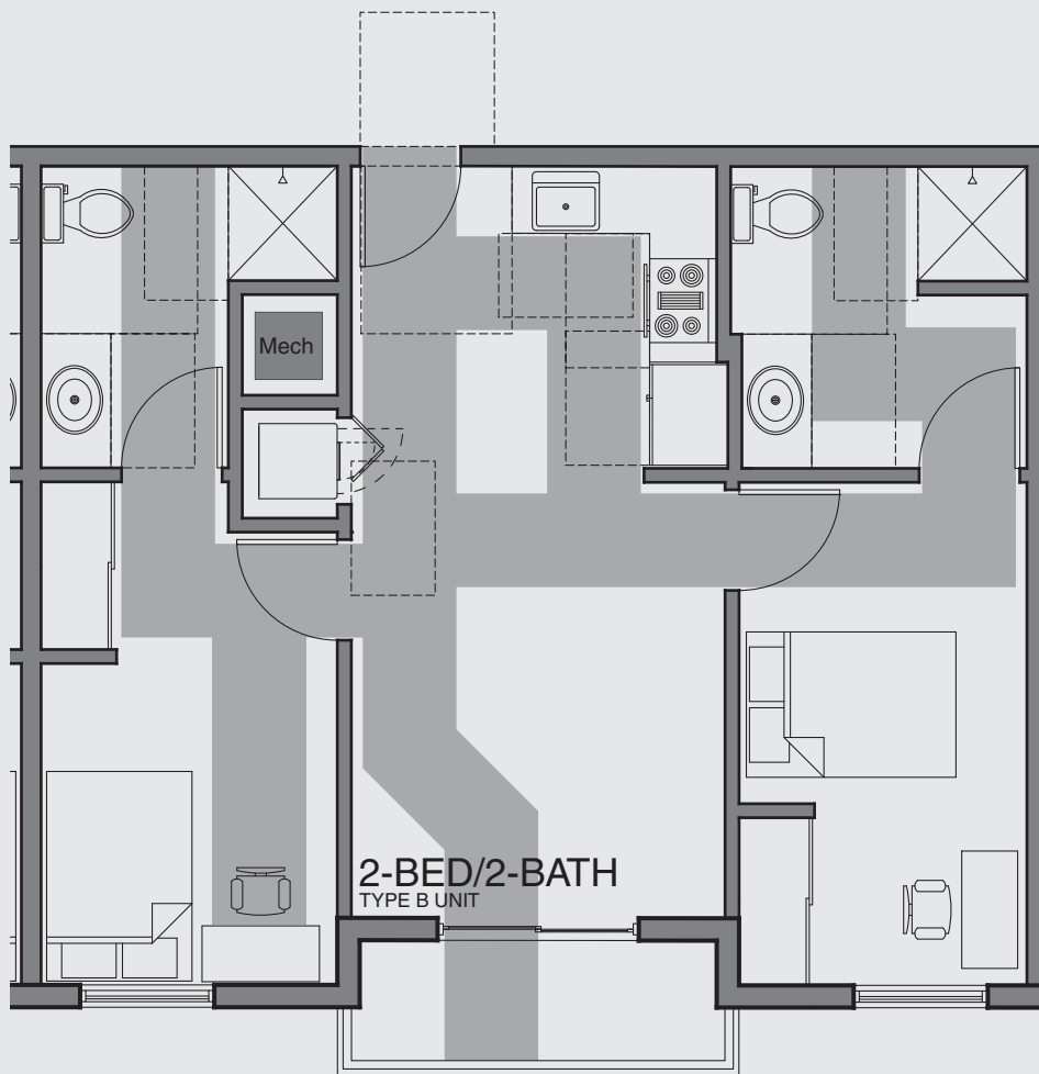
EXAMPLE PROJECT FIGURE 20-6. Type B accessible unit with 32-inch-wide assessable route.
