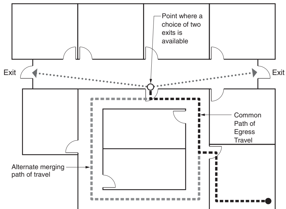
FIGURE 10.2.2-2. Merging paths are still considered a common path of egress travel .
