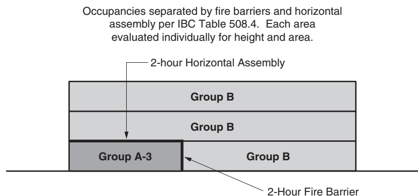
FIGURE 5.2-1. Separated occupancies.
