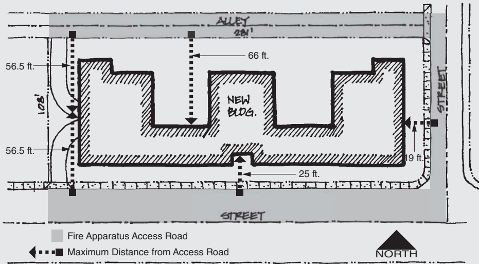
EXAMPLE PROJECT FIGURE 12-1. Site plan showing the reach around the building perimeter from the fire apparatus access roads.
