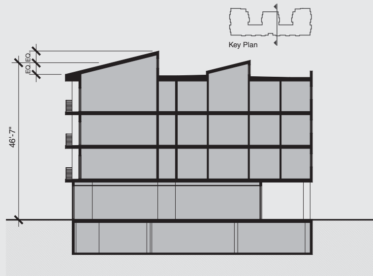
EXAMPLE PROJECT FIGURE 14-1. Revised height of building.
