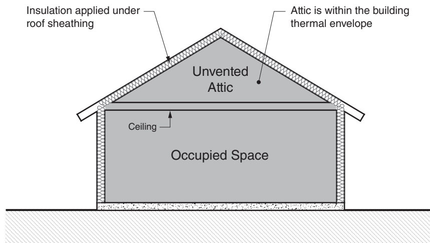
FIGURE 17.1.3.1-1. Location of insulation per the first condition of IBC Section 1203.3 making the attic part of the conditioned space .
