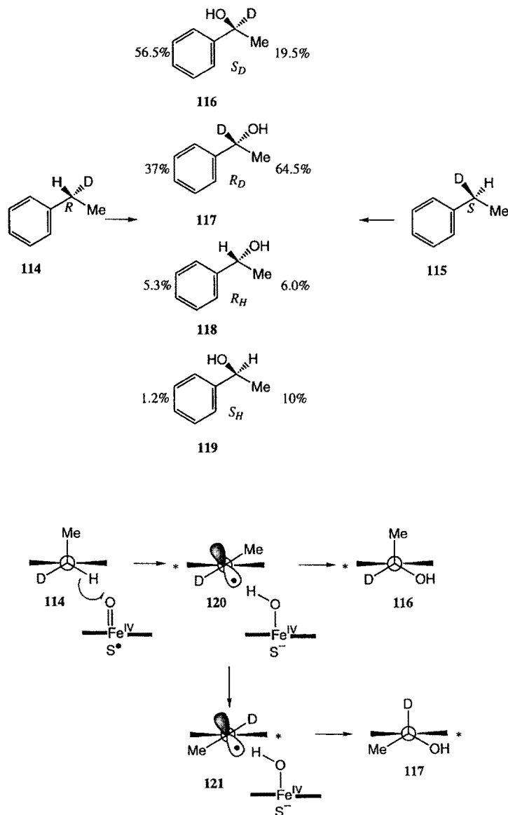
Fig. 18. Benzylic hydroxylation with P450 enzymes and model compounds
