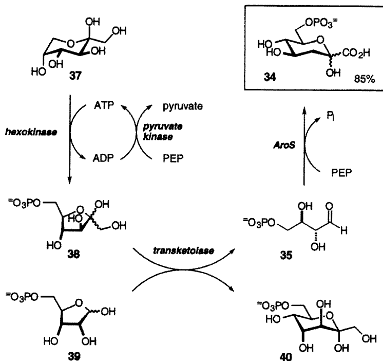
Scheme 5. Combined enzymatic synthesis of 3-deoxy-D-arabino-heptulosonic acid 7-phosphate
