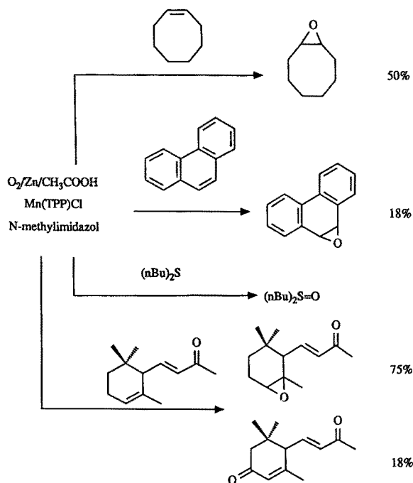
Fig. 38. Various epoxidations using Mn(III)TPP Cl/O 2 under reductive conditions
