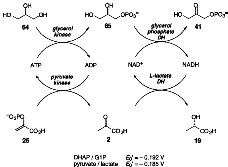
Scheme 12. ‘Artificial metabolism’ for closed-loop ATP/ \text{NAD}^+ -cofactor regeneration, applied to the multienzymatic in-situ preparation of DHAP from glycerol
