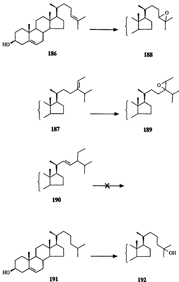
Fig. 31. Regio- and stereospecific oxidations with metallocporphyrin vesicles
