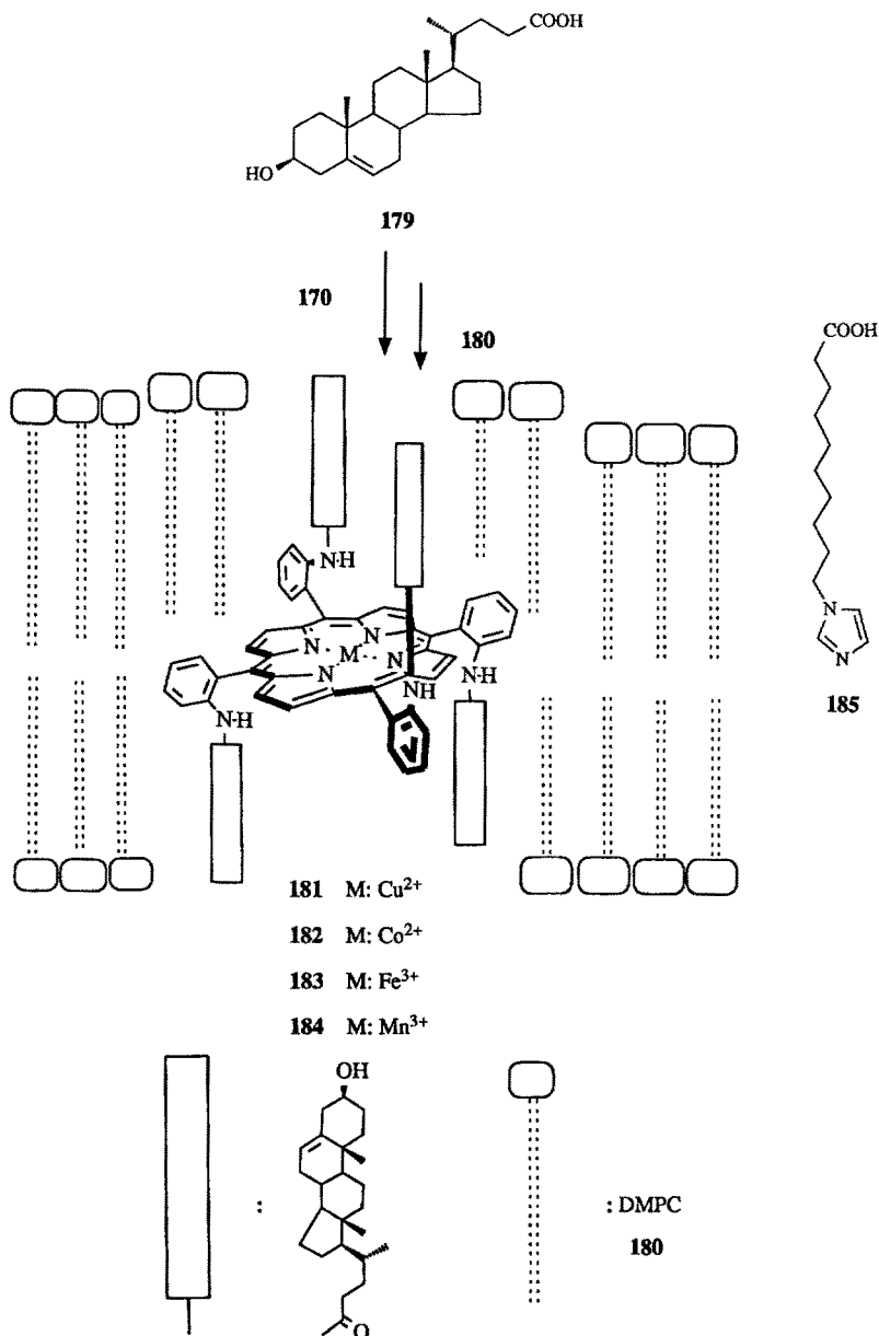
Fig. 30. Metalporphyrins embedded in bilayers
