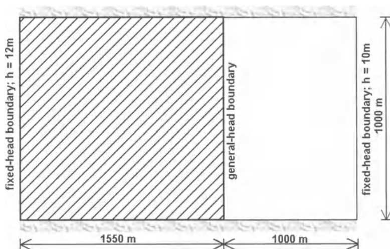
Fig. 6.18. Plan view of the model area
