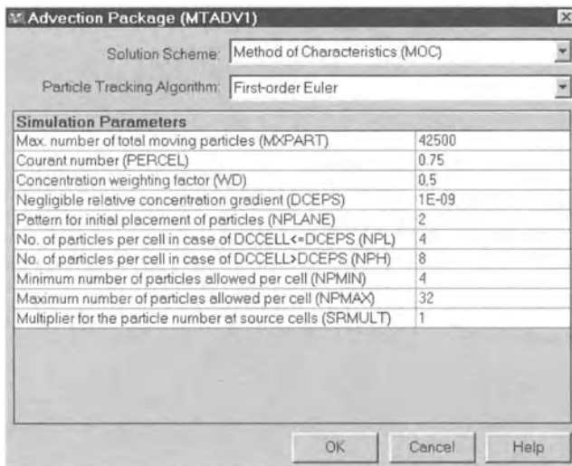
Fig. 2.22. The Advection Package (MTADV1) dialog box
