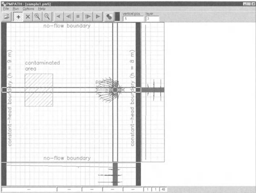
Fig. 2.19. The 100-days capture zone calculated by PMPATH
