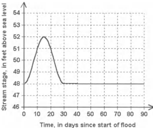
Fig. 6.30. Model calculated river stage
