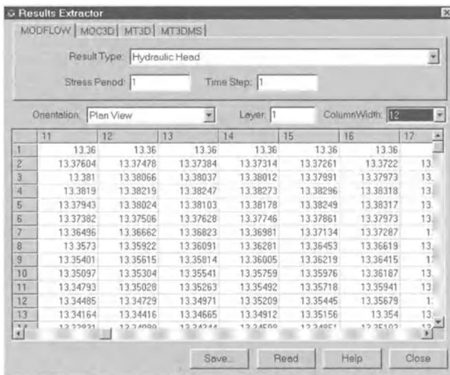
Fig. 5.7. The Results Extractor dialog box
