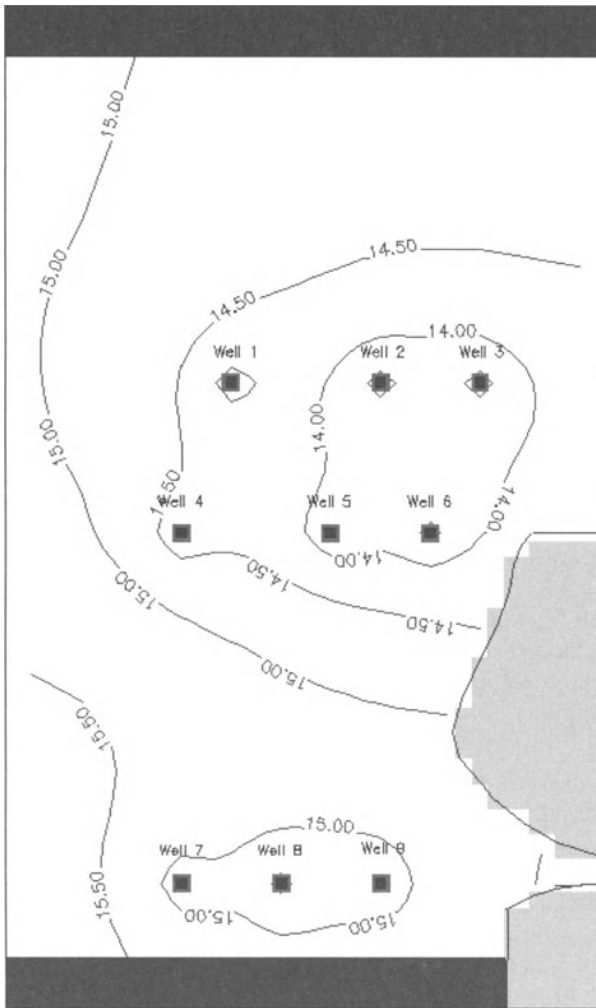
Fig. 6.5. Head distribution after 240 days of pumping (period 1, time step 12)
