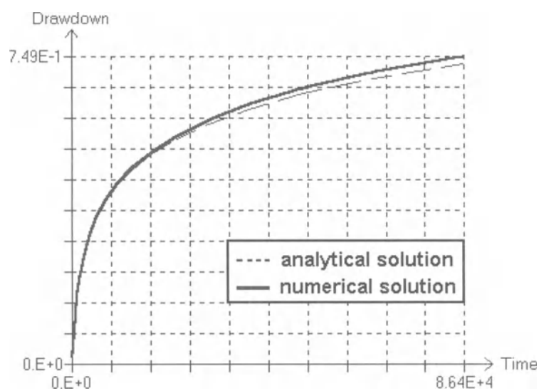
Fig. 6.40. Drawdown-time curves
