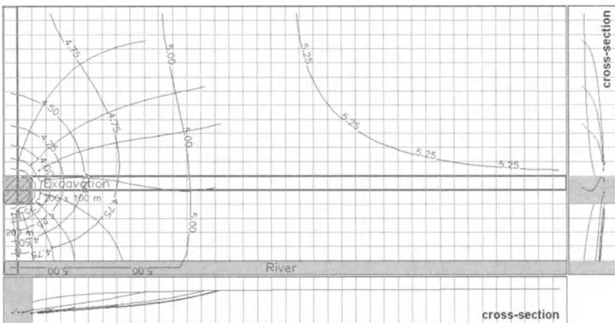
Fig. 6.44. Simulated head distribution and catchment area of the excavation pit
