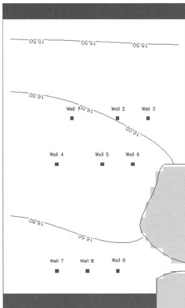
Fig. 6.6. Head distribution after 120 days of recharge (period 2, time step 6)
