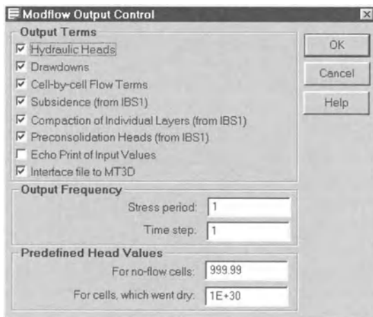
Fig. 3.28. The Modflow Output Control dialog box
