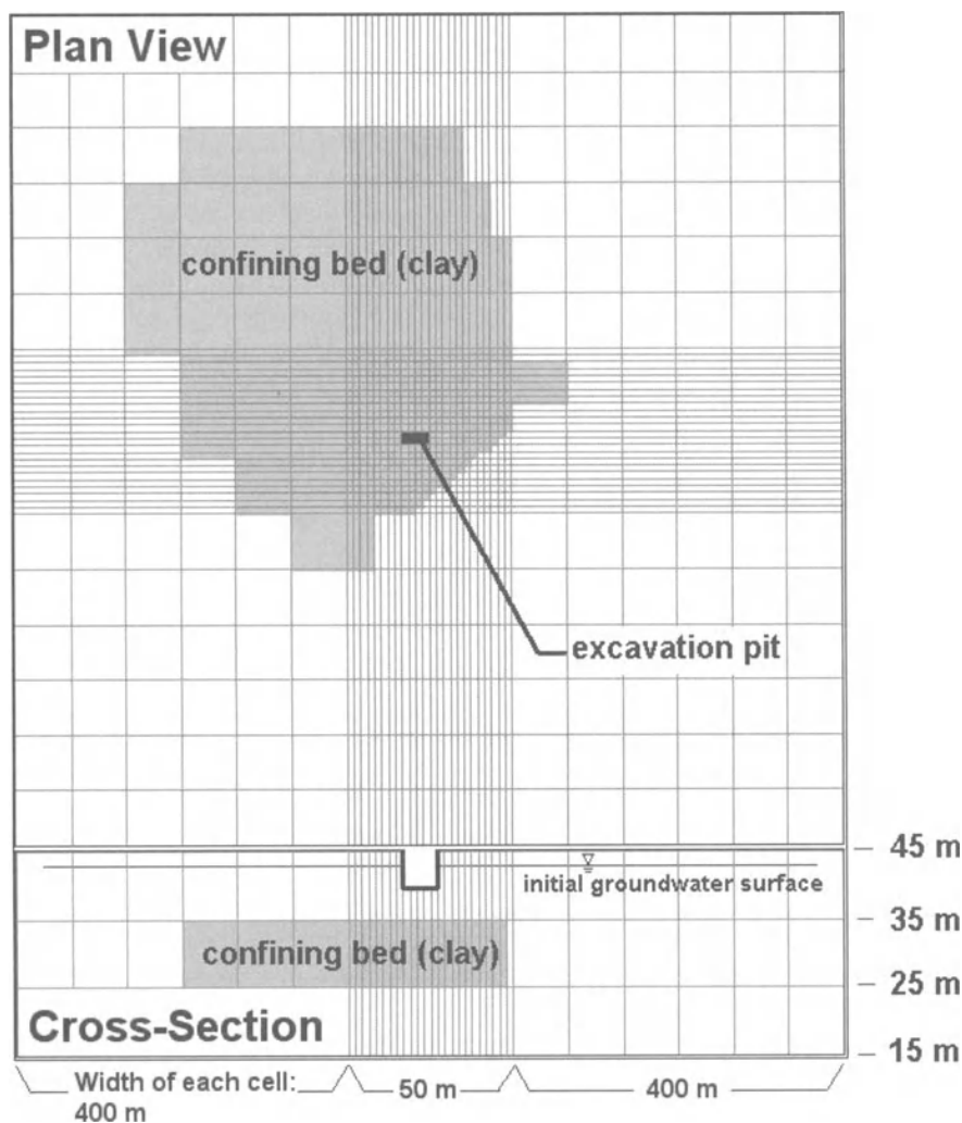
Fig. 6.56. Model grid and boundary conditions
