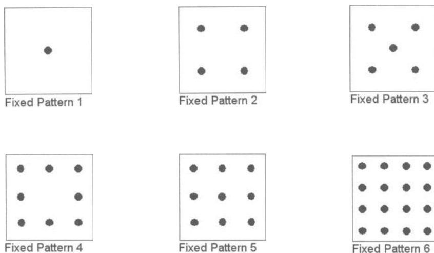
Fig. 3.42. Distribution of initial particles using the fixed pattern (adopted from Zheng 1990) If the fixed pattern is chosen, the number of particles placed per cell (NPL and NPH) is divided by the number of planes NPLANE to yield the number of particles to be placed on each plane, which is then rounded to one of the numbers of particles shown here.
