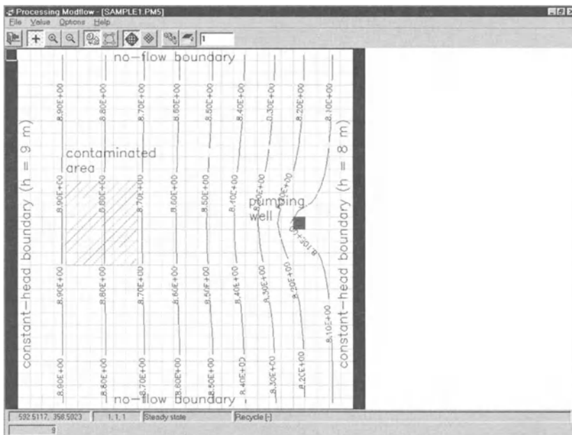
Fig. 2.14. A contour map of the hydraulic heads in the first layer
