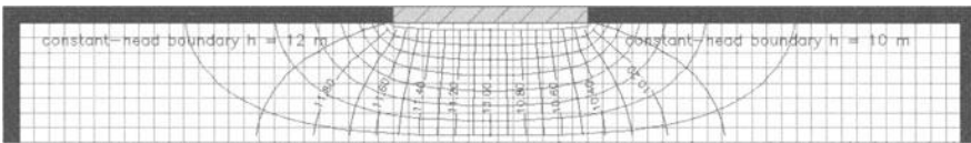
Fig. 6.47. Flowlines and calculated head contours for isotropic medium
