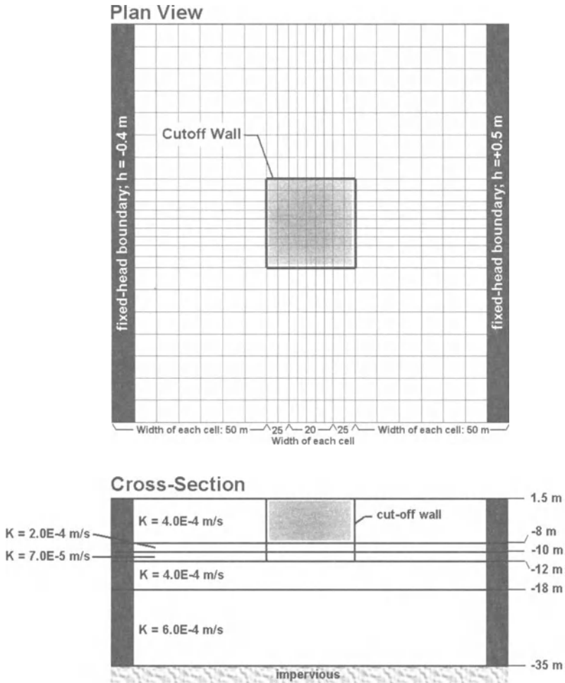
Fig. 6.53. Model grid and boundary conditions
