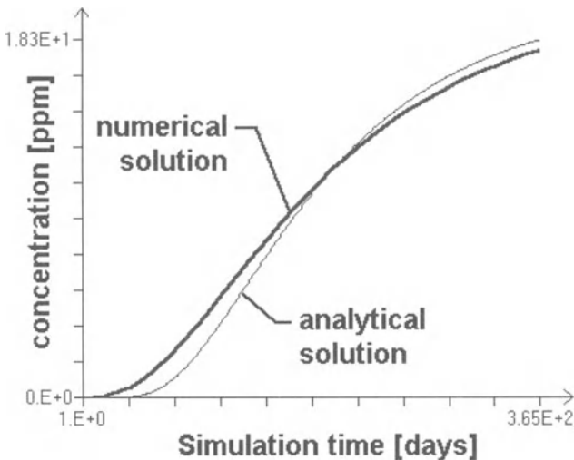
Fig. 6.62. Comparison of the breakthrough curves at the observation borehole. The numerical solution is obtained by using the upstream finite difference method.
