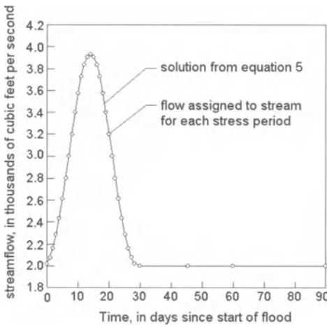
Fig. 6.29. Distribution of streamflow for a 30-day flood event used for the simulation (after Prudic 1988)
