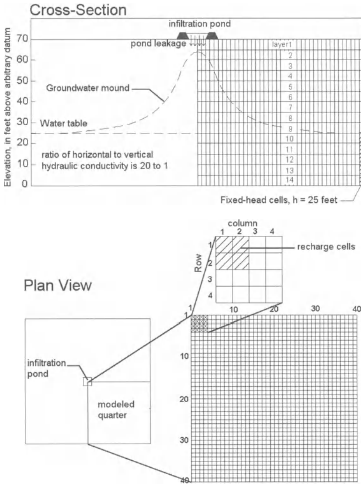
Fig. 6.22. Hydrogeology and model grid configuration
