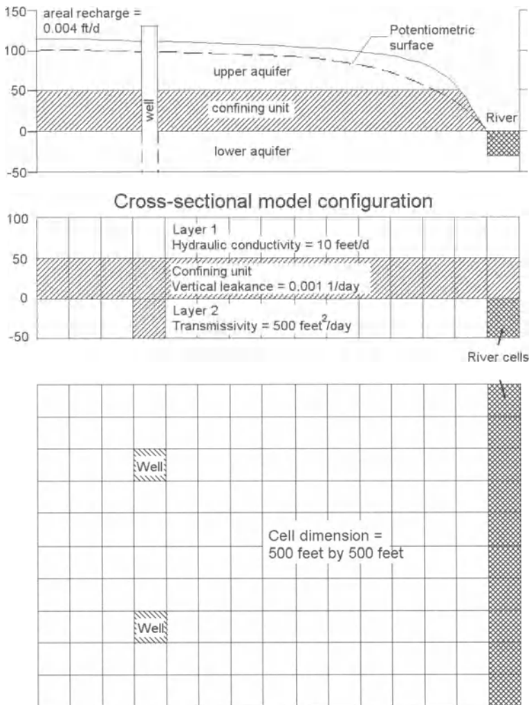
Fig. 6.21. Configuration of the hypothetical model (after McDonald et al. 1991)
