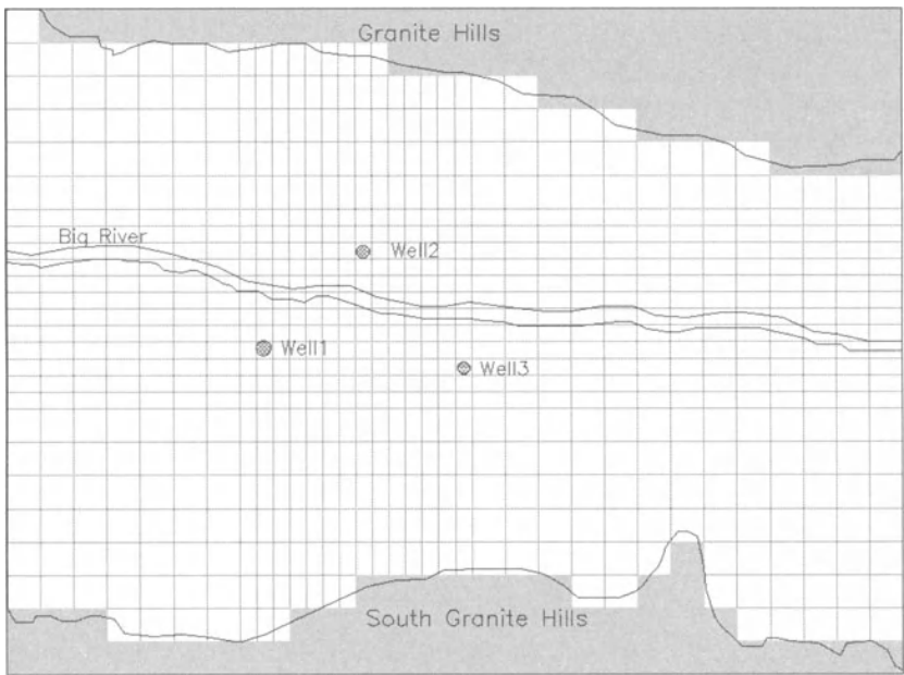
Fig. 6.10. Boundary conditions in the 2 nd layer
