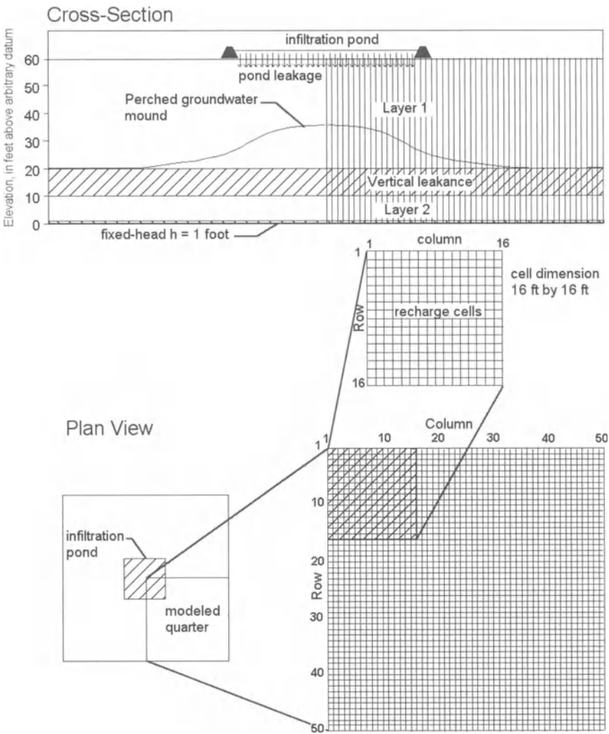
Fig. 6.24. Hydrogeology and model grid configuration
