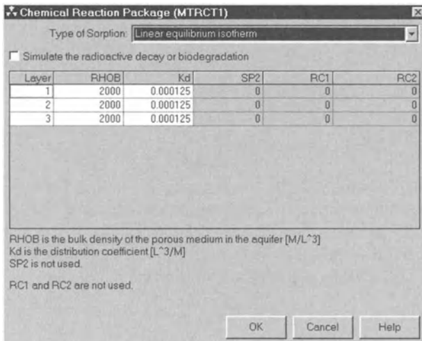
Fig. 3.44. The Chemical Reaction Package (MTRCT1) dialog box
