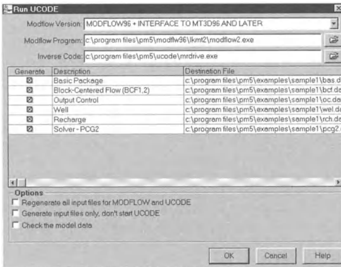
Fig. 3.57. The Run UCODE dialog box
