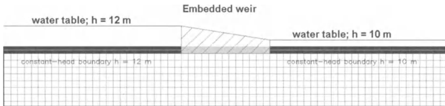
Fig. 6.46. Model grid and the boundary conditions
