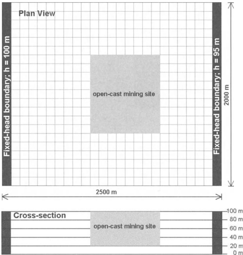
Fig. 6.32. Plan and cross-sectional views of the model area
