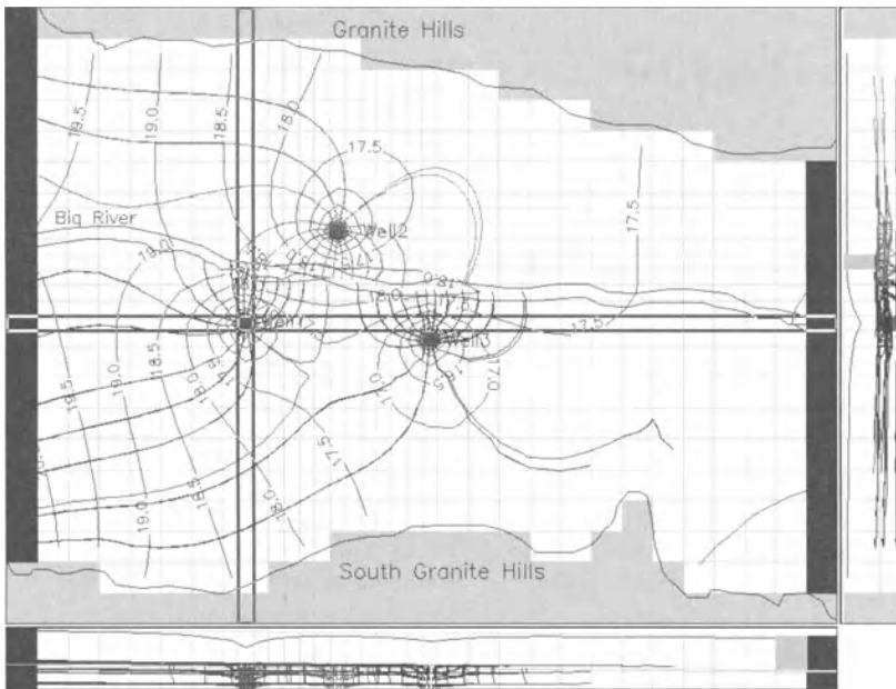
Fig. 6.12. Steady state hydraulic head distribution in the 3 rd model layer and capture zones of the pumping wells
