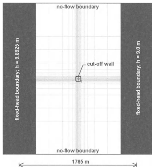
Fig. 6.36. Plan view of the model
