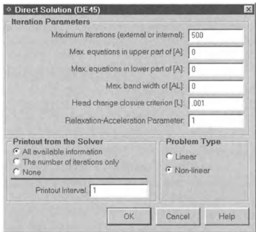
Fig. 3.29. The Direct Solution (DE45) dialog box
