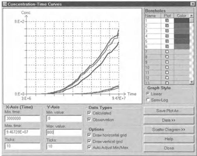
Fig. 2.28. Concentration-time curves at the observation boreholes 1-6
