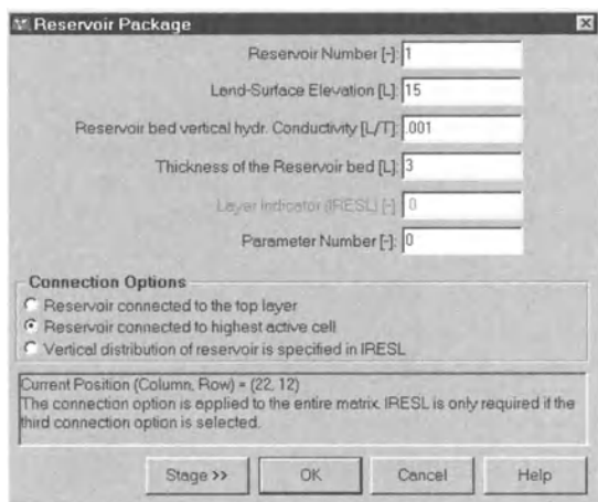
Fig. 3.21. The Reservoir Package dialog box
