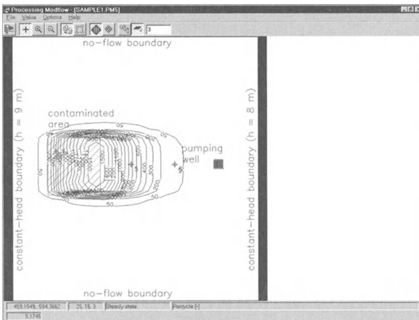
Fig. 2.34. Simulated concentration at 3 years in the third layer
