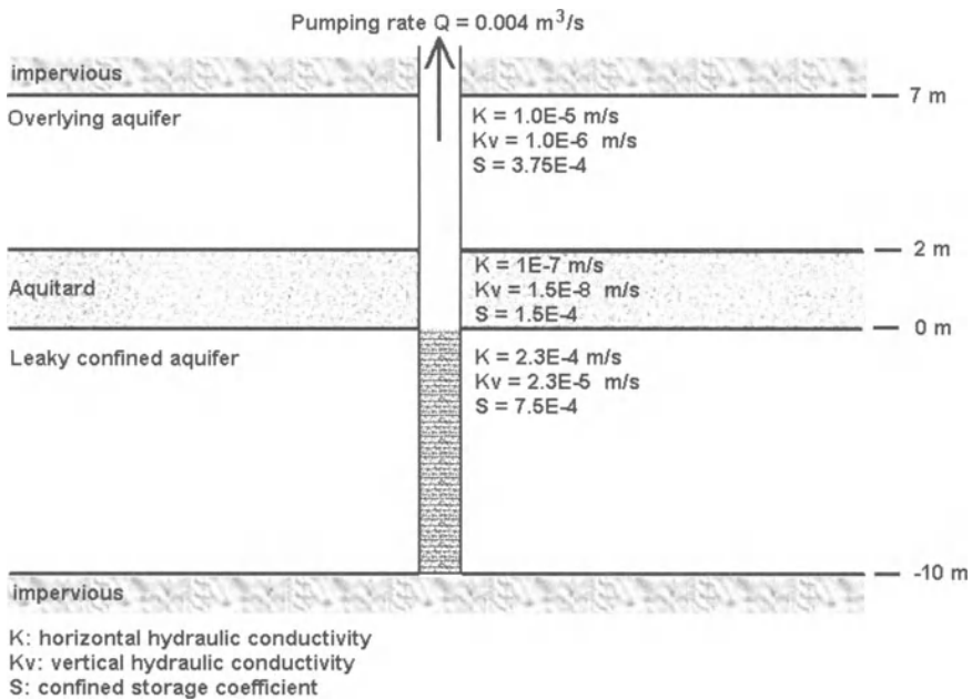
Fig. 6.41. Configuration of the leaky aquifer system and the aquifer parameters
