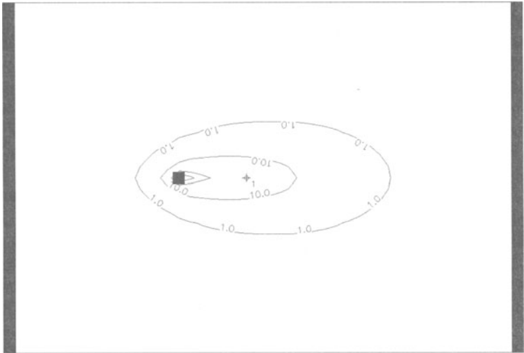
Fig. 6.60. Calculated concentration distribution
