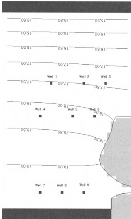
Fig. 6.4. Steady state head distribution
