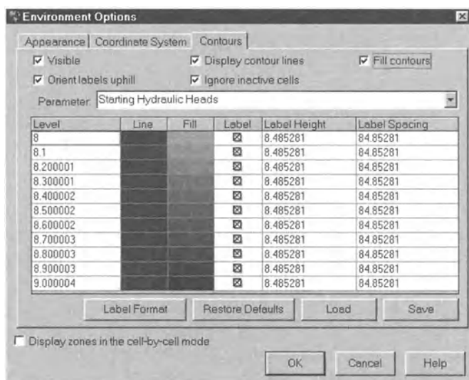
Fig. 3.65. The Contours tab of the Environment Options dialog box
