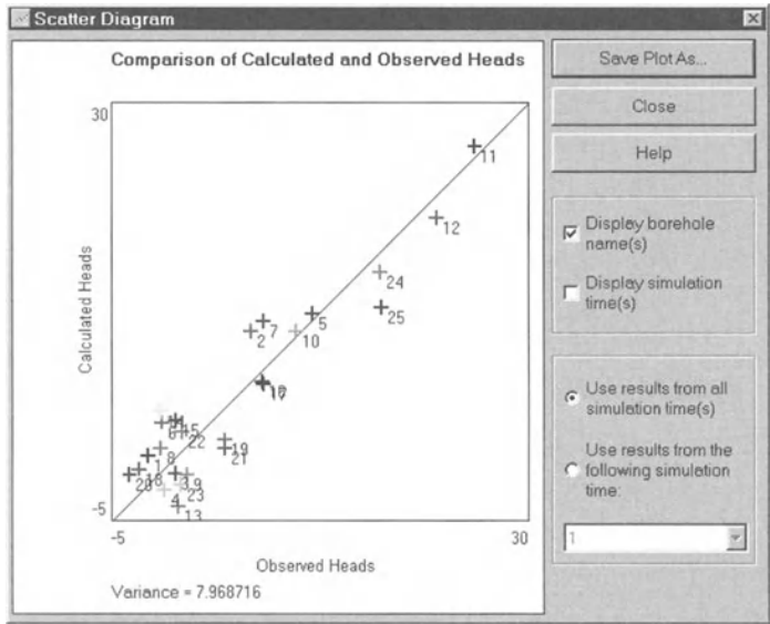
Fig. 5.11. The Scatter Diagram dialog box
