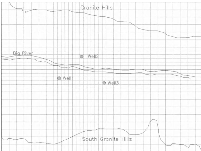
Fig. 6.8. Model discretization
