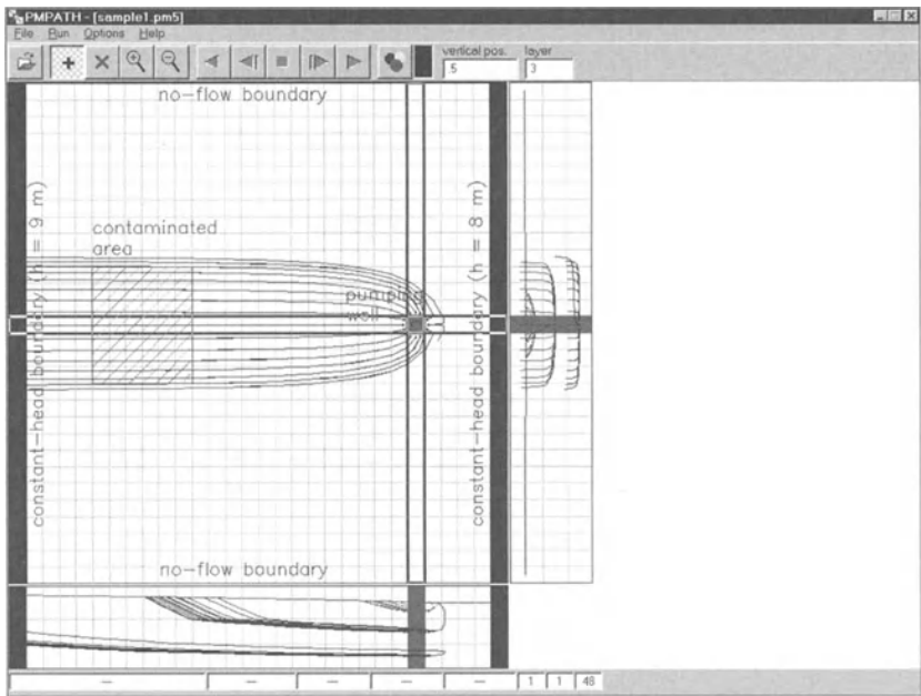
Fig. 2.18. The capture zone of the pumping well (with vertical exaggeration = 10)
