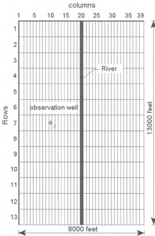
Fig. 6.26. Configuration of the model grid and the location of the observation well
