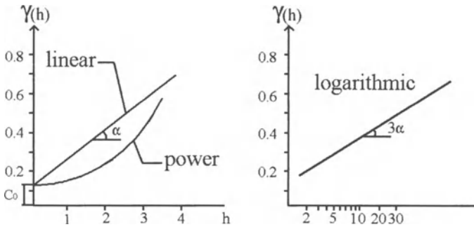
Fig. 5.4. Linear, power and logarithmic models
