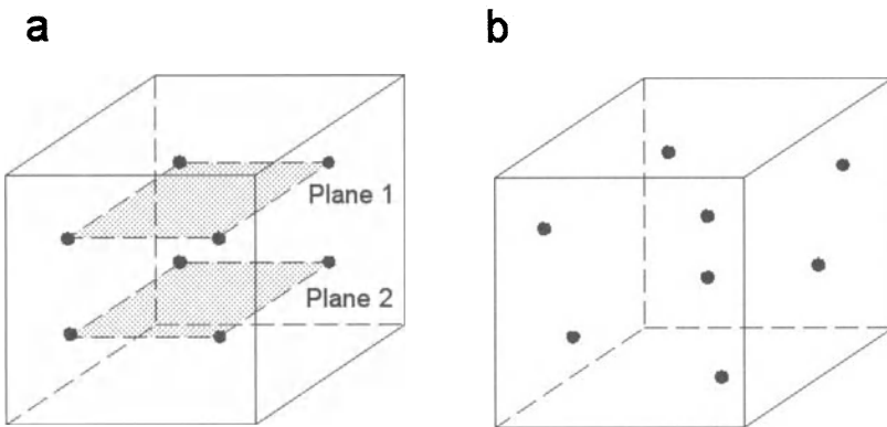
Fig. 3.41. Initial placement of moving particles (adopted from Zheng 1990)
