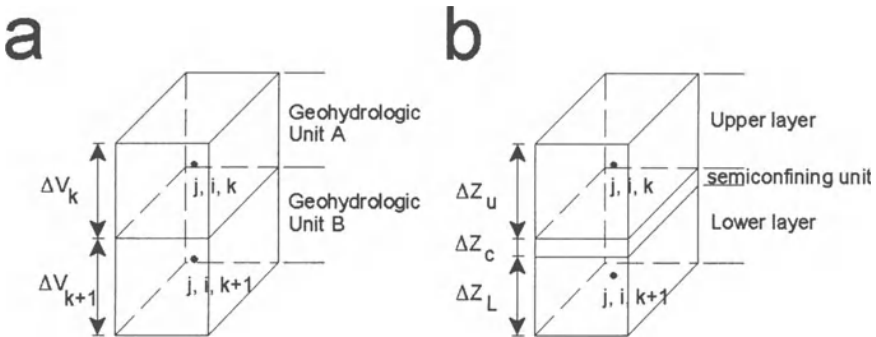
Fig. 3.15. Grid configurations used for the calculation of VCONT
