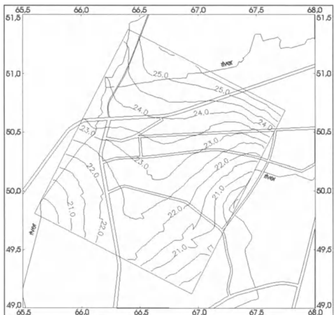
Fig. 6.65. Contours produced by the Kriging method
