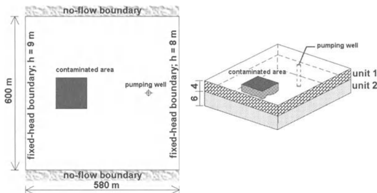
Fig. 2.1. Configuration of the sample problem
