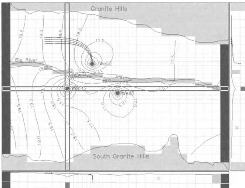
Fig. 6.13. 125-year streamlines; particles are started at the cell [6, 5, 1] and flow towards Well 2
