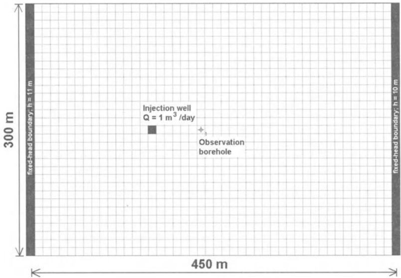
Fig. 6.59. Configuration of the model and the location of an observation borehole
