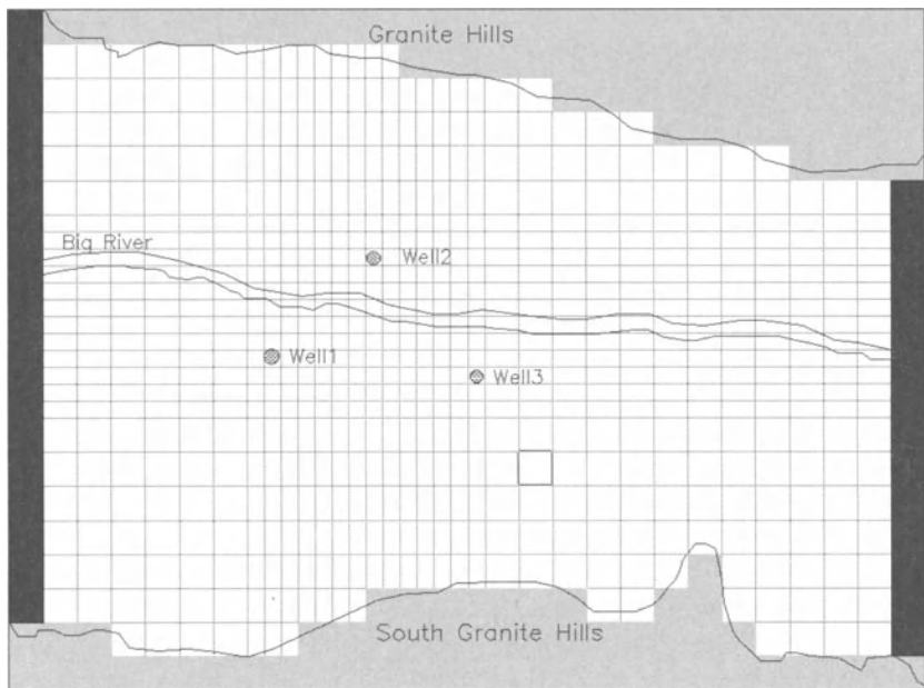
Fig. 6.9. Boundary conditions in the 1 st layer and 3 rd layer
