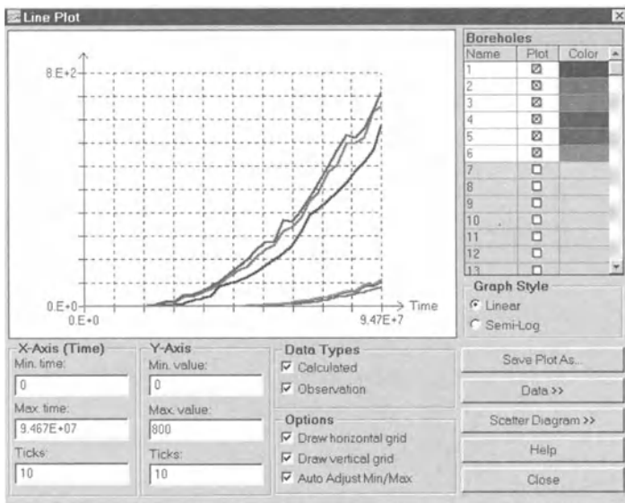
Fig. 2.35. Concentration-time curves at the observation boreholes
