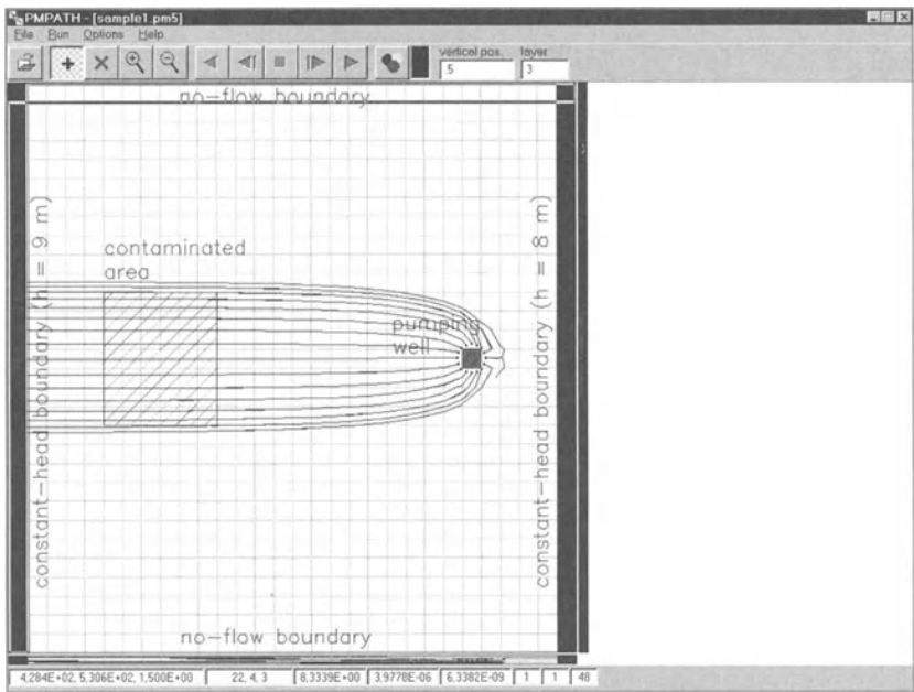
Fig. 2.17. The capture zone of the pumping well (with vertical exaggeration = 1)
