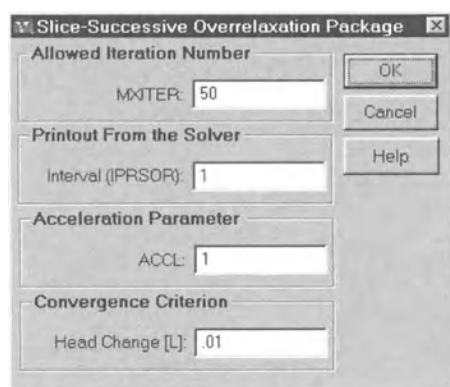
Fig. 3.32. The Slice-Successive Overrelaxation Package dialog box
