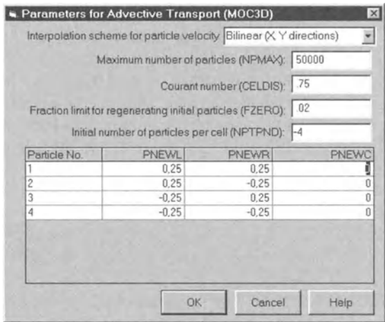
Fig. 3.35. The Parameters for Advective Transport (MOC3D) dialog box
