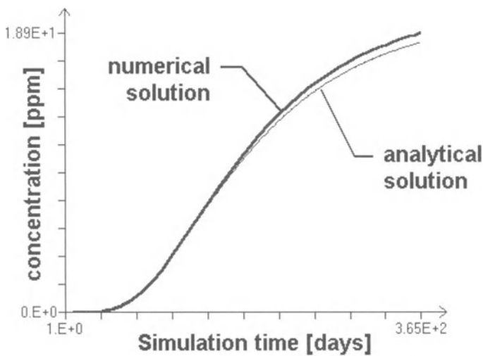
Fig. 6.61. Comparison of the breakthrough curves at the observation borehole. The numerical solution is obtained by using the 3rd order TVD scheme.
