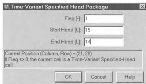
Fig. 3.26. The Time-Variant Specified-Head Package dialog box
