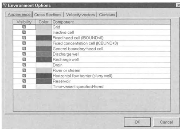
Fig. 4.7. The Environment Options dialog box
