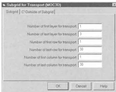
Fig. 2.29. The Subgrid for Transport (MOC3D) dialog box
