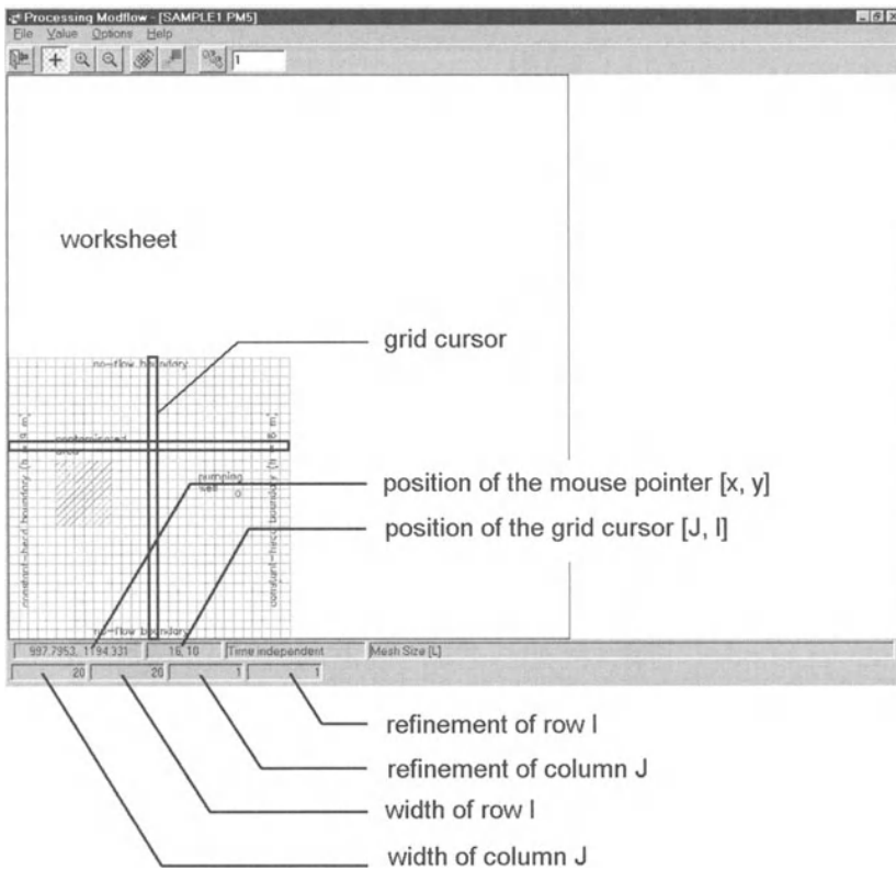
Fig. 3.3. The Grid Editor
