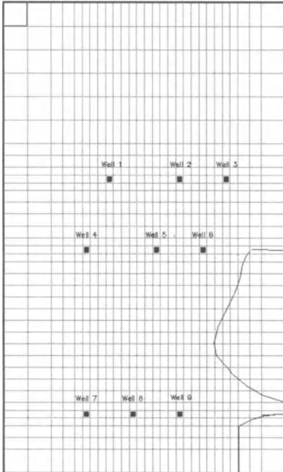
Fig. 6.2. Model discretization
