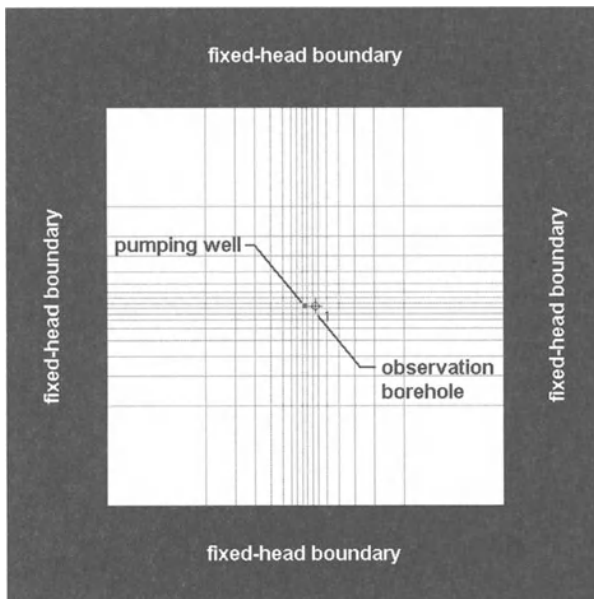
Fig. 6.39. Configuration of the groundwater model
