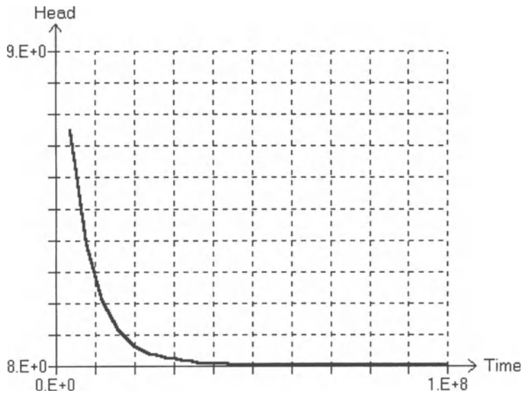
Fig. 6.38. Head versus time curve at the center of the contaminated area
