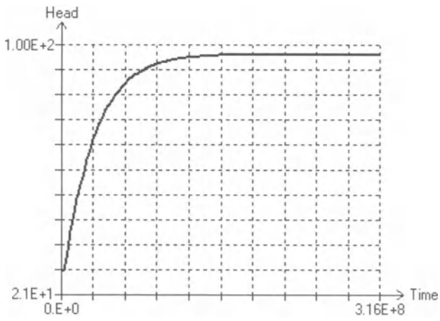
Fig. 6.34. Temporal development curve of the water stage in the artificial lake
