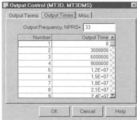
Fig. 3.46. Specifying the output times for MT3D and MT3DMS
