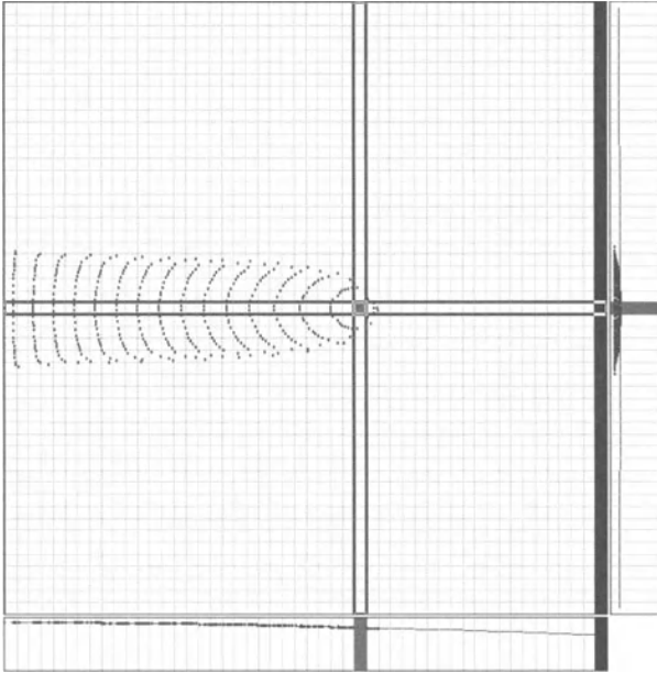
Fig. 6.17. Catchment area of the pumping well (3D-approach)
