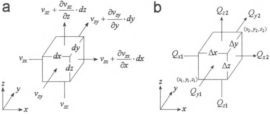
Fig. 4.2. (a) Flow through an infinitesimal volume of a porous medium and (b) the finite-difference approach
