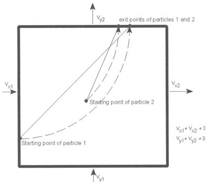
Fig. 4.4. Schematic illustration of the spurious intersection of two pathlines in a two-dimensional cell
