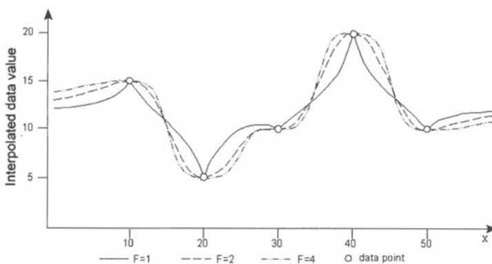
Fig. 5.2. Effects of different weighting exponents
