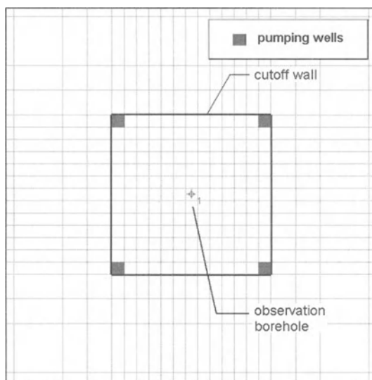
Fig. 6.37. Location of the cutoff wall and pumping wells
