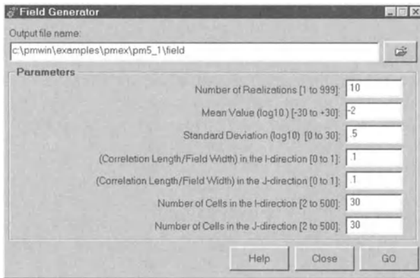
Fig. 5.6. The Field Interpolator dialog box
