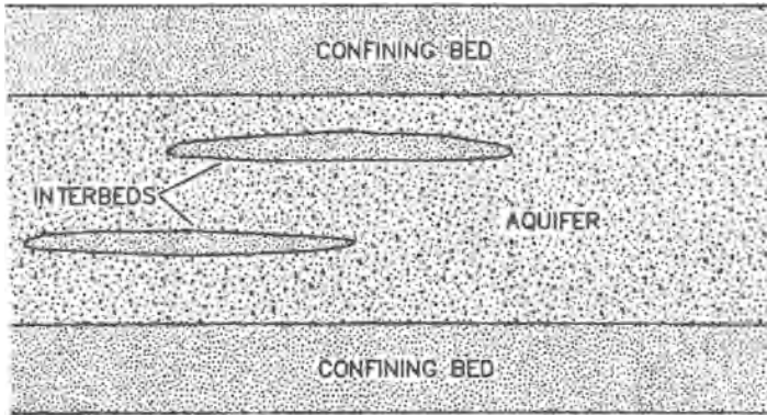
Fig. 3.19. Types of fine-grained beds in or adjacent to aquifers. Beds may be discontinuous interbeds or continuous confining beds. Adopted from Leake and Prudic (1991).
