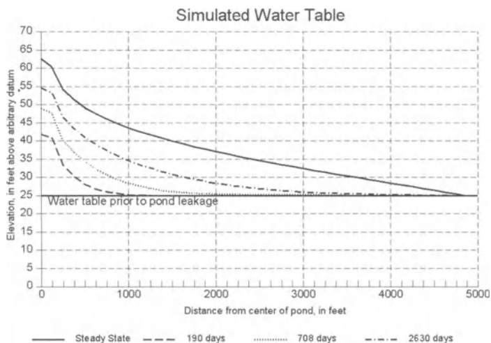
Fig. 6.23. Simulated water-table along row 1 beneath a leaking pond after 190, 708, 2630 days and steady state conditions (after McDonald et al. 1991)
