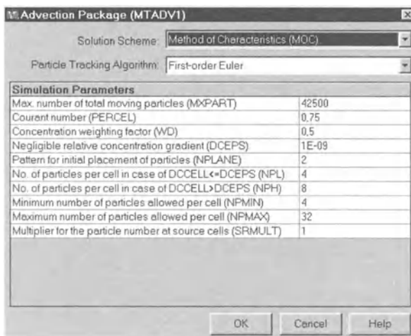
Fig. 3.40. The Advection Package (MTADV1) dialog box
