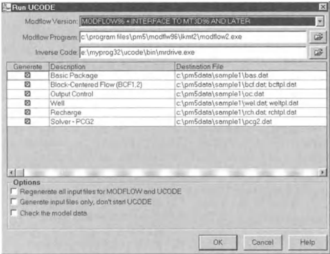
Fig. 2.41. The Run UCODE dialog box
