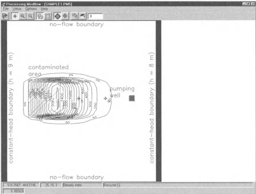
Fig. 2.27. Simulated concentration at 3 years in the third layer
