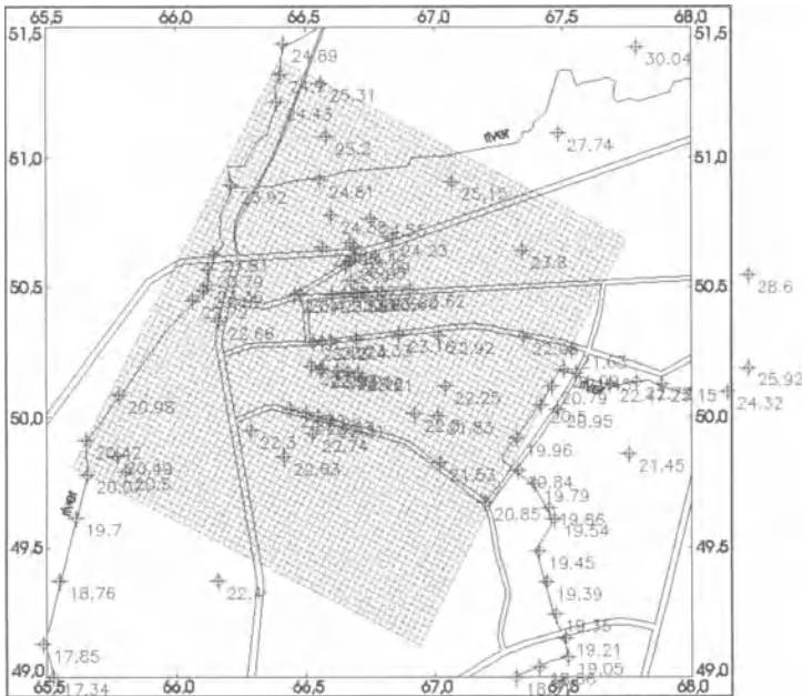
Fig. 6.63. Model domain and the measured hydraulic heads
