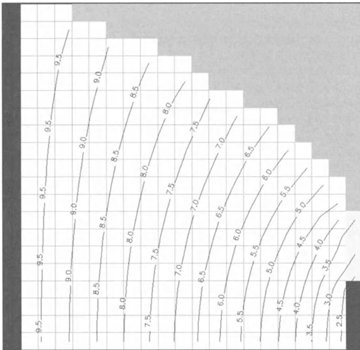
Fig. 6.52. Calculated hydraulic heads distribution and the form of the seepage surface
