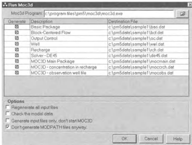
Fig. 3.39. The Run Moc3d dialog box
