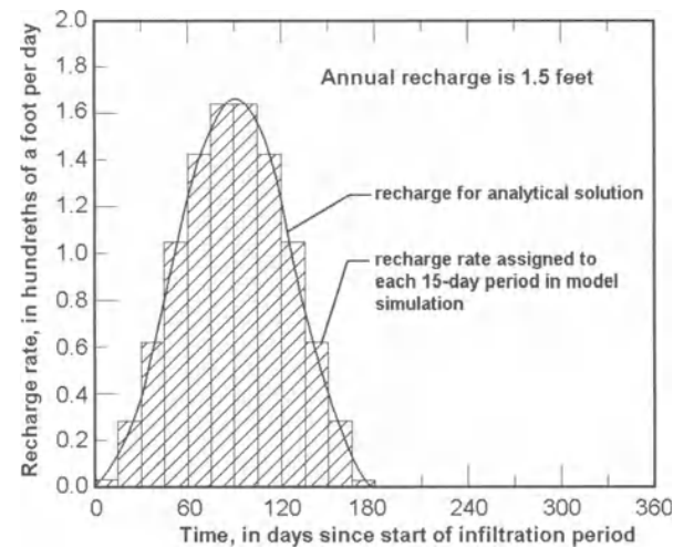
Fig. 6.27. Distribution of recharge used for analytical solution and the model simulation (after Prudic, 1988)
