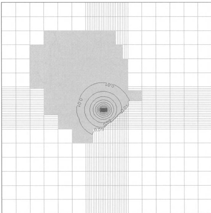
Fig. 6.57. Distribution of the land surface subsidence (maximum 0.11 m)
