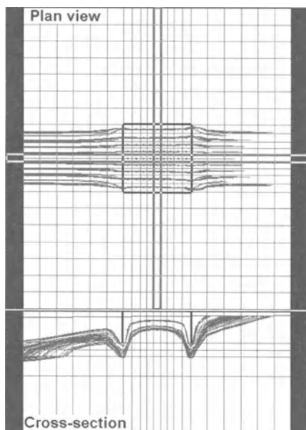
Fig. 6.54. Plan and cross-sectional views of flowlines. Particles are started from the contaminated area. The depth of the cutoff wall is -8 m.
