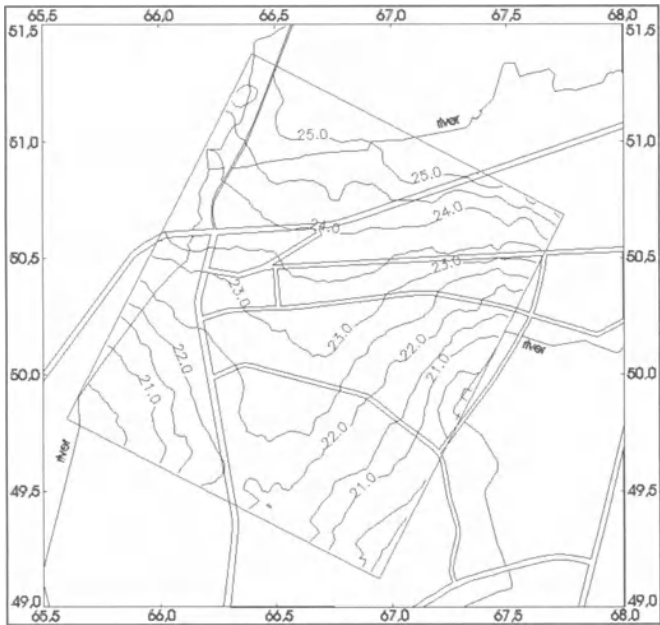
Fig. 6.64. Contours produced by Shepard's inverse distance method
