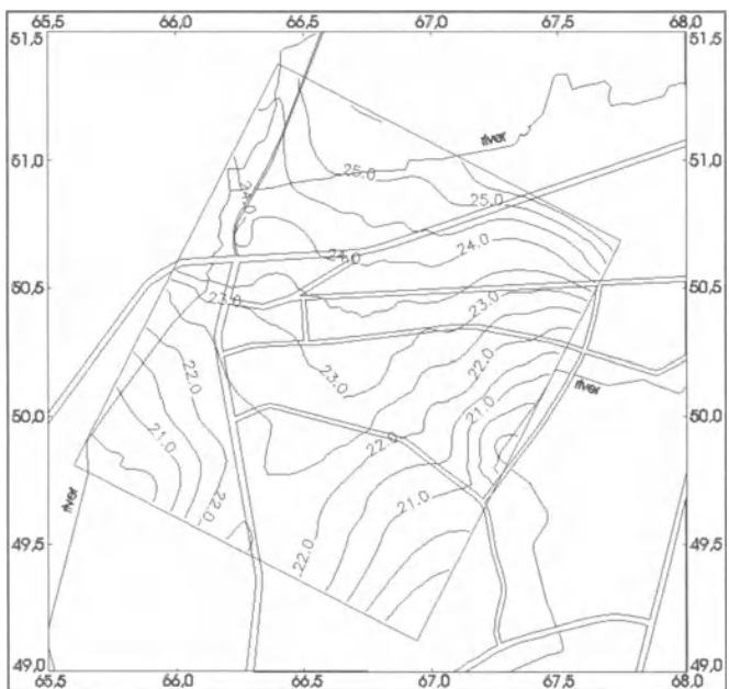
Fig. 6.66. Contours produced by Akima's bivariate interpolation
