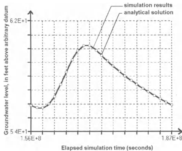
Fig. 6.28. Comparison of simulation results to analytical solution developed by Oakes and Wilkinson (1972)
