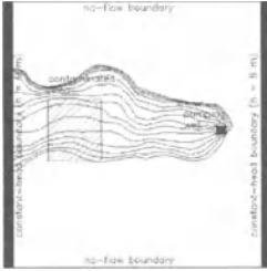
Fig. 6.68. Calculation of the mean safety criterion by the Monte Carlo method
