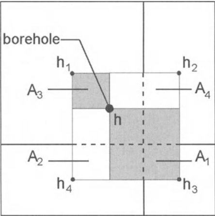
Fig. 5.9. Interpolation of simulation results to a user-specified borehole
