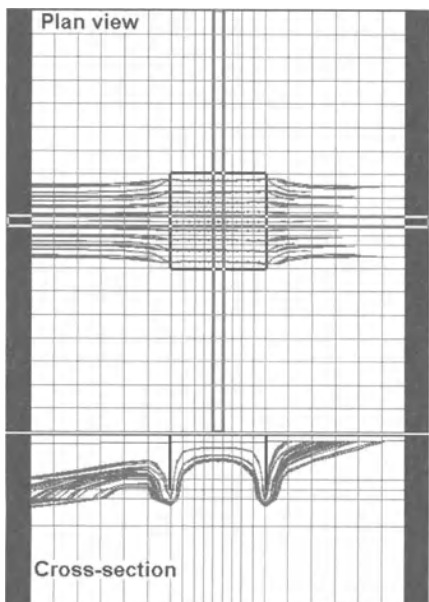
Fig. 6.55. Plan and cross-sectional views of flowlines. Particles are started from the contaminated area. The depth of the cutoff wall is -10 m.
