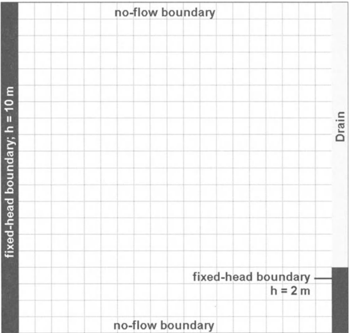
Fig. 6.50. Model grid and the boundary conditions
