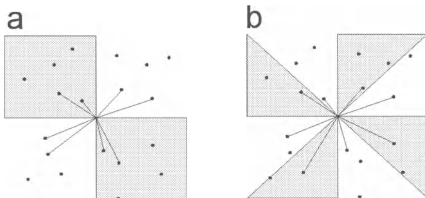
Fig. 5.5. Search pattern used by (a) the Quadrant Search method ( Data per sector=2 ) and (b) the Octant Search method ( Data per sector=1 )
