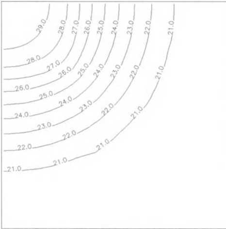
Fig. 6.25. Simulated steady state head distribution in layer 1
