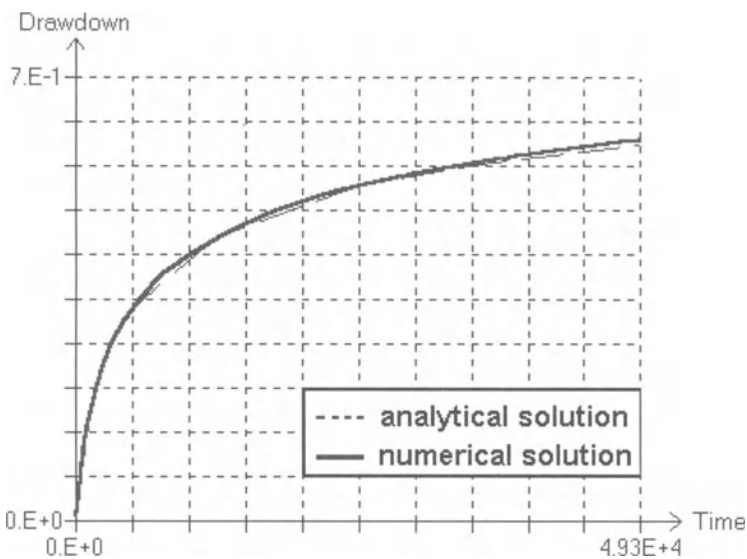
Fig. 6.42. Drawdown-time curves
