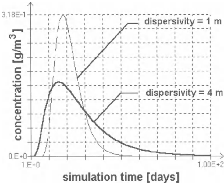
Fig. 6.58. Comparison of the calculated breakthrough curves with different dispersivity values
