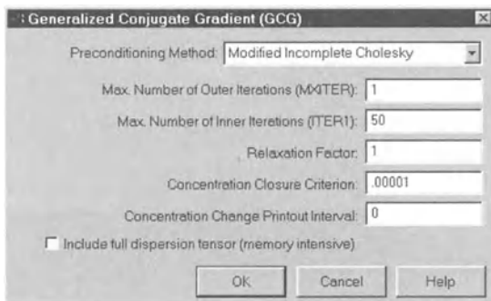
Fig. 3.51. The Generalized Conjugate Gradient (GCG) dialog box
