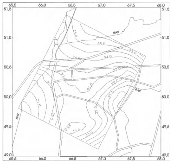
Fig. 6.67. Contours produced by Renka's triangulation algorithm
