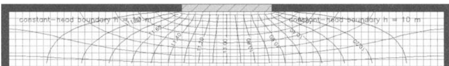
Fig. 6.48. Flowlines and calculated head contours for anisotropic medium
