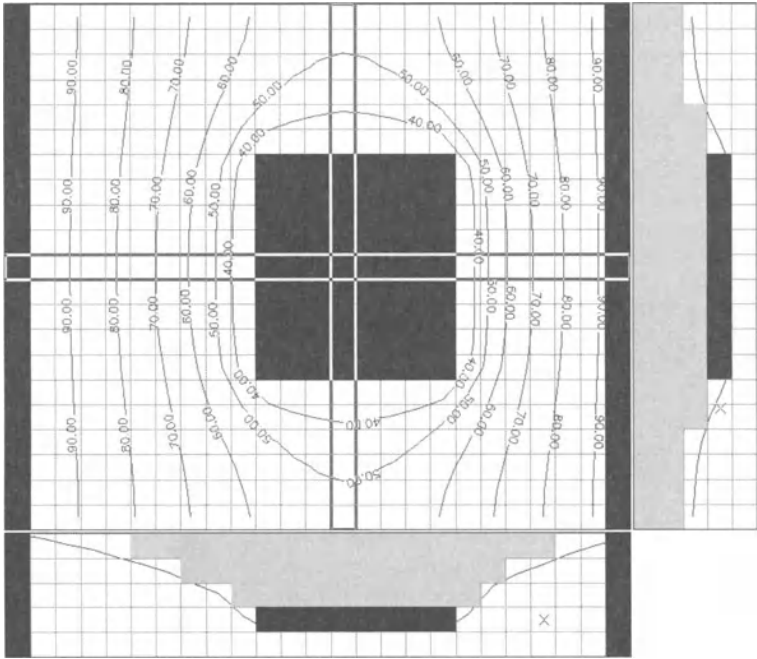
Fig. 6.33. Head contours in layer 4
