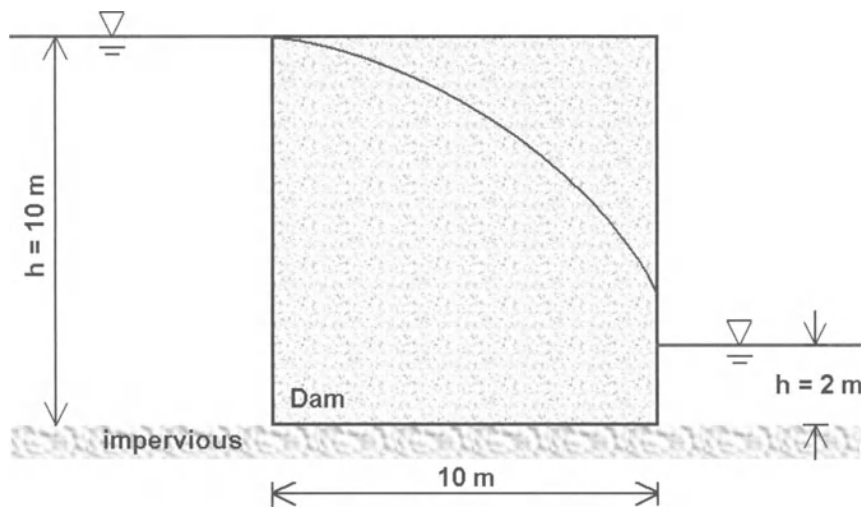
Fig. 6.49. Seepage surface through a dam
