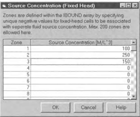
Fig. 3.37. The Source Concentration (Fixed Head) dialog box
