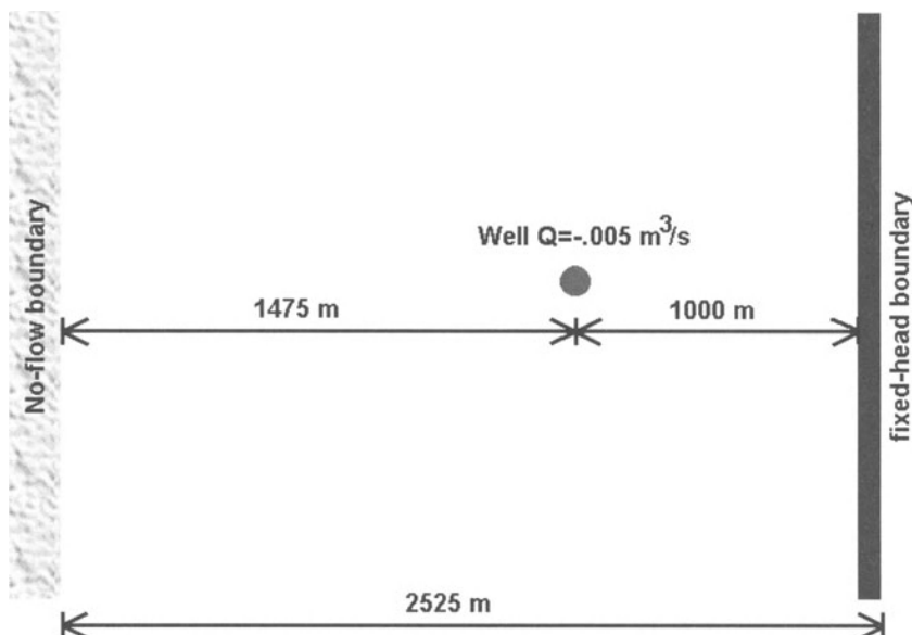
Fig. 6.14. Plan view of the model area
