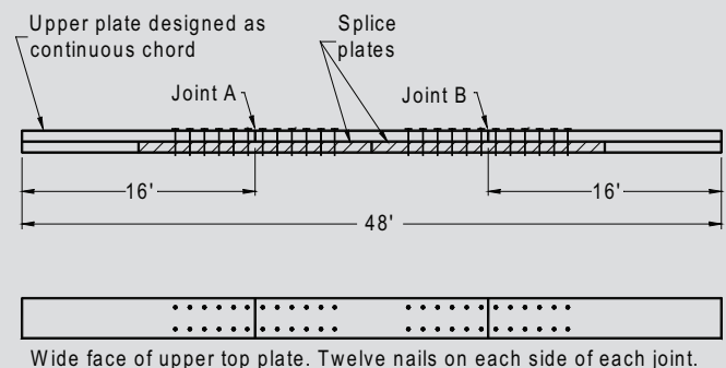
Figure C4.2.2-3b Diaphragm Chord, Double Top Plate with Two Joints in Upper Plate
