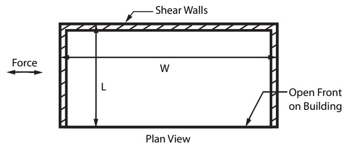
Figure 4A Open Front Structure
