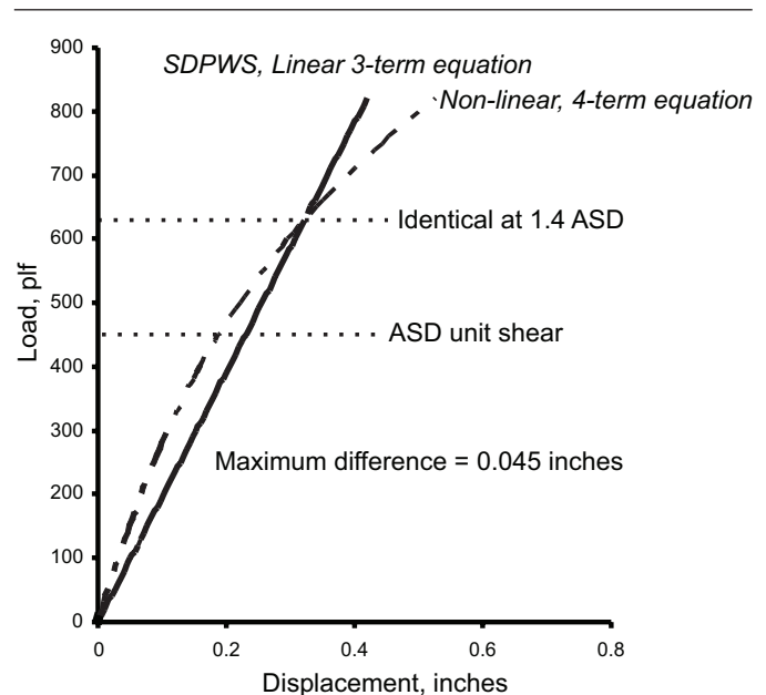
Figure C4.3.2 Comparison of 4-Term and 3-Term Deflection Equations
