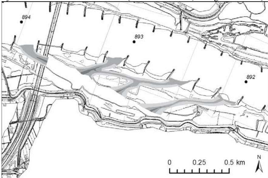
Fig. 2 Example of a CFR intervention at Beuningen. A number of secondary channels with varying characteristics cut across the sandbar creating a diverse landscape with semi-permanent islands (Source: Kater 2006).
