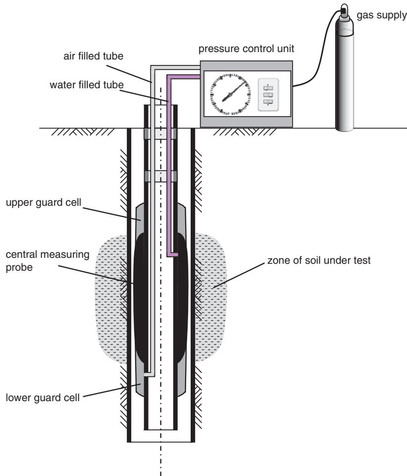
Fig. 6.13 Pressuremeter test.
