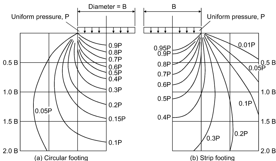
Fig. 3.12 Bulbs of pressure for vertical stress.
