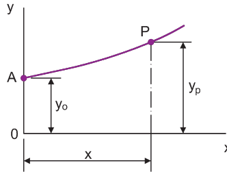
Fig. 12.11 Taylor's series.
