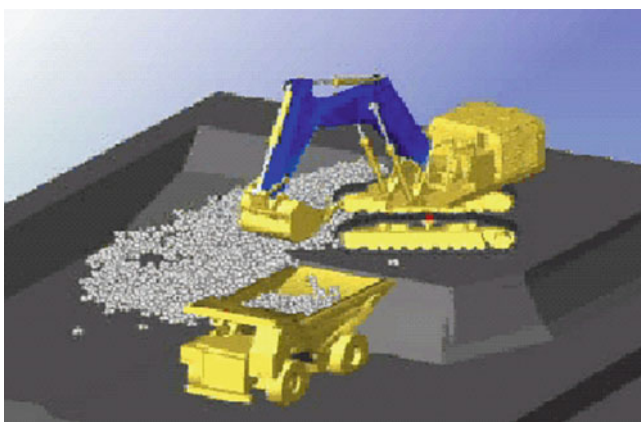
Fig. 1 Hydraulic excavator bucket loading – dumping operation (granular material) using Rocks3D TD
