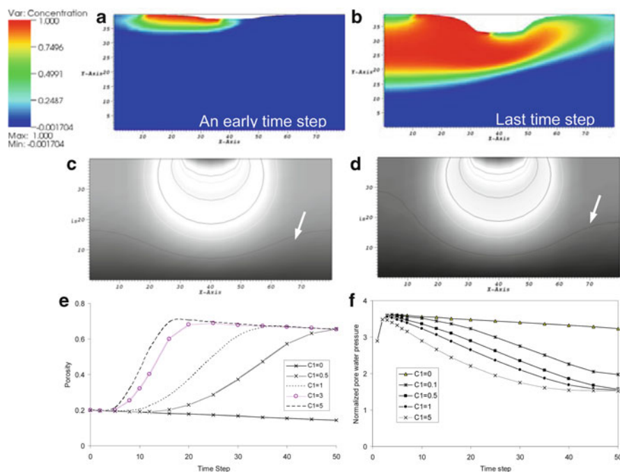
Fig. 3 (a) chemical transport in an early time step; (b) chemical transport in last time step; (c) symmetric velocity contours in the absence of chemical erosion; (d) non symmetric velocity contours in the presence of chemical erosion; (e) porosity-time graph for different concentrations; (f) variation of pore pressure with time for different concentrations
