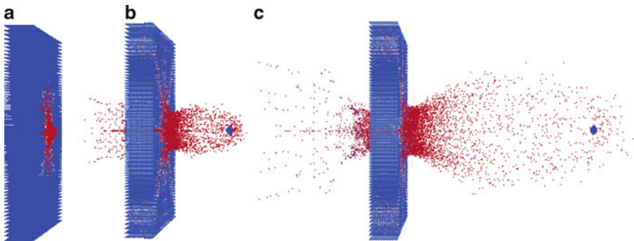
Fig. 4 Penetration process predicted by RKPM: (a) 50 \mu\text{sec} after impact, (b) 200 \mu\text{sec} after impact, (c) 500 \mu\text{sec} after impact
