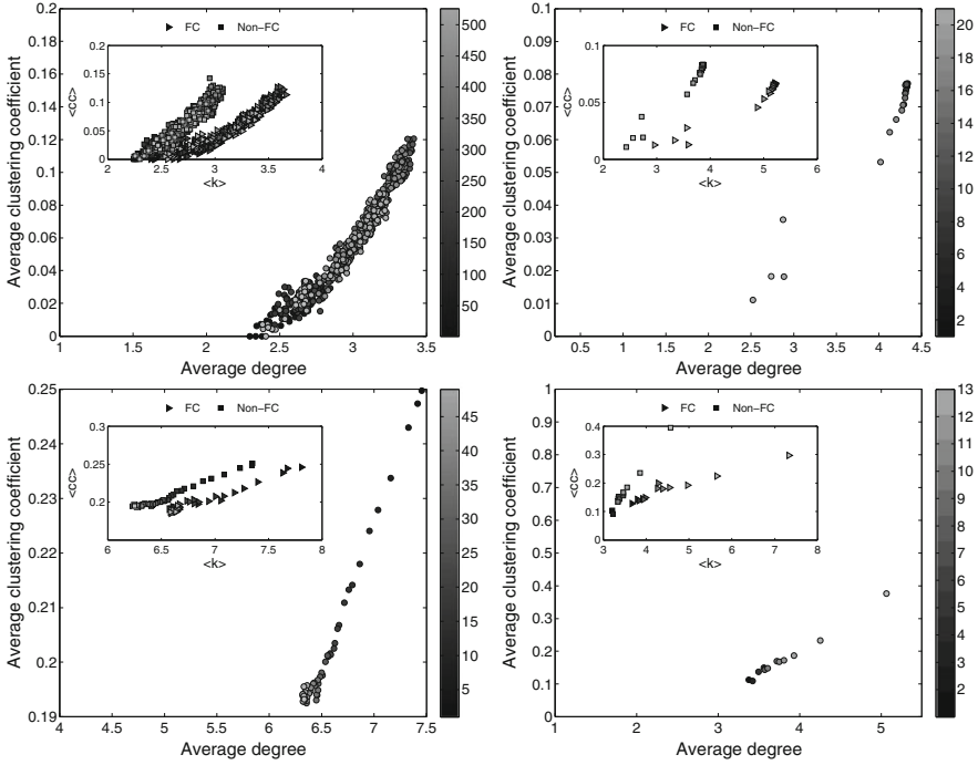
Fig. 4 Clockwise from top left , feature space by force chain: BCYS, TCP1, UCC and TCP2
