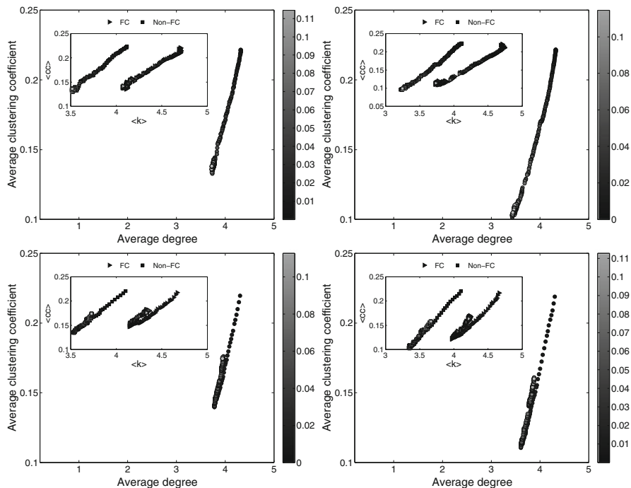
Fig. 3 Clockwise from top left , feature space by force chain: BCP1, BCP2, BCPV2 and BCPV1
