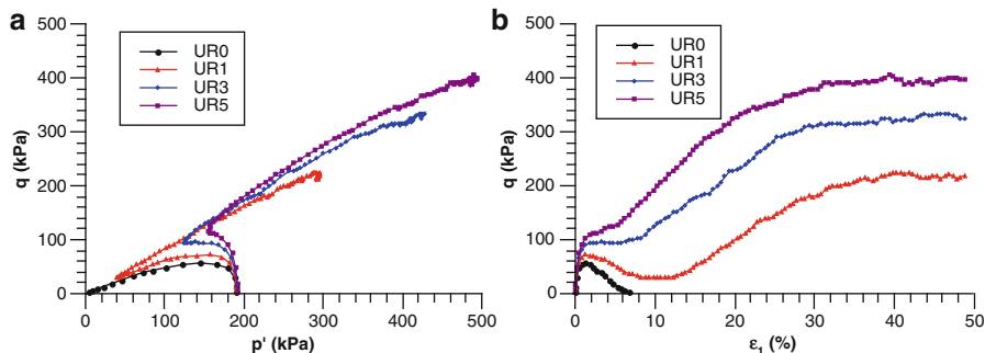
Fig. 3 Undrained behavior with rolling resistance: (a) p' - q ; (b) \epsilon_1 - q
