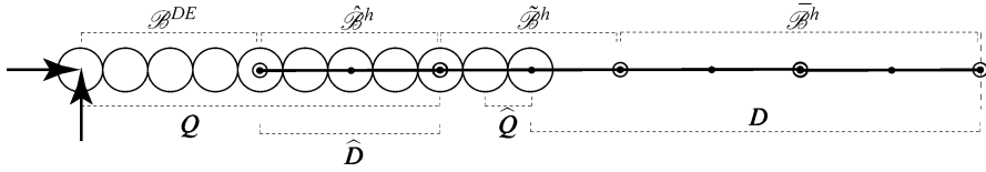
Fig. 1 1D string of 11 elastic spheres overlapped partially by 4 1D micropolar continuum FEs. Free particle dofs are indicated by \mathcal{Q} , ghost particle dofs by \hat{\mathcal{Q}} , prescribed FE nodal dofs by \hat{\mathcal{D}} , and free FE nodal dofs by \mathcal{D}
