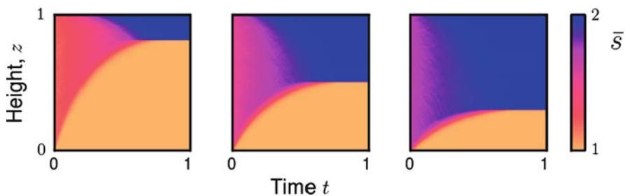
Fig. 3 Time evolution for inclined plane flow in one spatial dimension using w^{May} and \dot{\gamma} = \sqrt{H - z} . The system is initially filled with a bidisperse mixture with 30%, 50% and 80% (left to right) large concentration by volume. Colourbar represents the large particle concentration \phi
