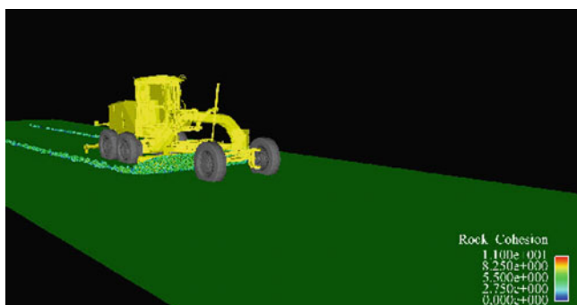
Fig. 8 Motor grader M160 dozing operation in cohesive materials using Rocks3D TD and analytic approach for the cutting edge forces
