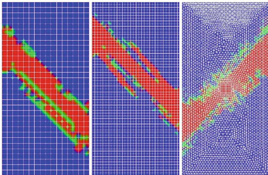
Fig. 4 Plots of instantaneous plastic state on Gauss points for the biaxial test after an axial displacement of 4 cm
