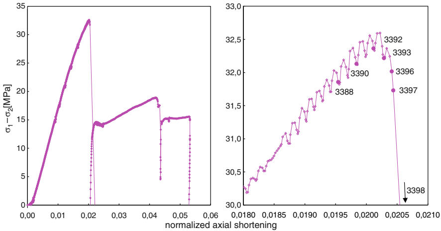
Fig. 2 Evolution of the differential stress (major stress minus minor stress) versus axial strain. At right , detail of the full curve at left , close to the stress peak. Numbers correspond to the photographs (The small oscillations of the right curve have been induced by an imperfect regulation of the axial piston pressure generator)
