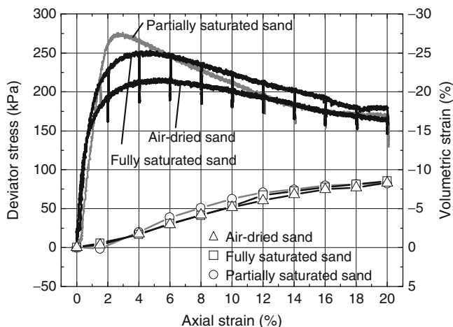
Fig. 1 Deviator stress-axial strain relations and volumetric strain-axial strain relations for triaxial compression tests on partially saturated sand, fully saturated sand, and air-dried sand (solid lines: deviator stress, open marks with lines: volumetric strain, compression is positive)
