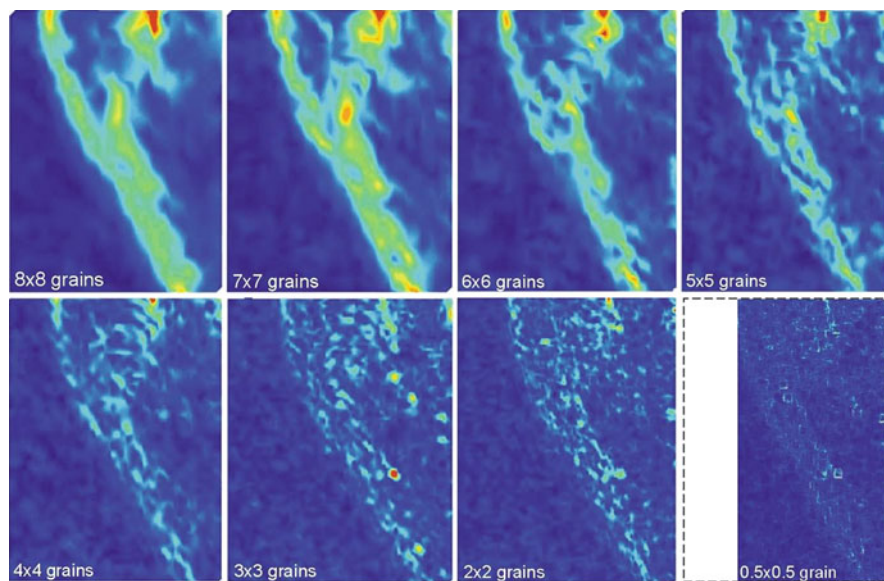
Fig. 3 An example of PIV analysis: fields of shear strains obtained for different dimensions of search patch (quoted as a number of grain diameters)
