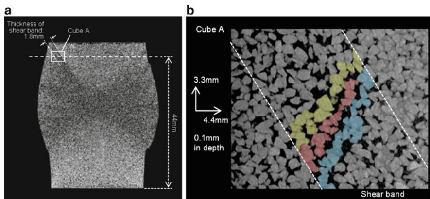
Fig. 4 Microstructure in the shear band of the partially saturated sand specimen (Case U). (a) Full CT image (F-2 vertical section), (b) Partial CT image (vertical section)
