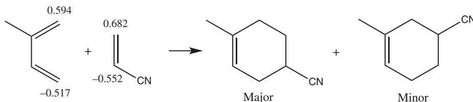
Figure 16.6 FMO rationalizes the stereochemistry of substituted Diels–Alder reactions.
