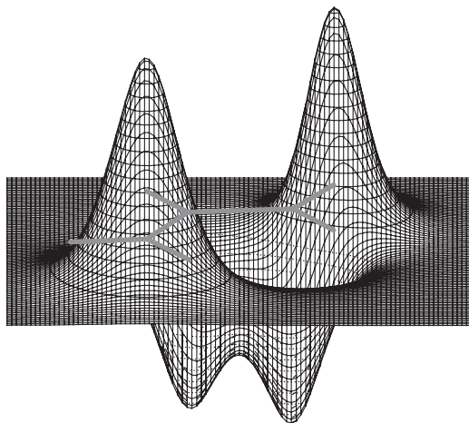
Figure 17.8 Representation of the acrolein LUMO orbital.
