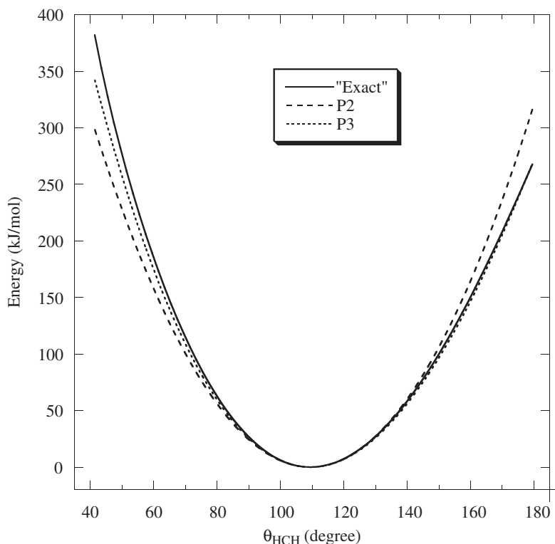
Figure 2.4 The bending energy for CH 4 .
