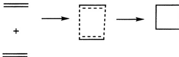
Figure 16.11 Reaction of two ethylenes to form cyclobutane under C_{2v} symmetry.
