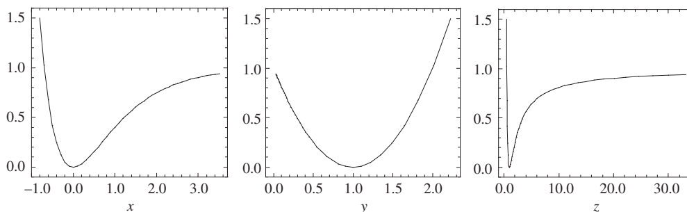
Figure 13.3 Morse curves as a function of x , y and z .
