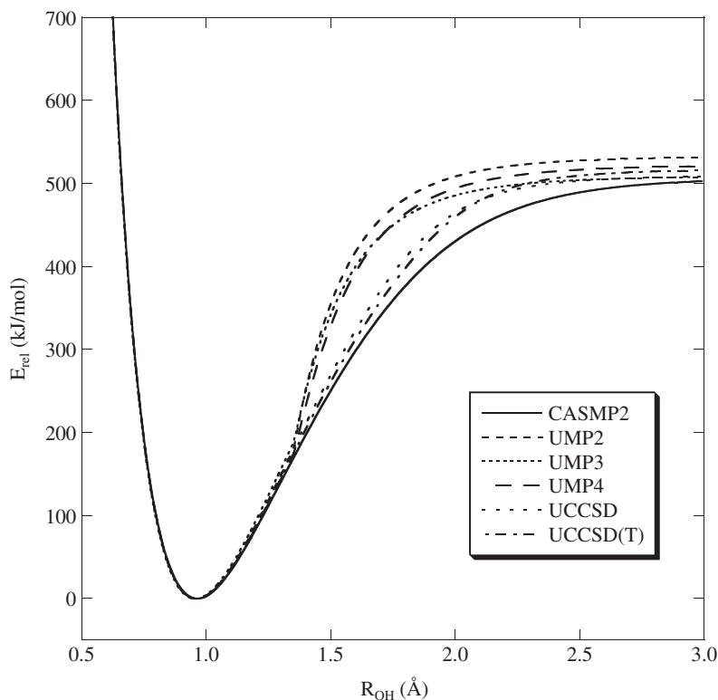
Figure 12.7 UMP2, UMP3, UMP4, UCCSD and UCCSD(T) dissociation curves for \text{H}_2\text{O} .
