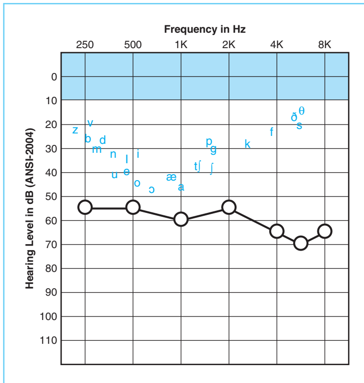
FIGURE 3-12 The inaudibility of speech sounds in the presence of a moderately severe, flat audiometric configuration.
