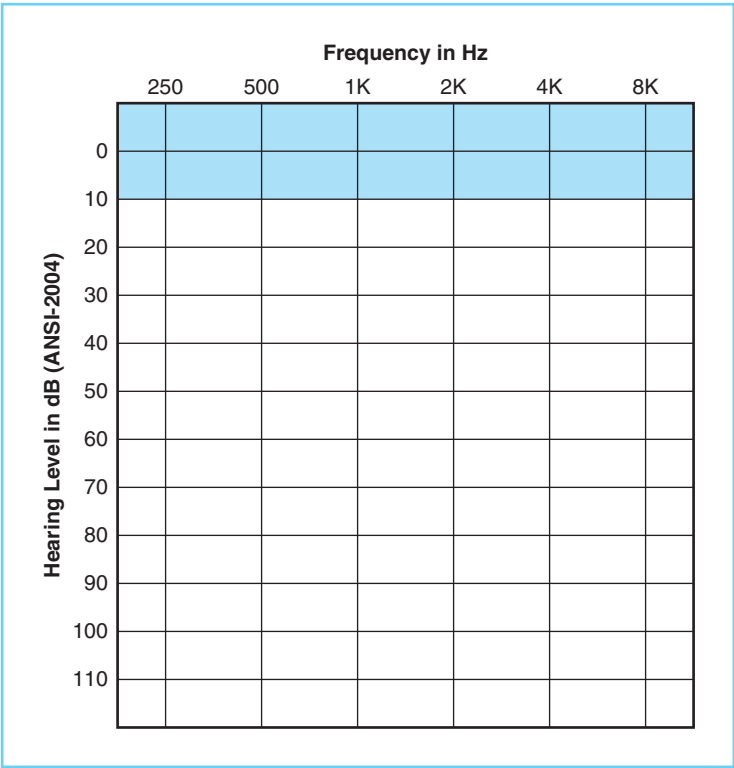
FIGURE 6-6 An audiogram, with frequency expressed in Hz plotted as a function of intensity expressed in dB HL.
