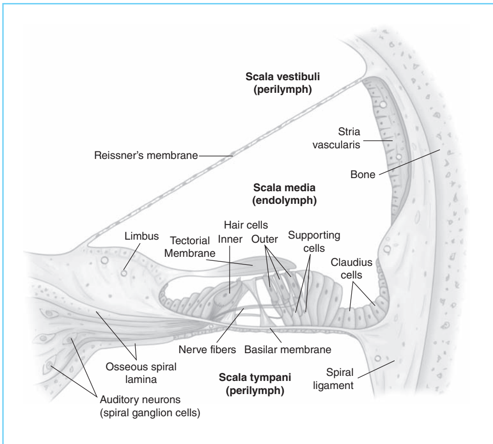
FIGURE 2-20 | The cochlear duct. (Adapted by B.A. Bohne, 2004 from Davis, H., et. al. (1953). Acoustic trauma in the guinea pig. Journal of the Acoustical Society of America , 25, 1180-1189.)
