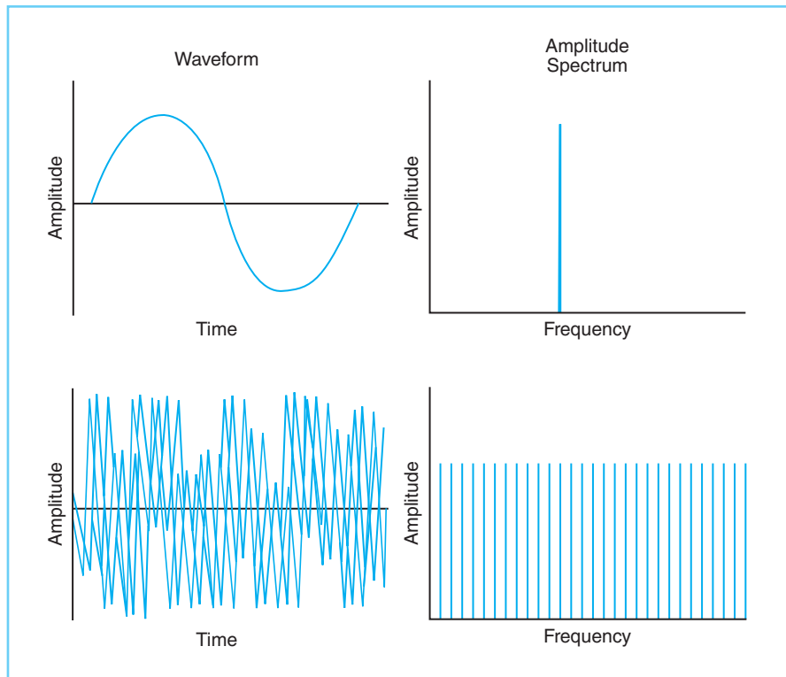
FIGURE 2-12 The spectral content of a single-frequency tone ( top ) and of a complex sound ( bottom ) are expressed as amplitude spectra, or amplitude of the individual frequency components.
