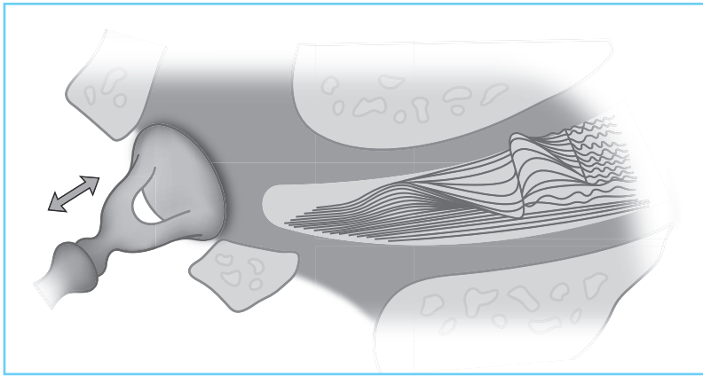
FIGURE 2-24 | Schematic drawing of the traveling wave along the cochlear partition.
