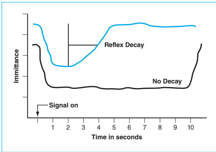
FIGURE 8-10 Examples of no acoustic reflex decay and abnormal acoustic reflex decay. Abnormal decay occurs when the amplitude of the reflex decreases to at least half of its initial maximum value.
