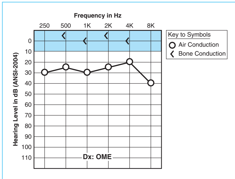
FIGURE 4-4 An audiogram representing the effects of otitis media with effusion.
