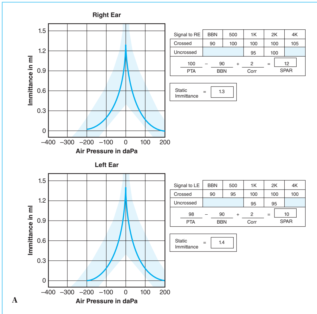
FIGURE 10-8 Hearing consultation results in a 78-year-old woman with long-standing, progressive hearing loss. Immittance measures (A) are consistent with normal middle-ear function. Pure-tone audiometric results (B) show bilateral, symmetric, moderate, sensorineural hearing loss. Speech audiometric results (C) show reduced word recognition in quiet, consistent with the degree and configuration of cochlear hearing loss. Sentence recognition in competition is substantially reduced, as is dichotic performance.
