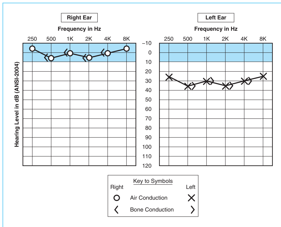
FIGURE 6-12 Audiogram representing asymmetric hearing loss.
