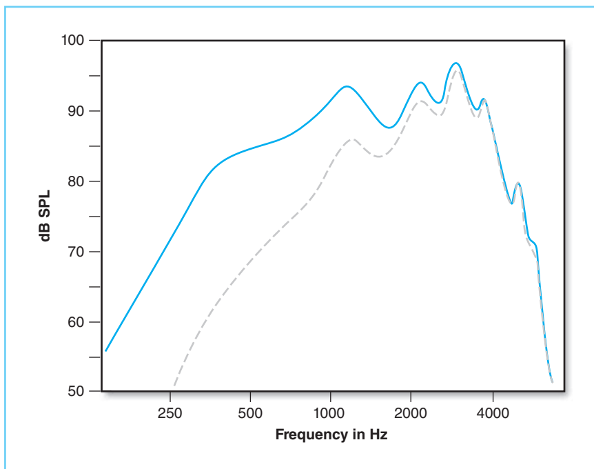
FIGURE 13-3 The effects of filtering on the frequency response of a hearing aid.
