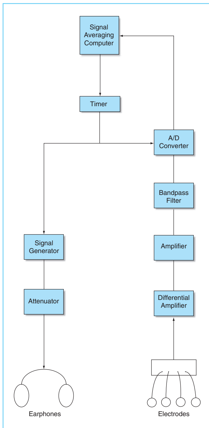
FIGURE 9-1 Schematic representation of the instrumentation used in recording auditory evoked potentials.
