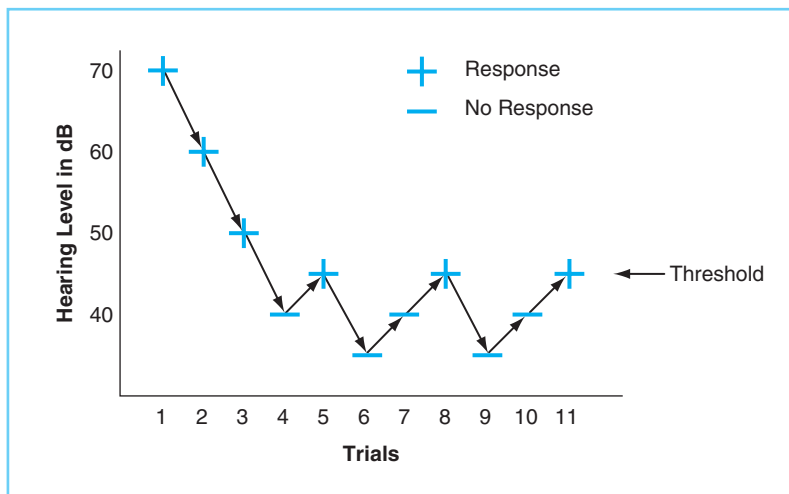
FIGURE 6-14 Schematic representation of a threshold search, showing the “down -10, up -5” strategy for bracketing hearing threshold level.
