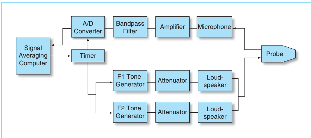
FIGURE 9-13 Schematic representation of the instrumentation used to elicit and measure distortion-product OAEs.
