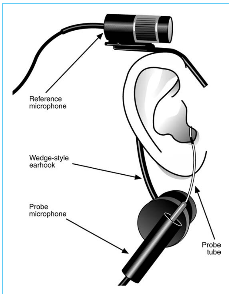
FIGURE 14-5 A probe-microphone system. (Drawing courtesy of Frye Electronics, Inc. Tigard, OR.)
