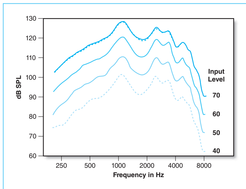
FIGURE 13-12 Frequency responses of a hearing aid to different input levels.
