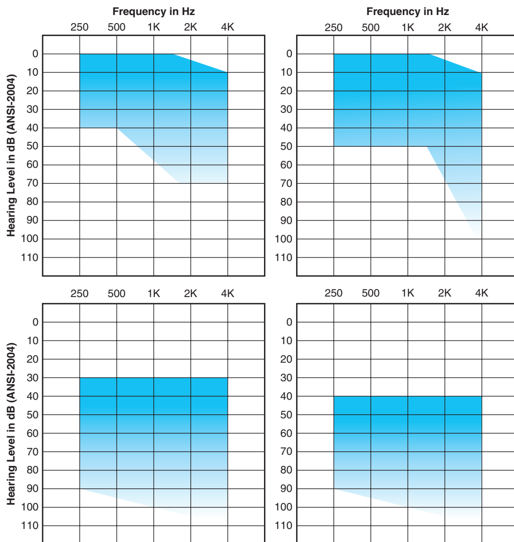
FIGURE 13-8 An example of a fitting range for four different hearing aids, ranging from a mild-gain to a power hearing device.
