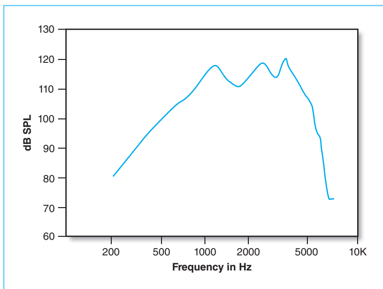
FIGURE 13-10 Frequency response of a hearing aid.
