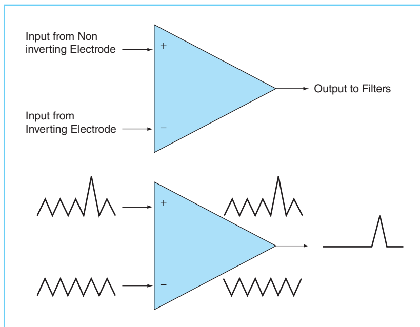
FIGURE 9-2 Schematic representation of the process of common-mode rejection. Activity that is identical or common to both electrodes is eliminated by inverting the input from one electrode and subtracting it from the input to the other.
