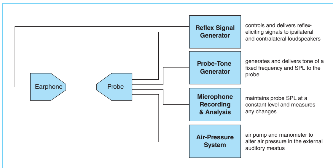
FIGURE 8-1 Schematic representation of the instrumentation used in immittance measurement.
