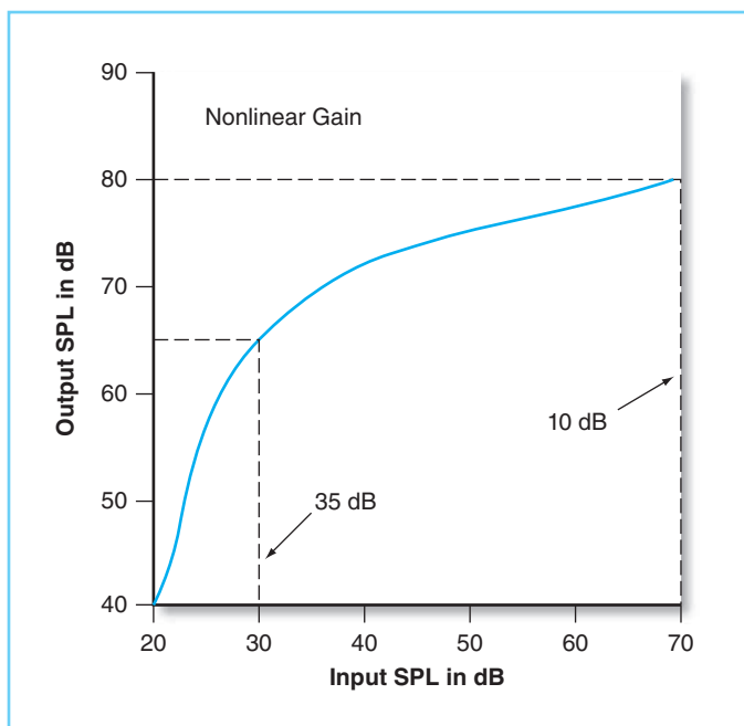
FIGURE 13-5 The relationship of sound input to output in a nonlinear hearing aid circuit. Amount of gain changes as a function of input level.
