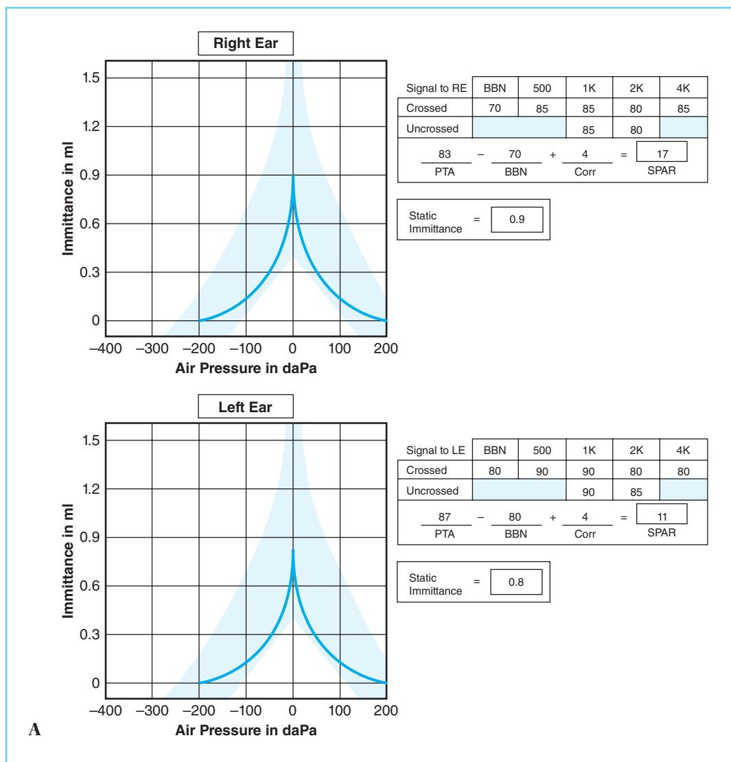
FIGURE 10-4 Hearing consultation results in a 45-year-old woman with hearing loss secondary to endolymphatic hydrops. Immittance measures (A) are consistent with normal middle-ear function. SPARs predict the presence of hearing loss in the left ear. Pure-tone audiometric results (B) show normal hearing sensitivity on the right and a moderate, rising sensorineural hearing loss on the left. Speech audiometric results show that speech-recognition ability on the left ear is poorer than would be predicted from the degree and configuration of hearing loss. Auditory brainstem response results (C) show that both the absolute and interpeak latencies are normal and symmetric, consistent with normal VIIIth nerve and auditory brainstem function.
