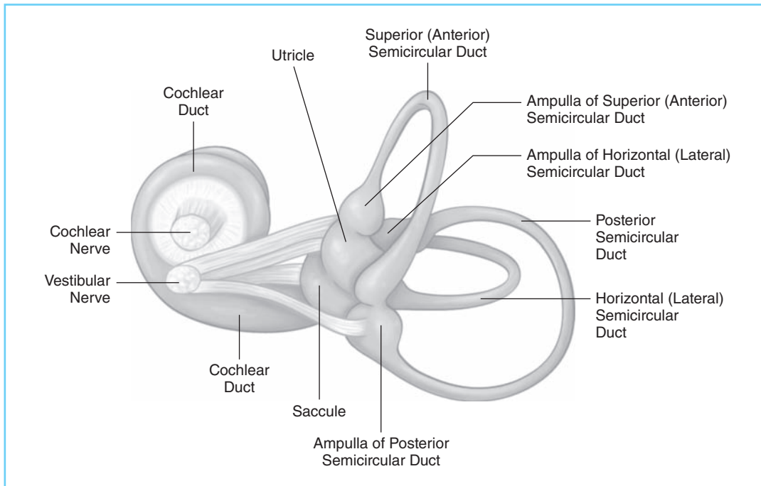
FIGURE 2-28 The vestibular labyrinth.
