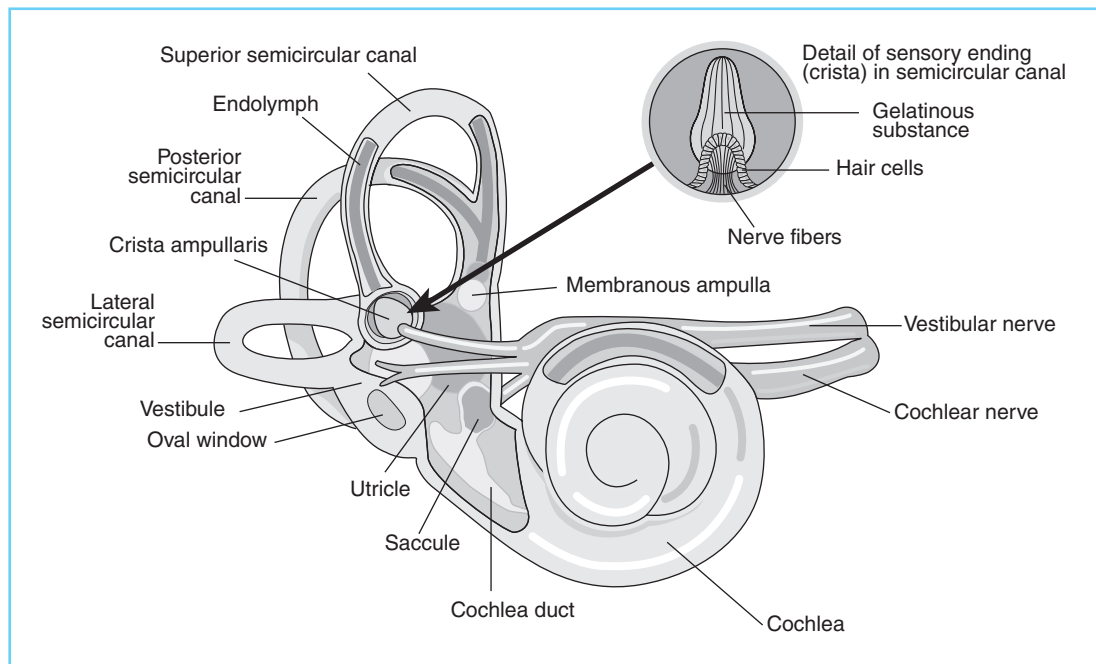
FIGURE 2-18 | The membranous labyrinth.
