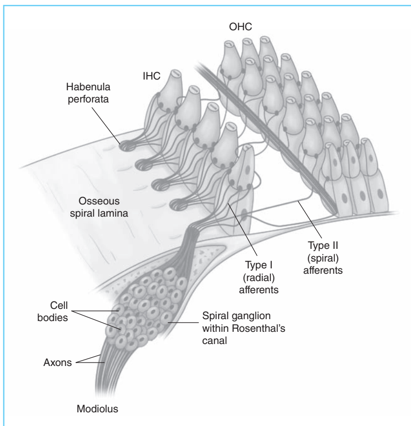
FIGURE 2-26 | The departure of afferent neurons from the inner and outer hair cells (IHC and OHC).
