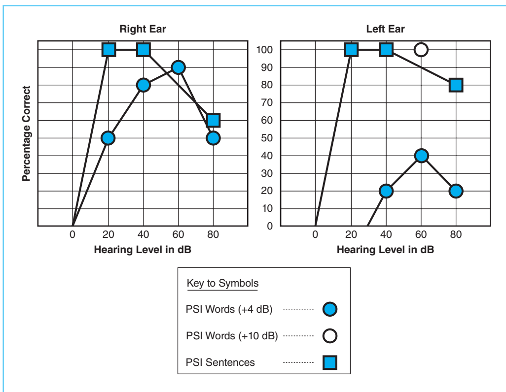
FIGURE 10-13 Speech audiometric results in a young child with auditory processing disorder. Results of the Pediatric Speech Intelligibility (PSI) test illustrate how assessment procedures can be used to control for nonauditory influences on test interpretation.
