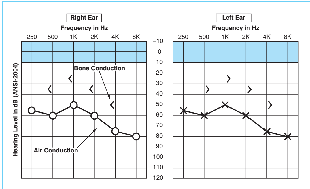
FIGURE 6-8 Right and left ear audiograms with unmasked air-conduction and bone-conduction thresholds.
