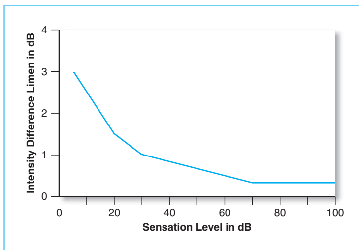
FIGURE 2-40 Generalized drawing of the relationship between intensity of a signal and difference limen for intensity.
