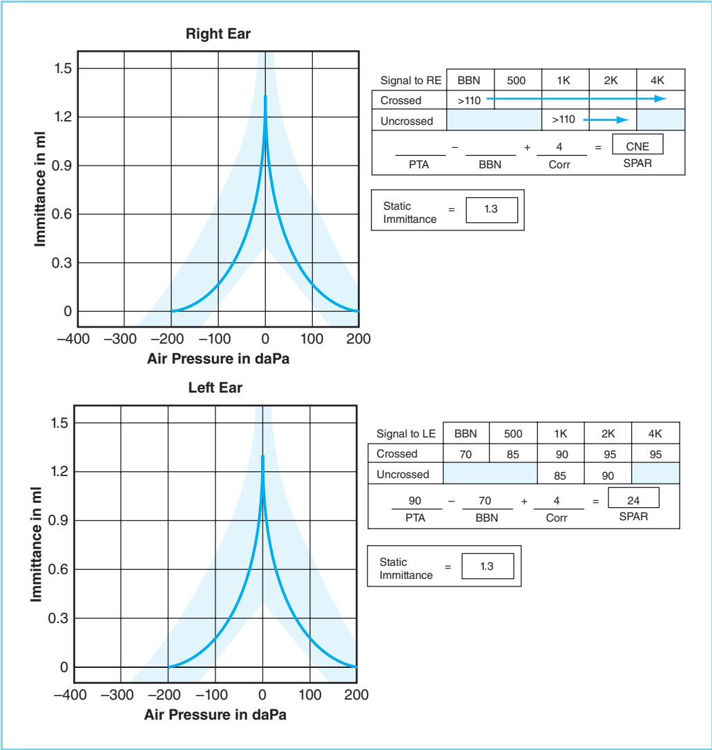
FIGURE 8-22 Immittance results consistent with normal middle-ear function and a right afferent acoustic reflex abnormality resulting from a right acoustic tumor.
