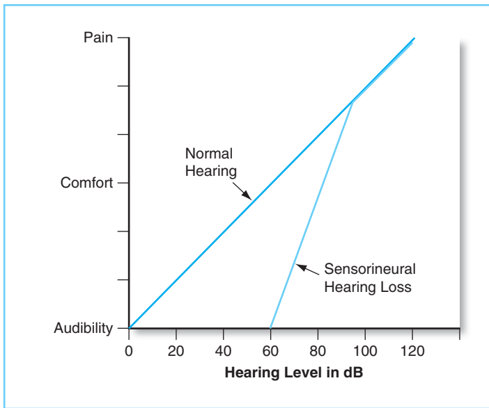
FIGURE 3-4 Generalized drawing of the relationship of loudness and intensity level in normal hearing and in sensorineural hearing loss.
