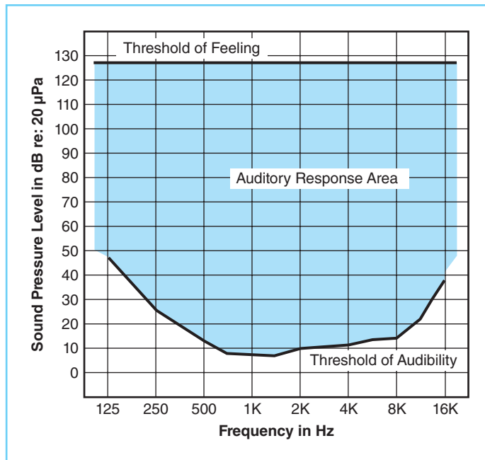
FIGURE 2-31 Auditory response area from the threshold of audibility to the threshold of feeling across the frequency range that encompasses most of human hearing.
