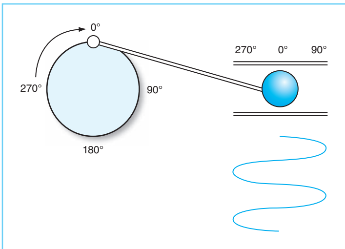
FIGURE 2-10 Schematic of the relationship between circular motion and the back and forth movement of an air molecule. Movement of the molecule results in sinusoidal motion.
