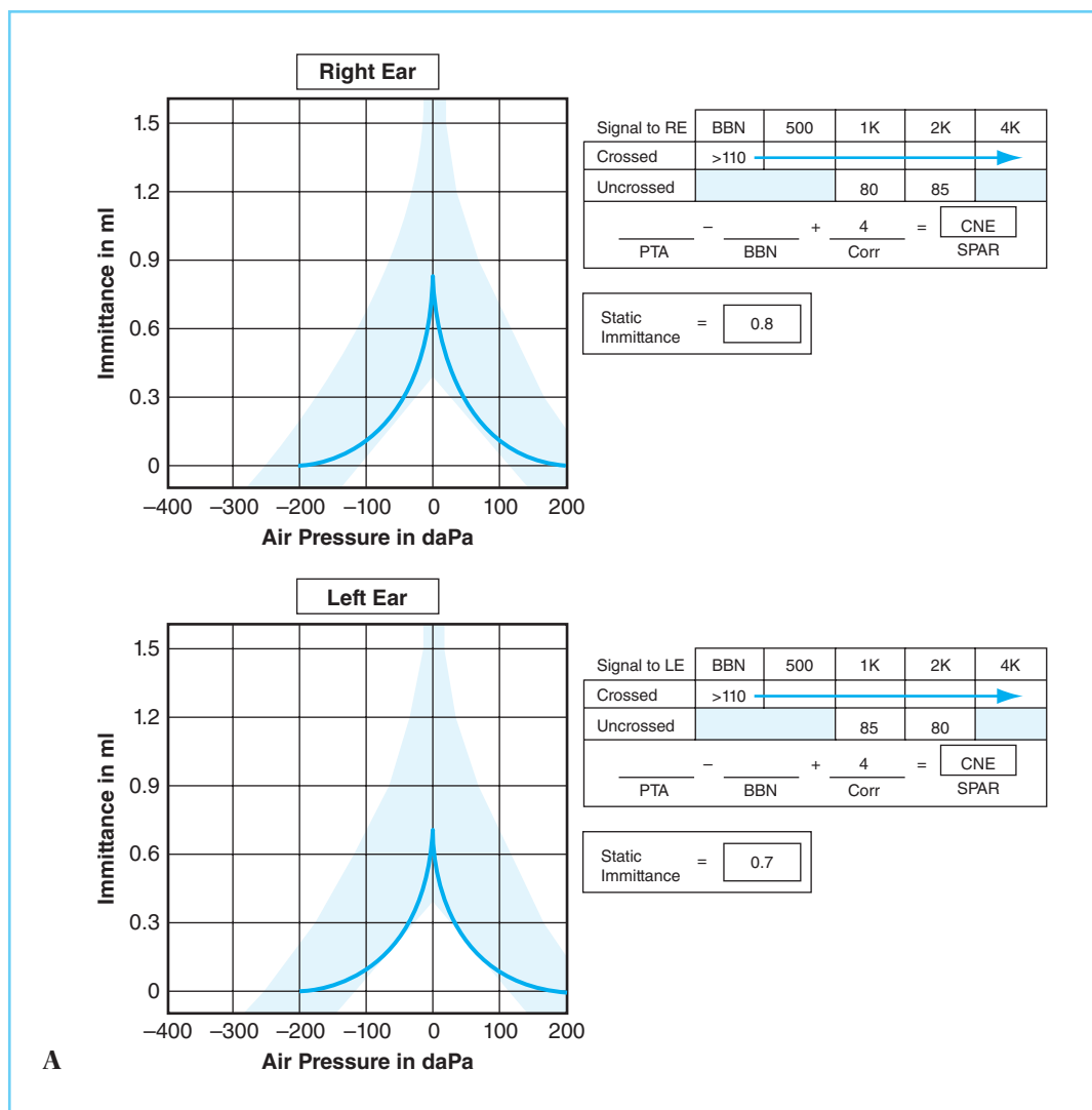
FIGURE 10-6 Hearing consultation results in a 34-year-old woman with multiple sclerosis. Immittance measures (A) are consistent with normal middle-ear function. However, left crossed and right crossed reflexes are absent, consistent with brainstem disorder. Pure-tone audiometric results (B) show mild low-frequency sensorineural hearing loss bilaterally. Speech audiometric results (C) show that word recognition in quiet is normal, but sentence recognition in competition is abnormal. Auditory brainstem response results (D) show no identifiable waves beyond Wave I on the left and significant prolongation of the Wave I-V interpeak interval on the right.
