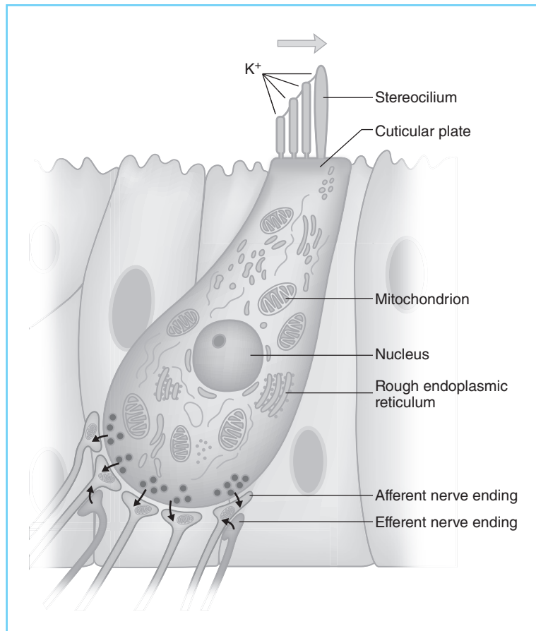
FIGURE 2-23 | Diagram of a single inner hair cell.
