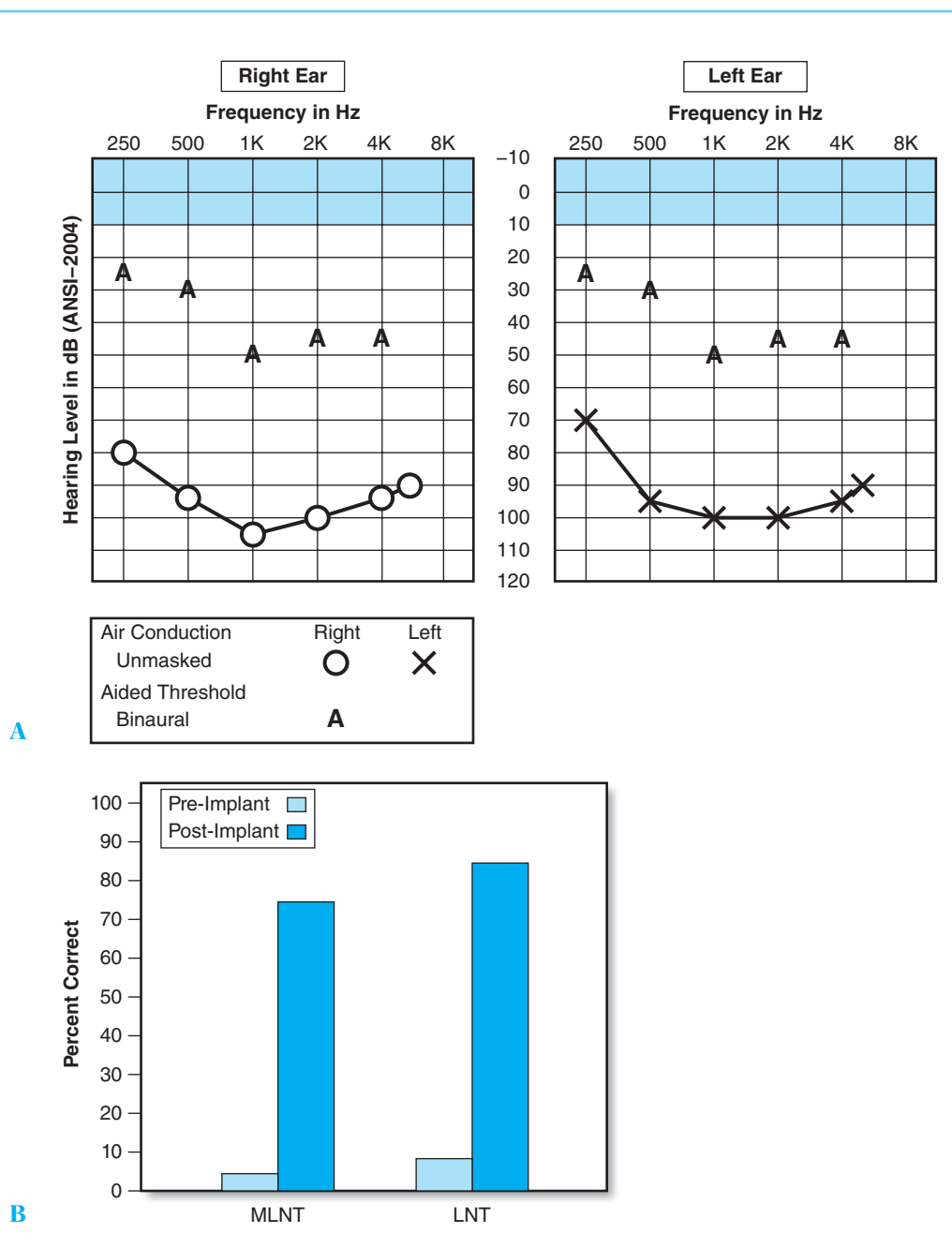
FIGURE 15-8 Hearing consultation results in a 6-year-old child with severe-to-profound sensorineural hearing loss. Pure-tone audiometric results (A) show bilateral hearing loss. Aided thresholds are with binaural hearing aids. Pre- and post-implant results (B) show substantial improvement and in performance on selected speech-recognition measures.
