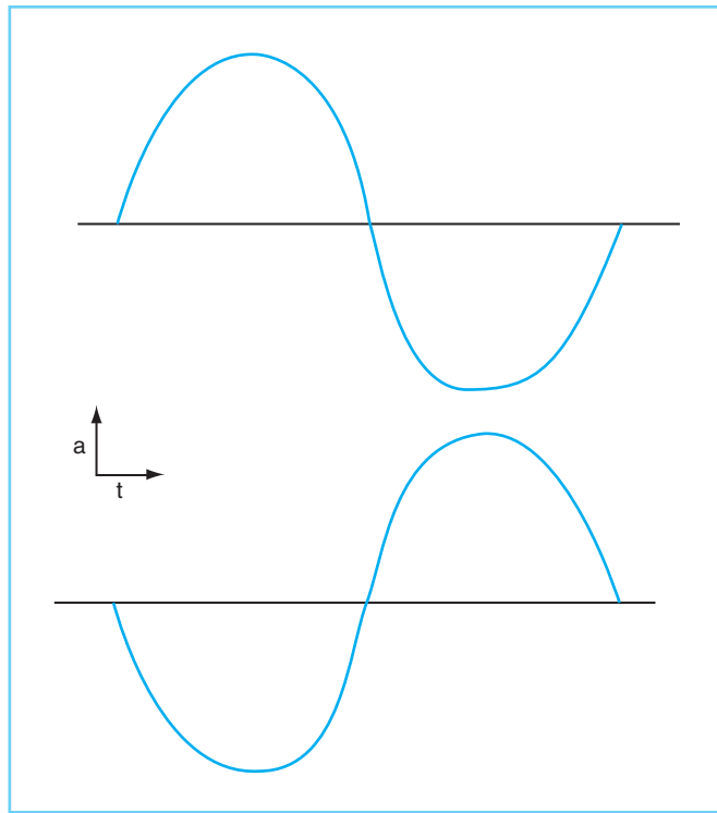
FIGURE 2-11 Two waveforms that are identical in amplitude ( a ) and frequency but vary in starting phase.
