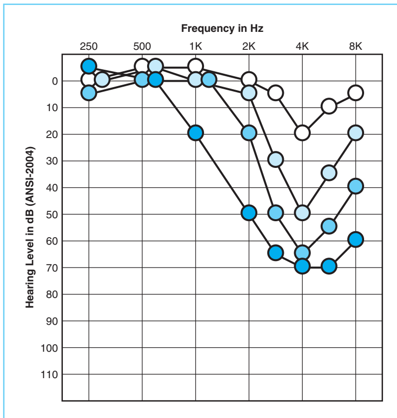
FIGURE 4-11 The progression of hearing loss from industrial noise exposure over a period of four decades.
