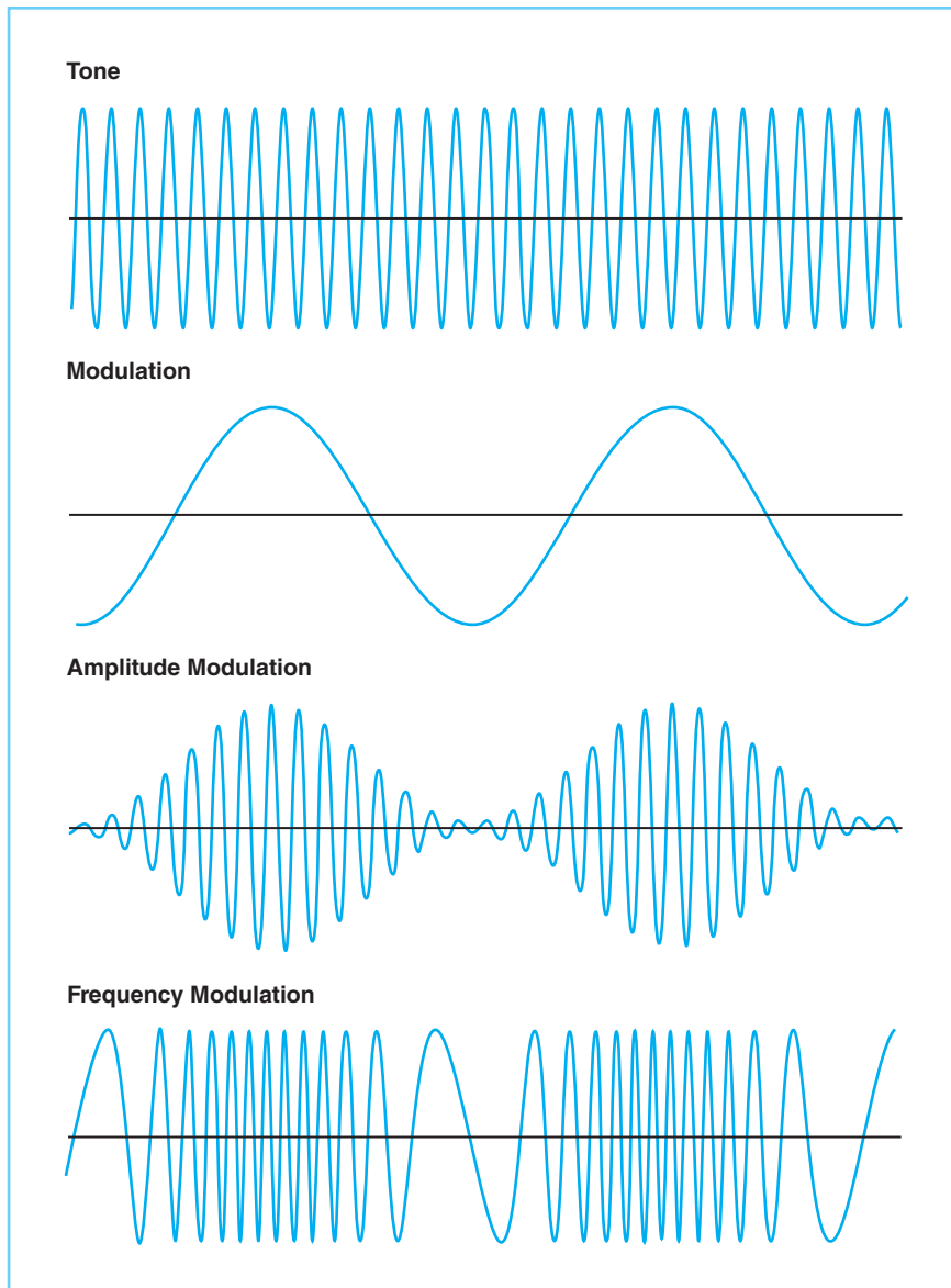
FIGURE 9-6 Schematic representation of modulation. A carrier tone is modulated in both the amplitude and frequency domain at a rate determined by the modulation frequency.
