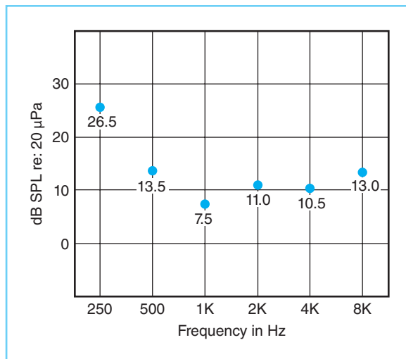
FIGURE 2-32 The designation of audiometric zero as different sound pressure levels across the frequency range.
