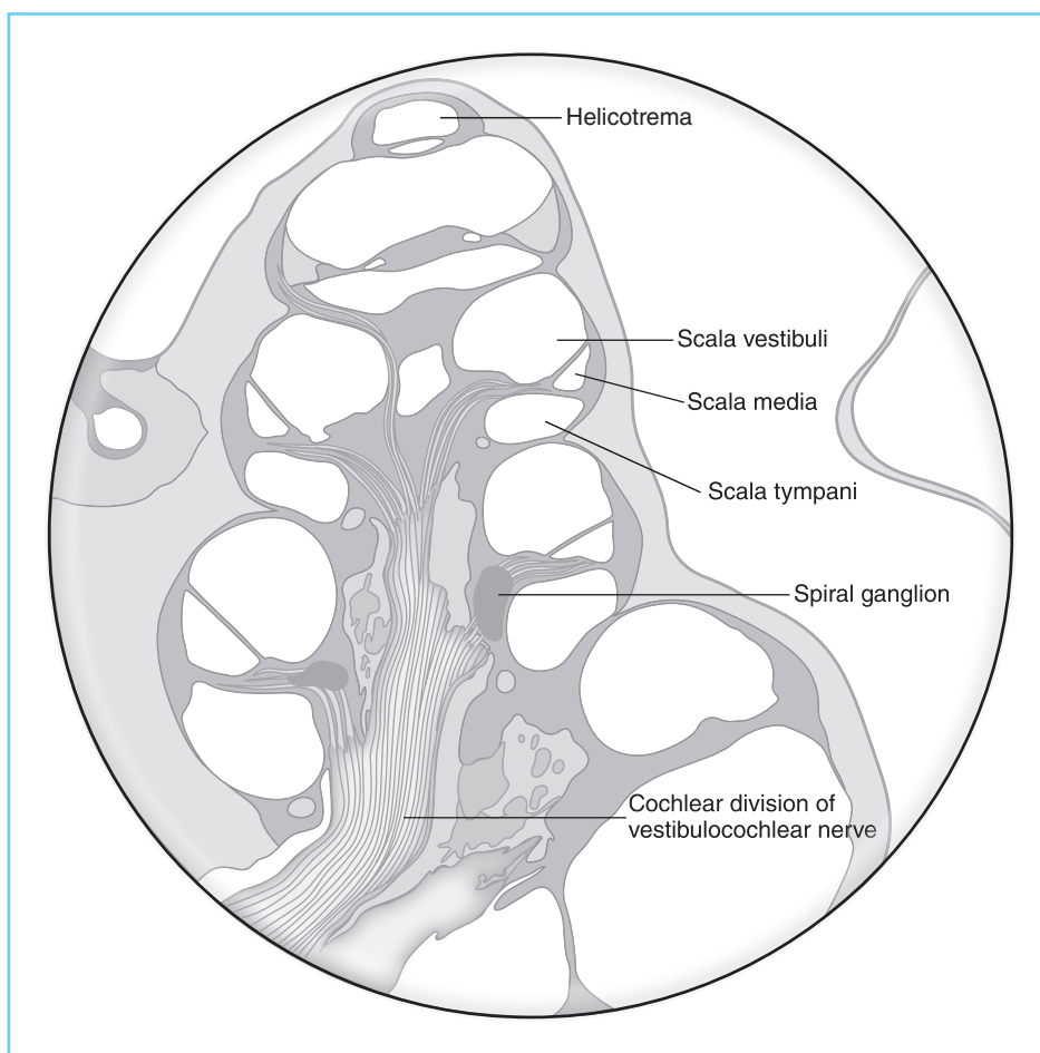
FIGURE 2-17 A section through the center of the cochlea, illustrating the bony labyrinth.
