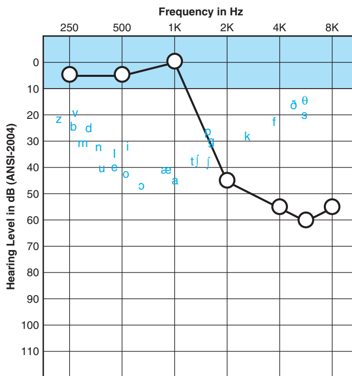
FIGURE 3-13 The selective audibility of speech sounds in the presence of a moderate, high-frequency audiometric configuration.
