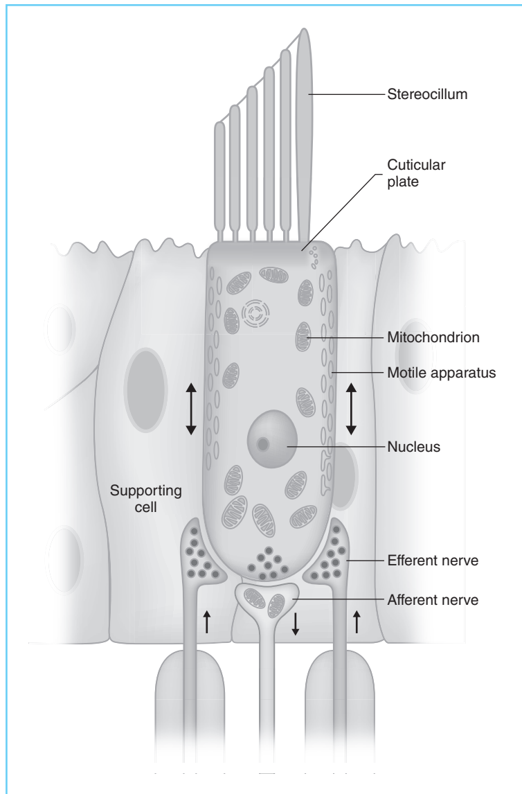
FIGURE 2-22 | Diagram of a single outer hair cell.
