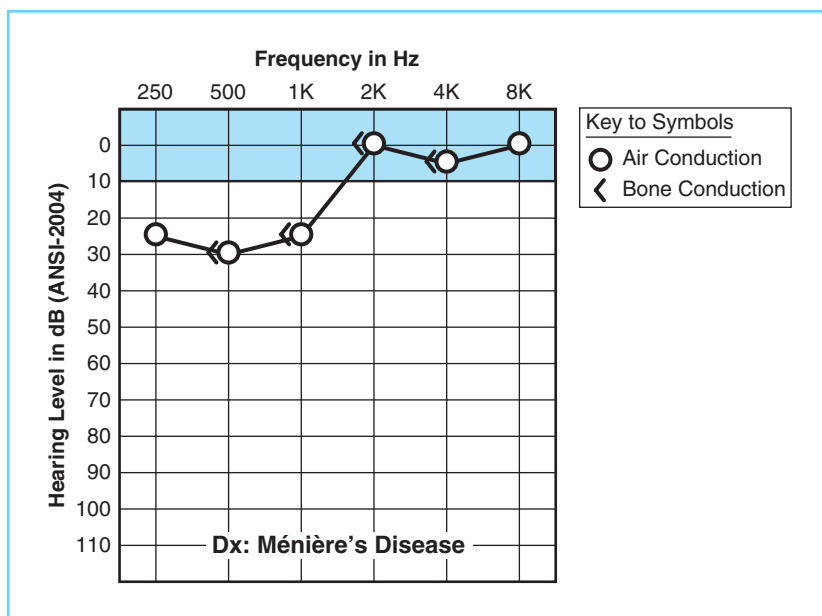
FIGURE 4-16 An audiogram representing the effects of the early stages of Ménière's disease.
