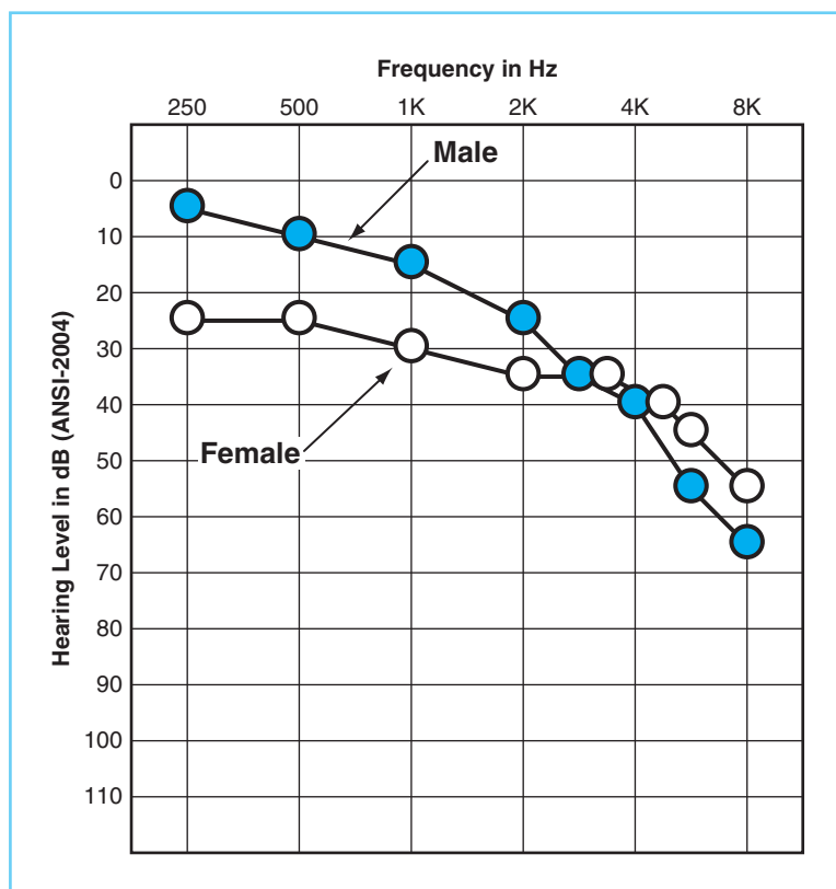
FIGURE 4-19 Generalized representation of the difference in the audiometric configurations of males and females as they age.
