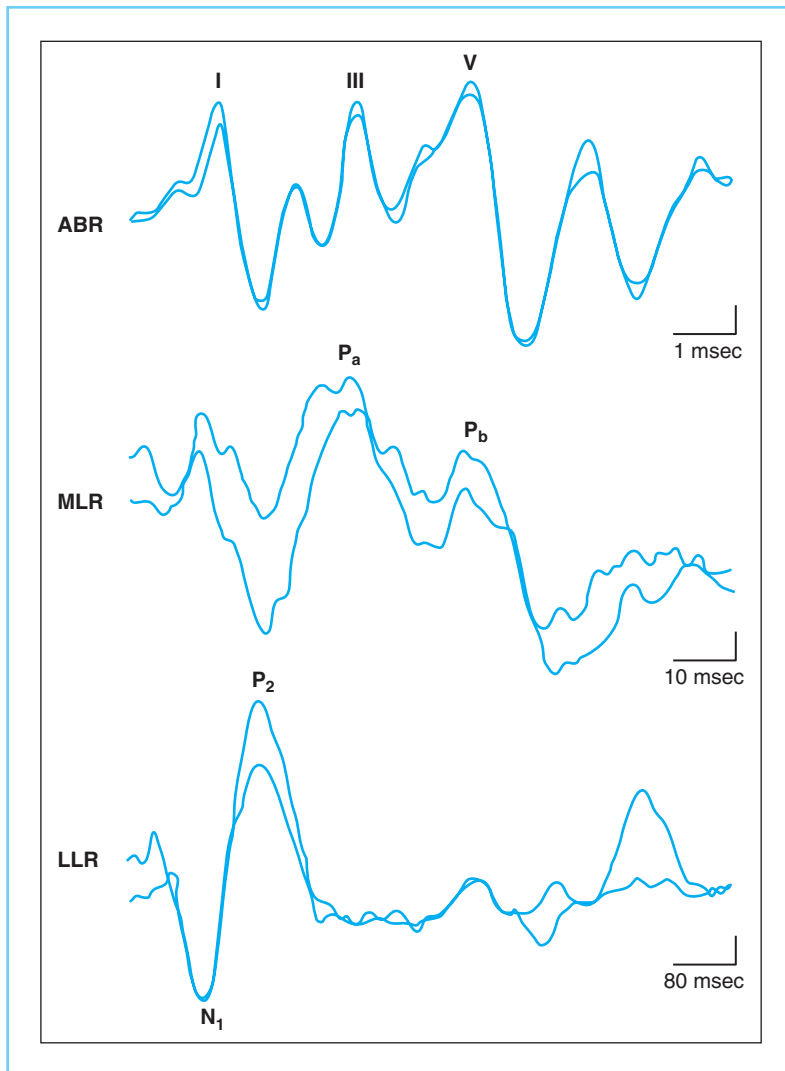
FIGURE 9-5 Normal auditory brainstem response (ABR), middle latency response (MLR), and late latency response (LLR) waveforms.
