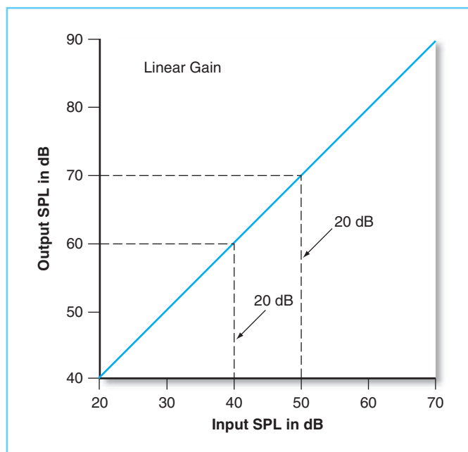
FIGURE 13-4 The relationship of sound input to output in a linear hearing aid circuit. Gain remains at a constant 20 dB, regardless of input level.
