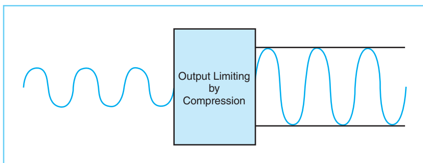
FIGURE 13-7 Schematic representation of output limiting by compression.
