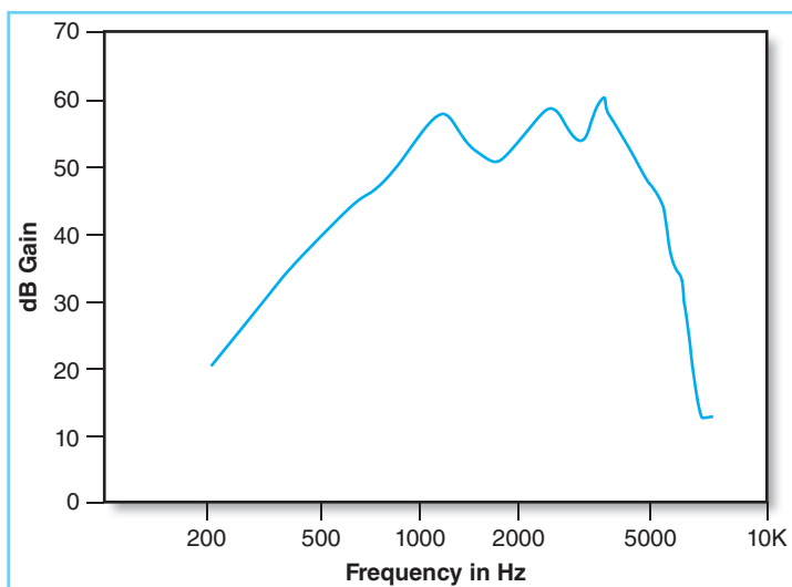
FIGURE 13-11 Frequency gain response of a hearing aid.
