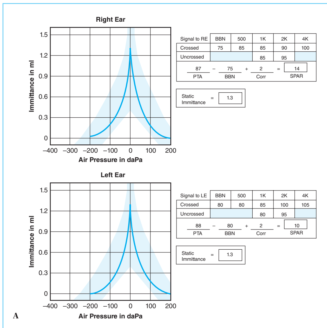
FIGURE 10-7 Hearing consultation results in a 54-year-old man with noise-induced hearing loss. Immittance measures (A) are consistent with normal middle-ear function. Pure-tone audiometric results (B) show high-frequency sensorineural hearing loss bilaterally, greatest at 4000 Hz. Speech audiometric results are consistent with the degree and configuration of cochlear hearing loss.
