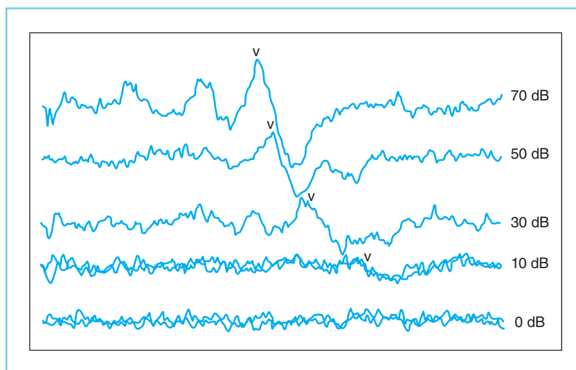
FIGURE 9-7 The prediction of hearing sensitivity with the ABR, showing the tracking of wave V as click intensity level is reduced.
