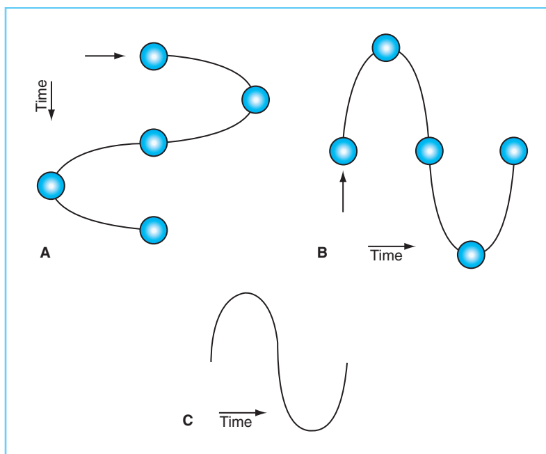
FIGURE 2-3 The back and forth movement of an air molecule over time can be represented as harmonic or sinusoidal motion. In A, the particle is set into motion by sound vibration, and its course is traced over time. The graph is replotted in B to show time along the x-axis. The line in C is a sinusoid that describes the movement.
