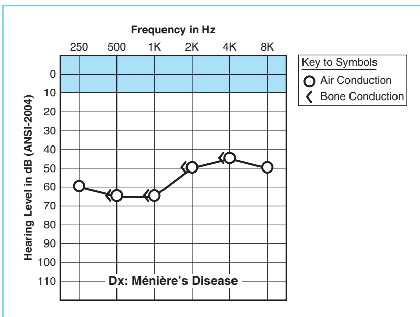
FIGURE 4-17 An audiogram representing the effects of Ménière's disease that has progressed.
