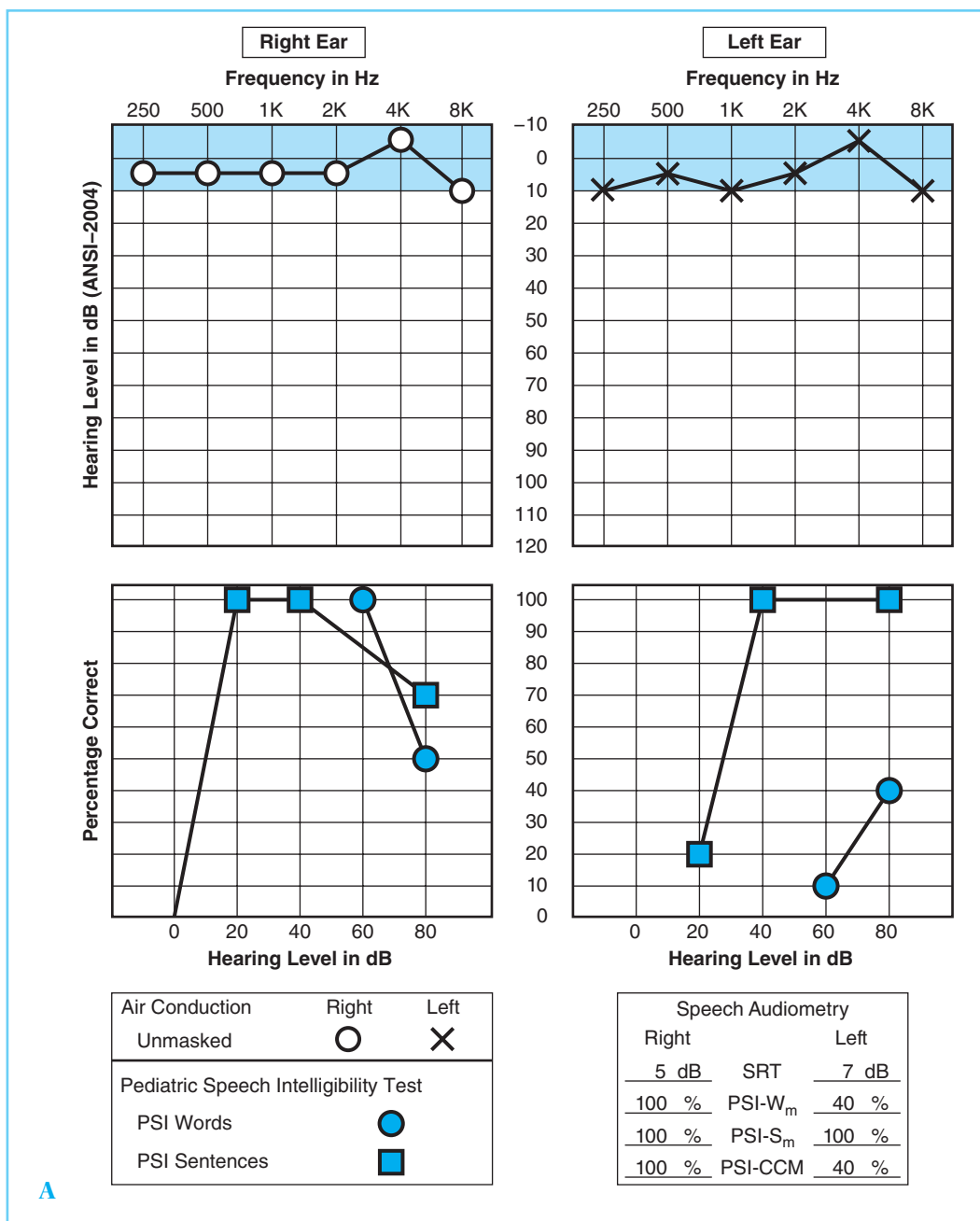
FIGURE 15-4 Hearing consultation results in a 6-year-old child with auditory processing disorder. Pure-tone and speech audiometric results (A) show normal hearing sensitivity and abnormal speech-recognition ability. Aided results (B) show good speech-recognition performance with an FM system in a soundfield.
