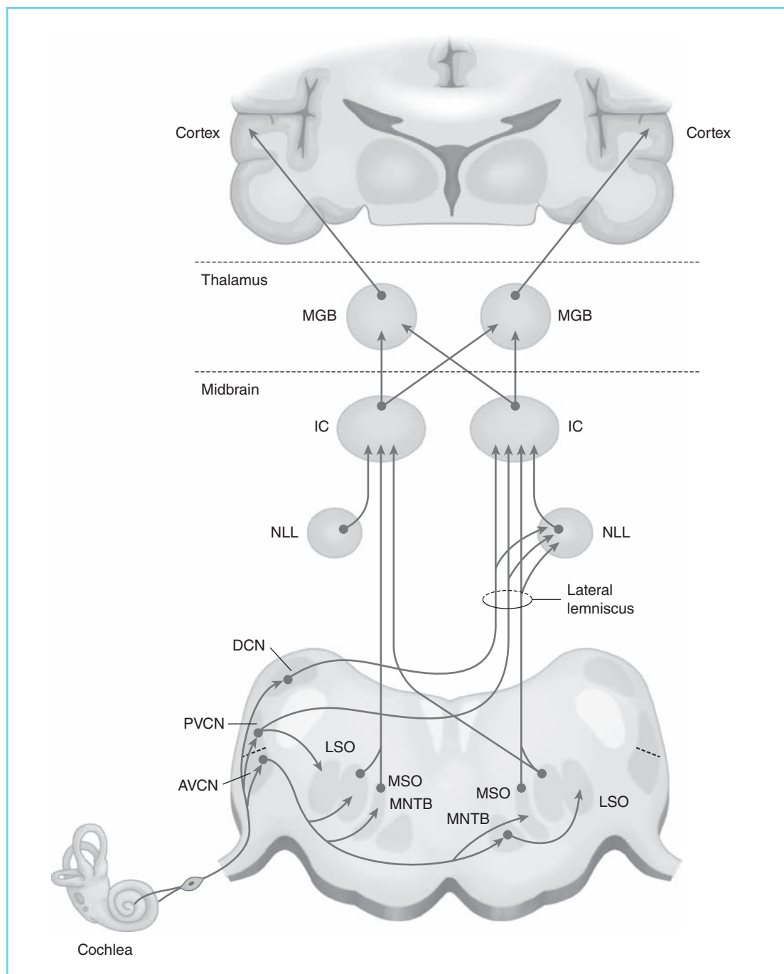
FIGURE 2-27 The central auditory nervous system. (Adapted from Pickles, J.O. (1982). Introduction to the physiology of hearing . New York: Academic Press.)
