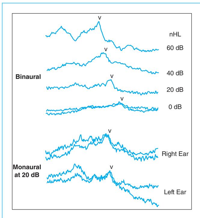
FIGURE 9-8 An example of the binaural approach to ABR prediction of hearing sensitivity.
