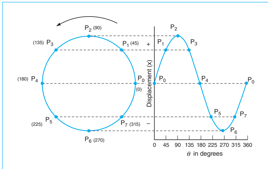
FIGURE 2-9 Schematic representation of a turning wheel undergoing simple harmonic motion. Points on the wheel are projected on a sinusoidal function, showing the magnitude of displacement corresponding to the angle of rotation and expressed in degrees of a circle.
