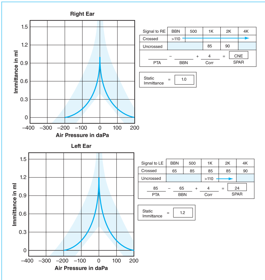
FIGURE 8-23 Immittance results consistent with a left efferent acoustic reflex abnormality, resulting from a left facial nerve paralysis of unknown cause.
