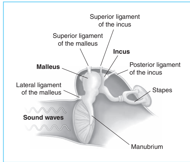
FIGURE 2-16 | The ossicular chain.
