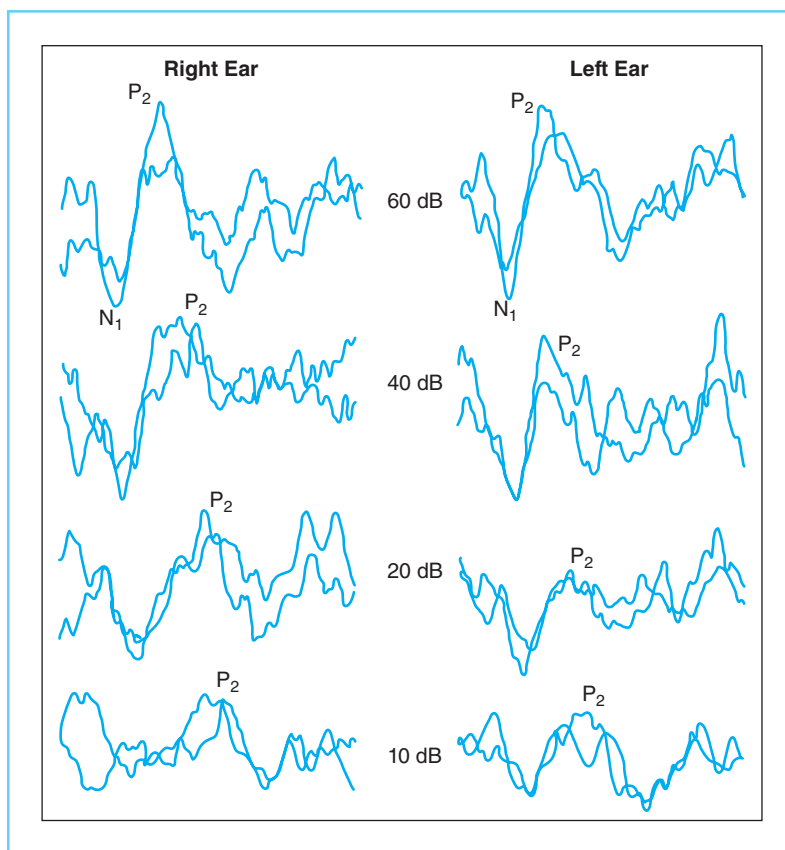
FIGURE 9-10 The prediction of hearing sensitivity with the late latency auditory evoked potential, showing the tracking of the N1/P2 component as intensity of a 500 Hz tone is reduced.
