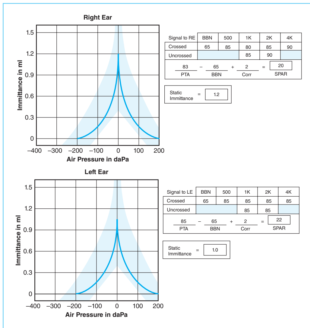
FIGURE 8-20 Immittance results, with SPARs predicting normal hearing sensitivity, from a patient who was feigning a right-ear hearing loss.
