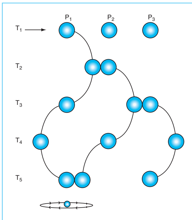
FIGURE 2-1 Schematic representation of the motion of particles in a medium over time ( T ). Here, a sound wave, designated by an arrow, moves particle P_1 into its neighbor, P_2 . Due to elasticity, P_1 moves back to its original position after displacement, and P_2 continues the energy transfer by moving into P_3 . The small inset shows the displacement of a single particle. The lines connecting particles trace the movement over time.
