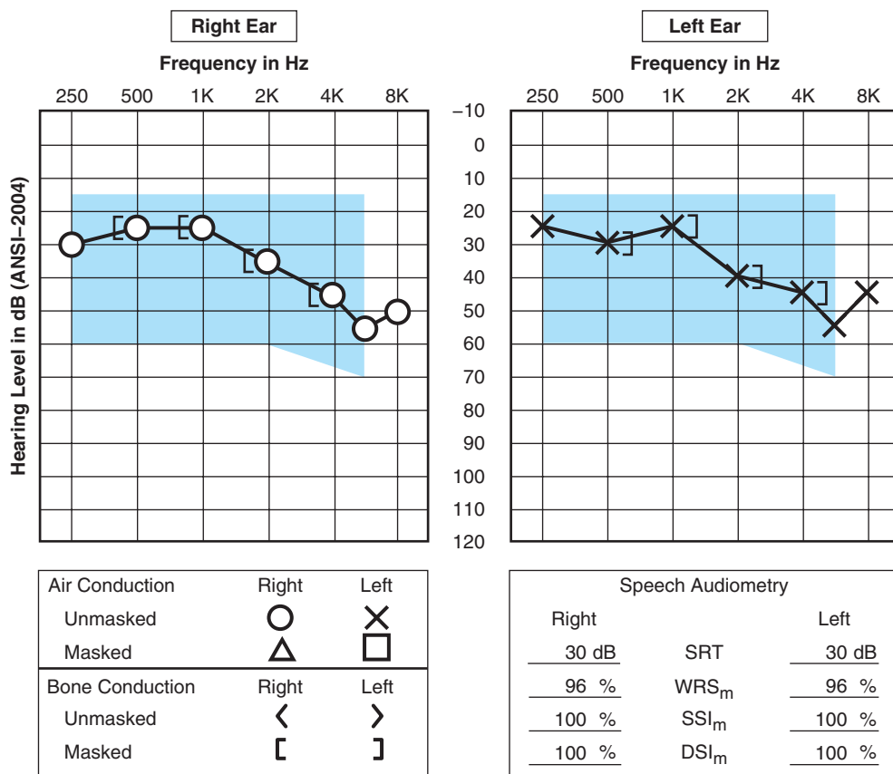
FIGURE 15-1 Hearing and hearing-aid consultation results in a 54-year-old man with bilateral sensorineural hearing loss. Pure-tone thresholds (A) are superimposed on the fitting range of the selected hearing aids. Probe-microphone measurements (B) from the right ear are compared to the targeted frequency gain.
