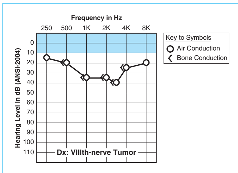
FIGURE 4-23 An audiogram representing the effects of an acoustic or VIIIth-nerve tumor.
