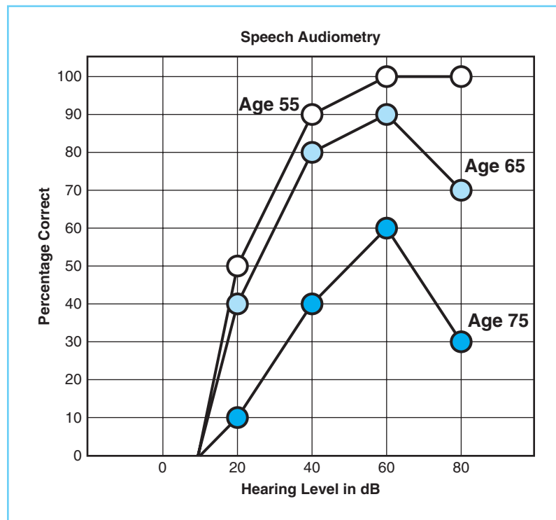
FIGURE 4-20 Decline with age in the ability to recognize speech in a background of competition.
