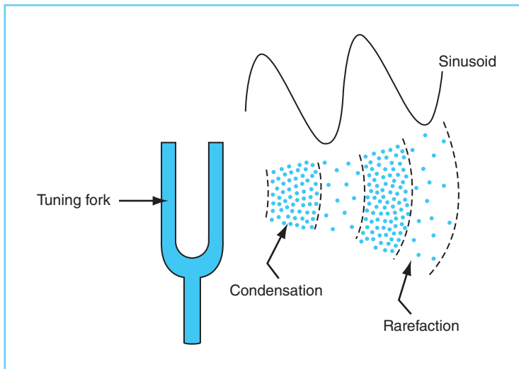
FIGURE 2-4 The relation between condensation and rarefaction waves and the sinusoidal function.
