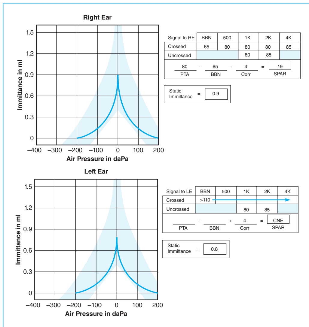
FIGURE 8-24 Immittance results consistent with a central pathway abnormality, resulting from brainstem disorder secondary to multiple sclerosis.
