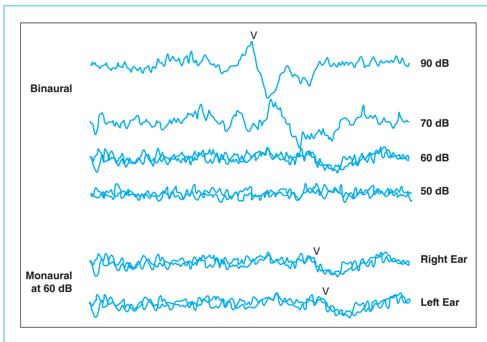
FIGURE 10-9 Results of ABR threshold assessment in a newborn who failed an AABR screening. ABRs were recorded down to 60 dB in both ears, consistent with a moderate sensorineural hearing loss.
