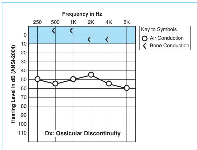
FIGURE 4-8 An audiogram representing the effects of a disarticulated ossicular chain.
