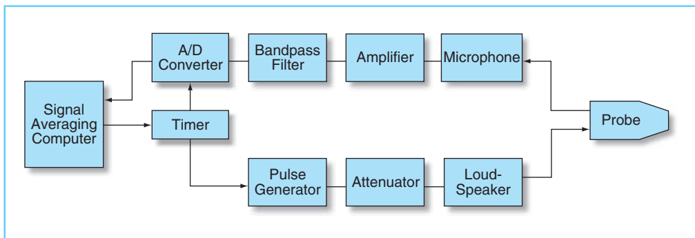
FIGURE 9-11 Schematic representation of the instrumentation used to elicit and measure transient-evoked OAEs.
