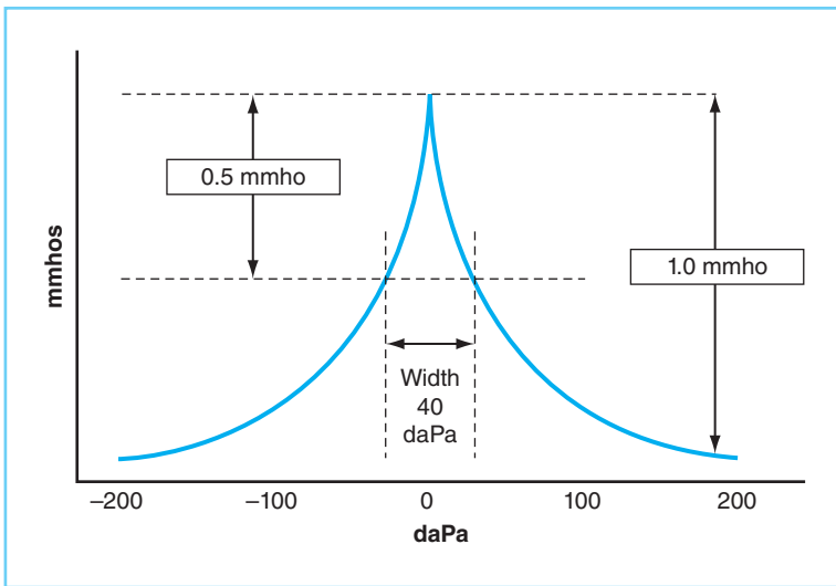
FIGURE 8-7 Illustration of the measurement of tympanogram width. Width is calculated by determining the daPa corresponding to 50% of the peak status immittance.
