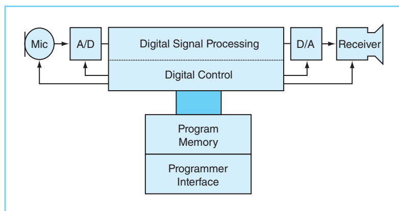
FIGURE 13 -16 Schematic representation of a modern hearing aid.
