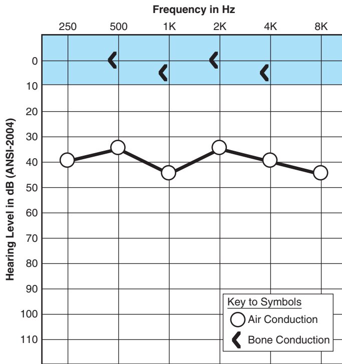
FIGURE 2-39 An audiogram demonstrating that when the outer or middle ears are not functioning normally, resulting in a conductive hearing loss, the intensity of the air-conducted signals must be raised before threshold is reached, while the bone-conduction thresholds remain normal.
