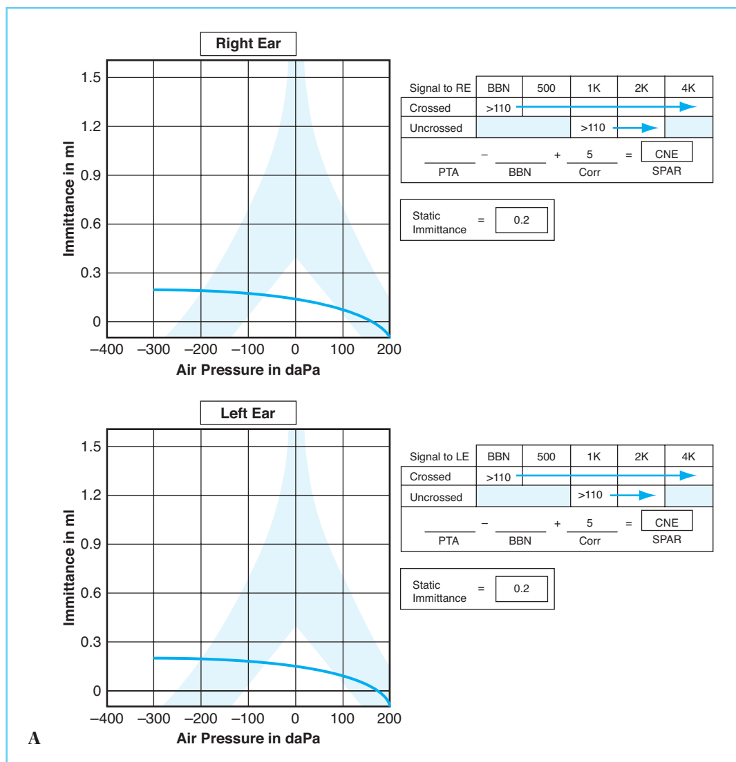
FIGURE 10-1 Hearing consultation results in a 4-year-old boy with a history of otitis media. Immittance measures (A) are consistent with an increase in the mass of the middle-ear mechanism, secondary to otitis media with effusion. Pure-tone audiometric results (B) show a mild conductive hearing loss bilaterally, with slightly more loss in the left ear. Speech audiometric results show excellent suprathreshold recognition of words and sentences once intensity level is sufficient to overcome the conductive hearing loss. (PSI- W_m = Pediatric Speech Intelligibility test maximum word score; PSI- S_m = PSI maximum sentence score; PSI-CCM = PSI with contralateral competing message.)
