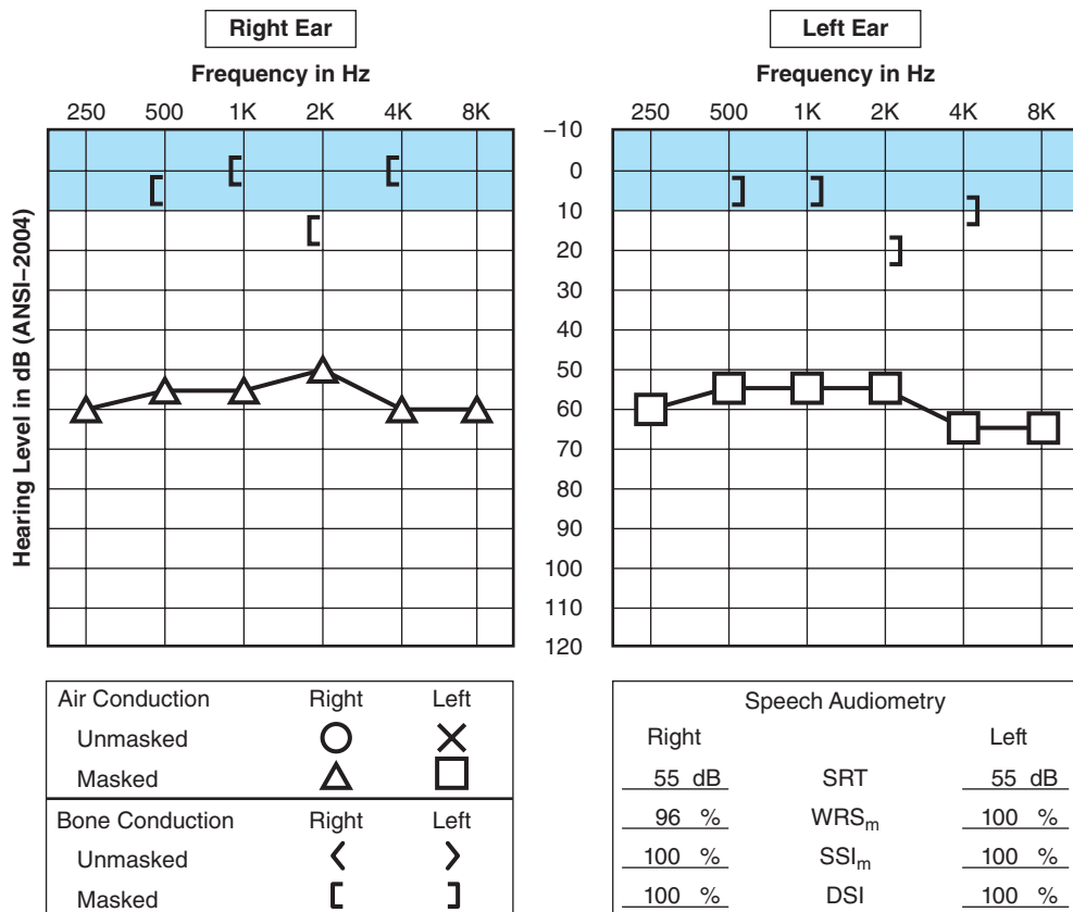
FIGURE 15-5 Hearing consultation results in a 19-year-old woman with intractable middle-ear disorder. Pure-tone and speech audiometric results (A) show flat conductive hearing loss and good suprathreshold speech-recognition ability bilaterally. Soundfield thresholds (B) show appropriate real-ear gain for both conventional hearing aids and a BAHA device.
