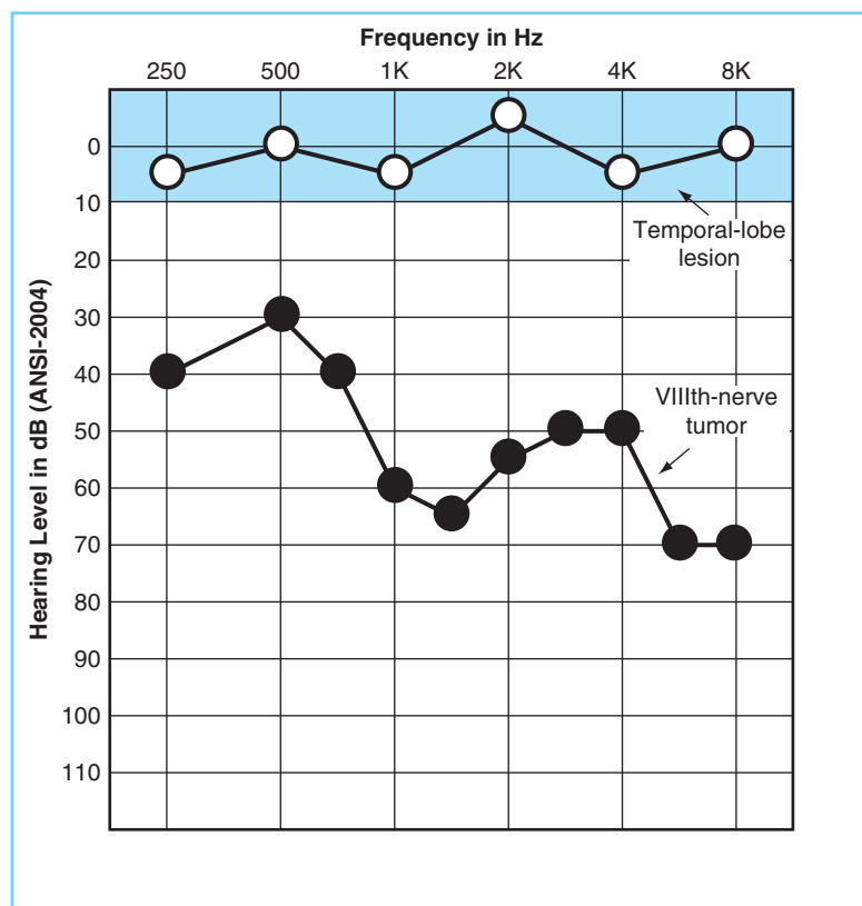
FIGURE 3-6 Representative audiometric outcomes resulting from temporal-lobe and VIIIth-nerve tumors.
