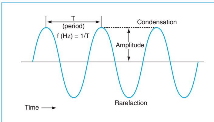
FIGURE 2-5 A sinusoidal waveform, describing the various properties of sound, including amplitude and frequency ( f ).
