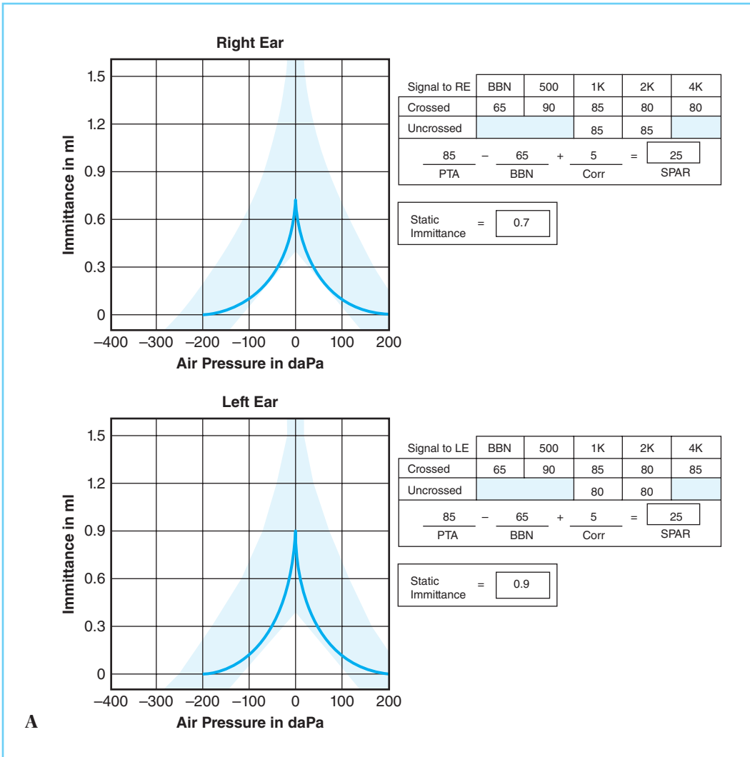
FIGURE 10-14 Hearing consultation results in a 6-year-old girl with auditory processing disorder. Immittance measures (A) are consistent with normal middle-ear function. Pure-tone audiometric results (B) show normal hearing sensitivity in both ears. Speech audiometric results (C) show significant rollover of PI functions for both word and sentence recognition. Results also show a dichotic deficit, with poorer performance on the left ear.
