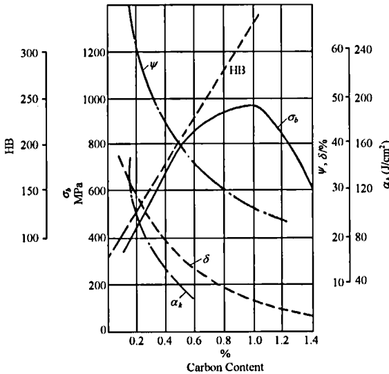
Figure 8.7 Influences of Carbon Content on Properties of Hot-rolled Carbon Steel \sigma_b . Tensile Strength ; \alpha_k .Impact Toughness; HB. Hardness; \delta . Elongation; \phi . Shrinkage of Cross-section
