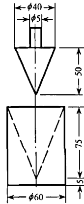
Test Figure 3.3 Normal Consistency Detector Test Figure 3.4 Test Cone and Cone Mold
