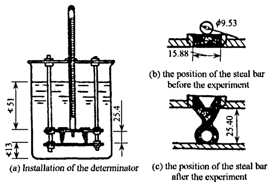
Test Figure 9.3 The Determinator of Softening Point
