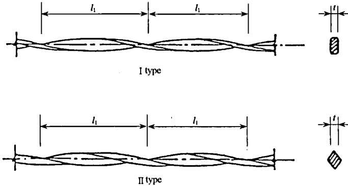
Figure 8.10 Shape and Cross-section of Cold-rolled-twisted Bar t , rolled thickness; l_1 , pitch
