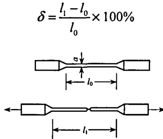
Figure 8.3 Elongation of Steel
