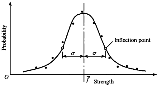
Figure 5.19 The Normal Distribution Curve of Concrete Strength
