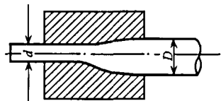
Figure 8.9 Cold Drawing
