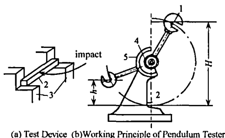
Figure 8.5 The Test Principle of Impact Durability
