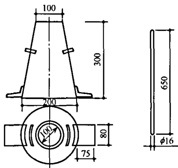
Test Figure 5.1 Slump Cone and Tamping Rod
