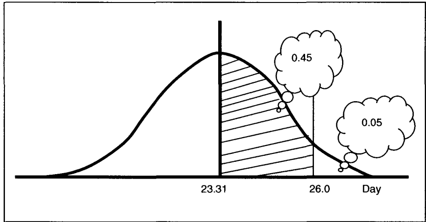
Figure 4.11 Probability distribution.
