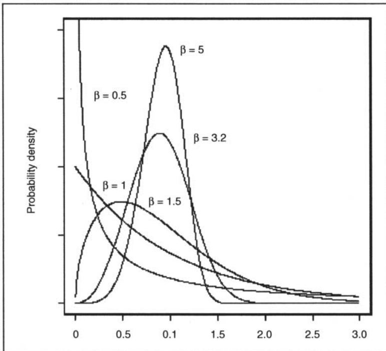
Figure 3.13 Weibull distribution.
