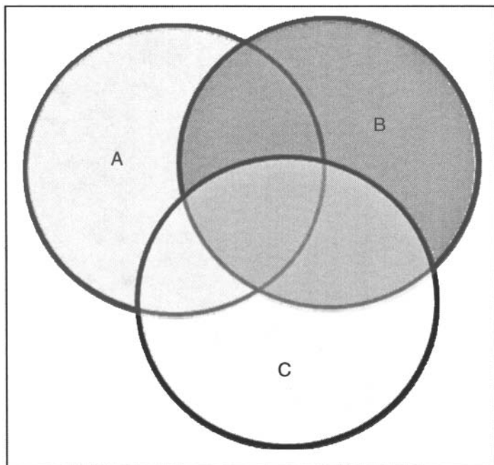
Figure 3.19 Probability theory.
