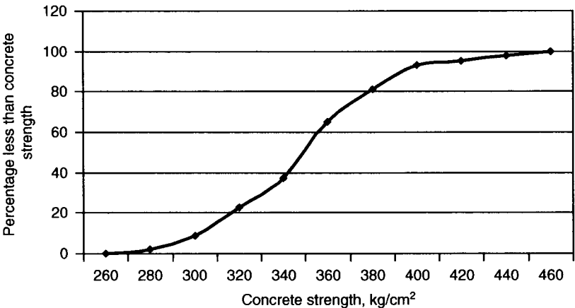
Figure 3.6 Cumulative distribution curve for concrete strength.
