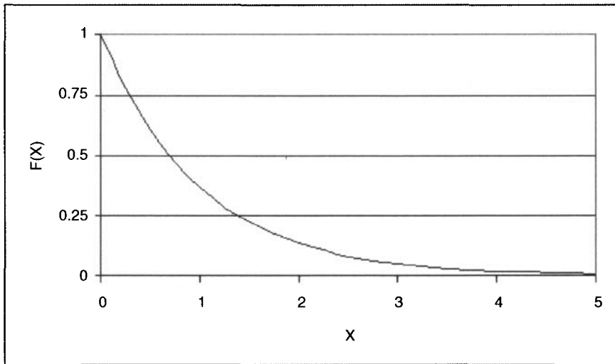
Figure 3.12 The exponential distribution.
