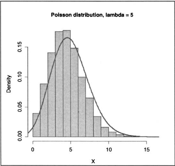
Figure 3.11 Poisson distribution.
