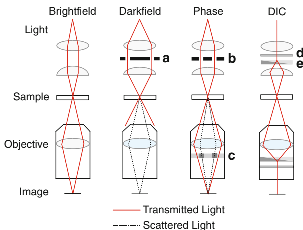
Fig. 1 Different illumination techniques for light microscopy. In brightfield, light is focused on the sample, collected by the objective, and focused to an image. In darkfield, an aperture ( a ) is placed before the condenser lens to create a hollow cone of light that is focused on the sample. The objective collects scattered light and rejects directly transmitted light, producing a bright image on a dark background. In phase contrast, an annulus ( b ) is placed before the condenser, and both the scattered light and directly transmitted light are collected and focused to an image. A phase plate ( c ) in the objective modulates the phase of transmitted light relative to the scattered light such that they interfere at the image plane to create contrast. In differential interference contrast (DIC), light is polarized with a filter ( d ) and split by a prism ( e ) to create two beams that take different optical path lengths through the sample. The beams interfere upon being recombined, producing contrast proportional to the optical path lengths
