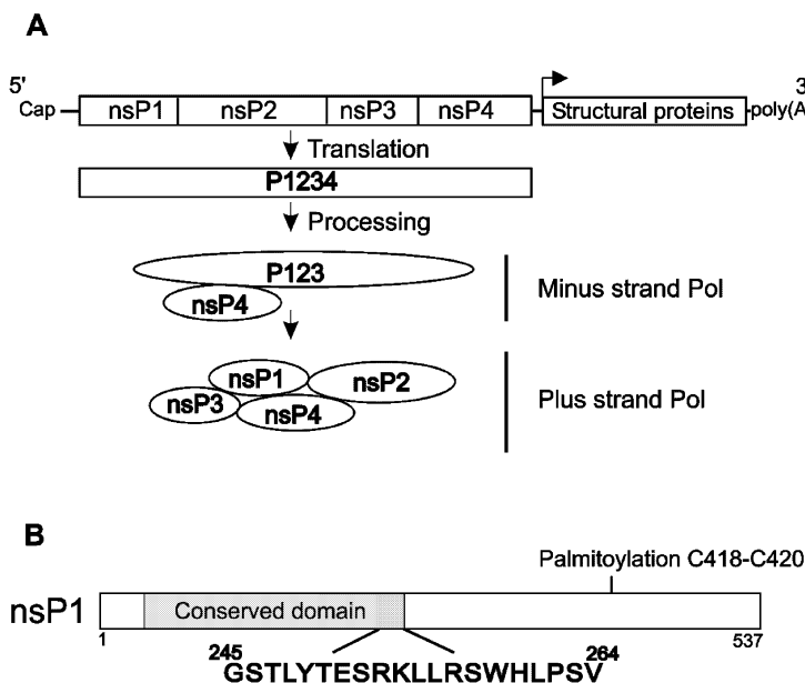
Fig. 1. A Genome organization of SFV. The translation and processing products relevant for SFV replication are shown. Physical interactions have been identified between nsP1 and nsP4, as well as nsP1 and nsP3 (Salonen et al. 2003). B Scheme of SFV nsP1 showing the two regions responsible for membrane binding. The amino acid sequence of the lipid binding peptide is given in single-letter code , and the position of palmitoylated cysteines is marked
