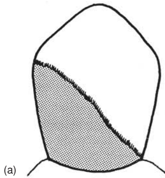
Fig. 24.6 The four basic survey lines with the undercut areas shaded:
