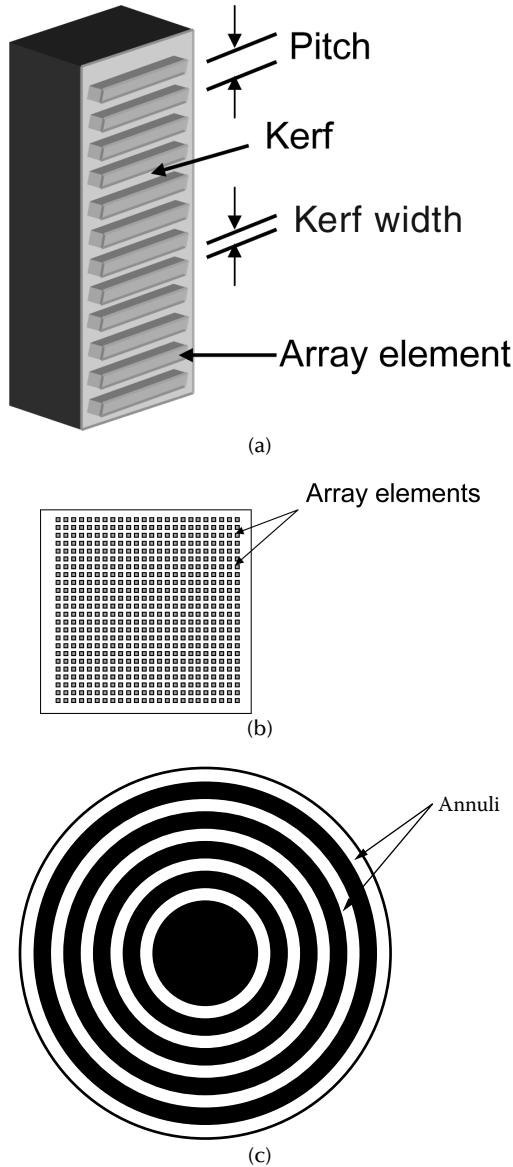
FIGURE 3.24 (a) Linear array; (b) two-dimensional array; and (c) annular array.
