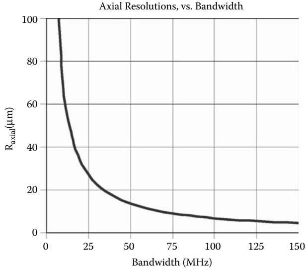
FIGURE 8.1 Calculated axial resolution as a function of bandwidth.
