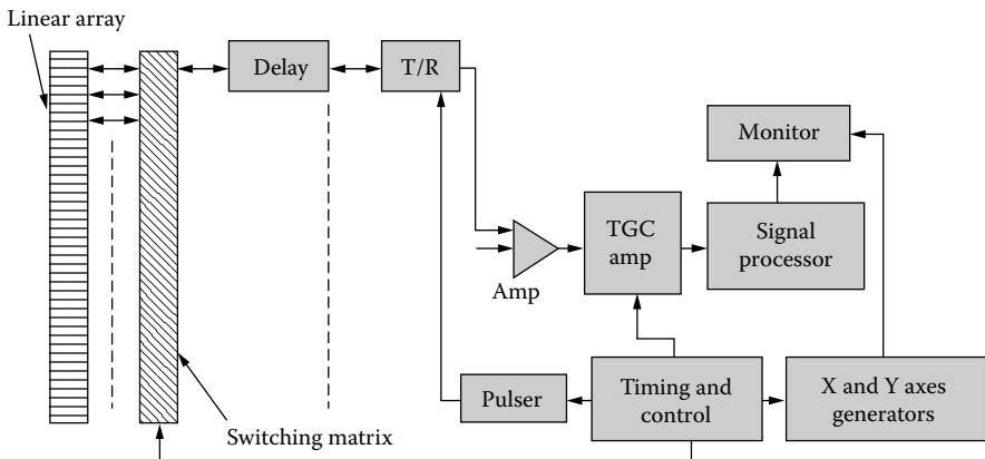
Analog imaging architecture
