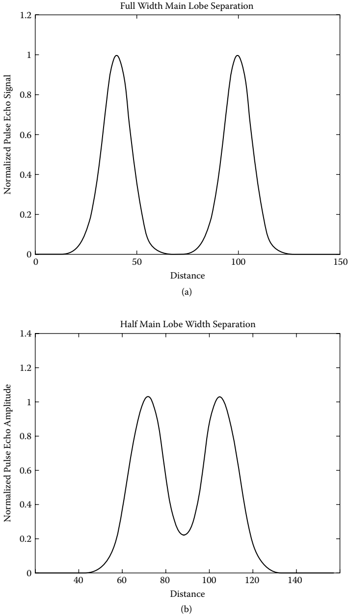
FIGURE 3.21 The spatial resolutions of an ultrasonic transducer in the axial and lateral directions are determined by the pulse duration and beam width.
