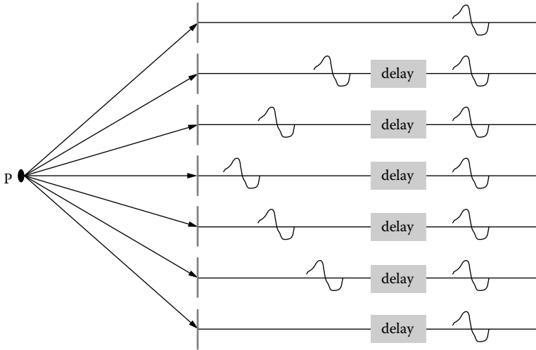
FIGURE 3.28 The echoes returned from a point scatterer at point P can be made to arrive at the same time by appropriately delaying the echoes detected at the elements of a linear array.
