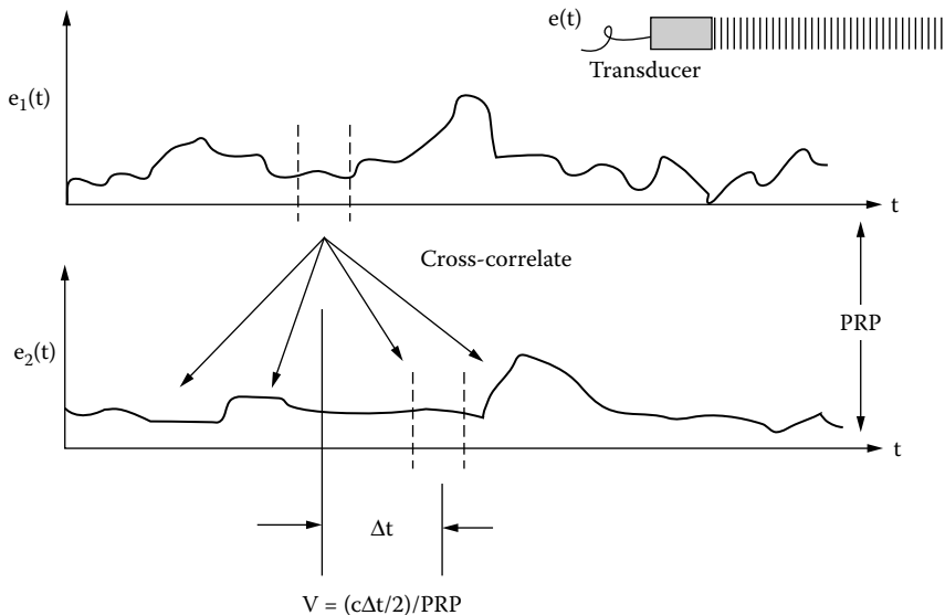
FIGURE 6.7 Cross-correlation can be used to estimate blood flow in time domain.
