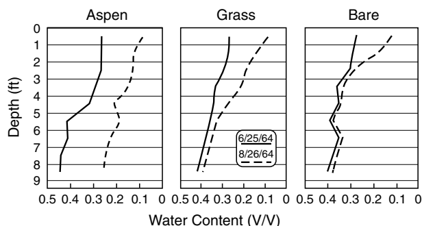
FIGURE 10.5 Evapotranspiration from aspen, grass, and bare plots. (After Johnston, R.S., Water Resour. Res. , 6:324–327, 1970.)
