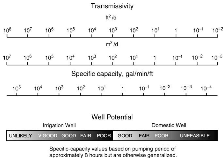
FIGURE 11.6 Bar chart for range of transmissivity values relative to the potential of various types of wells. (Modified from Bureau of Reclamation, Ground Water Manual , U.S. Department of the Interior, Washington, DC, 1977.)
