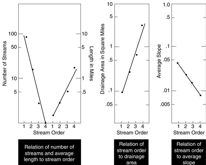
FIGURE 14.12 Stream ordering for Clarksville, MD, watershed.
