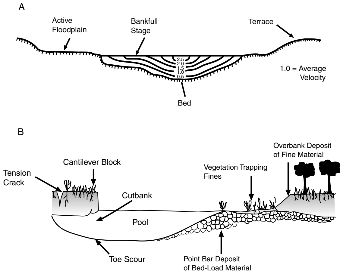
FIGURE 6.13 Typical channel cross section at (A) a straight reach showing velocity distributions ( isovels ) and (B) a bend showing a pool, cut bank, and formation of a point bar.
