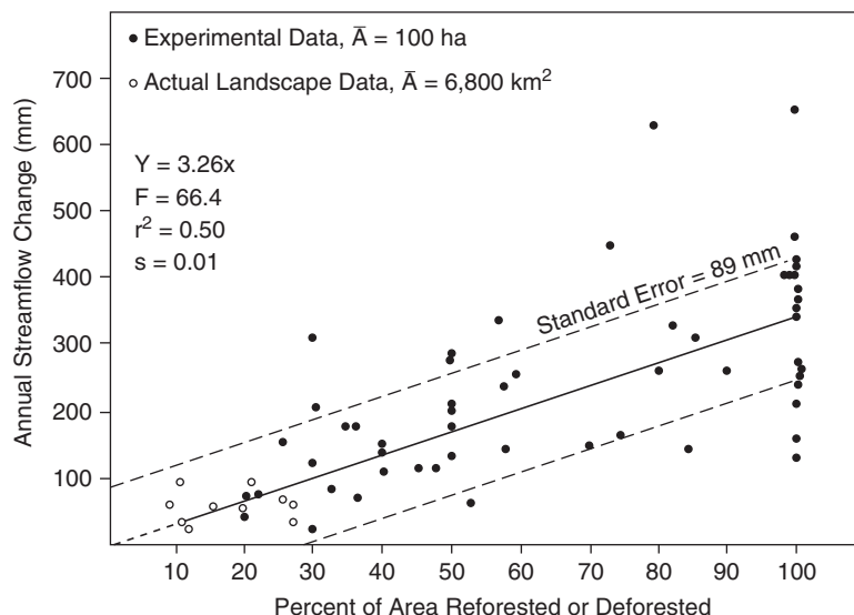
FIGURE 10.12 Regression model to predict the effect of forest change in a watershed. (Redrawn from Trimble, S.W., F. Weirich, and B.L. Hoag, Water Resour. Res. , 23:425–437, 1987. See also Calder, I.R., Hydrologic effects of land use, in Handbook of Hydrology , D. Maidment, Ed., McGraw-Hill, New York, 1993, pp. 13.18.) (Experimental data, \bar{A} = 100 ha from Bosch, J.M., and J.D. Hewlett, Hydrology , 55:2–23, 1982. Actual landscape data, \bar{A} = 6800 km 2 from Trimble, S.W., F. Weirich, and B.L. Hoag, Water Resour. Res. , 23:425–437, 1987.)
