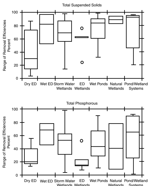
FIGURE 12.20 Pollutant removal performance for stormwater ponds and wetlands. (From Schueler, T.R., Design of Stormwater Wetland Systems: Guidelines for Creating Diverse and Effective Stormwater Wetland Systems in the Mid-Atlantic Region , Anacostia Restoration Team, Department of Environmental Programs, Metropolitan Washington Council of Governments, Washington, DC, 1992. With permission.)
