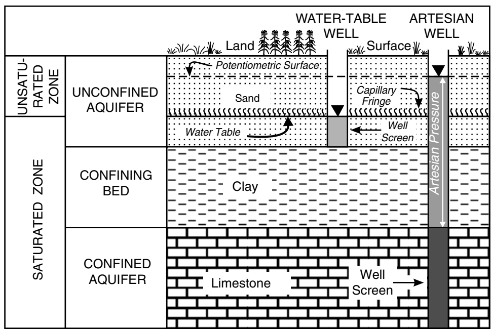
FIGURE 11.7 Diagram showing hydrogeologic conditions for an unconfined aquifer and a confined aquifer. (Modified from Heath, R.C., Basic Ground-Water Hydrology , U.S. Geological Survey Water Supply Paper 2220, U.S. Government Printing Office, Washington, DC, 1983.)
