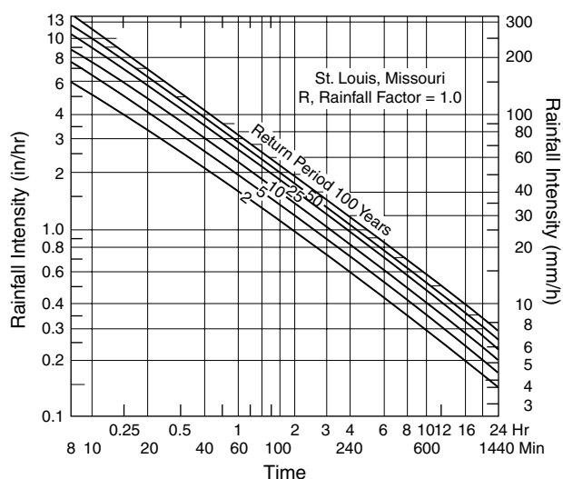
FIGURE 2.17 Rainfall rate-duration-frequency distribution for St. Louis, MO. (From Hershfield, D.N., Rainfall Frequency Atlas of the United States , U.S. Weather Bureau Technical Paper 40, 1961, and Weiss, L.L., Monthly Weather Rev. , 90:87–88, 1962.)
