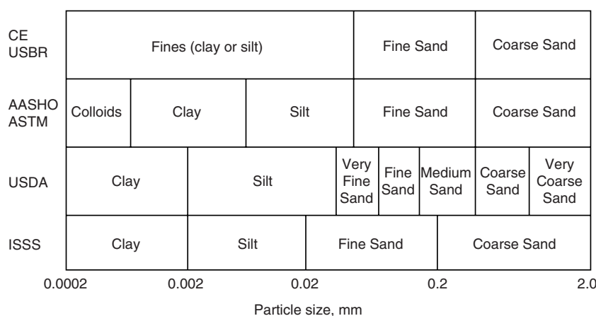
FIGURE 3.1 Soil classification based on particle size (AASHTO = American Association of State Highway Officials; ASTM = American Society for Testing and Materials; CE = Corps of Engineers; ISSS = International Society of Soil Science; USBR = U.S. Bureau of Reclamation; USDA = U.S. Department of Agriculture).
