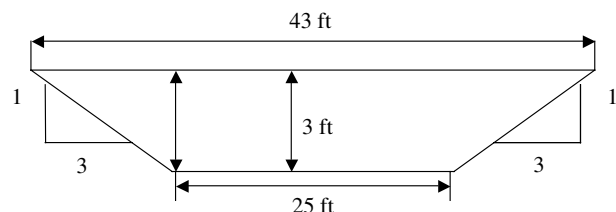
FIGURE 7.2 Cross section of channel for Example 7.4.
