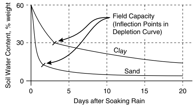
FIGURE 3.7 The elusive nature of field capacity.
