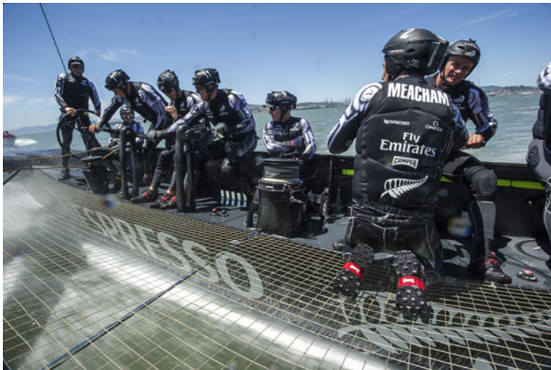
Fig. 22.7 Onboard Emirates Team New Zealand AC72, NZL5 during testing June 14, 2013. Helmsman steering and crew-members sail trimming, grinding, and top-handle winching shown (Photo: Chris Cameron)
