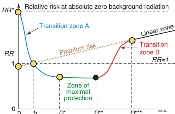
Fig. 4.1 Schematic representation of cancer relative risk (RR) showing the hormesis relative risk model. D is radiation dose or exposure level or exposure rate (for continuous lifetime exposure). The variable b is the natural background radiation level. RR = 1 at the natural background exposure level. RR^* is the relative risk in the absence of any radiation exposure. The reference to phantom risk relates to use of the invalid linear no-threshold LNT hypothesis to extrapolate from high- to low-radiation doses (With kind permission of Bobby Scott [17])
