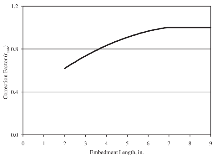
Figure 6. Adjustment factor for embedment length.
