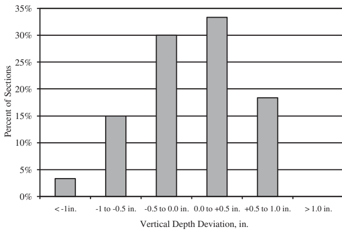
Figure 3. Distribution of vertical dowel bar translations.
