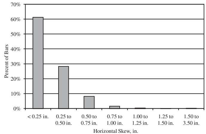
Figure 4. Distribution of the horizontal skew.
