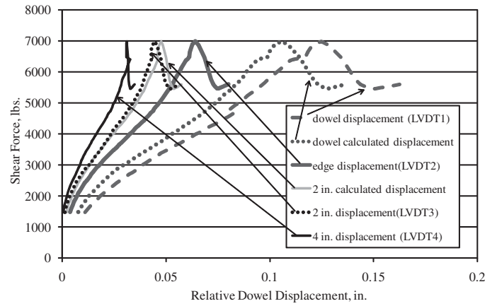
Figure 2.11. Measured and calculated force versus displacement for a 2 in. vertically tilted dowel.
