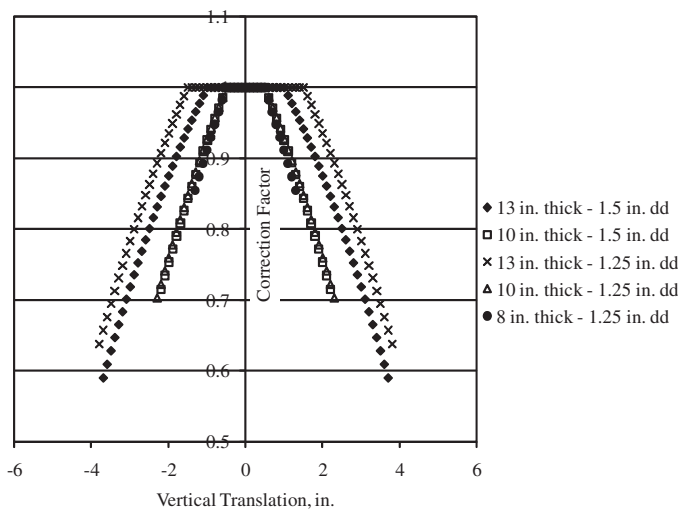
Figure 3.16. Concrete cover adjustment factors ( r_{cc} ) versus vertical translation for combinations of dowel diameter and PCC thickness.
